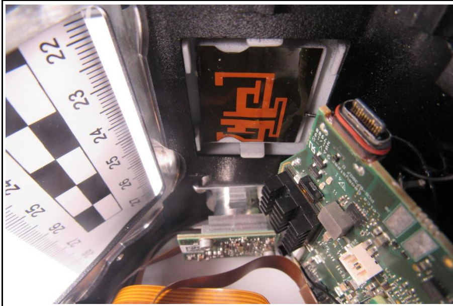
WLAN/BT Antenna 2
