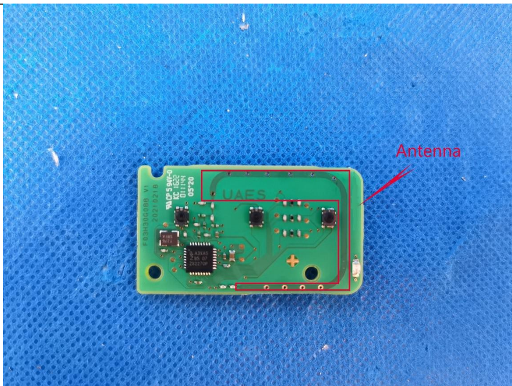
EUT Photo(6)-Antenna
