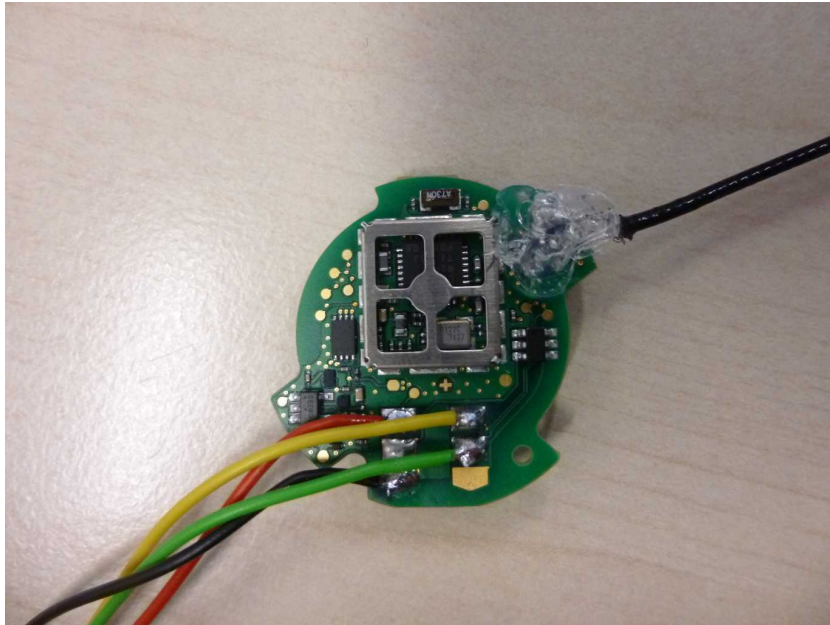
Photo 3: PCB back side view, without shielding
