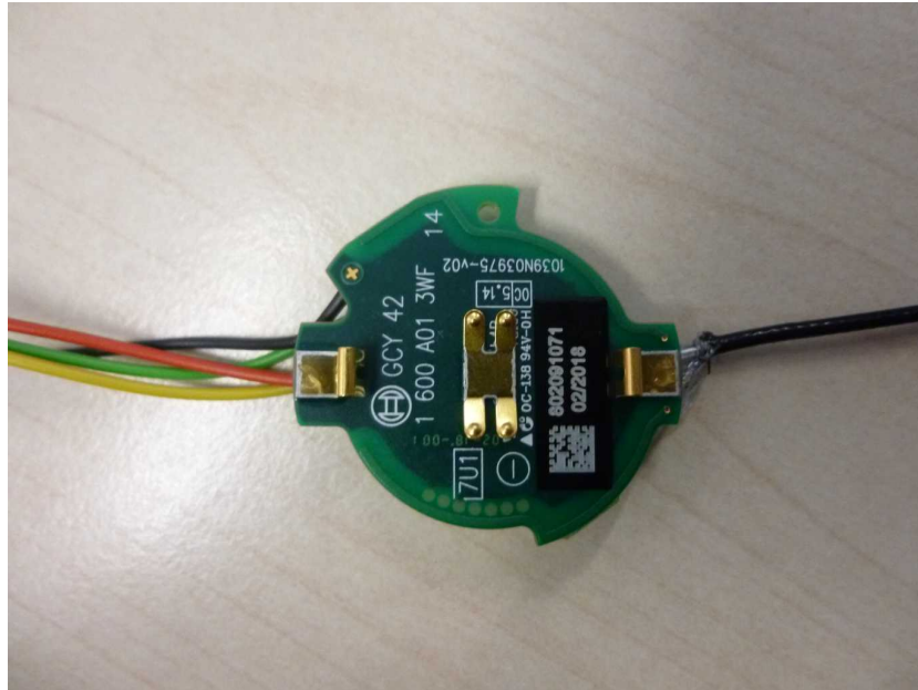
Photo 1: PCB front side view
