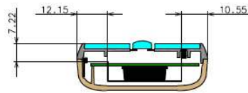
Sec. A-A (Plate antenna)
