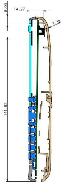
Sec. C-C (Plate antenna)
