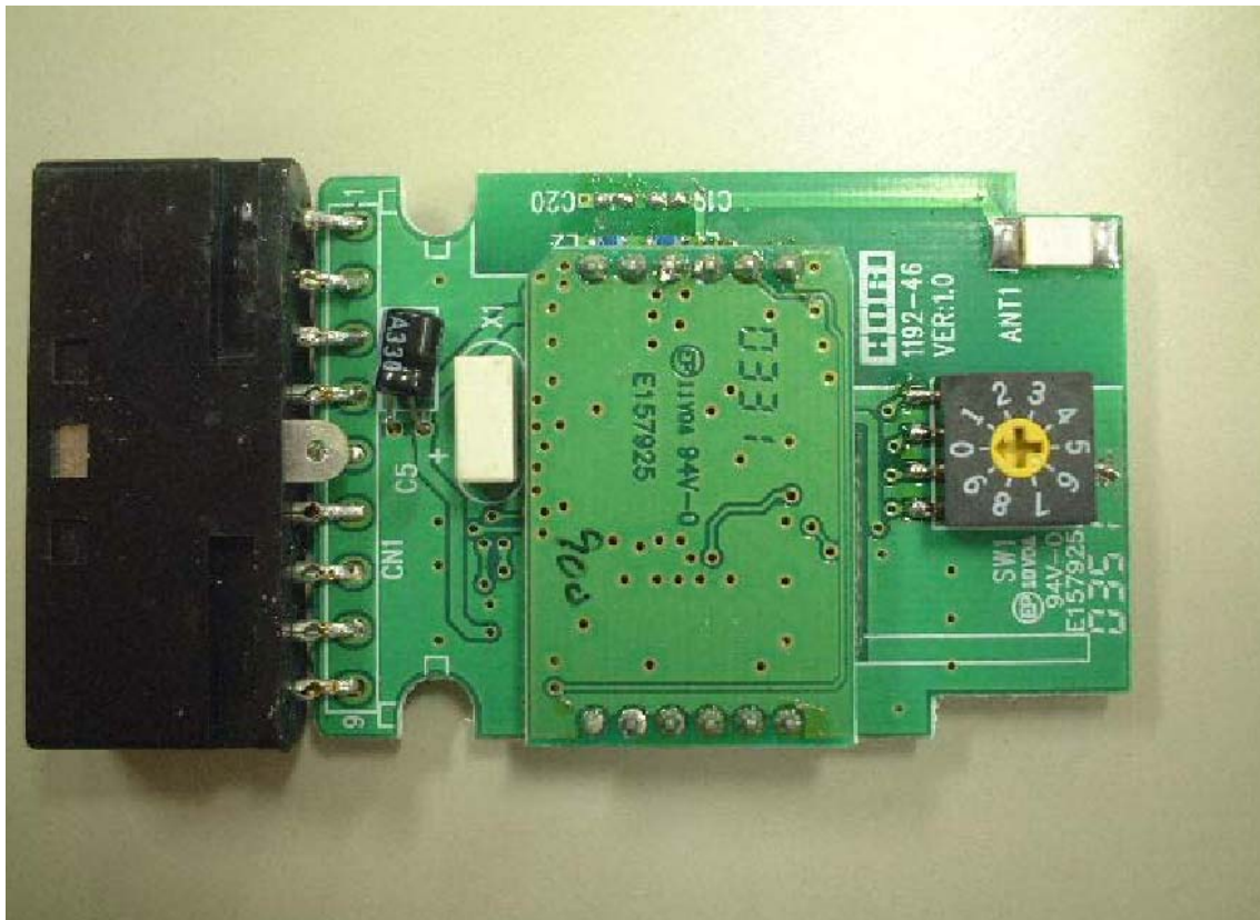
Location of RF Module
