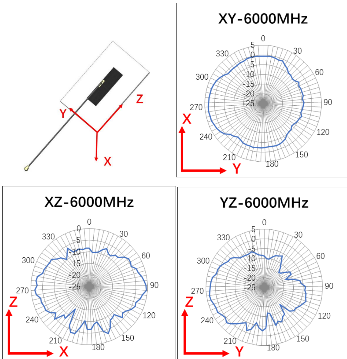
FIGURE 4.5.3 2D RADIATION PATTERN OF ANTENNA AT 6000MHZ IN FREE SPACE
