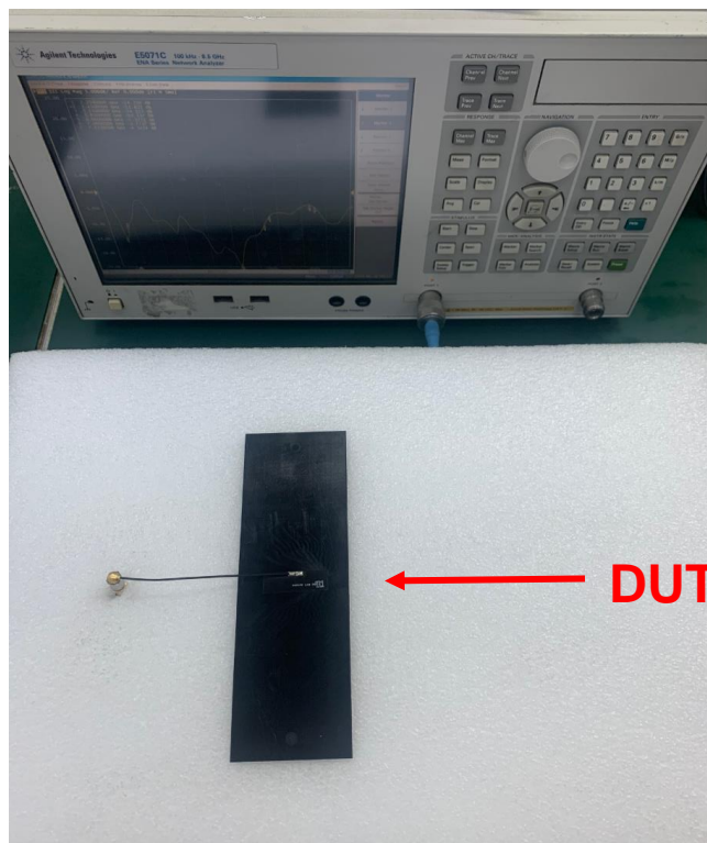
FIGURE 4.1.2 ANTENNA LOADED WITH PC/ABS BLOCK OF 1.5 MM THICKNESS WITH VNA
