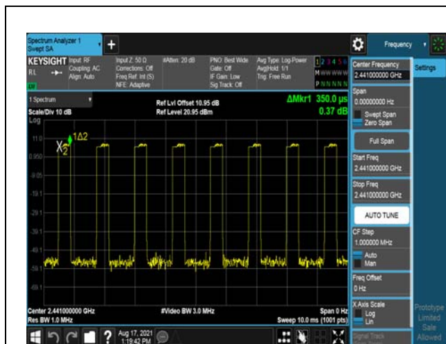
Modulation: 8DPSK DH1 2441MHz
