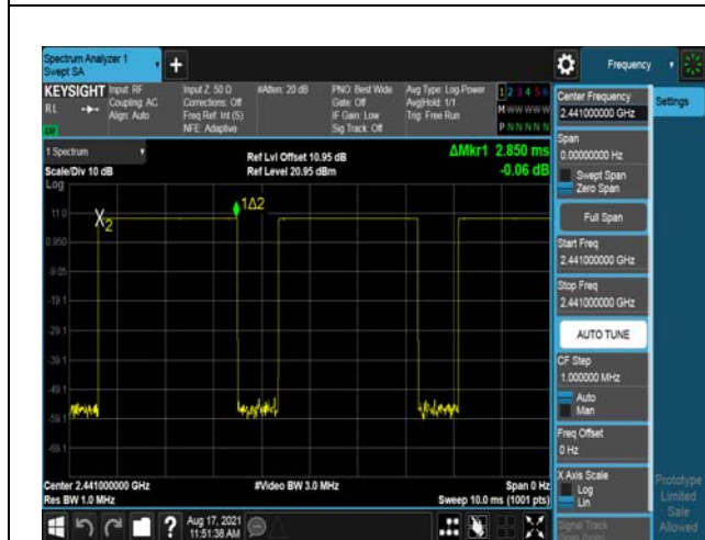
Modulation: GFSK DH5 2441MHz
