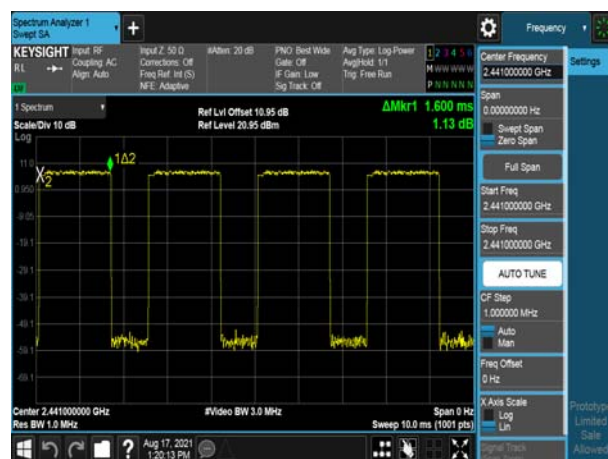
Modulation: 8DPSK DH3 2441MHz
