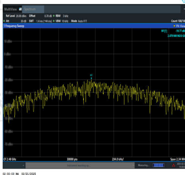
BLE_2M-Ant1-2480-PASS
