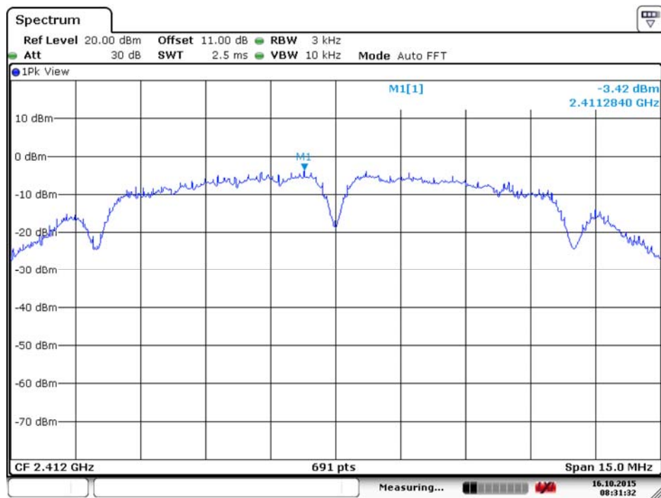
802.11b - Channel 1
