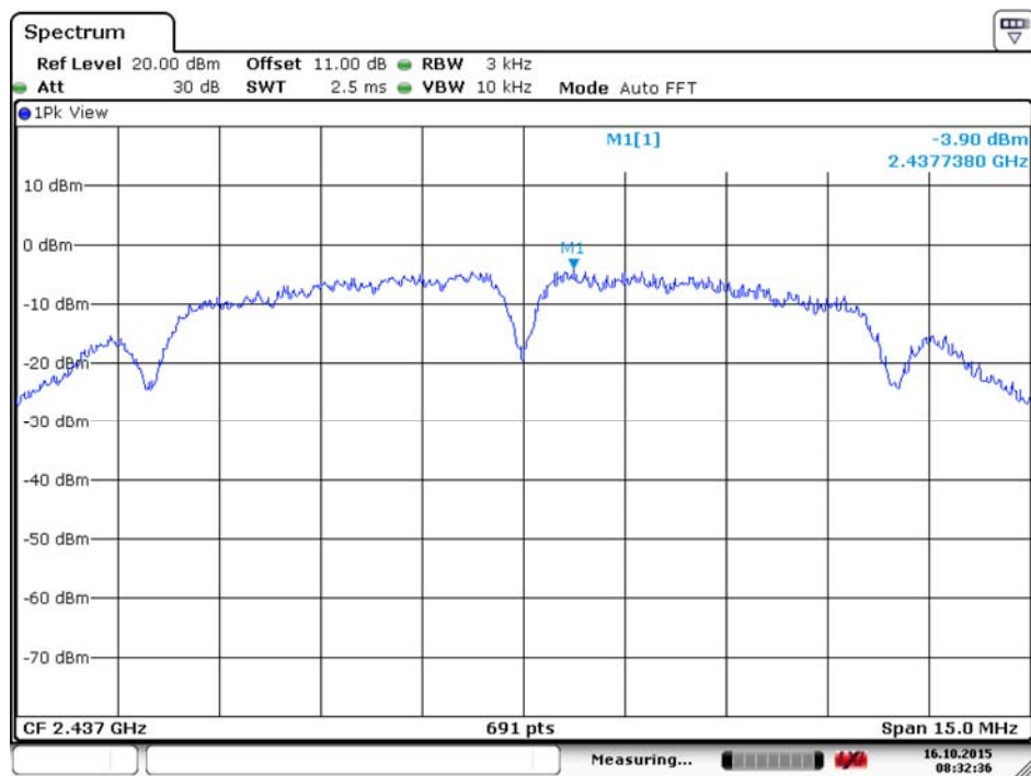
802.11b - Channel 6
