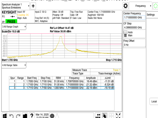
Band70_5MHz_QPSK_RB1_24_CH133097
