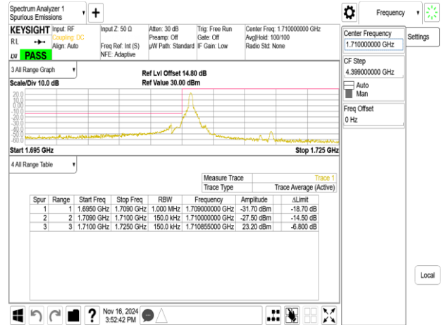
Band66_15MHz_QPSK_RB75_0_CH132047
