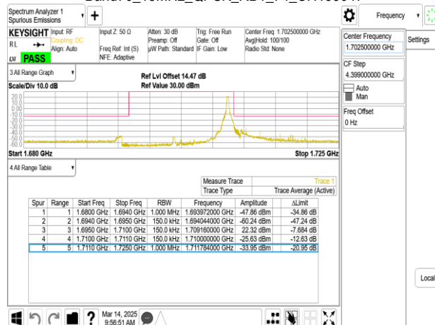
Band70_15MHz_QPSK_RB75_0_CH133047
