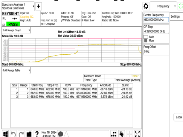
Band71_15MHz_QPSK_RB75_0_CH133197
