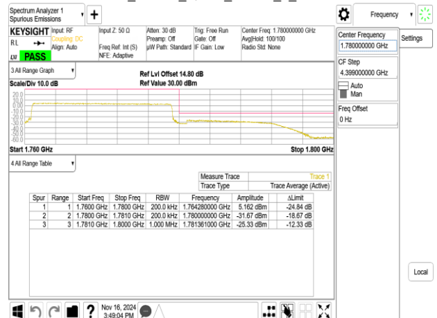
Band66_20MHz_QPSK_RB100_0_CH132572
