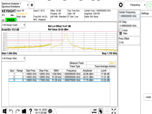
Band70_5MHz_QPSK_RB25_0_CH132997
