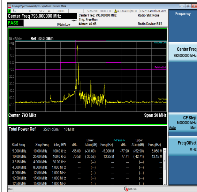
NTNV-Band14-10MHz-QPSK-23330-1RB#0-PASS
