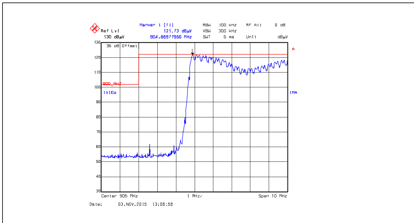
Plot 5.5.4.2.26. Band-Edge RF Radiated Emissions at 3 m, Horizontal Polarization Pseudorandom Hopping Mode, Low End of Frequency Band, 905.0 MHz, XTC0, Data Rate at 10 kbps
