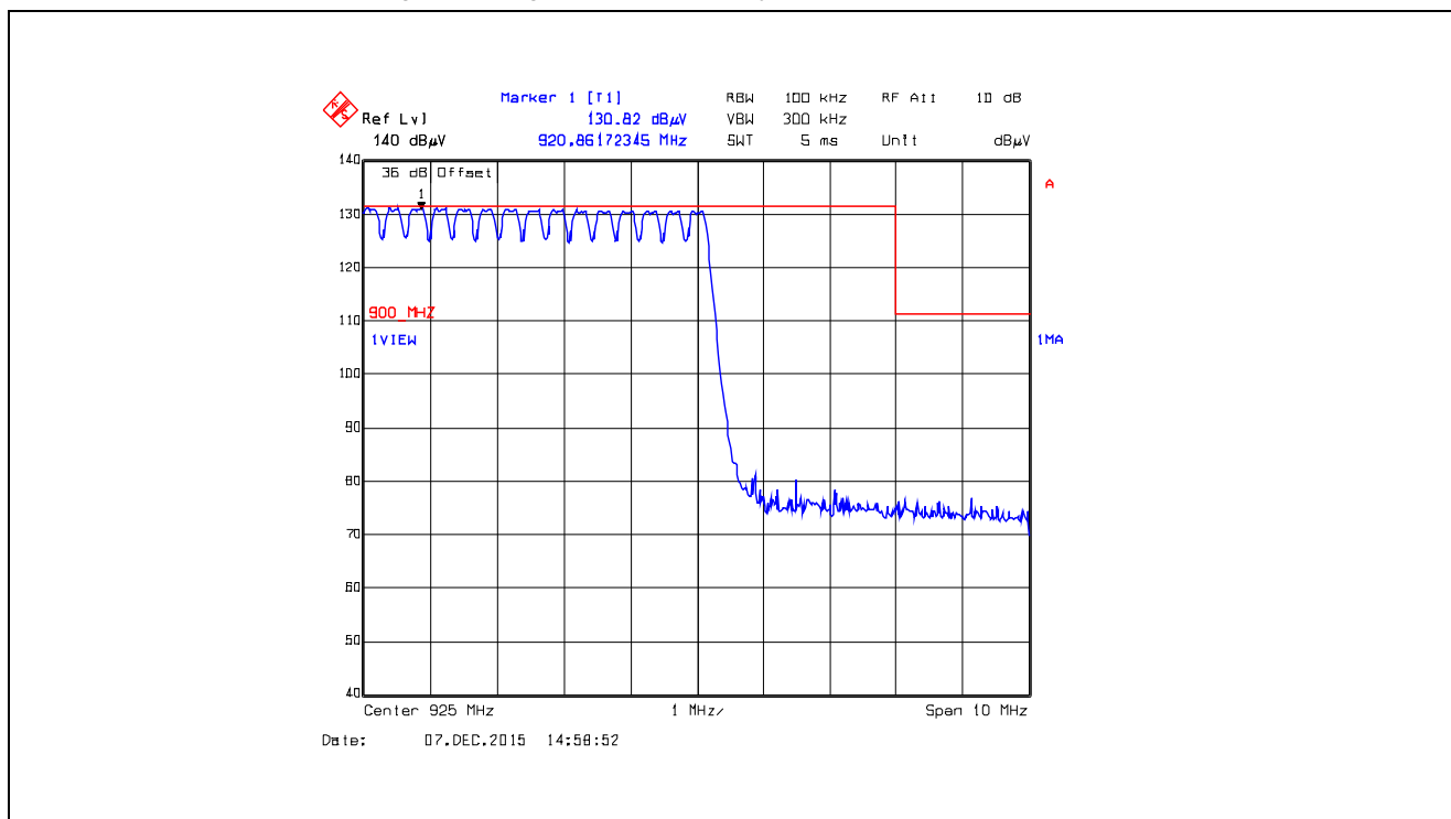
Plot 5.5.4.5.2.38. Band-Edge RF Radiated Emissions at 3 m, Horizontal Polarization Pseudorandom Hopping Mode, High End of Frequency Band, 925.0 MHz, XTC1, Data Rate at 125 kbps
