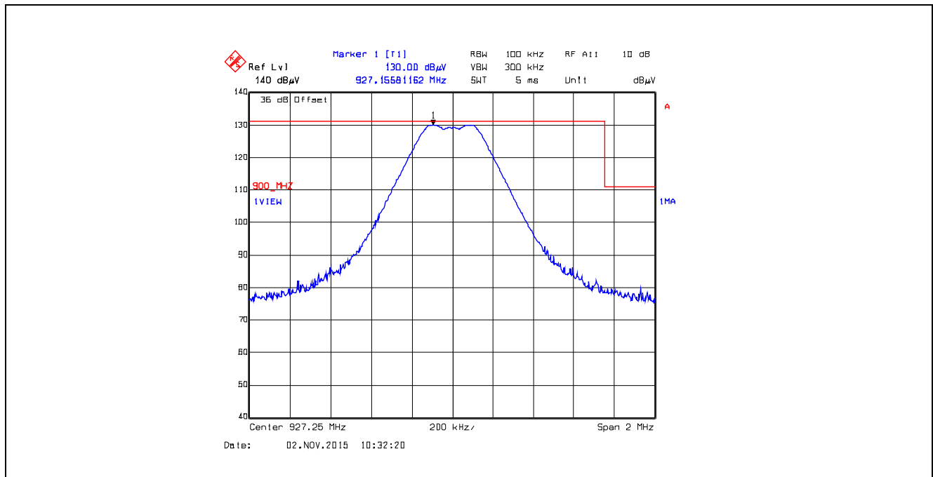
Plot 5.5.4.4.2.21. Band-Edge RF Radiated Emissions at 3 m, Horizontal Polarization Single Frequency Mode, High End of Frequency Band, 927.25 MHz, XB2, Data Rate at 250 kbps
