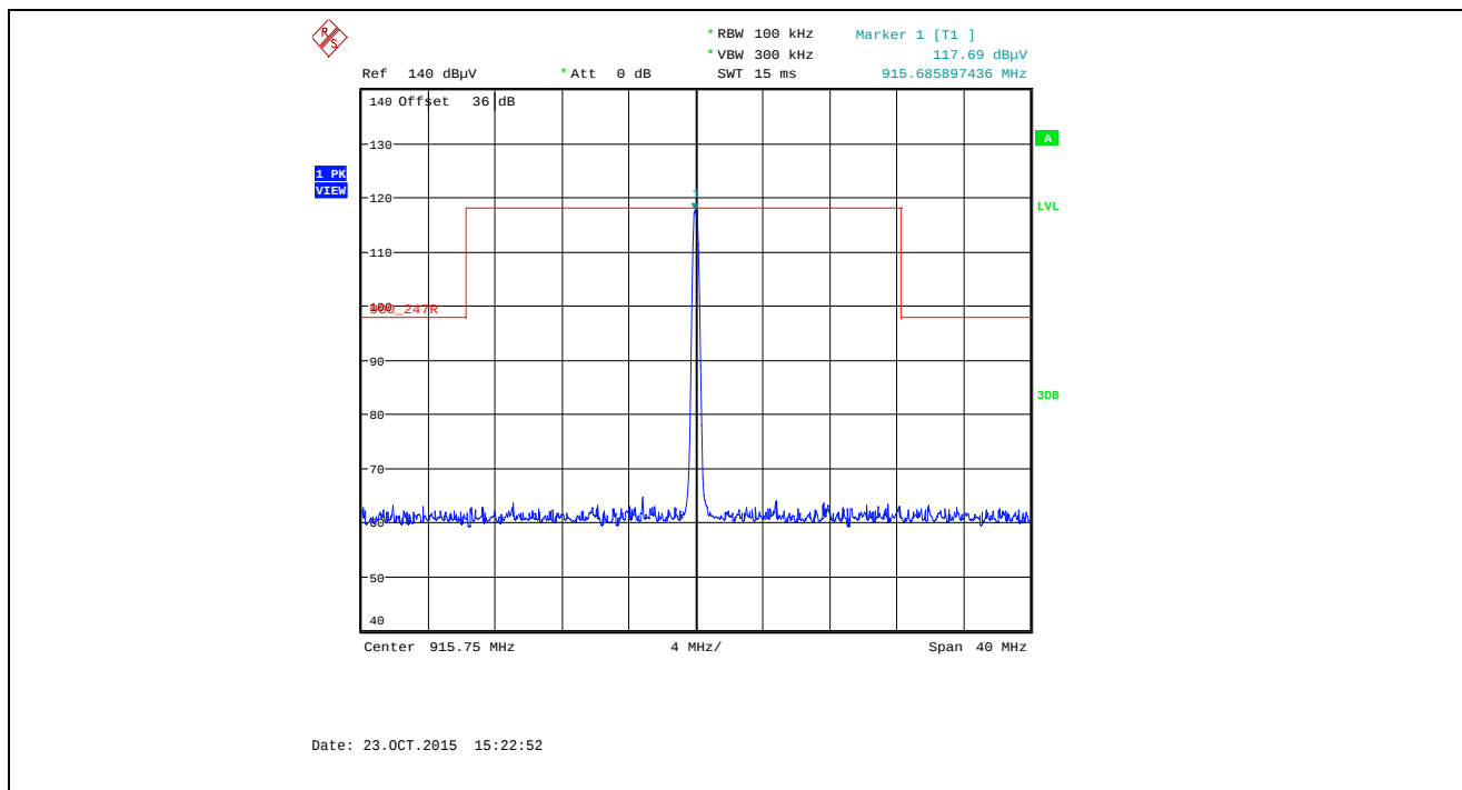
Plot 5.5.4.3.2.41. Band-Edge RF Radiated Emissions at 3 m, Horizontal Polarization Single Frequency Mode, Low End of Frequency Band, 915.75 MHz, XTCA0, Data Rate at 10 kbps
