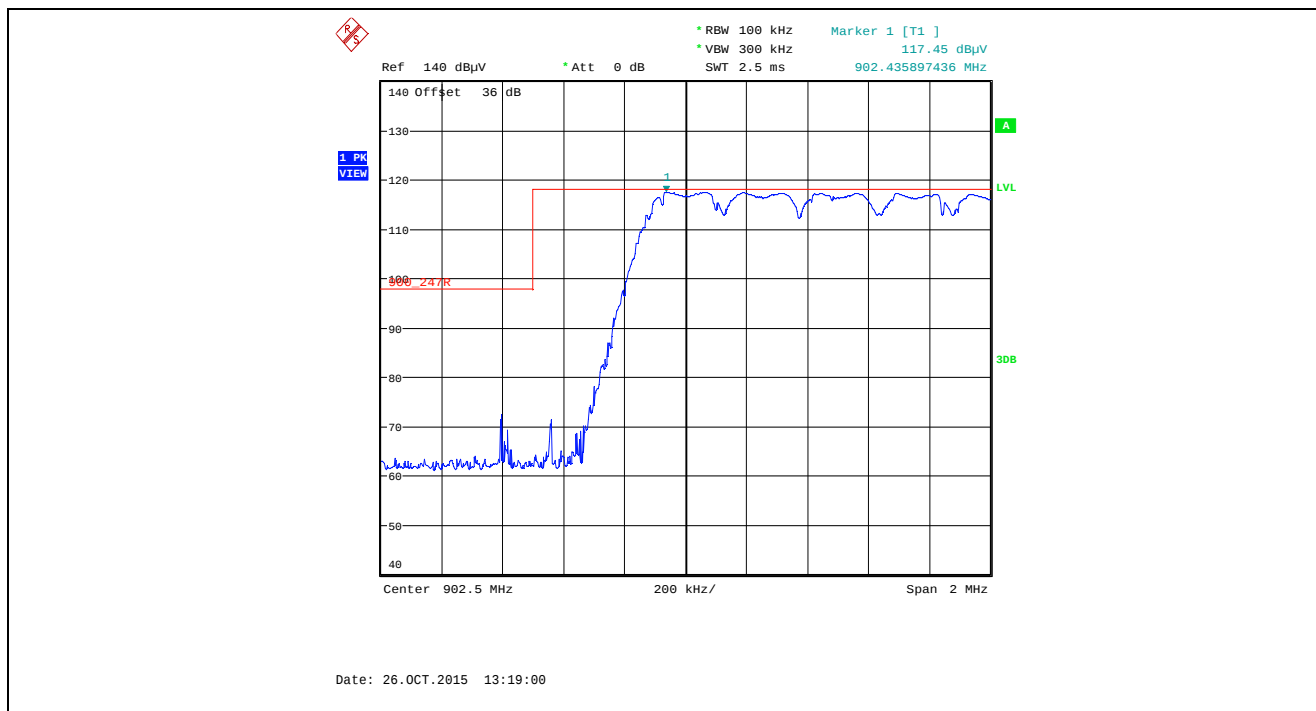
Plot 5.5.4.3.2.10. Band-Edge RF Radiated Emissions at 3 m, Horizontal Polarization Pseudorandom Hopping Mode, Low End of Frequency Band, 902.5 MHz, XB1, Data Rate at 110 kbps
