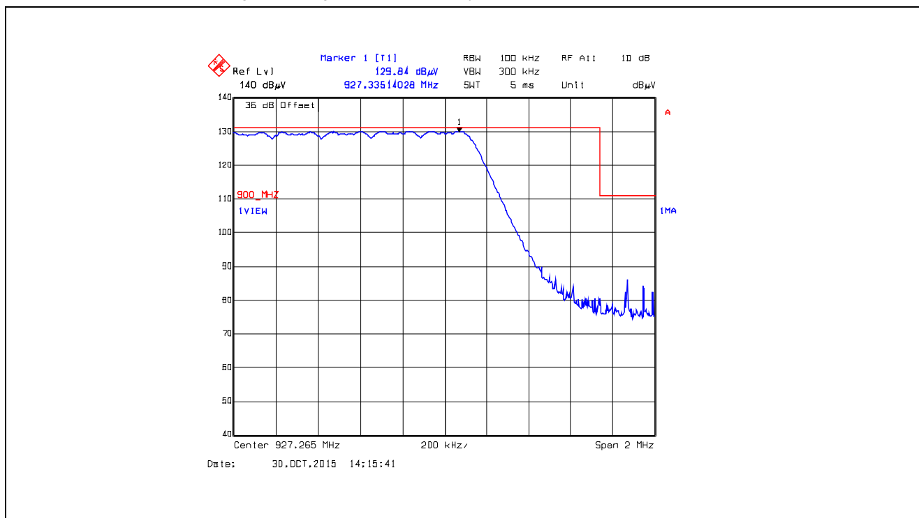
Plot 5.5.4.4.2.56. Band-Edge RF Radiated Emissions at 3 m, Vertical Polarization Pseudorandom Hopping Mode, High End of Frequency Band, 927.265 MHz, XTCA1, Data Rate at 105kbps
