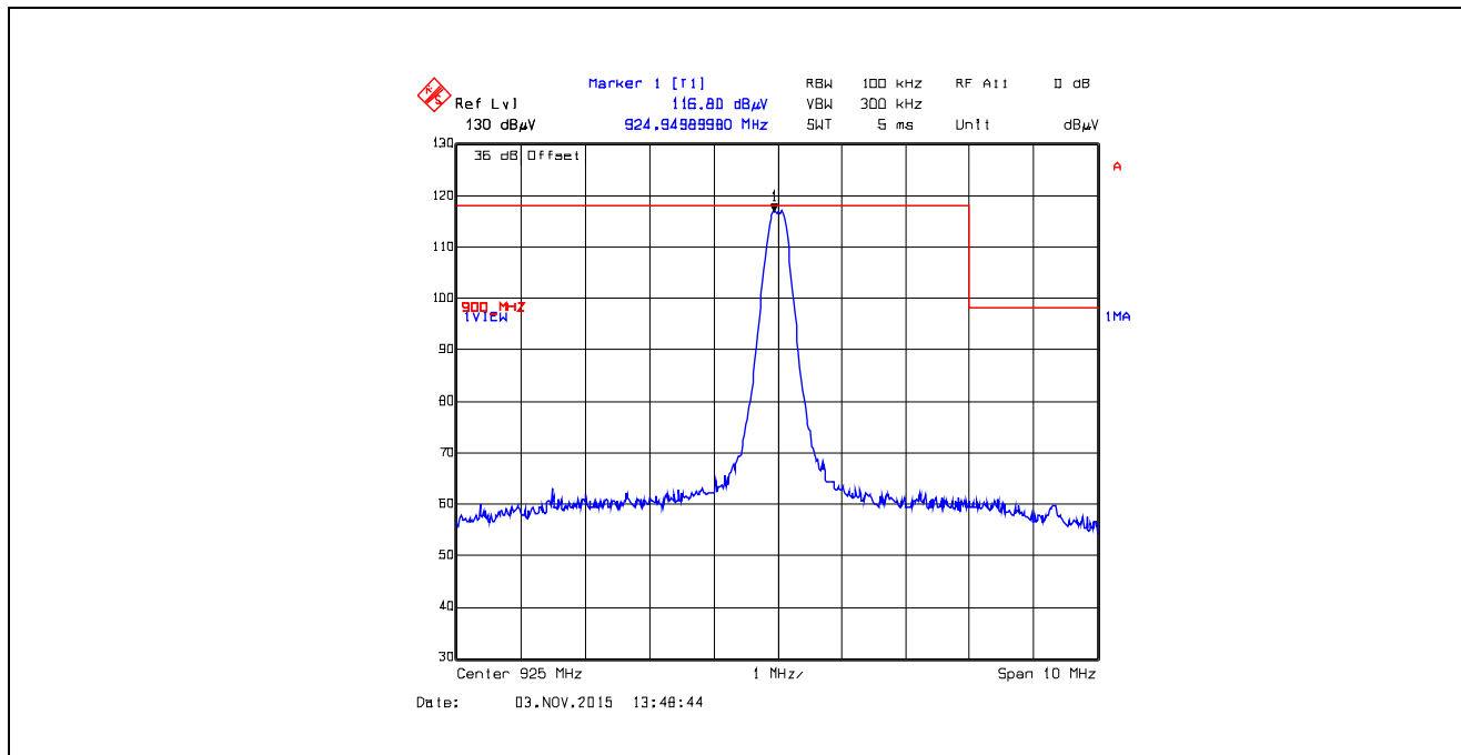
Plot 5.5.4.2.2.38. Band-Edge RF Radiated Emissions at 3 m, Horizontal Polarization Pseudorandom Hopping Mode, High End of Frequency Band, 925.0 MHz, XTC1, Data Rate at 125 kbps
