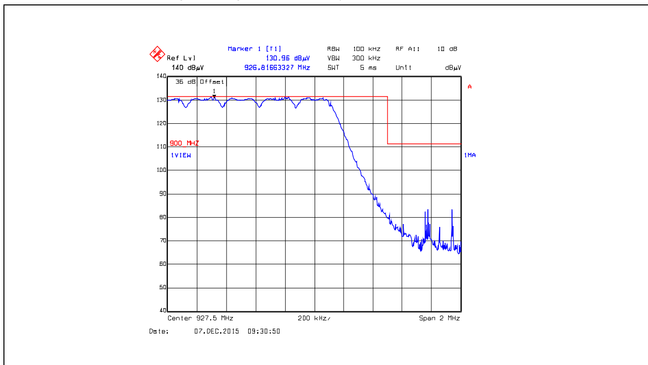
Plot 5.5.4.5.2.16. Band-Edge RF Radiated Emissions at 3 m, Vertical Polarization Pseudorandom Hopping Mode, High End of Frequency Band, 927.5 MHz, XBX1, Data Rate at 110 kbps
