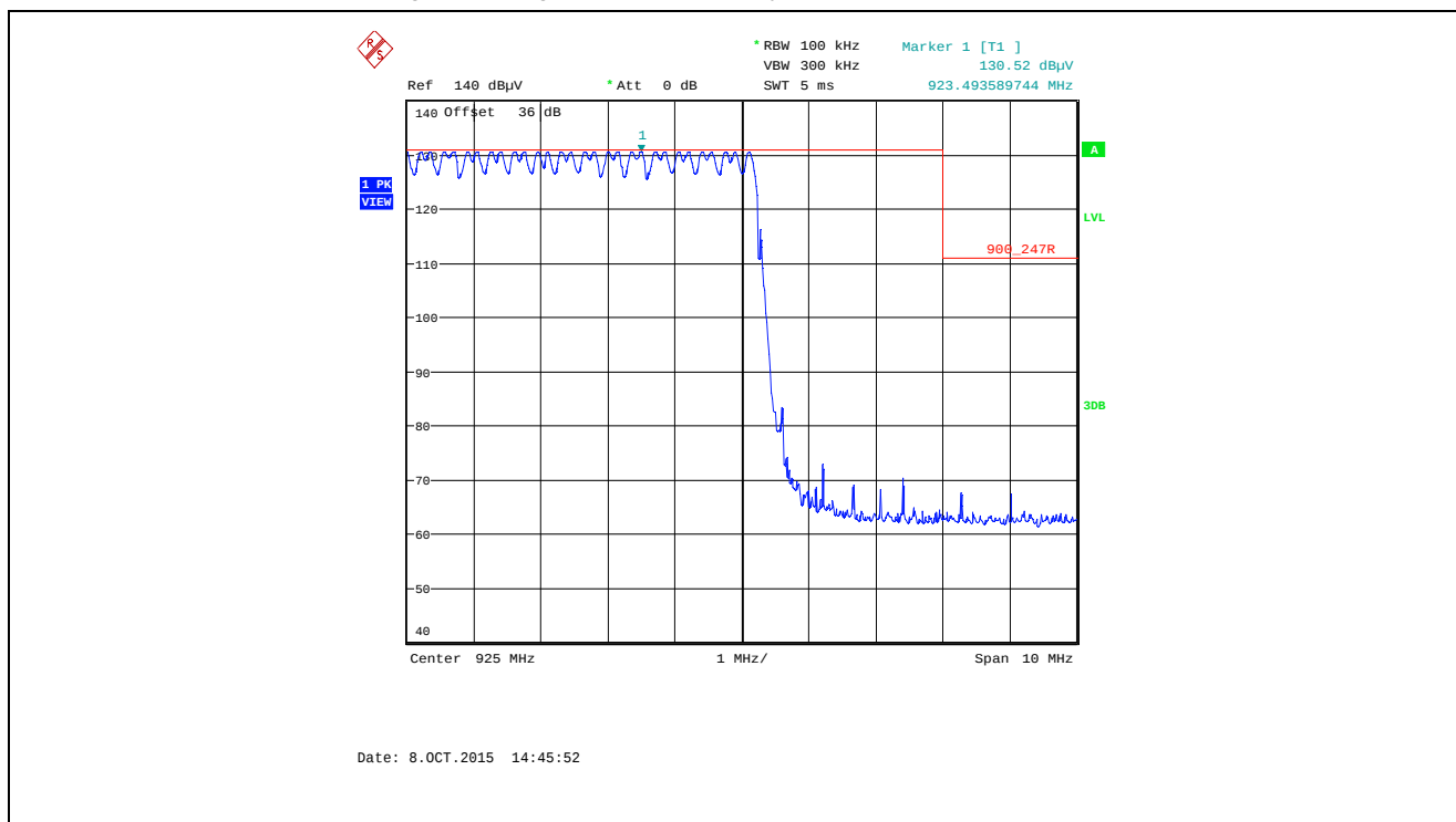
Plot 5.5.4.1.2.30. Band-Edge RF Radiated Emissions at 3 m, Horizontal Polarization Pseudorandom Hopping Mode, High End of Frequency Band, 925.0 MHz, XTC0, Data Rate at 10 kbps
