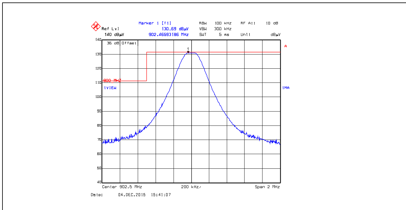
Plot 5.5.4.5.2.3. Band-Edge RF Radiated Emissions at 3 m, Vertical Polarization Single Frequency Mode, Low End of Frequency Band, 902.5 MHz, XB0, Data Rate at 10 kbps
