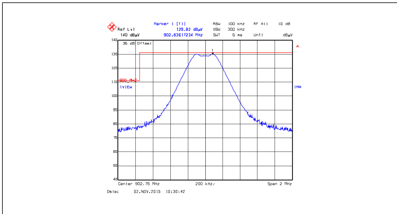
Plot 5.5.4.4.2.17. Band-Edge RF Radiated Emissions at 3 m, Horizontal Polarization Single Frequency Mode, Low End of Frequency Band, 902.75 MHz, XBX2, Data Rate at 250 kbps
