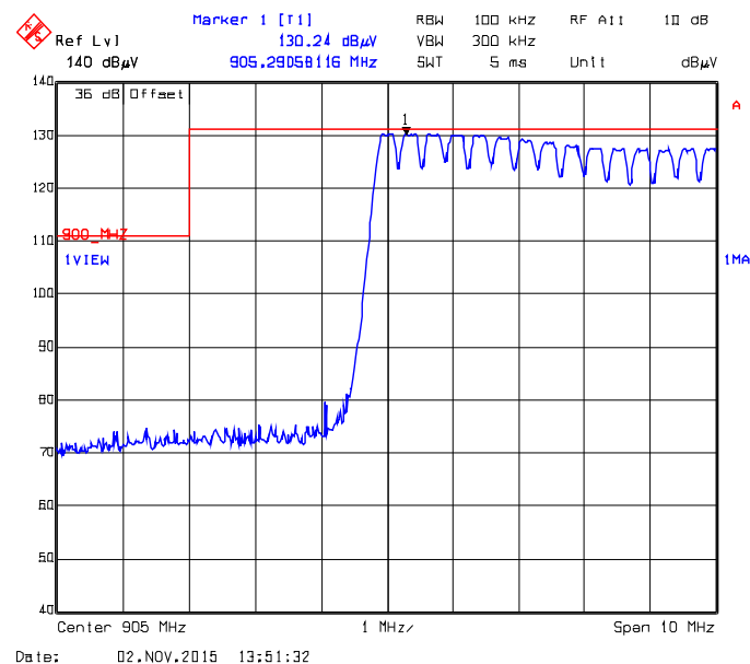
Plot 5.5.4.4.2.34. Band-Edge RF Radiated Emissions at 3 m, Horizontal Polarization Pseudorandom Hopping Mode, Low End of Frequency Band, 905.0 MHz, XTC1, Data Rate at 125 kbps
