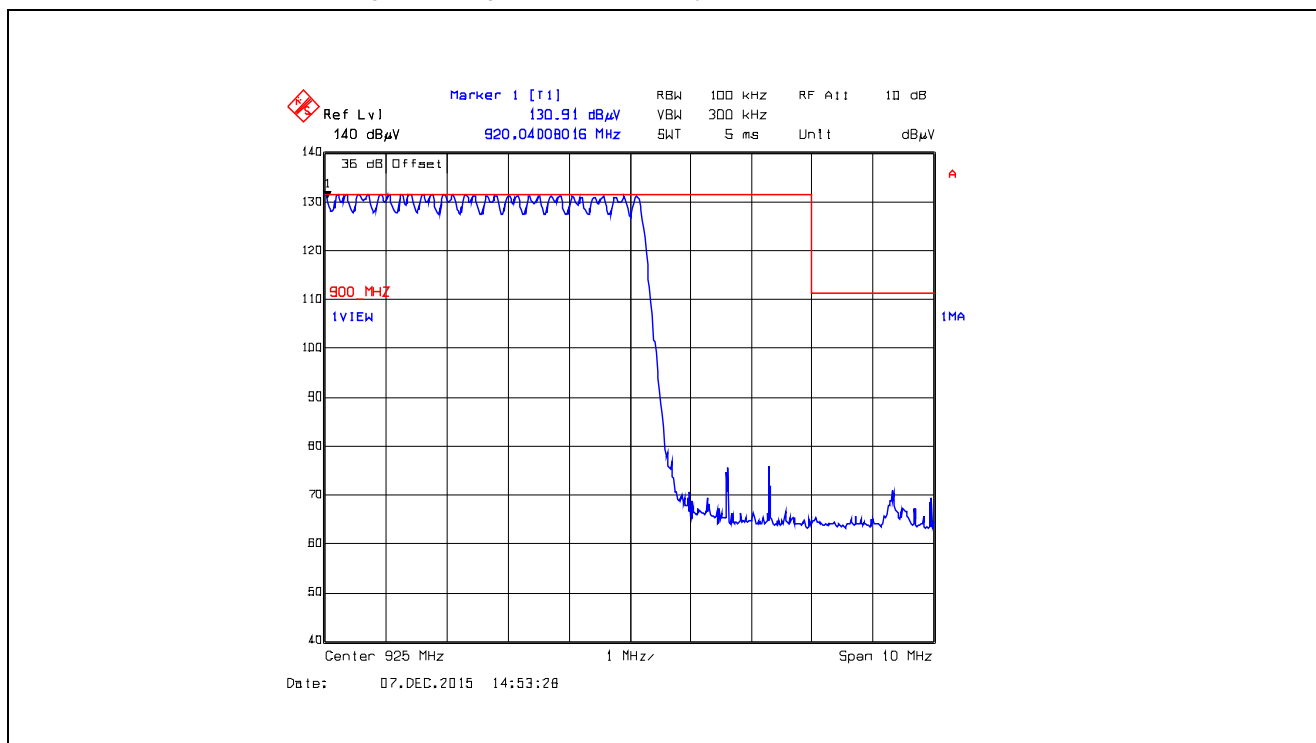
Plot 5.5.4.5.2.30. Band-Edge RF Radiated Emissions at 3 m, Horizontal Polarization Pseudorandom Hopping Mode, High End of Frequency Band, 925.0 MHz, XTC0, Data Rate at 10 kbps
