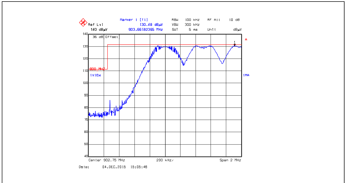
Plot 5.5.4.5.2.18. Band-Edge RF Radiated Emissions at 3 m, Horizontal Polarization Pseudorandom Hopping Mode, Low End of Frequency Band, 902.75 MHz, XB2, Data Rate at 250 kbps
