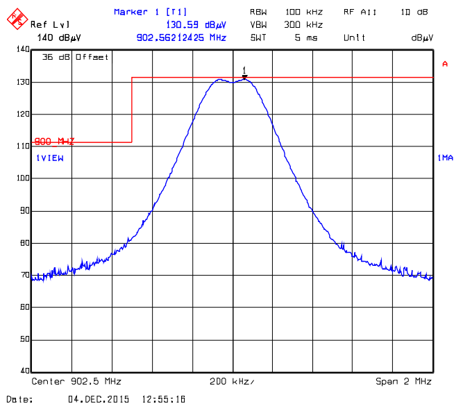
Plot 5.5.4.5.2.10. Band-Edge RF Radiated Emissions at 3 m, Horizontal Polarization Pseudorandom Hopping Mode, Low End of Frequency Band, 902.5 MHz, XBX1, Data Rate at 110 kbps
