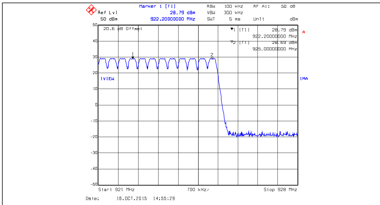
Plot 5.3.4.38. Number of Hopping Frequencies, XTC1, Data Rate at 125 kbps 09 Hopping Channels from 922 – 928 MHz
