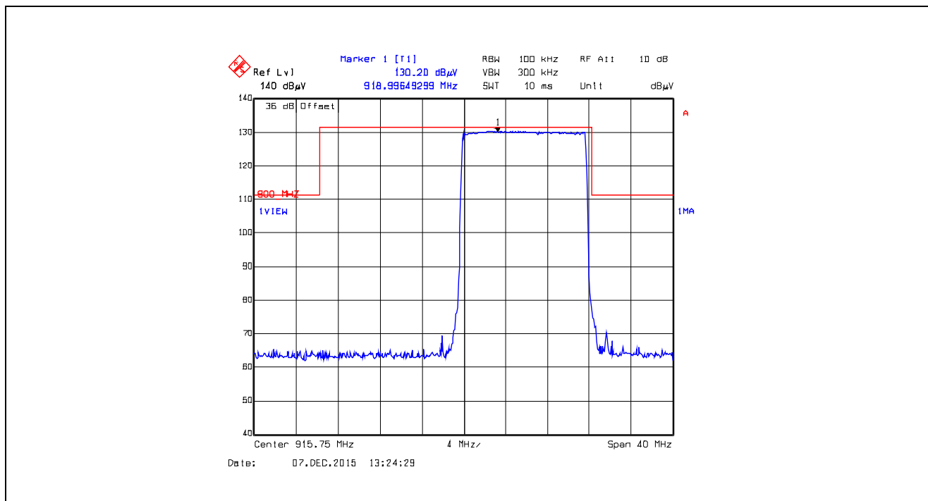
Plot 5.5.4.5.2.44. Band-Edge RF Radiated Emissions at 3 m, Vertical Polarization Pseudorandom Hopping Mode, Low End of Frequency Band, 915.75 MHz, XTCA0, Data Rate at 10 kbps
