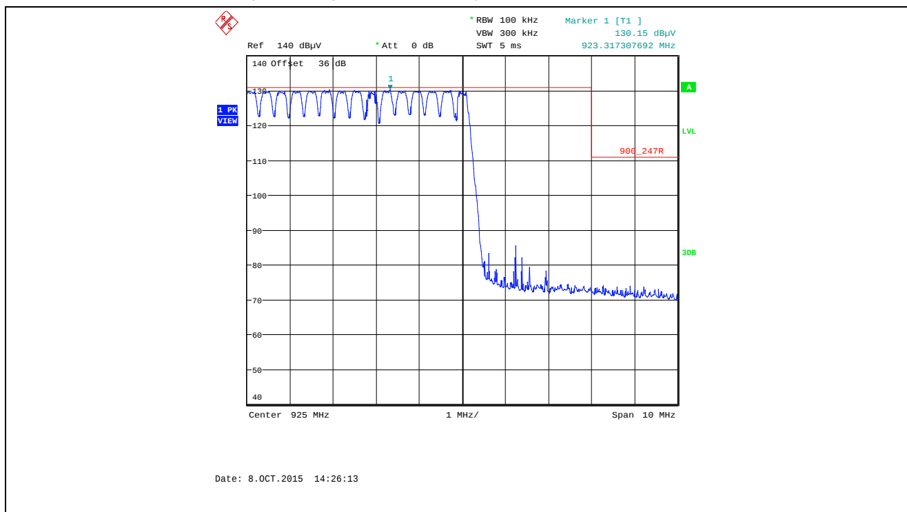
Plot 5.5.4.1.2.40. Band-Edge RF Radiated Emissions at 3 m, Vertical Polarization Pseudorandom Hopping Mode, High End of Frequency Band, 925.0 MHz, XTC1, Data Rate at 125 kbps
