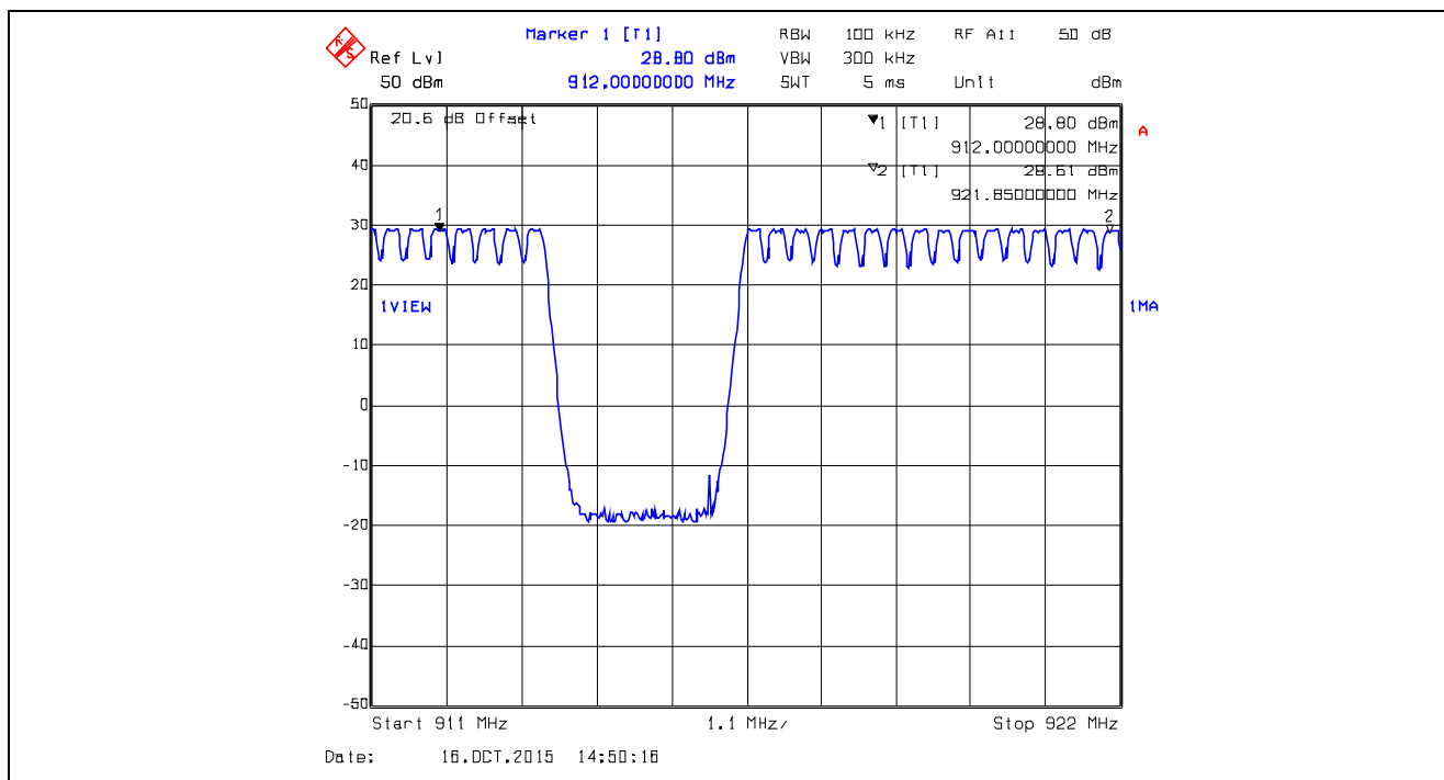
Plot 5.3.4.37. Number of Hopping Frequencies, XTC1, Data Rate at 125 kbps 21 Hopping Channels from 912 – 922 MHz
