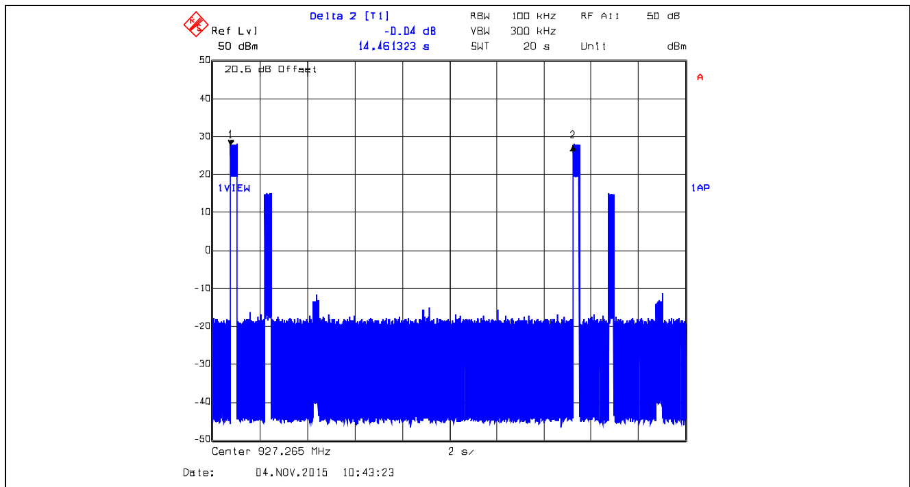
Plot 5.3.4.83. Time of Occupancy, 927.265 MHz XTCA0, Data Rate at 10 kbps Average time of occupancy = 20 \times (T_{\text{on}}) / (T_{\text{total}}) = 20 \times 0.2729459\text{s} / 14.4613\text{s} = 0.3775\text{s} < 0.4\text{s}
