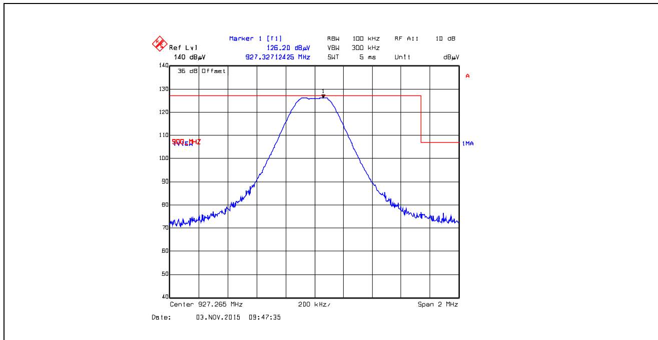
Plot 5.5.4.2.56. Band-Edge RF Radiated Emissions at 3 m, Vertical Polarization Pseudorandom Hopping Mode, High End of Frequency Band, 927.265 MHz, XTCA1, Data Rate at 105kbps
