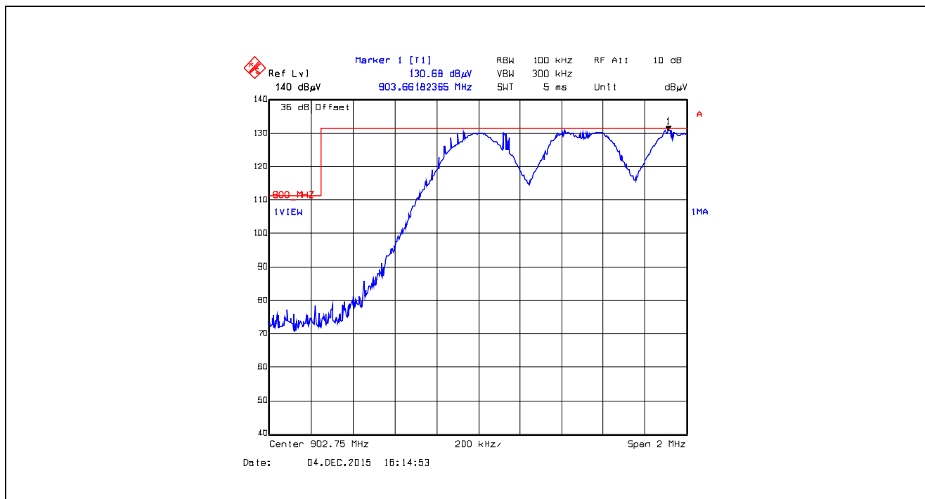
Plot 5.5.4.5.2.20. Band-Edge RF Radiated Emissions at 3 m, Vertical Polarization Pseudorandom Hopping Mode, Low End of Frequency Band, 902.75 MHz, XB2, Data Rate at 250 kbps
