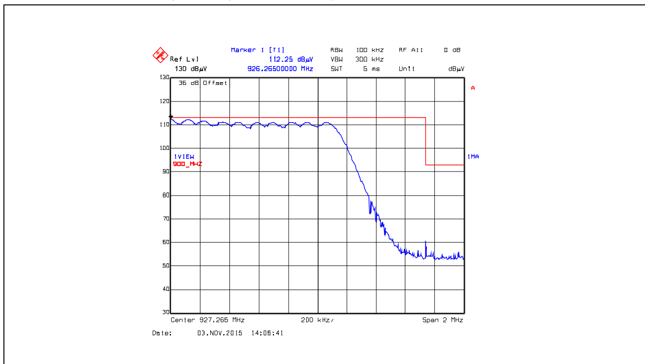
Plot 5.5.4.2.2.46. Band-Edge RF Radiated Emissions at 3 m, Horizontal Polarization Pseudorandom Hopping Mode, High End of Frequency Band, 927.265 MHz, XTCA0, Data Rate at 10 kbps
