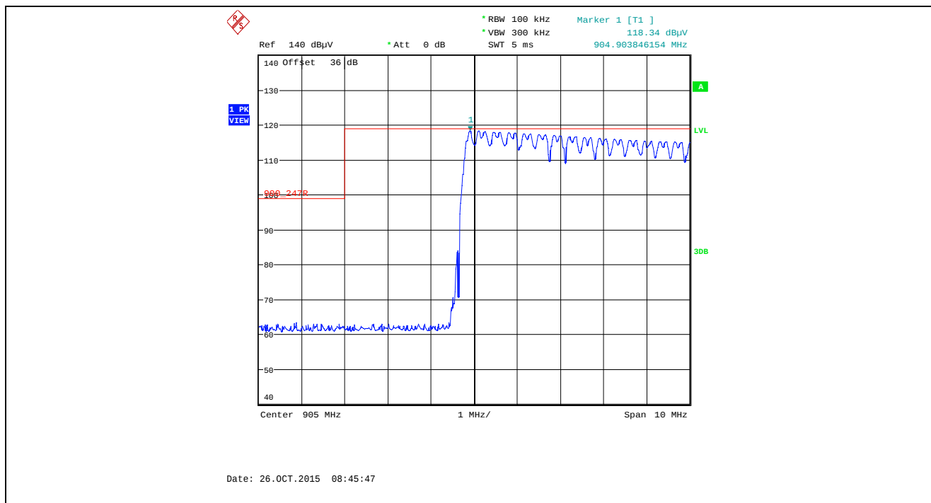
Plot 5.5.4.3.2.26. Band-Edge RF Radiated Emissions at 3 m, Horizontal Polarization Pseudorandom Hopping Mode, Low End of Frequency Band, 905.0 MHz, XTC0, Data Rate at 10 kbps
