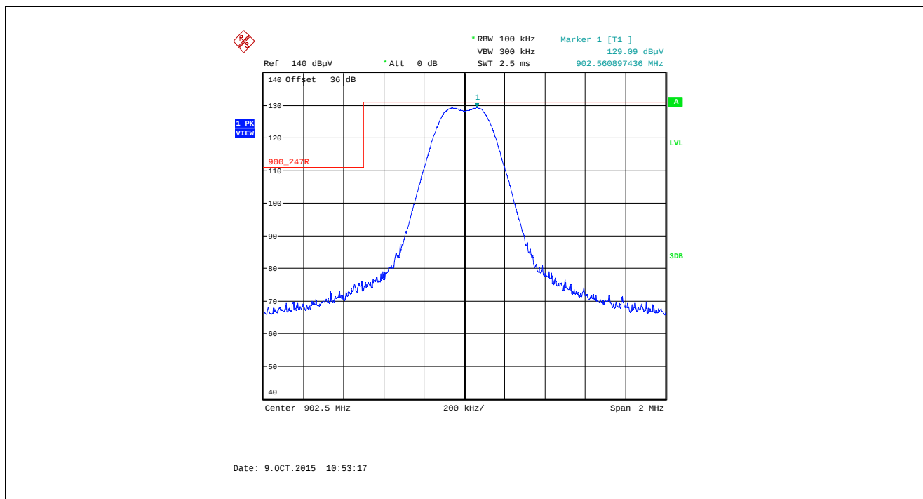
Plot 5.5.4.1.2.11. Band-Edge RF Radiated Emissions at 3 m, Vertical Polarization Single Frequency Mode, Low End of Frequency Band, 902.5 MHz, XBX1, Data Rate at 110 kbps
