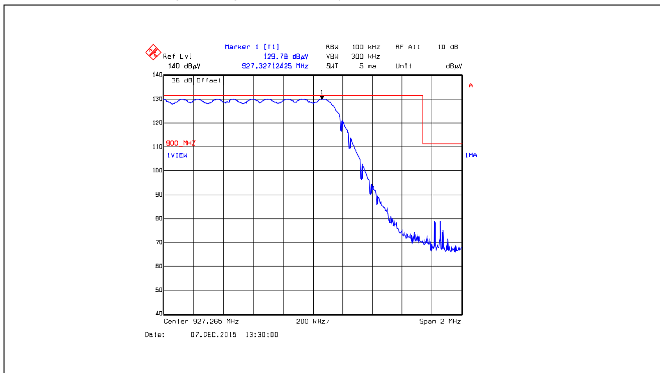
Plot 5.5.4.5.2.48. Band-Edge RF Radiated Emissions at 3 m, Vertical Polarization Pseudorandom Hopping Mode, High End of Frequency Band, 927.265 MHz, XTCA0, Data Rate at 10 kbps
