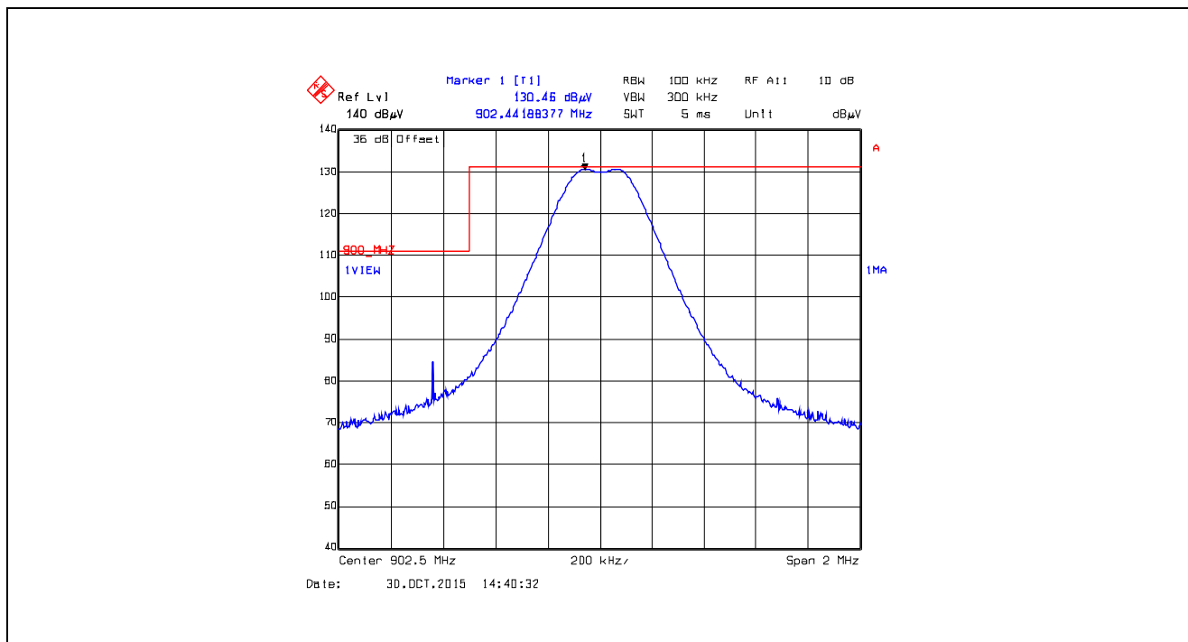
Plot 5.5.4.4.2.11. Band-Edge RF Radiated Emissions at 3 m, Vertical Polarization Single Frequency Mode, Low End of Frequency Band, 902.5 MHz, XBX1, Data Rate at 110 kbps
