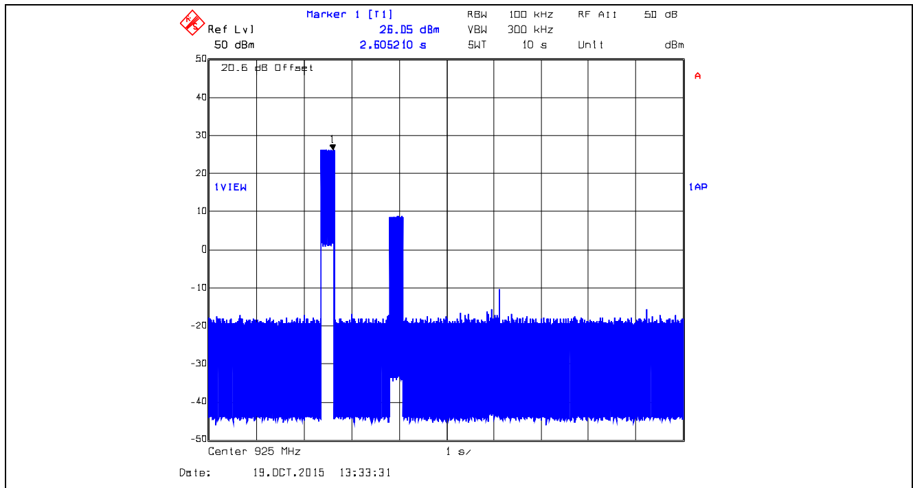
Plot 5.3.4.71. Time of Occupancy, 925.0 MHz, XTC0, Data Rate at 10 kbps Average time of occupancy = (Dwell Time) x (number of hops) = 274.55 ms x 1 = 274.55 ms < 0.4 sec within 10 sec
