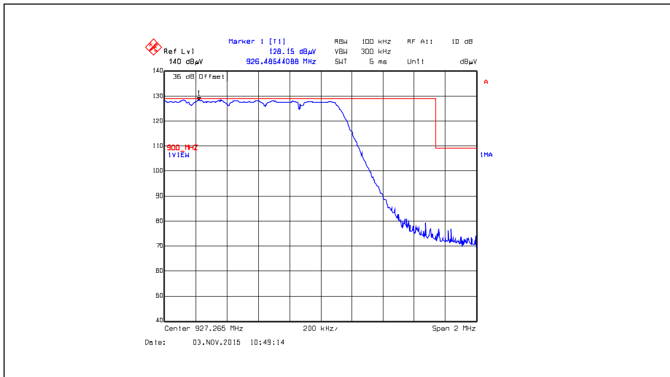
Plot 5.5.4.2.56. Band-Edge RF Radiated Emissions at 3 m, Vertical Polarization Pseudorandom Hopping Mode, High End of Frequency Band, 927.265 MHz, XTCA1, Data Rate at 105kbps
