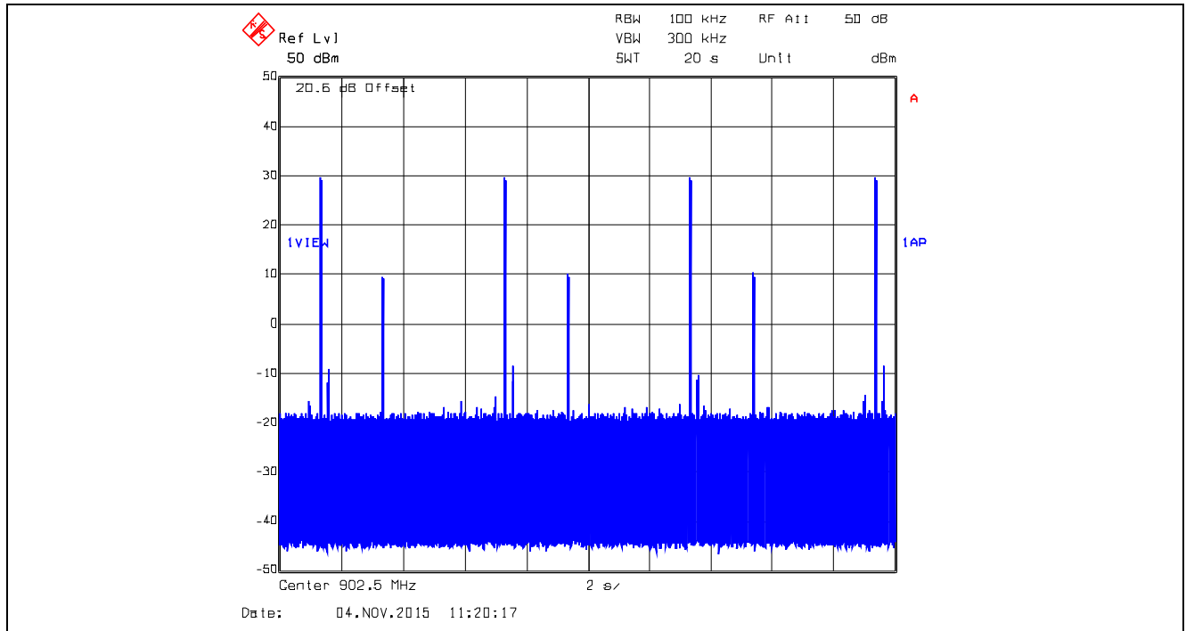
Plot 5.3.4.55. Time of Occupancy, 902.5 MHz, XB1, Data Rate at 110 kbps Average time of occupancy = (Dwell Time) x (number of hops) = 19.0381 ms x 4 = 76.1524 ms < 0.4 sec within 20 sec
