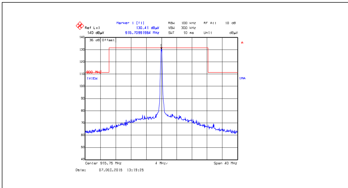
Plot 5.5.4.5.2.51. Band-Edge RF Radiated Emissions at 3 m, Vertical Polarization Single Frequency Mode, Low End of Frequency Band, 915.75 MHz, XTCA1, Data Rate at 105kbps
