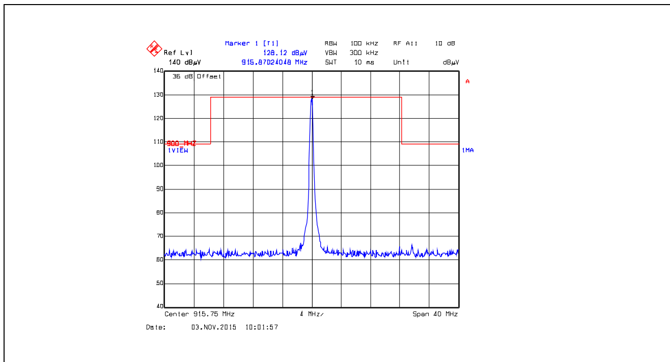
Plot 5.5.4.2.2.43. Band-Edge RF Radiated Emissions at 3 m, Vertical Polarization Single Frequency Mode, Low End of Frequency Band, 915.75 MHz, XTCA0, Data Rate at 10 kbps
