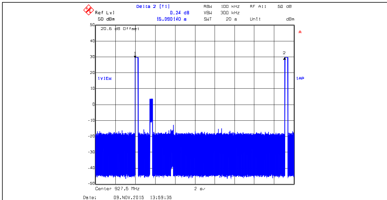
Plot 5.3.4.53. Time of Occupancy, 927.5 MHz XB0, Data Rate at 10 kbps Average time of occupancy = 20 \times (T_{\text{on}}) / (T_{\text{total}}) = 20 \times 0.3006012\text{s} / 15.0901\text{s} = 0.3984\text{s} < 0.4\text{s}
