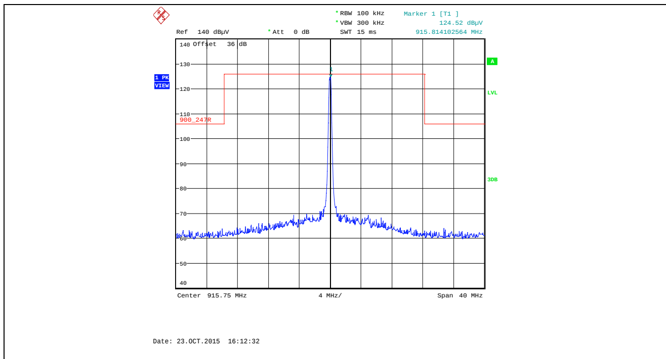
Plot 5.5.4.3.2.51. Band-Edge RF Radiated Emissions at 3 m, Vertical Polarization Single Frequency Mode, Low End of Frequency Band, 915.75 MHz, XTCA1, Data Rate at 105kbps
