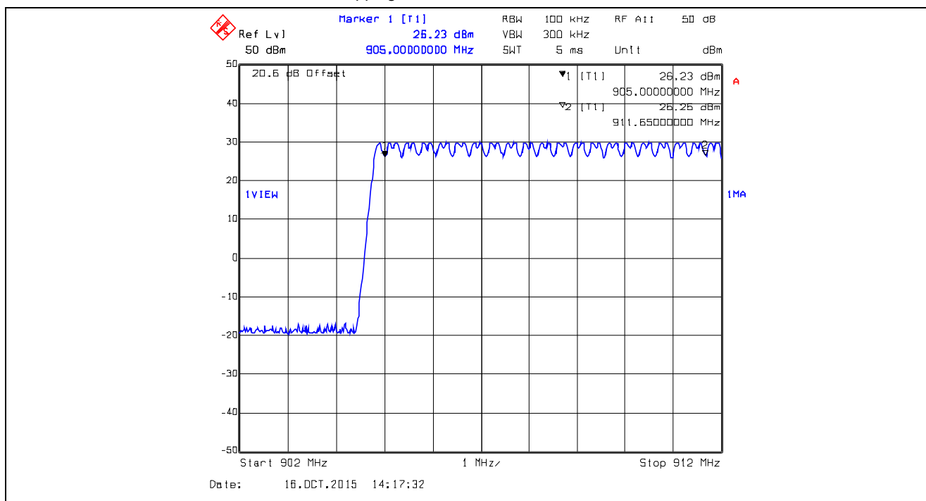
Plot 5.3.4.32. Number of Hopping Frequencies, XTC0, Data Rate at 10 kbps 20 Hopping Channels from 902 – 912 MHz
