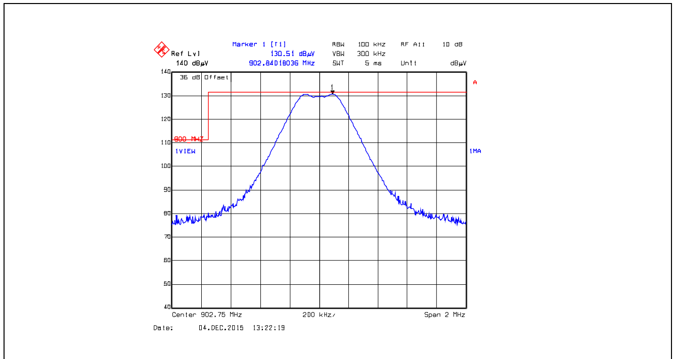
Plot 5.5.4.5.2.17. Band-Edge RF Radiated Emissions at 3 m, Horizontal Polarization Single Frequency Mode, Low End of Frequency Band, 902.75 MHz, XB2, Data Rate at 250 kbps
