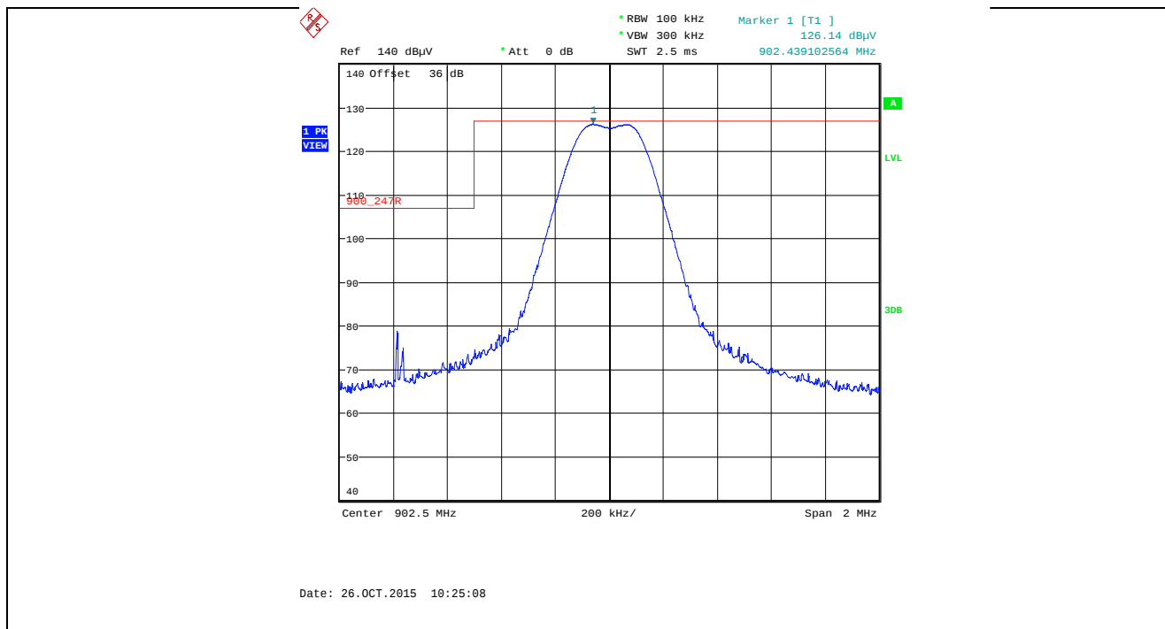
Plot 5.5.4.3.2.11. Band-Edge RF Radiated Emissions at 3 m, Vertical Polarization Single Frequency Mode, Low End of Frequency Band, 902.5 MHz, XB1, Data Rate at 110 kbps
