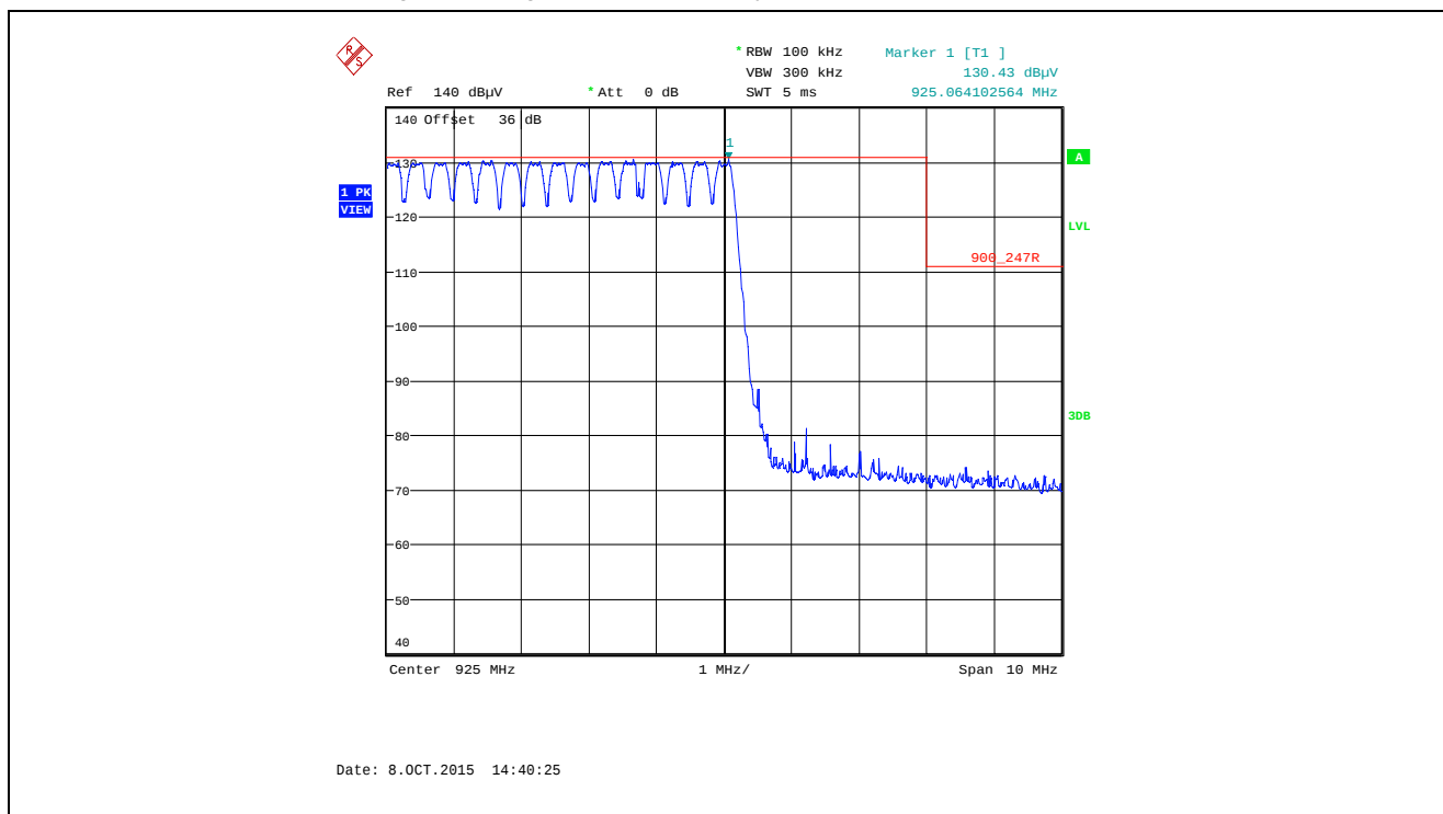
Plot 5.5.4.1.2.38. Band-Edge RF Radiated Emissions at 3 m, Horizontal Polarization Pseudorandom Hopping Mode, High End of Frequency Band, 925.0 MHz, XTC1, Data Rate at 125 kbps
