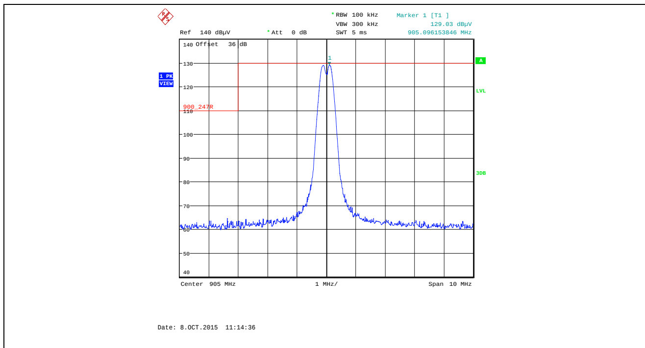
Plot 5.5.4.1.2.27. Band-Edge RF Radiated Emissions at 3 m, Vertical Polarization Single Frequency Mode, Low End of Frequency Band, 905.0 MHz, XTC0, Data Rate at 10 kbps
