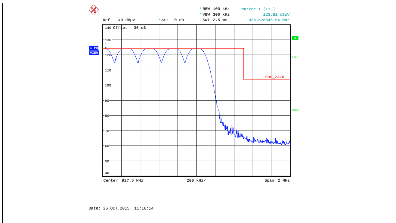
Plot 5.5.4.3.2.8. Band-Edge RF Radiated Emissions at 3 m, Vertical Polarization Pseudorandom Hopping Mode, High End of Frequency Band, 927.5 MHz, XB0, Data Rate at 10 kbps
