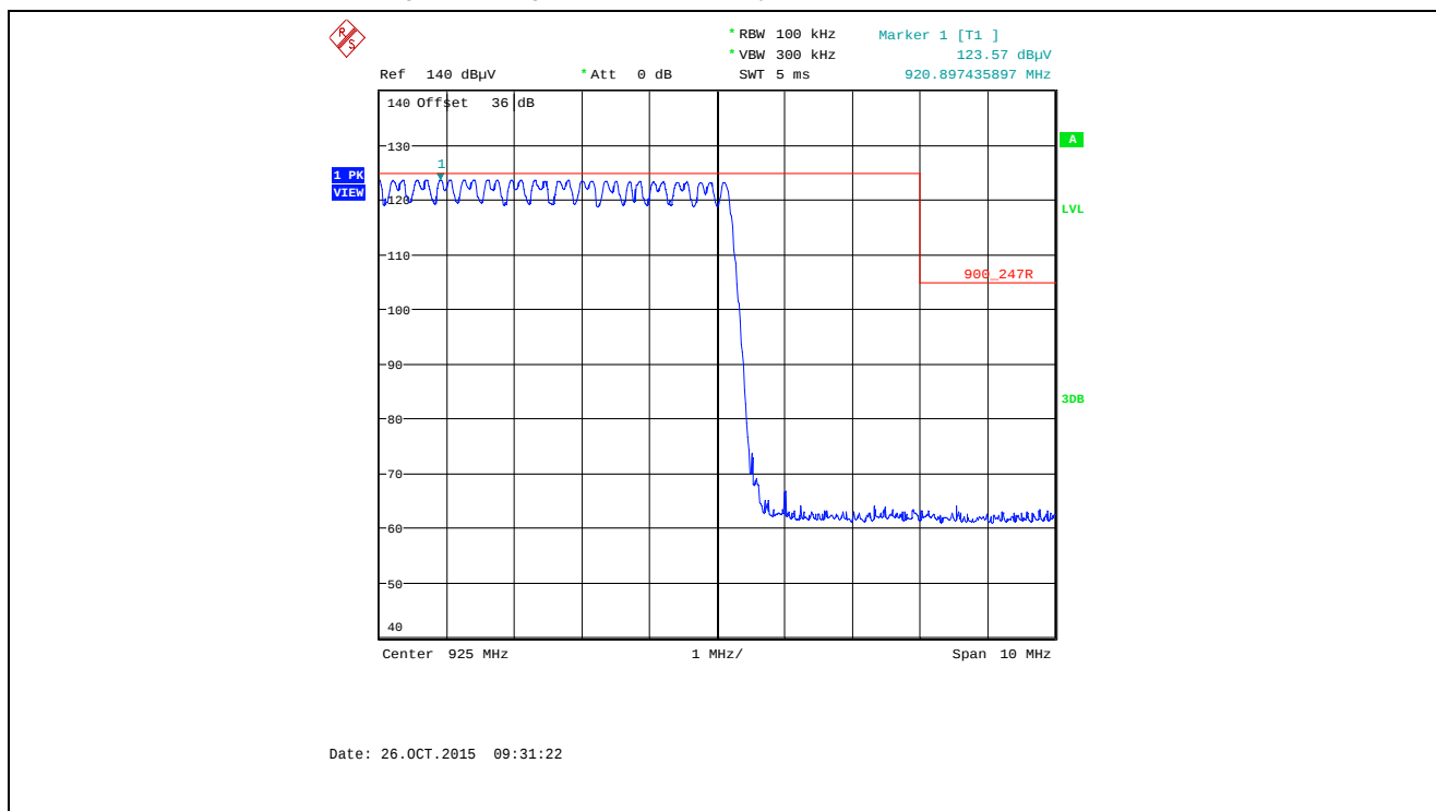
Plot 5.5.4.3.2.32. Band-Edge RF Radiated Emissions at 3 m, Vertical Polarization Pseudorandom Hopping Mode, High End of Frequency Band, 925.0 MHz, XTC0, Data Rate at 10 kbps
