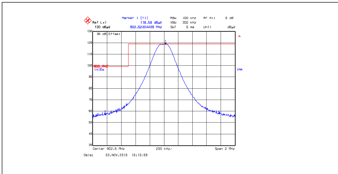
Plot 5.5.4.2.2.1. Band-Edge RF Radiated Emissions at 3 m, Horizontal Polarization Single Frequency Mode, Low End of Frequency Band, 902.5 MHz, XB0, Data Rate at 10 kbps
