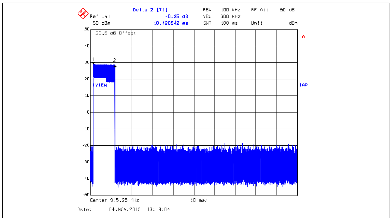
Plot 5.3.4.62. Time of Occupancy, 915.25 MHz, XB2, Data Rate at 250 kbps Dwell Time @ 915.25 MHz = 10.4208 ms
