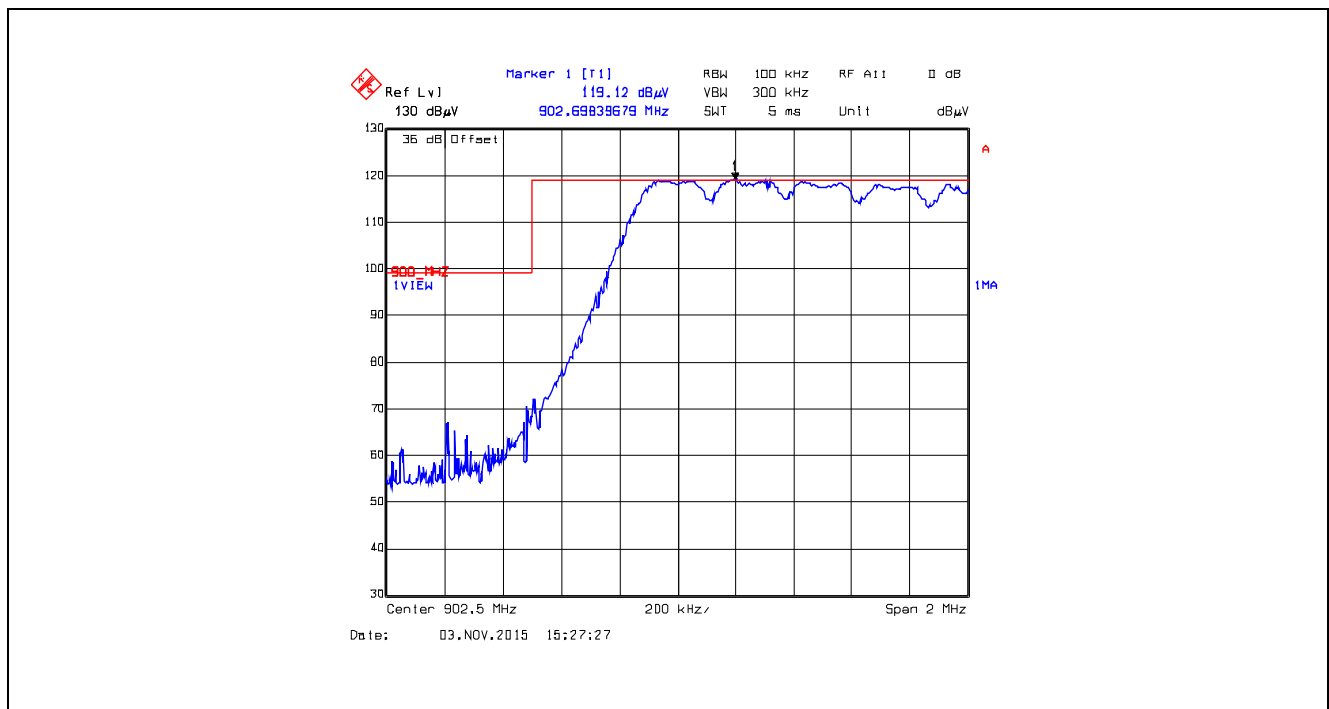
Plot 5.5.4.2.10. Band-Edge RF Radiated Emissions at 3 m, Horizontal Polarization Pseudorandom Hopping Mode, Low End of Frequency Band, 902.5 MHz, XBX1, Data Rate at 110 kbps
