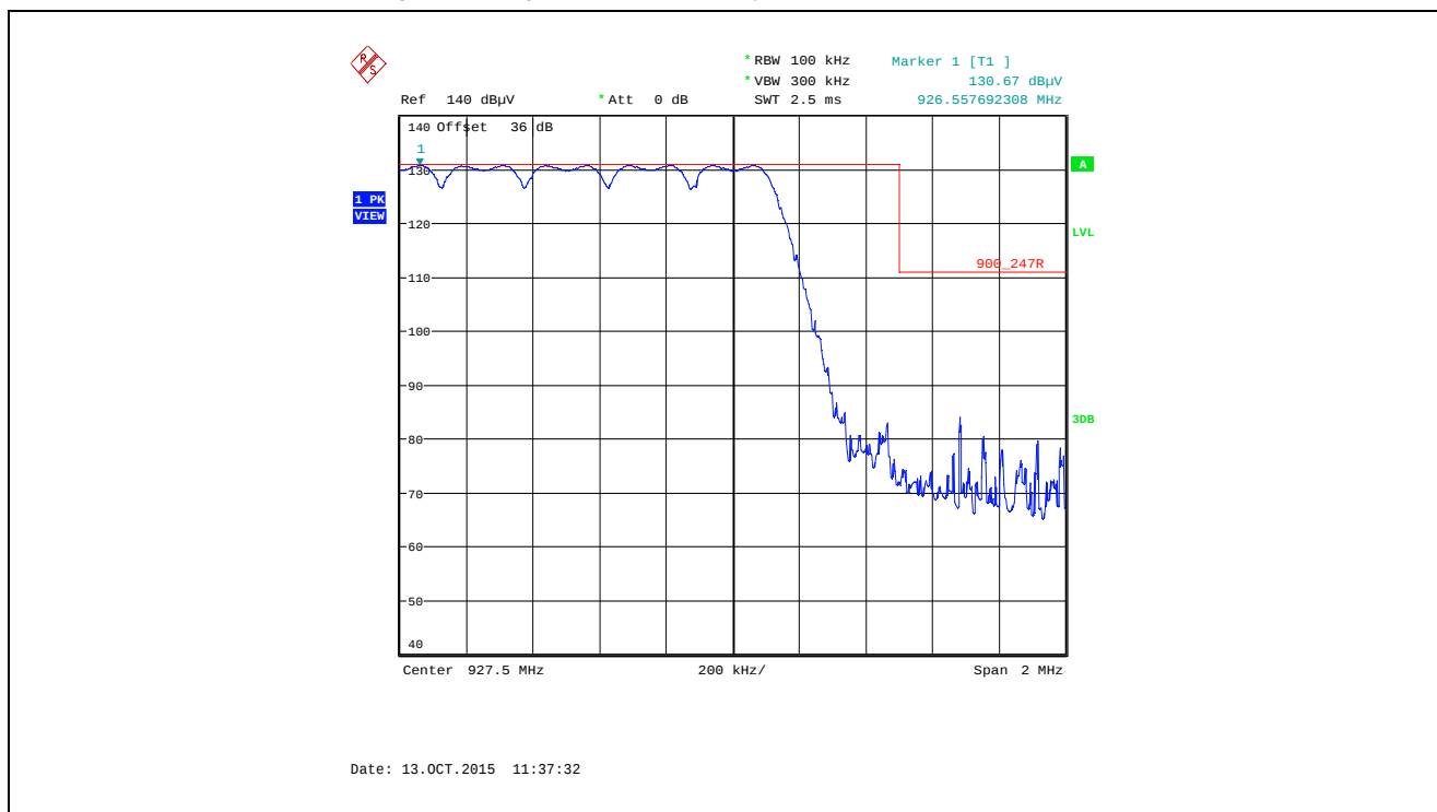
Plot 5.5.4.1.2.16. Band-Edge RF Radiated Emissions at 3 m, Vertical Polarization Pseudorandom Hopping Mode, High End of Frequency Band, 927.5 MHz, XBX1, Data Rate at 110 kbps
