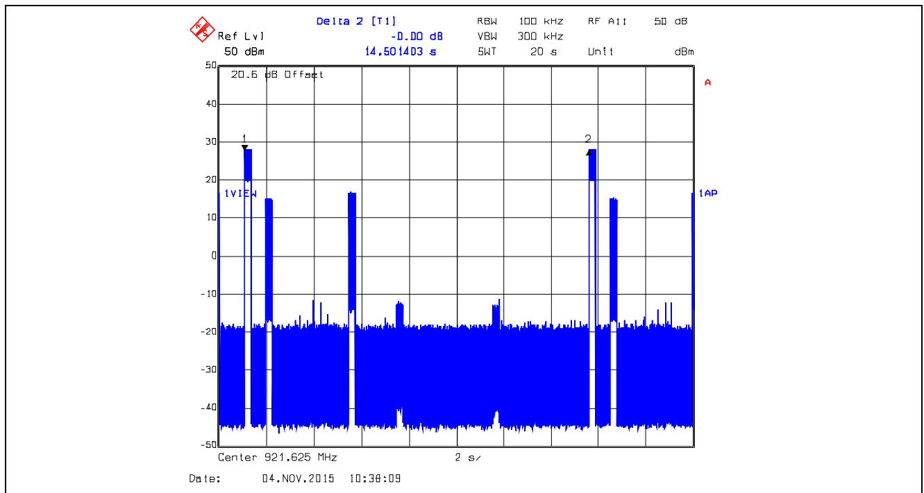
Plot 5.3.4.81. Time of Occupancy, 921.625 MHz XTCA0, Data Rate at 10 kbps Average time of occupancy = 20 \times (T_{\text{on}}) / (T_{\text{total}}) = 20 \times 0.272946\text{s} / 14.5014\text{s} = 0.3764\text{s} < 0.4\text{s}
