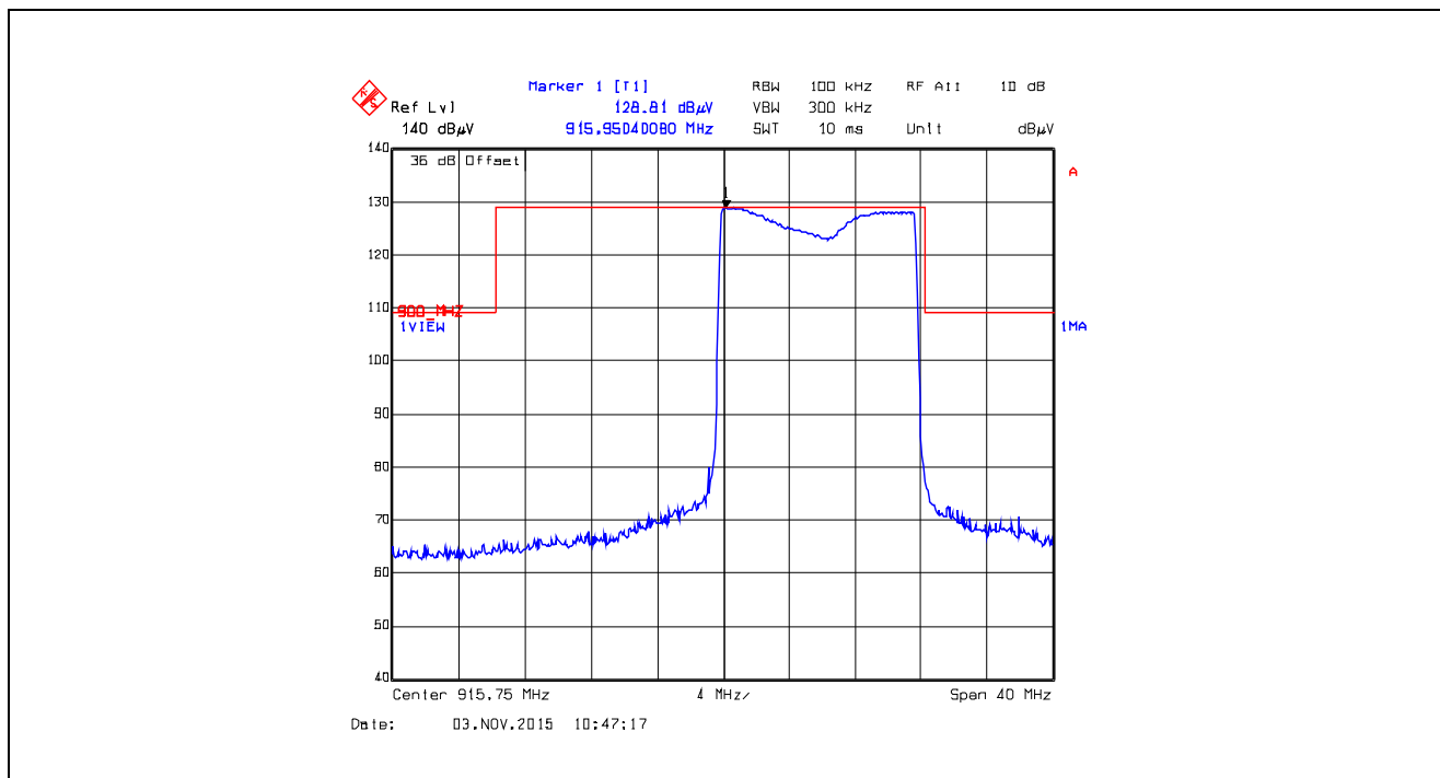
Plot 5.5.4.2.52. Band-Edge RF Radiated Emissions at 3 m, Vertical Polarization Pseudorandom Hopping Mode, Low End of Frequency Band, 915.75 MHz, XTCA1, Data Rate at 105kbps
