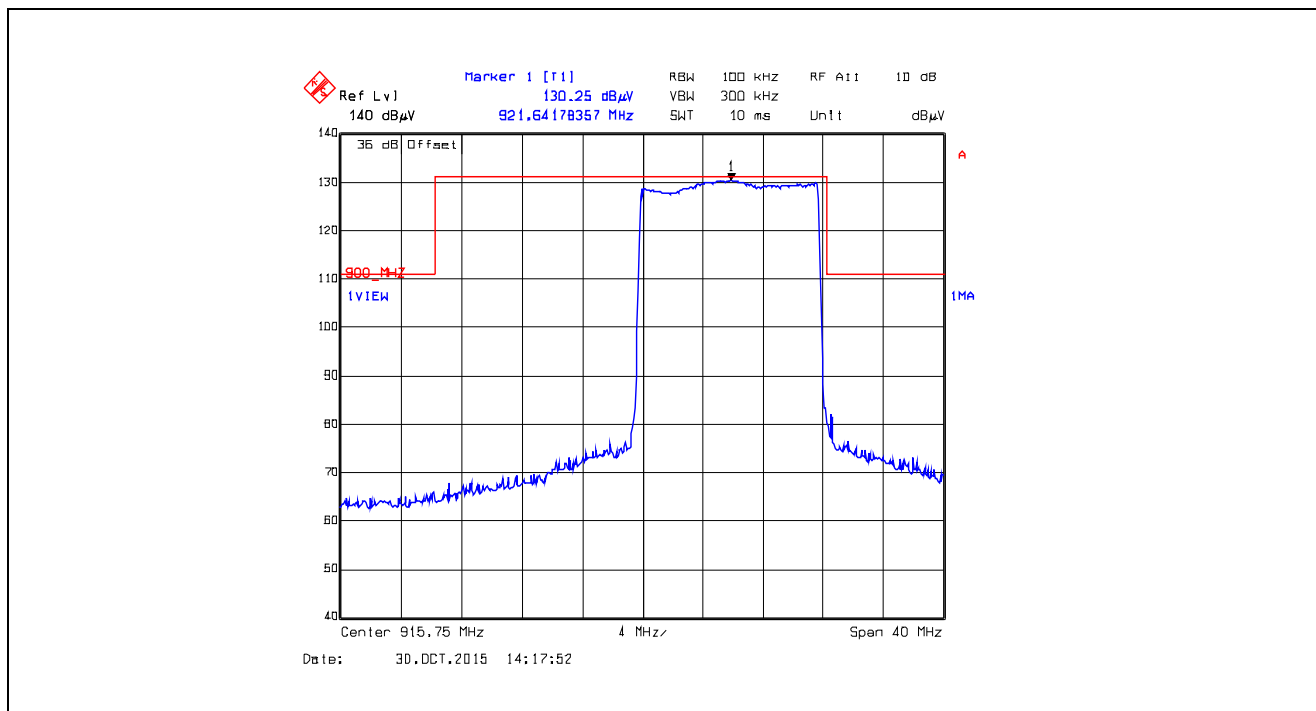
Plot 5.5.4.4.2.52. Band-Edge RF Radiated Emissions at 3 m, Vertical Polarization Pseudorandom Hopping Mode, Low End of Frequency Band, 915.75 MHz, XTCA1, Data Rate at 105kbps
