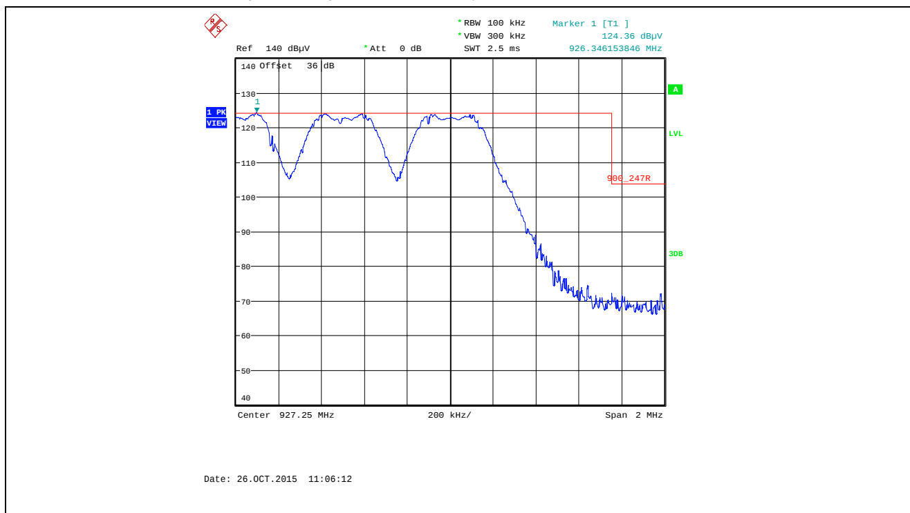
Plot 5.5.4.3.2.24. Band-Edge RF Radiated Emissions at 3 m, Vertical Polarization Pseudorandom Hopping Mode, High End of Frequency Band, 927.25 MHz, XB2, Data Rate at 250 kbps
