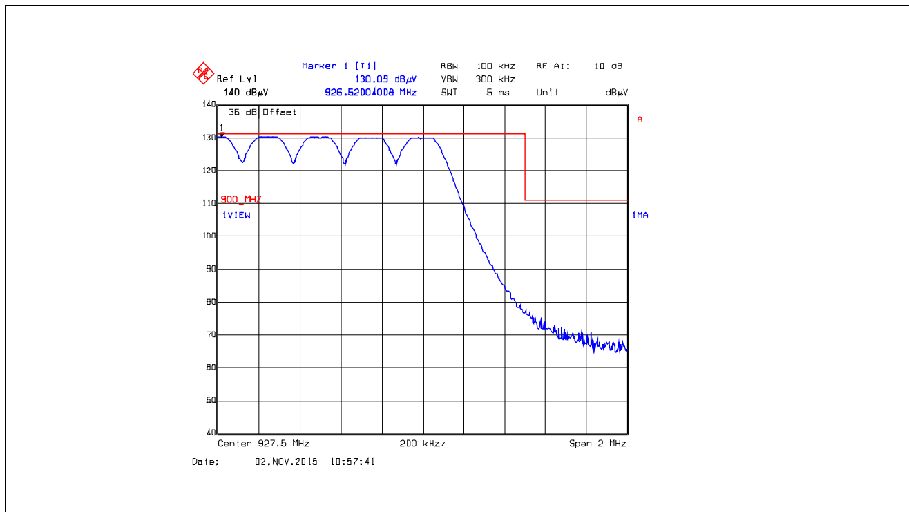
Plot 5.5.4.4.2.6. Band-Edge RF Radiated Emissions at 3 m, Horizontal Polarization Pseudorandom Hopping Mode, High End of Frequency Band, 927.5 MHz, XB0, Data Rate at 10 kbps
