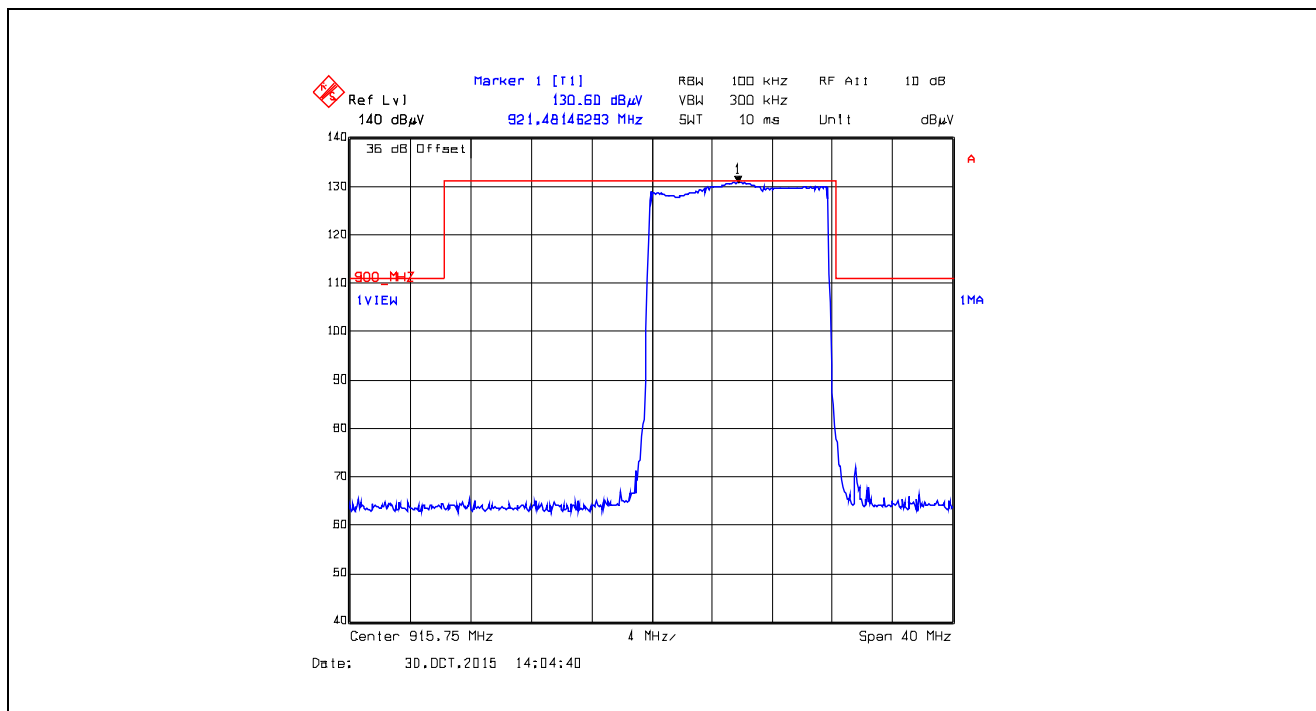
Plot 5.5.4.4.2.44. Band-Edge RF Radiated Emissions at 3 m, Vertical Polarization Pseudorandom Hopping Mode, Low End of Frequency Band, 915.75 MHz, XTCA0, Data Rate at 10 kbps
