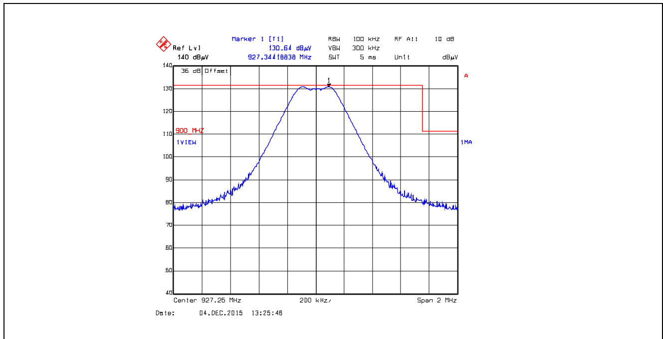
Plot 5.5.4.5.2.21. Band-Edge RF Radiated Emissions at 3 m, Horizontal Polarization Single Frequency Mode, High End of Frequency Band, 927.25 MHz, XB2, Data Rate at 250 kbps
