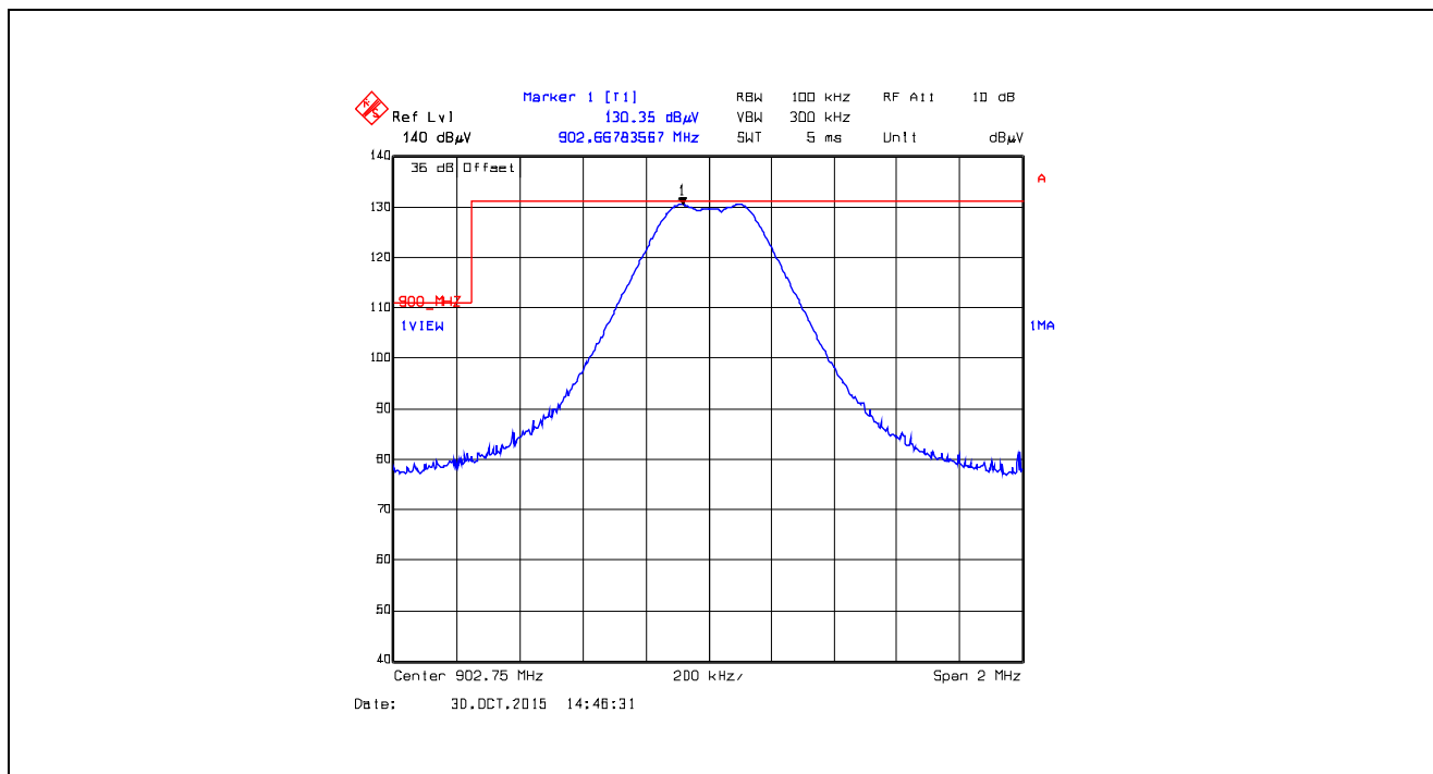
Plot 5.5.4.4.2.19. Band-Edge RF Radiated Emissions at 3 m, Vertical Polarization Single Frequency Mode, Low End of Frequency Band, 902.75 MHz, XBX2, Data Rate at 250 kbps
