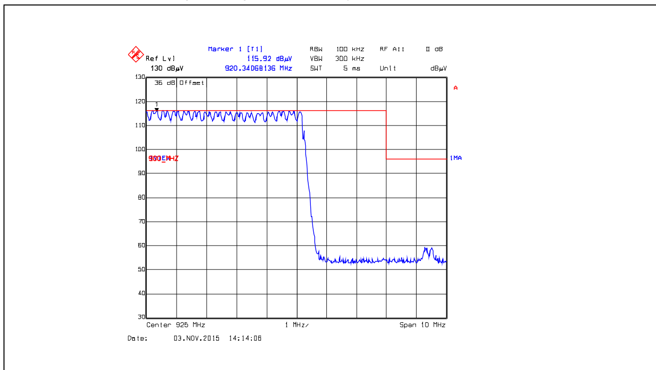
Plot 5.5.4.2.230. Band-Edge RF Radiated Emissions at 3 m, Horizontal Polarization Pseudorandom Hopping Mode, High End of Frequency Band, 925.0 MHz, XTC0, Data Rate at 10 kbps
