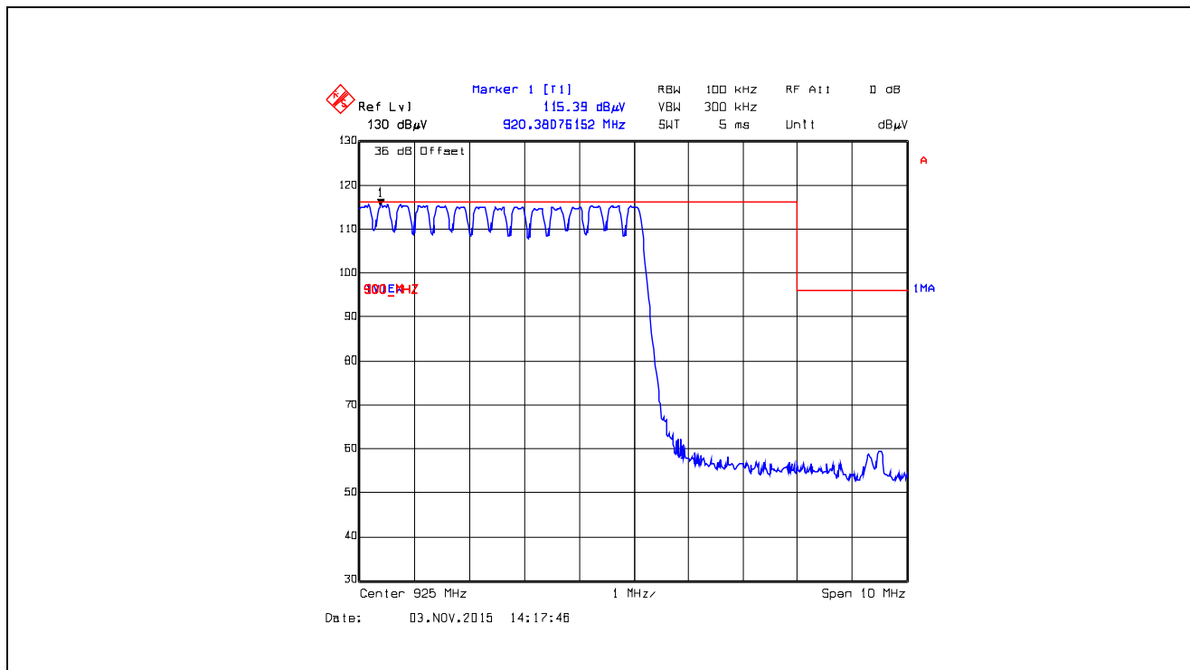
Plot 5.5.4.2.2.38. Band-Edge RF Radiated Emissions at 3 m, Horizontal Polarization Pseudorandom Hopping Mode, High End of Frequency Band, 925.0 MHz, XTC1, Data Rate at 125 kbps
