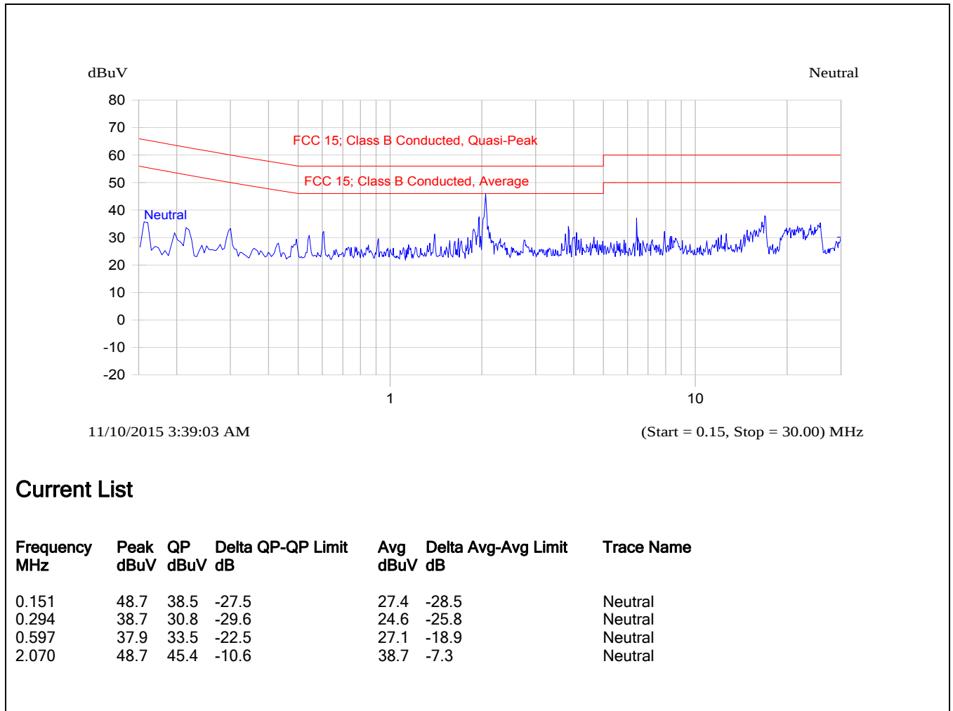
Plot 5.1.4.2. Power Line Conducted Emissions (Tx Mode) Line Voltage: 120 VAC; Line Tested: Neutral
