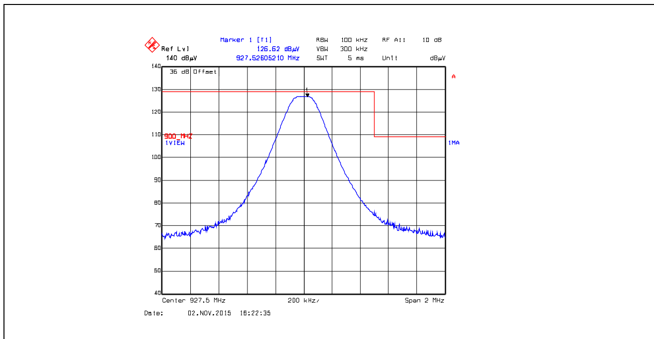
Plot 5.5.4.2.15. Band-Edge RF Radiated Emissions at 3 m, Vertical Polarization Single Frequency Mode, High End of Frequency Band, 927.5 MHz, XBX1, Data Rate at 110 kbps
