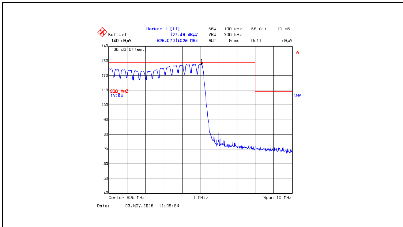
Plot 5.5.4.2.40. Band-Edge RF Radiated Emissions at 3 m, Vertical Polarization Pseudorandom Hopping Mode, High End of Frequency Band, 925.0 MHz, XTC1, Data Rate at 125 kbps
