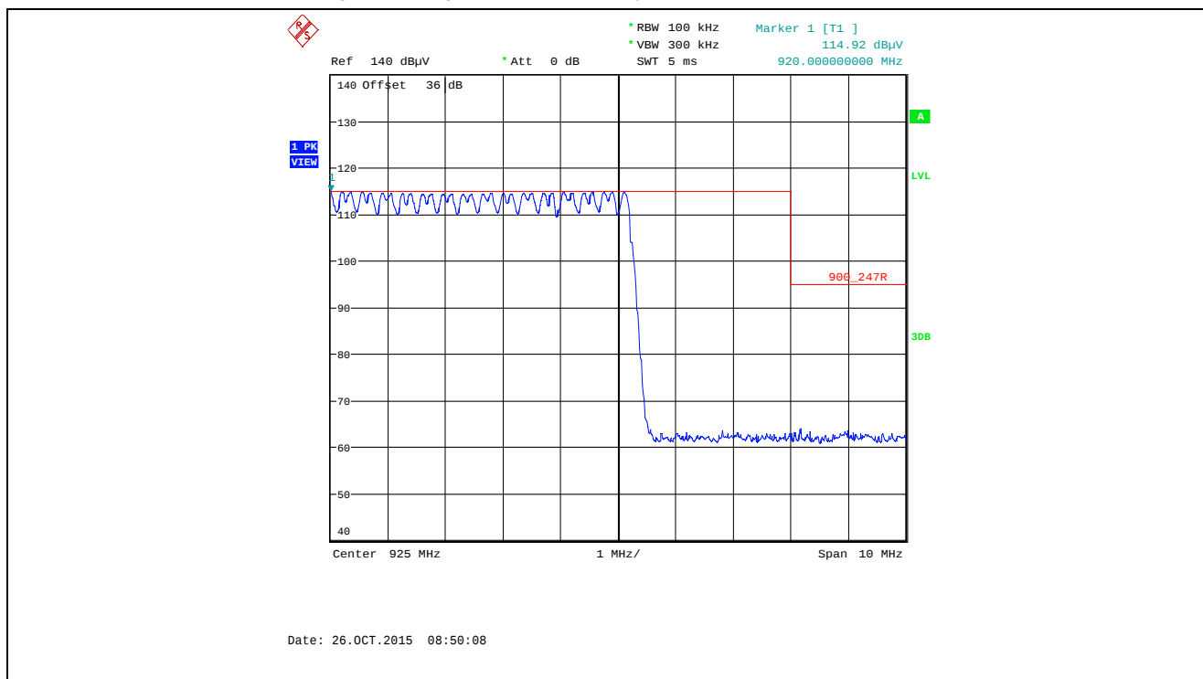
Plot 5.5.4.3.2.30. Band-Edge RF Radiated Emissions at 3 m, Horizontal Polarization Pseudorandom Hopping Mode, High End of Frequency Band, 925.0 MHz, XTC0, Data Rate at 10 kbps
