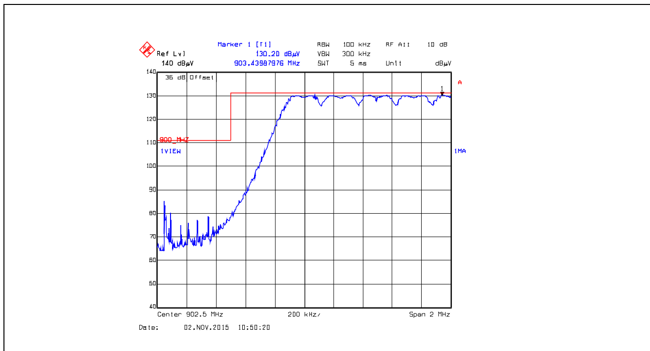
Plot 5.5.4.4.2.10. Band-Edge RF Radiated Emissions at 3 m, Horizontal Polarization Pseudorandom Hopping Mode, Low End of Frequency Band, 902.5 MHz, XBX1, Data Rate at 110 kbps
