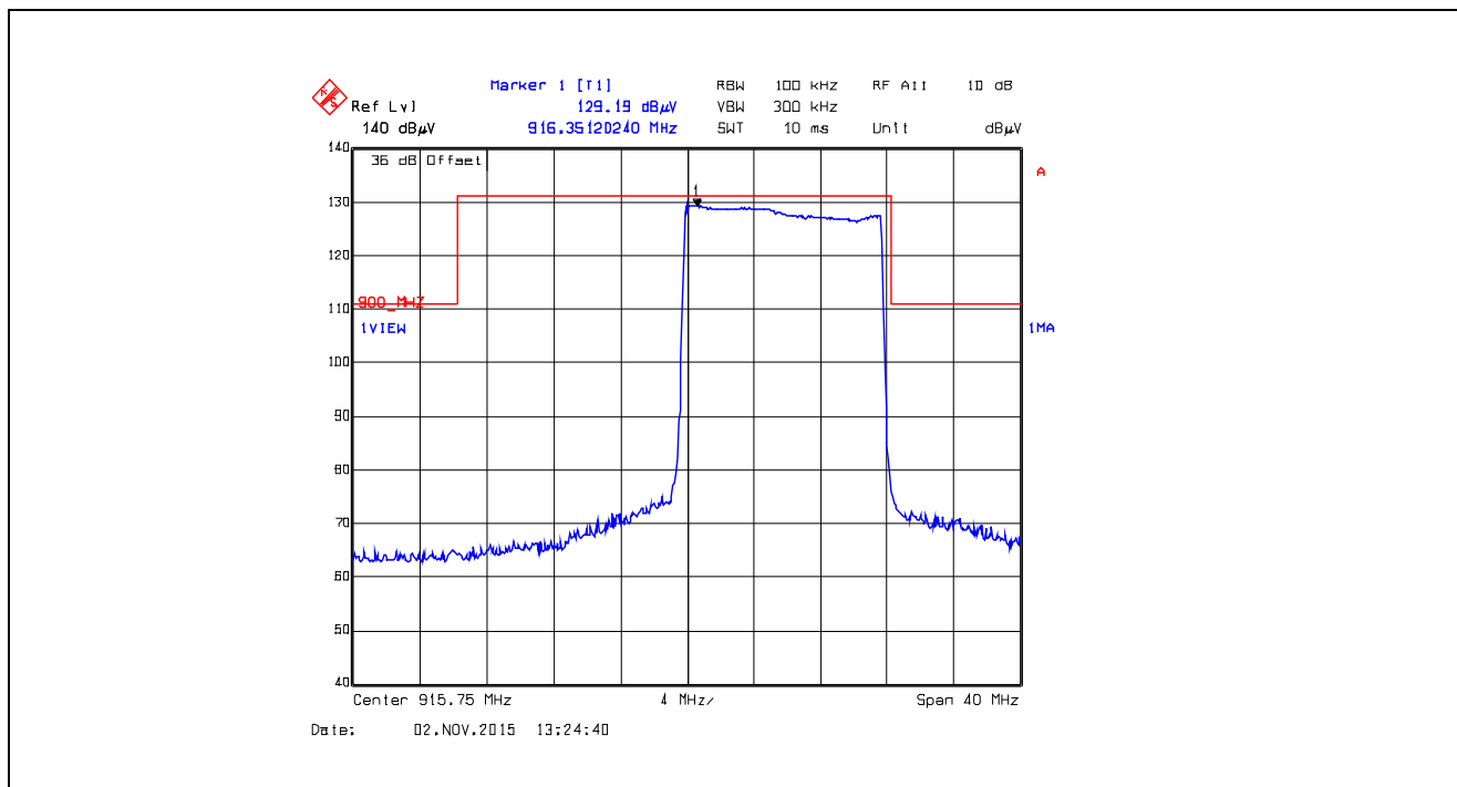
Plot 5.5.4.4.2.50. Band-Edge RF Radiated Emissions at 3 m, Horizontal Polarization Pseudorandom Hopping Mode, Low End of Frequency Band, 915.75 MHz, XTCA1, Data Rate at 105kbps
