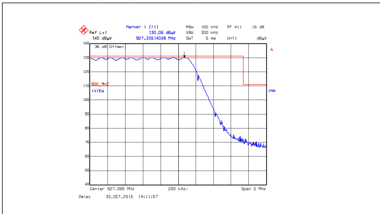
Plot 5.5.4.4.2.48. Band-Edge RF Radiated Emissions at 3 m, Vertical Polarization Pseudorandom Hopping Mode, High End of Frequency Band, 927.265 MHz, XTCA0, Data Rate at 10 kbps
