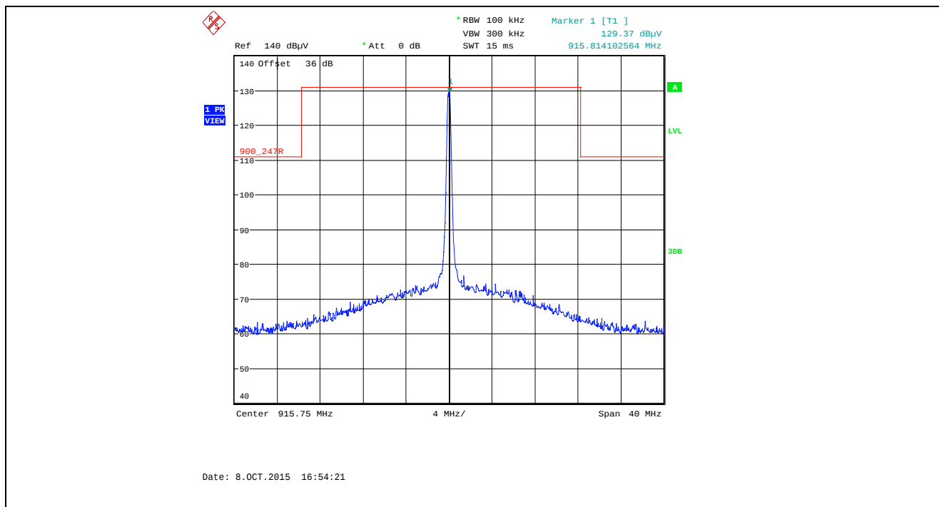
Plot 5.5.4.1.2.51. Band-Edge RF Radiated Emissions at 3 m, Vertical Polarization Single Frequency Mode, Low End of Frequency Band, 915.75 MHz, XTCA1, Data Rate at 105kbps
