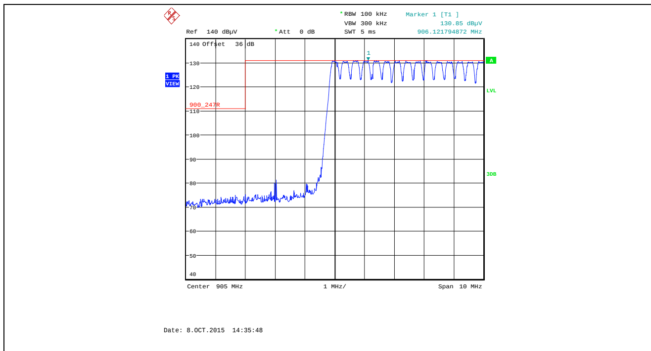
Plot 5.5.4.1.2.34. Band-Edge RF Radiated Emissions at 3 m, Horizontal Polarization Pseudorandom Hopping Mode, Low End of Frequency Band, 905.0 MHz, XTC1, Data Rate at 125 kbps
