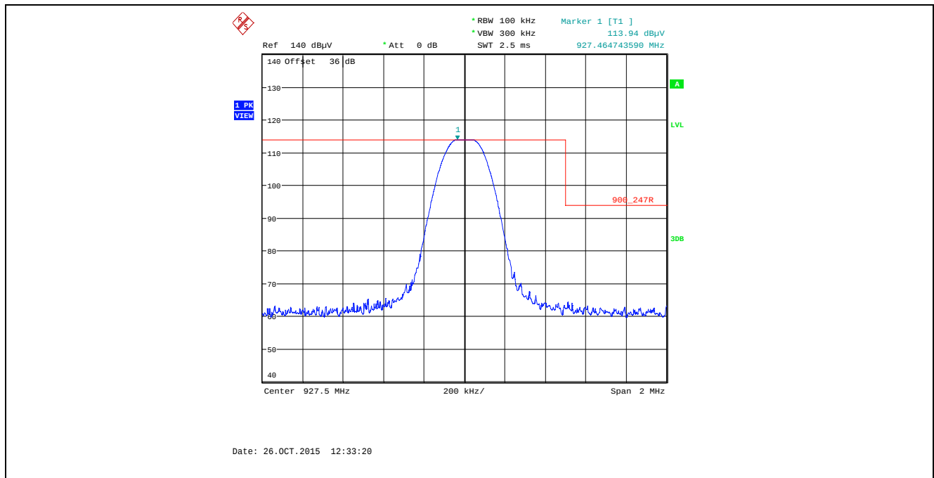
Plot 5.5.4.3.2.5. Band-Edge RF Radiated Emissions at 3 m, Horizontal Polarization Single Frequency Mode, High End of Frequency Band, 927.5 MHz, XB0, Data Rate at 10 kbps
