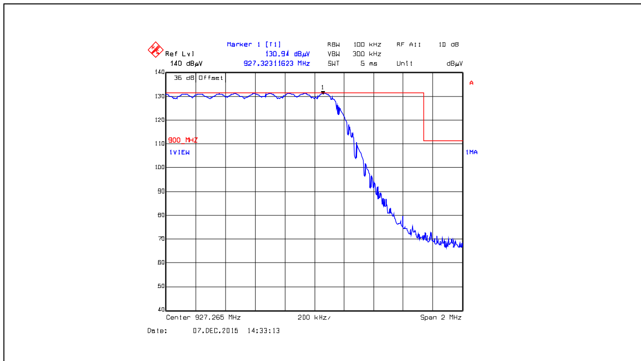
Plot 5.5.4.5.2.46. Band-Edge RF Radiated Emissions at 3 m, Horizontal Polarization Pseudorandom Hopping Mode, High End of Frequency Band, 927.265 MHz, XTCA0, Data Rate at 10 kbps
