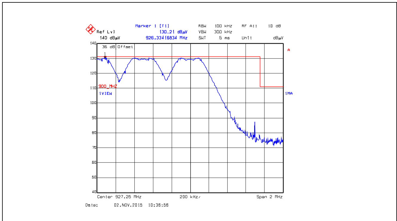
Plot 5.5.4.4.2.22. Band-Edge RF Radiated Emissions at 3 m, Horizontal Polarization Pseudorandom Hopping Mode, High End of Frequency Band, 927.25 MHz, XB2, Data Rate at 250 kbps
