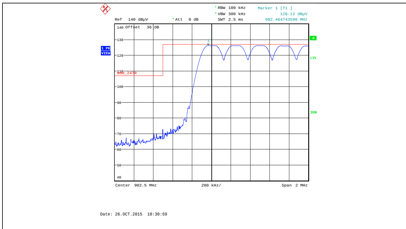
Plot 5.5.4.3.2.4. Band-Edge RF Radiated Emissions at 3 m, Vertical Polarization Pseudorandom Hopping Mode, Low End of Frequency Band, 902.5 MHz, XB0, Data Rate at 10 kbps
