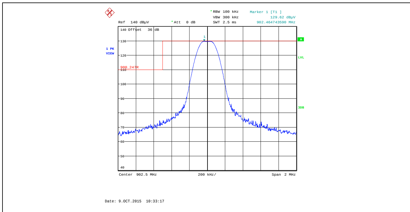
Plot 5.5.4.1.2.3. Band-Edge RF Radiated Emissions at 3 m, Vertical Polarization Single Frequency Mode, Low End of Frequency Band, 902.5 MHz, XB0, Data Rate at 10 kbps
