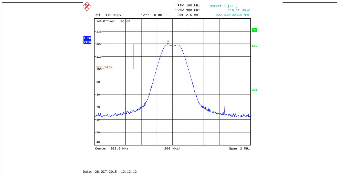
Plot 5.5.4.3.2.9. Band-Edge RF Radiated Emissions at 3 m, Horizontal Polarization Single Frequency Mode, Low End of Frequency Band, 902.5 MHz, XB1, Data Rate at 110 kbps
