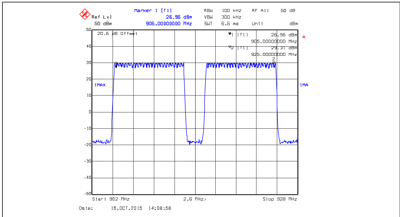
Plot 5.3.4.35. Total Number of Hopping Frequencies, XTC0, Data Rate at 10 kbps 50 Hopping Channels from 902 – 928 MHz (20+21+09 = 50)
