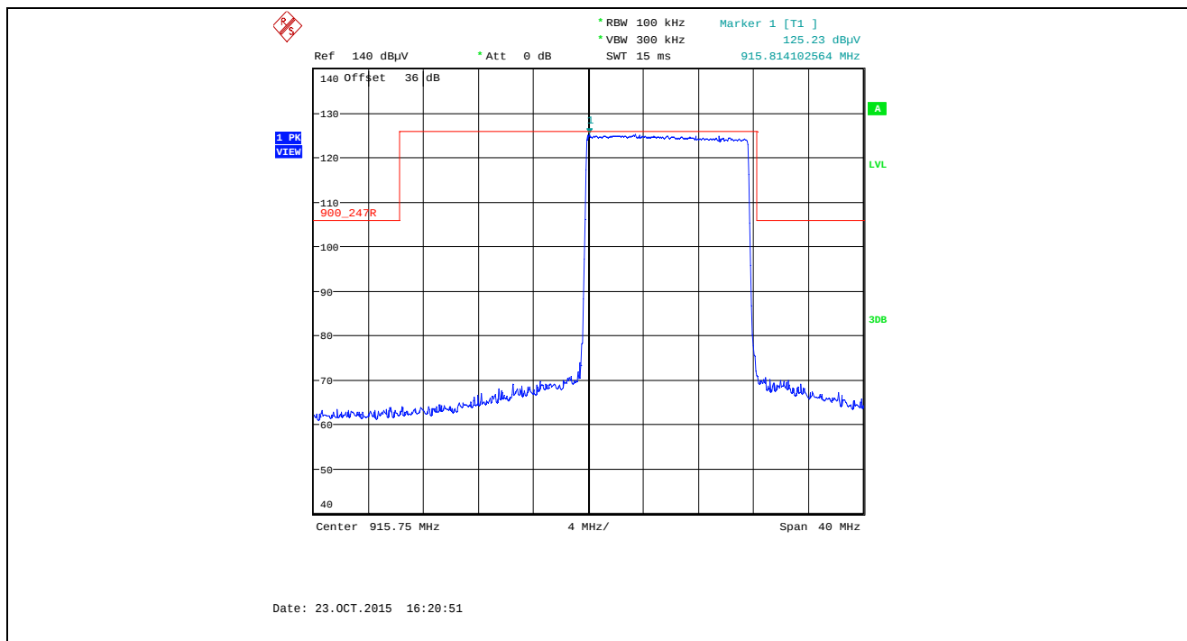
Plot 5.5.4.3.2.52. Band-Edge RF Radiated Emissions at 3 m, Vertical Polarization Pseudorandom Hopping Mode, Low End of Frequency Band, 915.75 MHz, XTCA1, Data Rate at 105kbps
