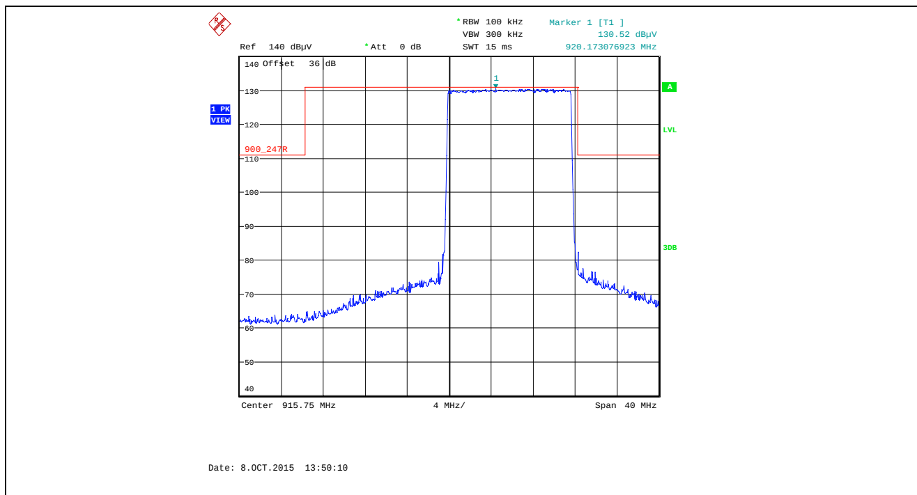
Plot 5.5.4.1.2.52. Band-Edge RF Radiated Emissions at 3 m, Vertical Polarization Pseudorandom Hopping Mode, Low End of Frequency Band, 915.75 MHz, XTCA1, Data Rate at 105kbps
