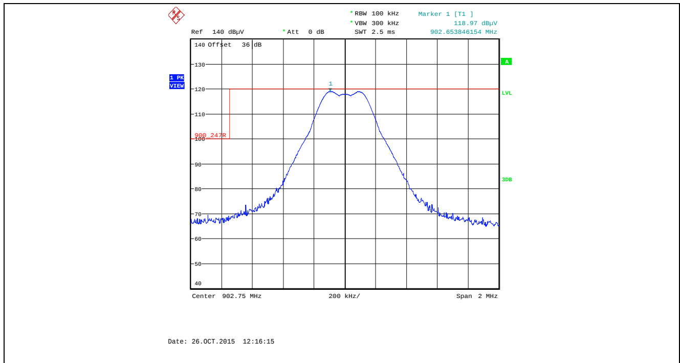
Plot 5.5.4.3.2.17. Band-Edge RF Radiated Emissions at 3 m, Horizontal Polarization Single Frequency Mode, Low End of Frequency Band, 902.75 MHz, XB2, Data Rate at 250 kbps
