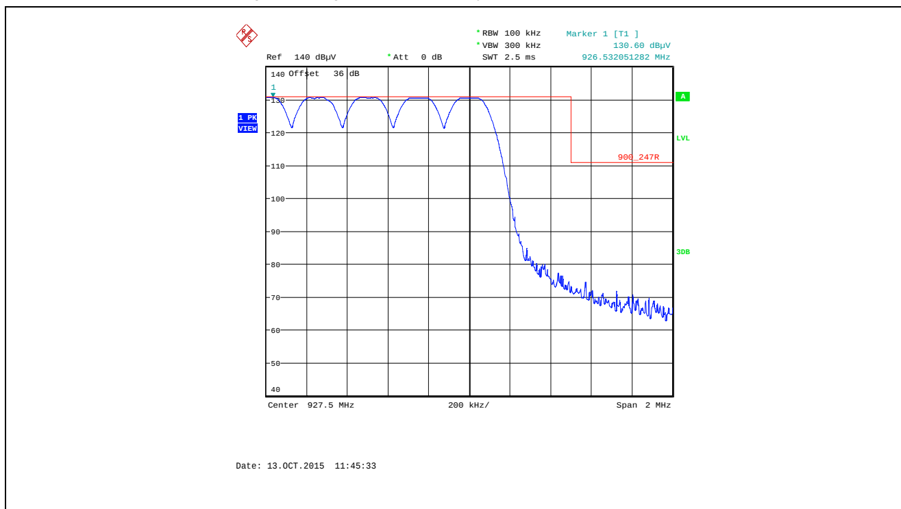
Plot 5.5.4.1.2.8. Band-Edge RF Radiated Emissions at 3 m, Vertical Polarization Pseudorandom Hopping Mode, High End of Frequency Band, 927.5 MHz, XB0, Data Rate at 10 kbps
