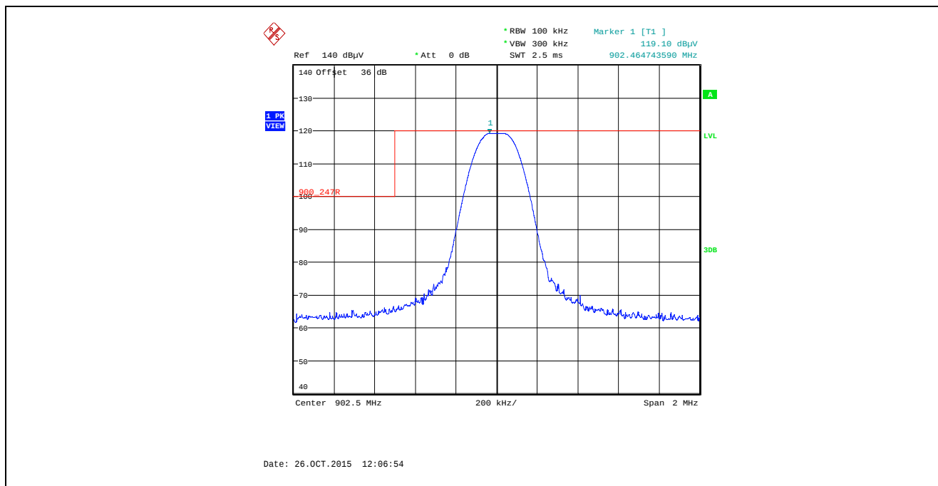
Plot 5.5.4.3.2.1. Band-Edge RF Radiated Emissions at 3 m, Horizontal Polarization Single Frequency Mode, Low End of Frequency Band, 902.5 MHz, XB0, Data Rate at 10 kbps
