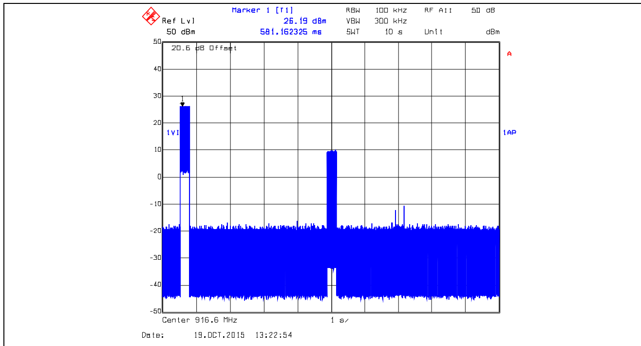
Plot 5.3.4.69. Time of Occupancy, 916.6 MHz, XTC0, Data Rate at 10 kbps Average time of occupancy = (Dwell Time) x (number of hops) = 272.75 ms x 1 = 272.75 ms < 0.4 sec within 10 sec
