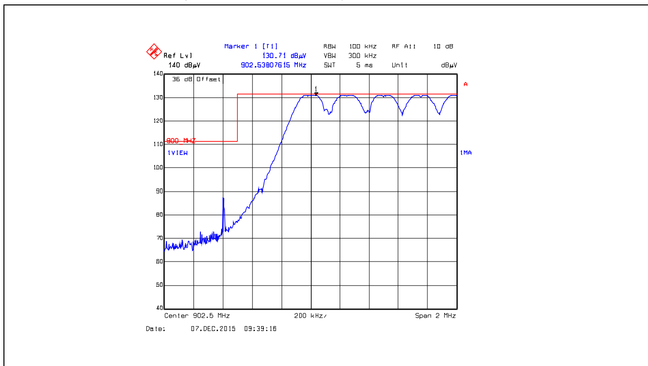
Plot 5.5.4.5.2.4. Band-Edge RF Radiated Emissions at 3 m, Vertical Polarization Pseudorandom Hopping Mode, Low End of Frequency Band, 902.5 MHz, XB0, Data Rate at 10 kbps
