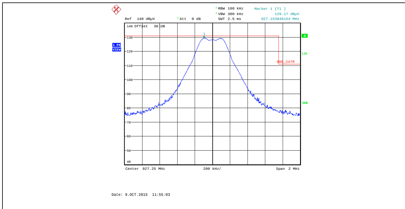
Plot 5.5.4.1.2.21. Band-Edge RF Radiated Emissions at 3 m, Horizontal Polarization Single Frequency Mode, High End of Frequency Band, 927.25 MHz, XB2, Data Rate at 250 kbps
