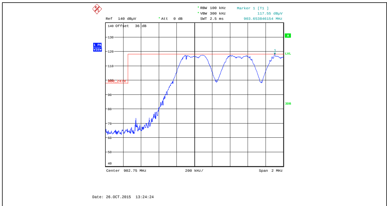
Plot 5.5.4.3.2.18. Band-Edge RF Radiated Emissions at 3 m, Horizontal Polarization Pseudorandom Hopping Mode, Low End of Frequency Band, 902.75 MHz, XB2, Data Rate at 250 kbps
