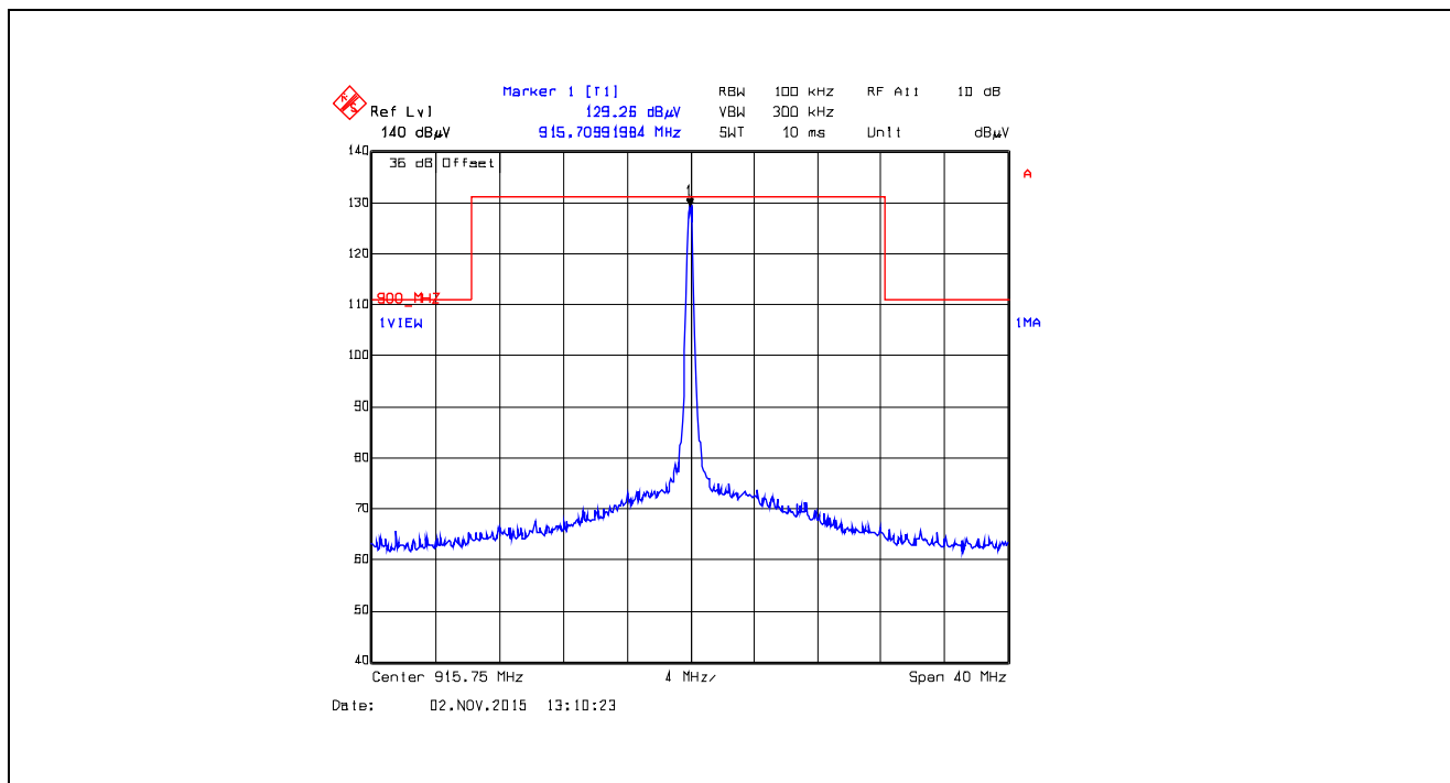
Plot 5.5.4.4.2.49. Band-Edge RF Radiated Emissions at 3 m, Horizontal Polarization Single Frequency Mode, Low End of Frequency Band, 915.75 MHz, XTCA1, Data Rate at 105kbps
