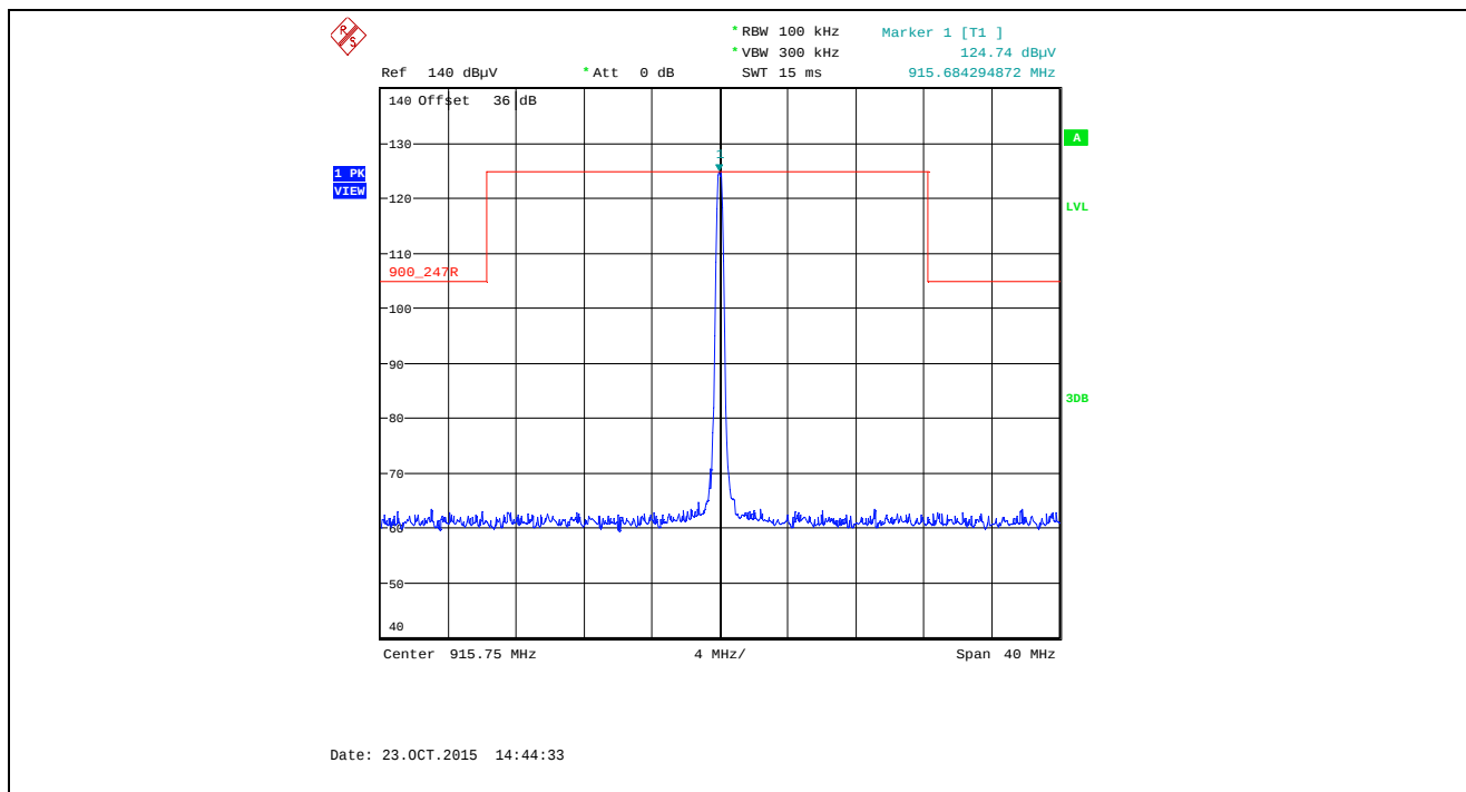
Plot 5.5.4.3.2.43. Band-Edge RF Radiated Emissions at 3 m, Vertical Polarization Single Frequency Mode, Low End of Frequency Band, 915.75 MHz, XTCA0, Data Rate at 10 kbps
