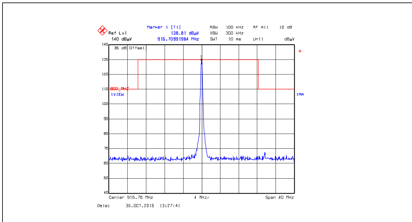
Plot 5.5.4.4.2.43. Band-Edge RF Radiated Emissions at 3 m, Vertical Polarization Single Frequency Mode, Low End of Frequency Band, 915.75 MHz, XTCA0, Data Rate at 10 kbps
