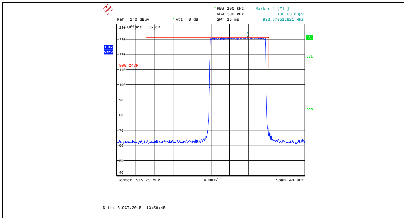
Plot 5.5.4.1.2.44. Band-Edge RF Radiated Emissions at 3 m, Vertical Polarization Pseudorandom Hopping Mode, Low End of Frequency Band, 915.75 MHz, XTCA0, Data Rate at 10 kbps
