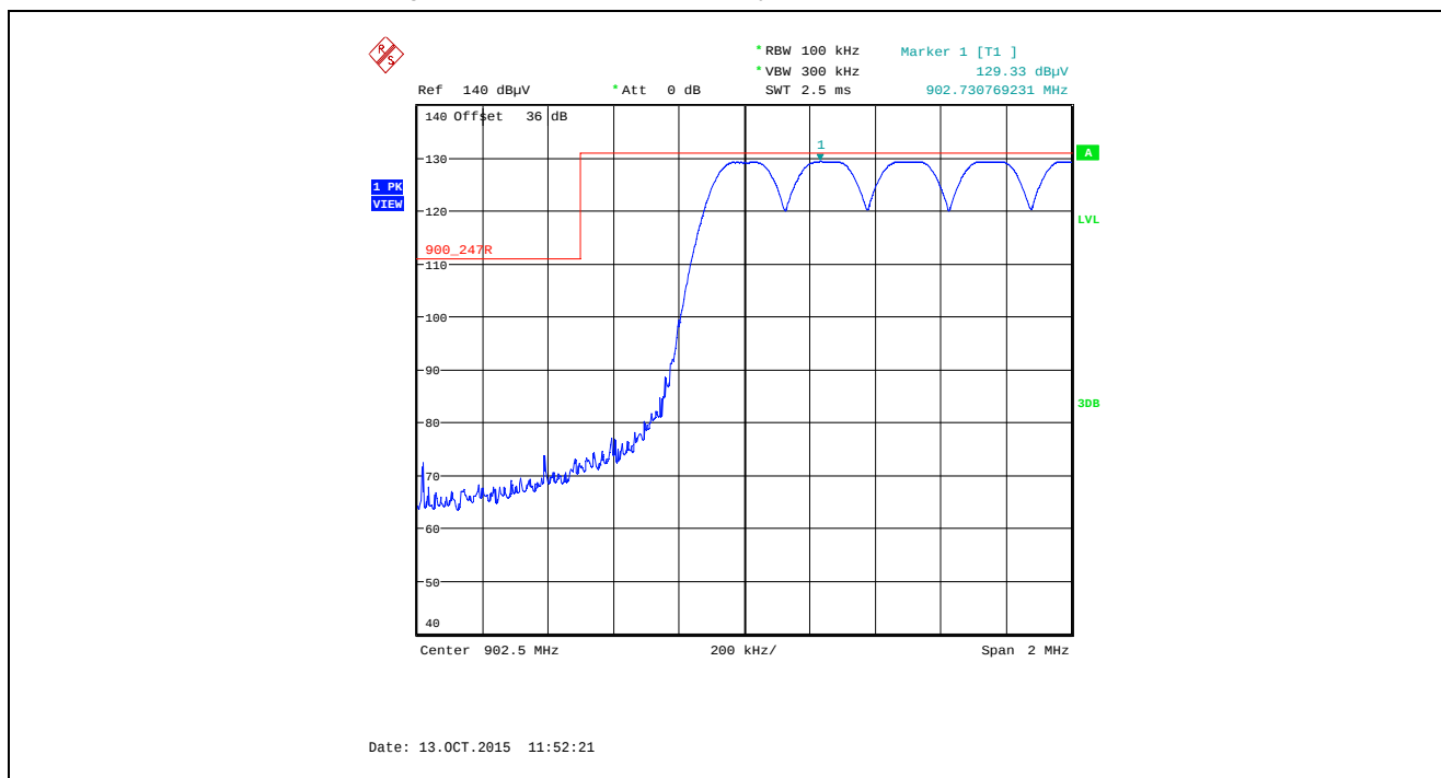
Plot 5.5.4.1.2.4. Band-Edge RF Radiated Emissions at 3 m, Vertical Polarization Pseudorandom Hopping Mode, Low End of Frequency Band, 902.5 MHz, XB0, Data Rate at 10 kbps
