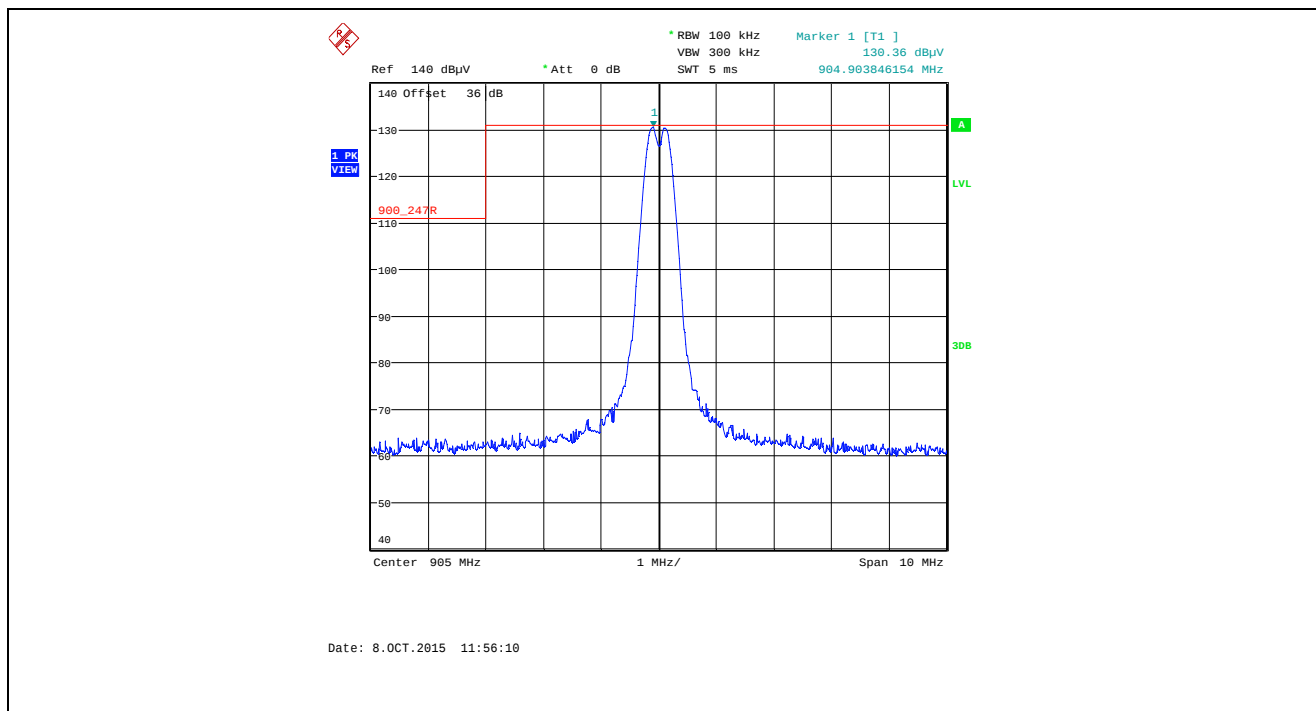
Plot 5.5.4.1.2.25. Band-Edge RF Radiated Emissions at 3 m, Horizontal Polarization Single Frequency Mode, Low End of Frequency Band, 905.0 MHz, XTC0, Data Rate at 10 kbps
