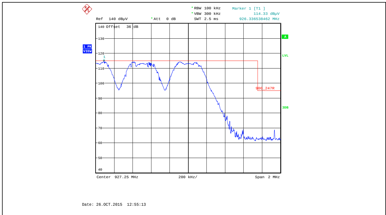
Plot 5.5.4.3.2.22. Band-Edge RF Radiated Emissions at 3 m, Horizontal Polarization Pseudorandom Hopping Mode, High End of Frequency Band, 927.25 MHz, XB2, Data Rate at 250 kbps
