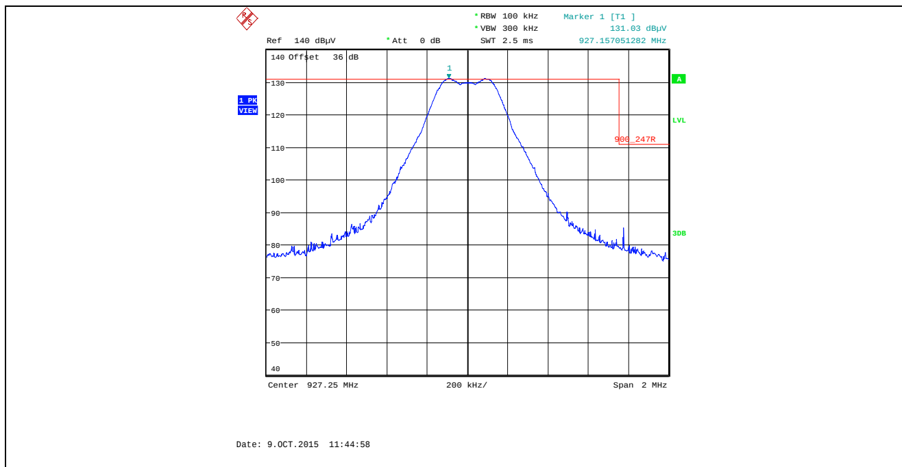
Plot 5.5.4.1.2.23. Band-Edge RF Radiated Emissions at 3 m, Vertical Polarization Single Frequency Mode, High End of Frequency Band, 927.25 MHz, XB2, Data Rate at 250 kbps
