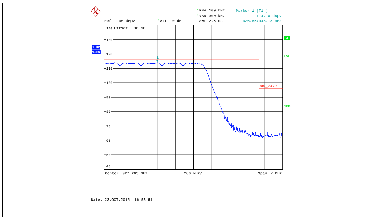
Plot 5.5.4.3.2.54. Band-Edge RF Radiated Emissions at 3 m, Horizontal Polarization Pseudorandom Hopping Mode, High End of Frequency Band, 927.265 MHz, XTCA1, Data Rate at 105kbps
