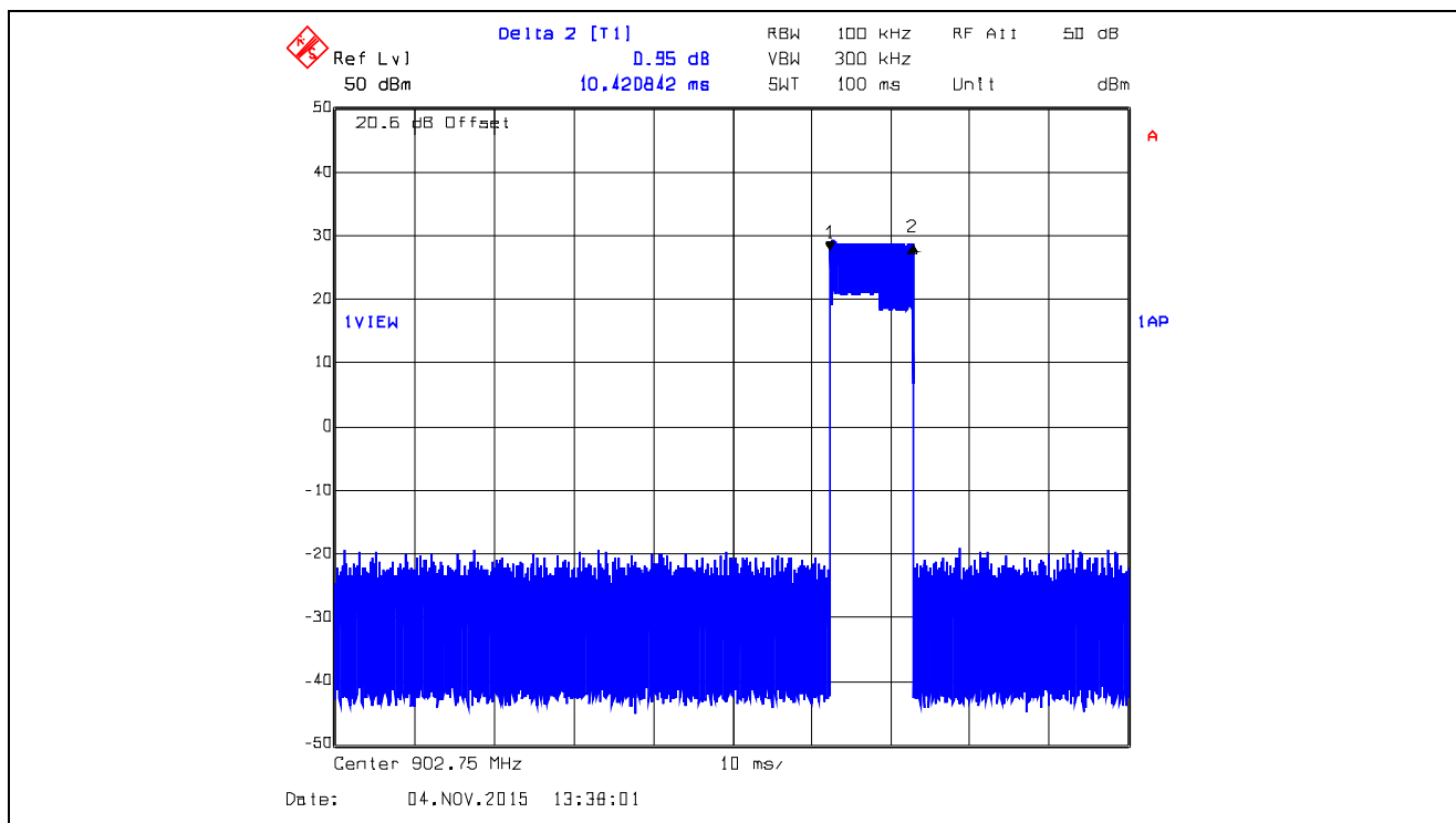
Plot 5.3.4.60. Time of Occupancy, 902.75 MHz, XBX2, Data Rate at 250 kbps Dwell Time @ 902.75 MHz = 10.420842 ms
