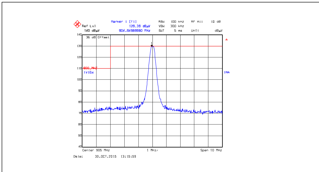
Plot 5.5.4.4.2.35. Band-Edge RF Radiated Emissions at 3 m, Vertical Polarization Single Frequency Mode, Low End of Frequency Band, 905.0 MHz, XTC1, Data Rate at 125 kbps
