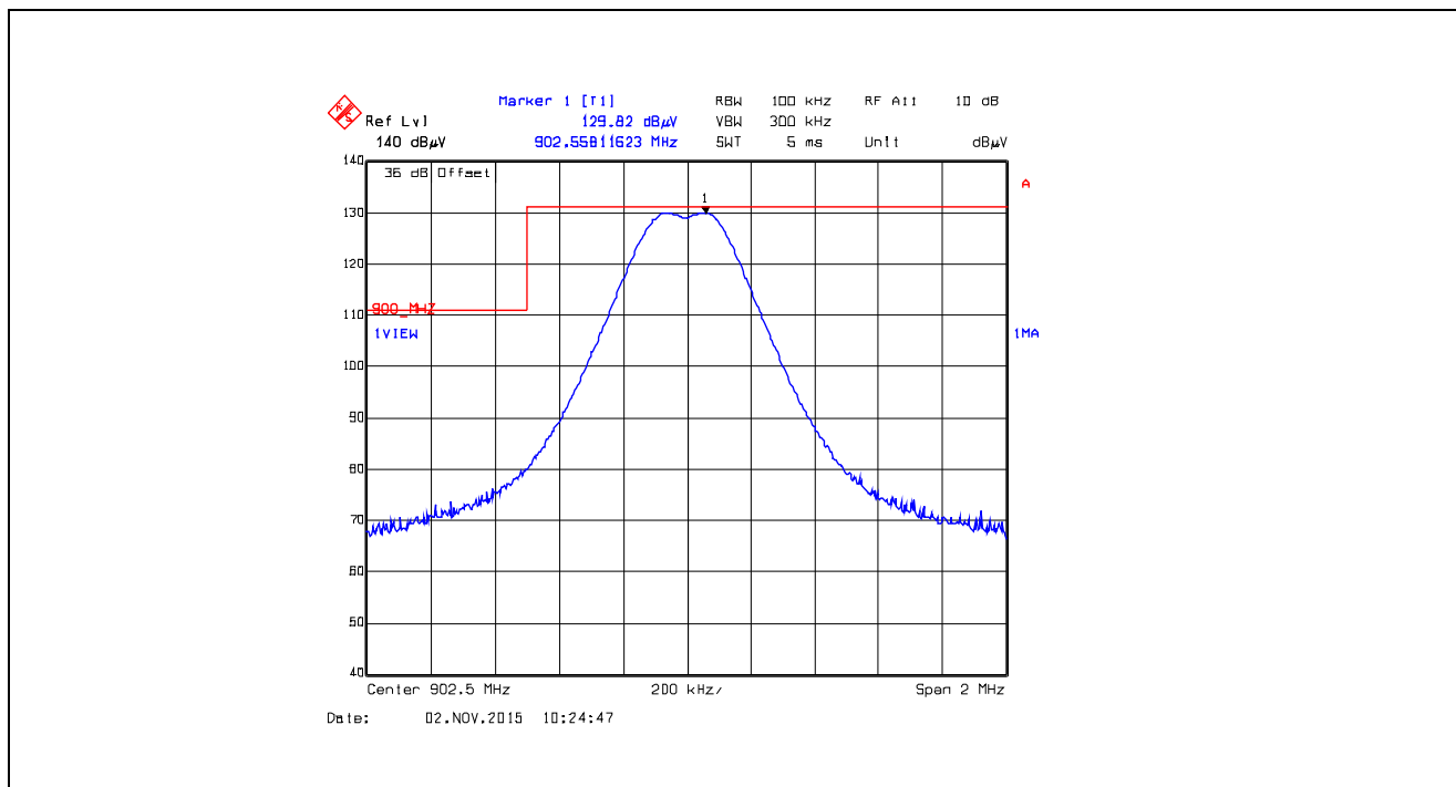
Plot 5.5.4.4.2.9. Band-Edge RF Radiated Emissions at 3 m, Horizontal Polarization Single Frequency Mode, Low End of Frequency Band, 902.5 MHz, XBX1, Data Rate at 110 kbps
