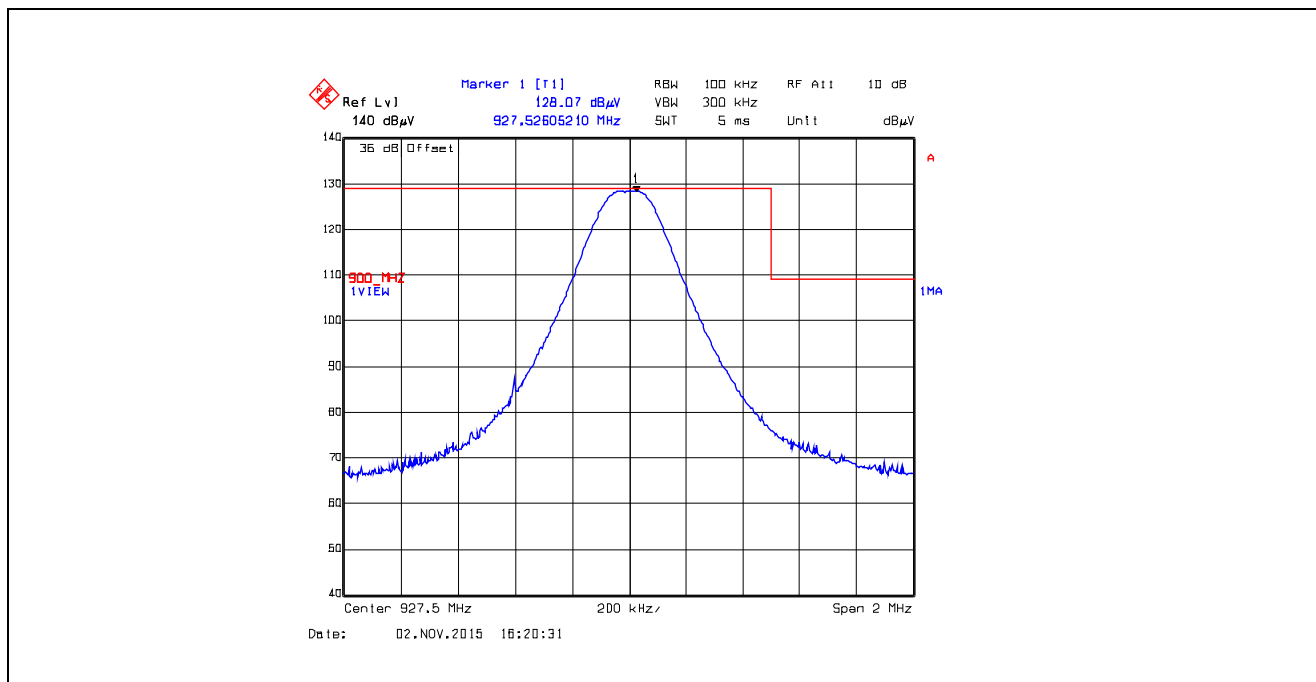
Plot 5.5.4.2.7. Band-Edge RF Radiated Emissions at 3 m, Vertical Polarization Single Frequency Mode, High End of Frequency Band, 927.5 MHz, XB0, Data Rate at 10 kbps
