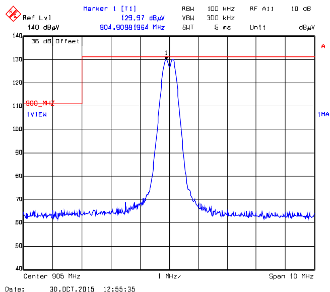
Plot 5.5.4.4.28. Band-Edge RF Radiated Emissions at 3 m, Vertical Polarization Pseudorandom Hopping Mode, Low End of Frequency Band, 905.0 MHz, XTC0, Data Rate at 10 kbps
