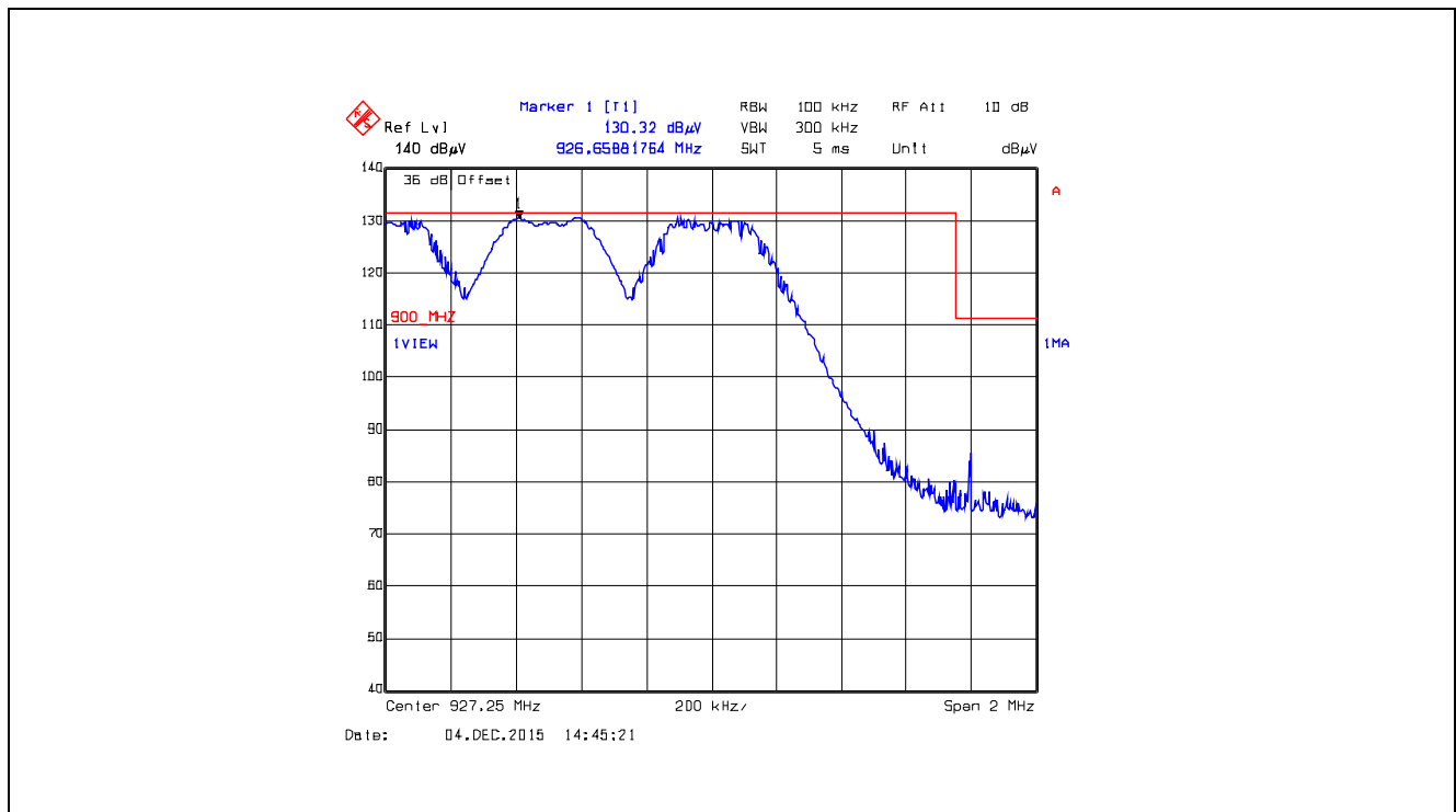
Plot 5.5.4.5.2.22. Band-Edge RF Radiated Emissions at 3 m, Horizontal Polarization Pseudorandom Hopping Mode, High End of Frequency Band, 927.25 MHz, XB2, Data Rate at 250 kbps
