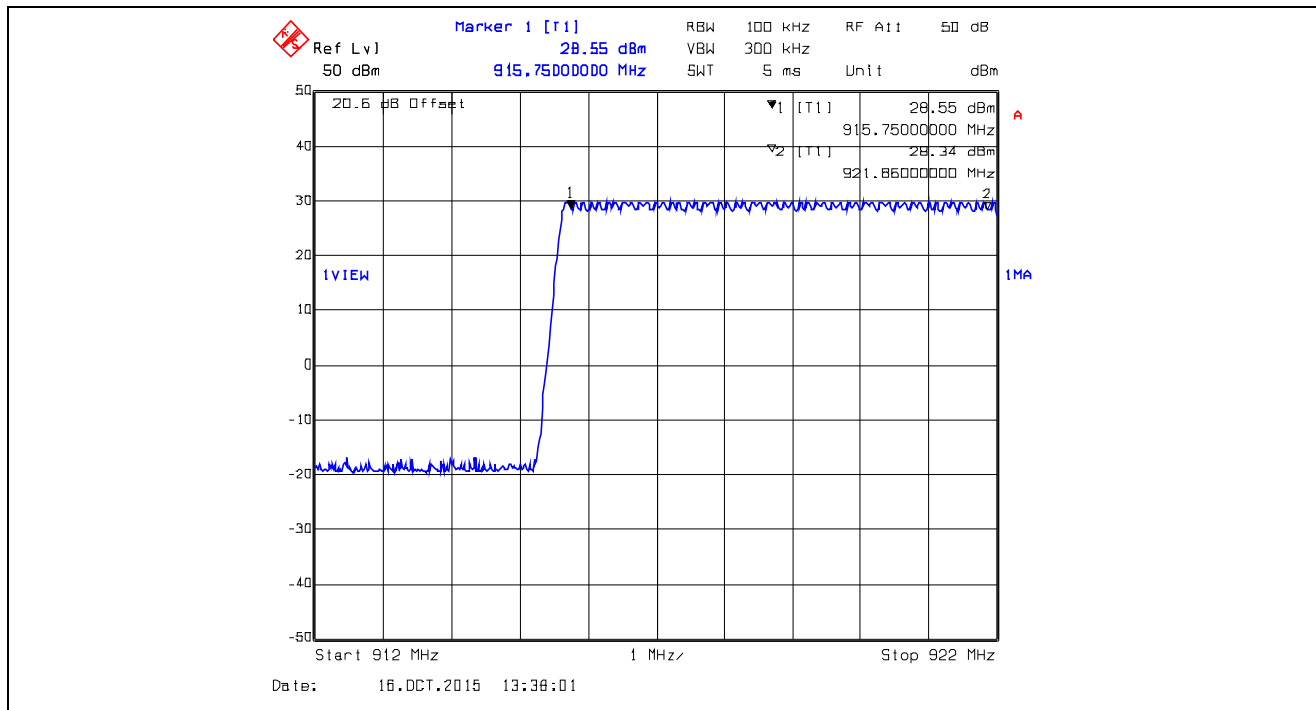
Plot 5.3.4.41. Number of Hopping Frequencies, XTCA0, Data Rate at 10 kbps 27 Hopping Channels from 912 – 922 MHz
