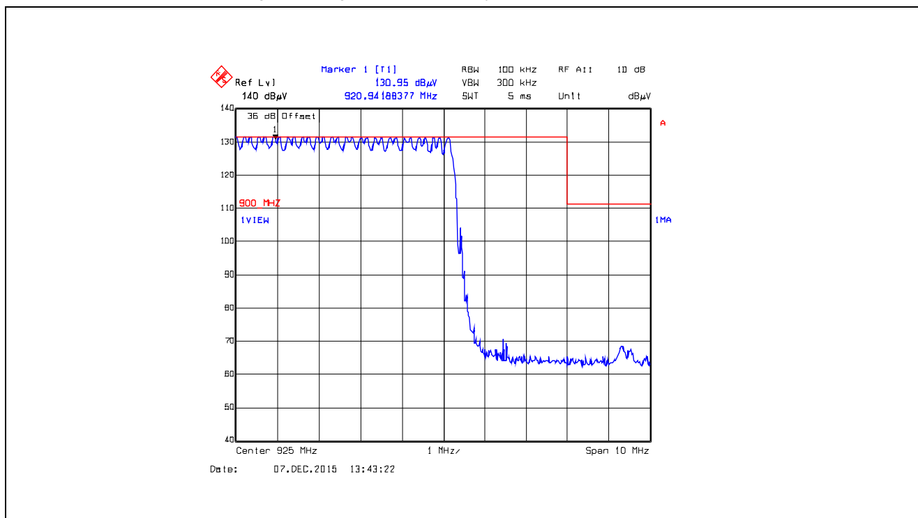
Plot 5.5.4.5.2.32. Band-Edge RF Radiated Emissions at 3 m, Vertical Polarization Pseudorandom Hopping Mode, High End of Frequency Band, 925.0 MHz, XTC0, Data Rate at 10 kbps
