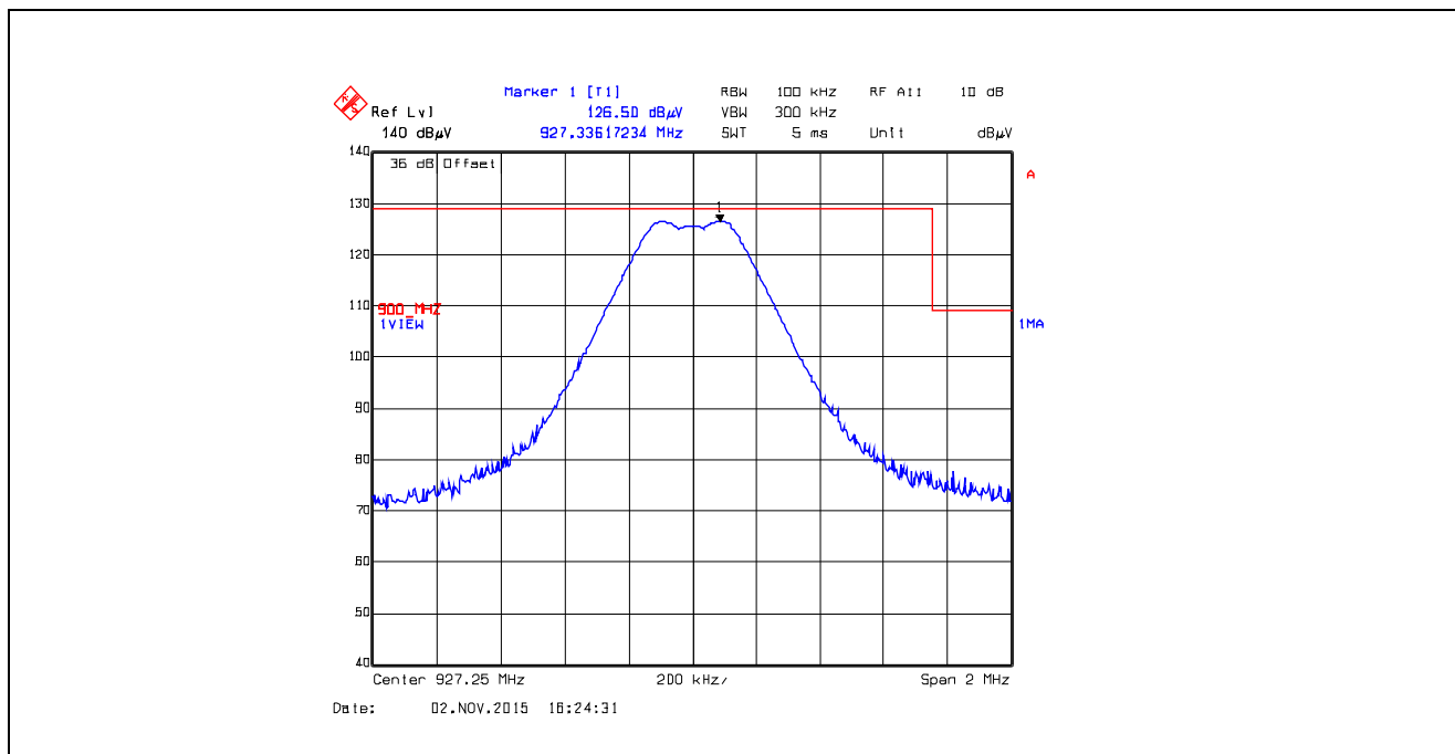
Plot 5.5.4.2.23. Band-Edge RF Radiated Emissions at 3 m, Vertical Polarization Single Frequency Mode, High End of Frequency Band, 927.25 MHz, XB2, Data Rate at 250 kbps
