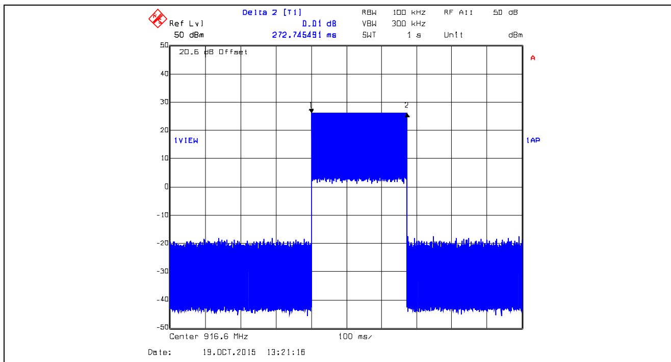
Plot 5.3.4.68. Time of Occupancy, 916.6 MHz, XTC0, Data Rate at 10 kbps Dwell Time @ 916.6 MHz = 272.75 ms
