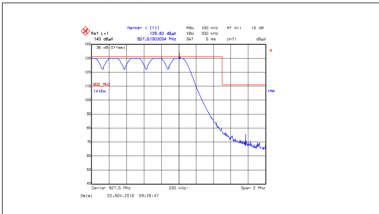
Plot 5.5.4.4.2.8. Band-Edge RF Radiated Emissions at 3 m, Vertical Polarization Pseudorandom Hopping Mode, High End of Frequency Band, 927.5 MHz, XB0, Data Rate at 10 kbps
