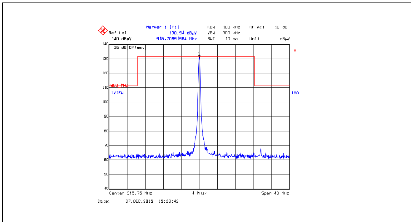
Plot 5.5.4.5.2.41. Band-Edge RF Radiated Emissions at 3 m, Horizontal Polarization Single Frequency Mode, Low End of Frequency Band, 915.75 MHz, XTCA0, Data Rate at 10 kbps
