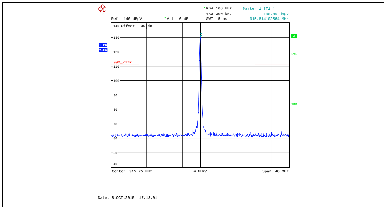
Plot 5.5.4.1.2.43. Band-Edge RF Radiated Emissions at 3 m, Vertical Polarization Single Frequency Mode, Low End of Frequency Band, 915.75 MHz, XTCA0, Data Rate at 10 kbps
