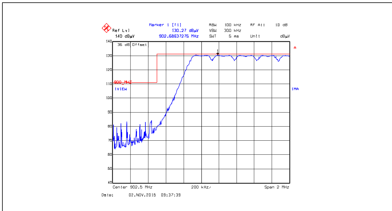
Plot 5.5.4.4.2.12. Band-Edge RF Radiated Emissions at 3 m, Vertical Polarization Pseudorandom Hopping Mode, Low End of Frequency Band, 902.5 MHz, XBX1, Data Rate at 110 kbps
