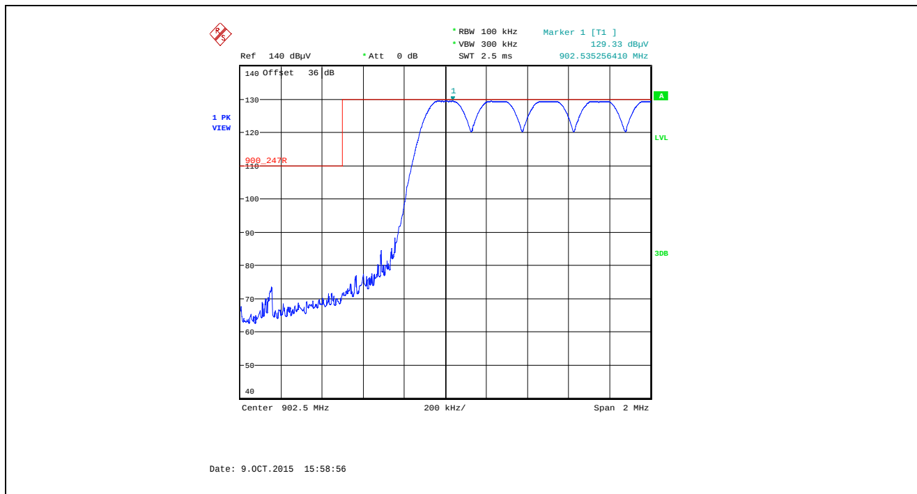
Plot 5.5.4.1.2.2. Band-Edge RF Radiated Emissions at 3 m, Horizontal Polarization Pseudorandom Hopping Mode, Low End of Frequency Band, 902.5 MHz, XB0, Data Rate at 10 kbps
