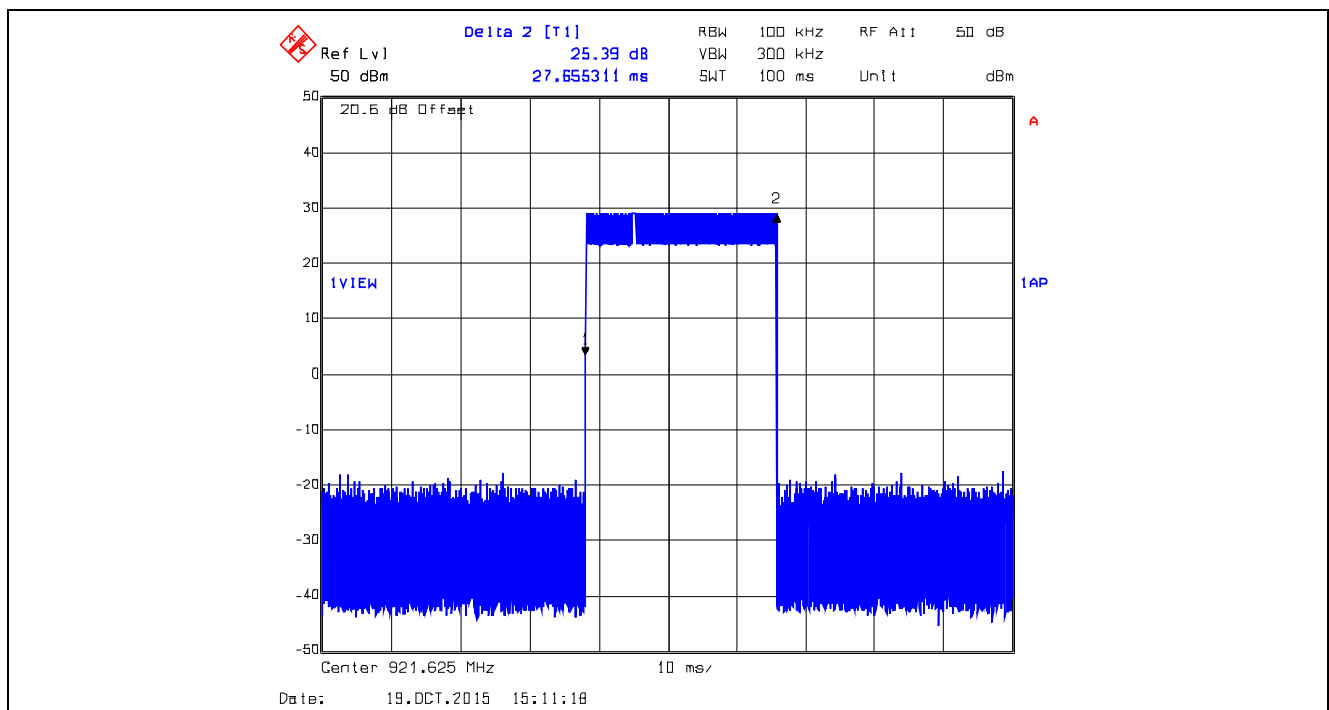
Plot 5.3.4.86. Time of Occupancy, 921.625 MHz, XTCA1, Data Rate at 105 kbps Dwell Time @ 921.625 MHz = 27.6553 ms
