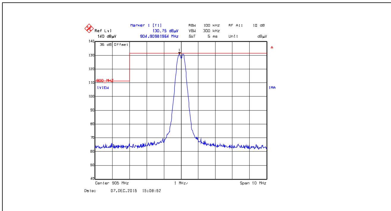
Plot 5.5.4.5.2.25. Band-Edge RF Radiated Emissions at 3 m, Horizontal Polarization Single Frequency Mode, Low End of Frequency Band, 905.0 MHz, XTC0, Data Rate at 10 kbps
