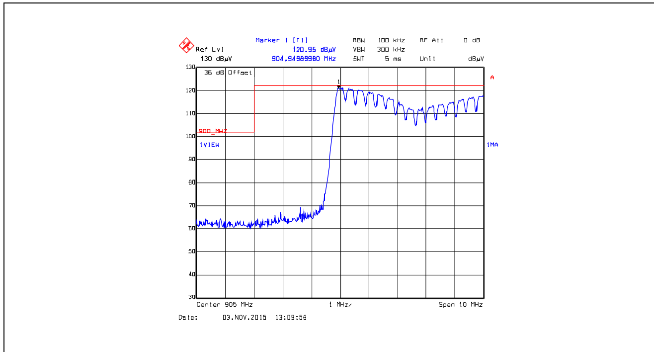
Plot 5.5.4.2.2.34. Band-Edge RF Radiated Emissions at 3 m, Horizontal Polarization Pseudorandom Hopping Mode, Low End of Frequency Band, 905.0 MHz, XTC1, Data Rate at 125 kbps
