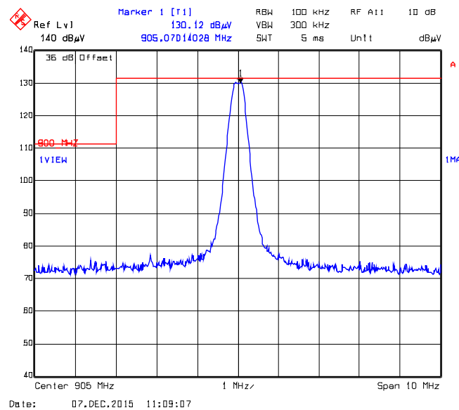
Plot 5.5.4.5.2.36. Band-Edge RF Radiated Emissions at 3 m, Vertical Polarization Pseudorandom Hopping Mode, Low End of Frequency Band, 905.0 MHz, XTC1, Data Rate at 125 kbps
