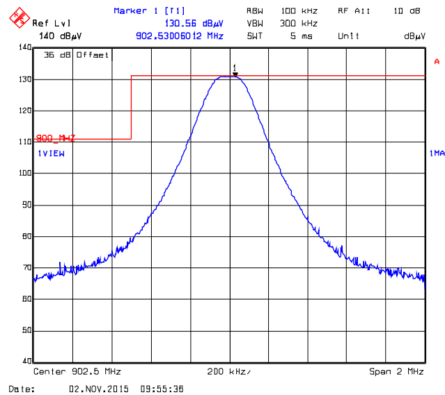
Plot 5.5.4.4.2.2. Band-Edge RF Radiated Emissions at 3 m, Horizontal Polarization Pseudorandom Hopping Mode, Low End of Frequency Band, 902.5 MHz, XB0, Data Rate at 10 kbps
