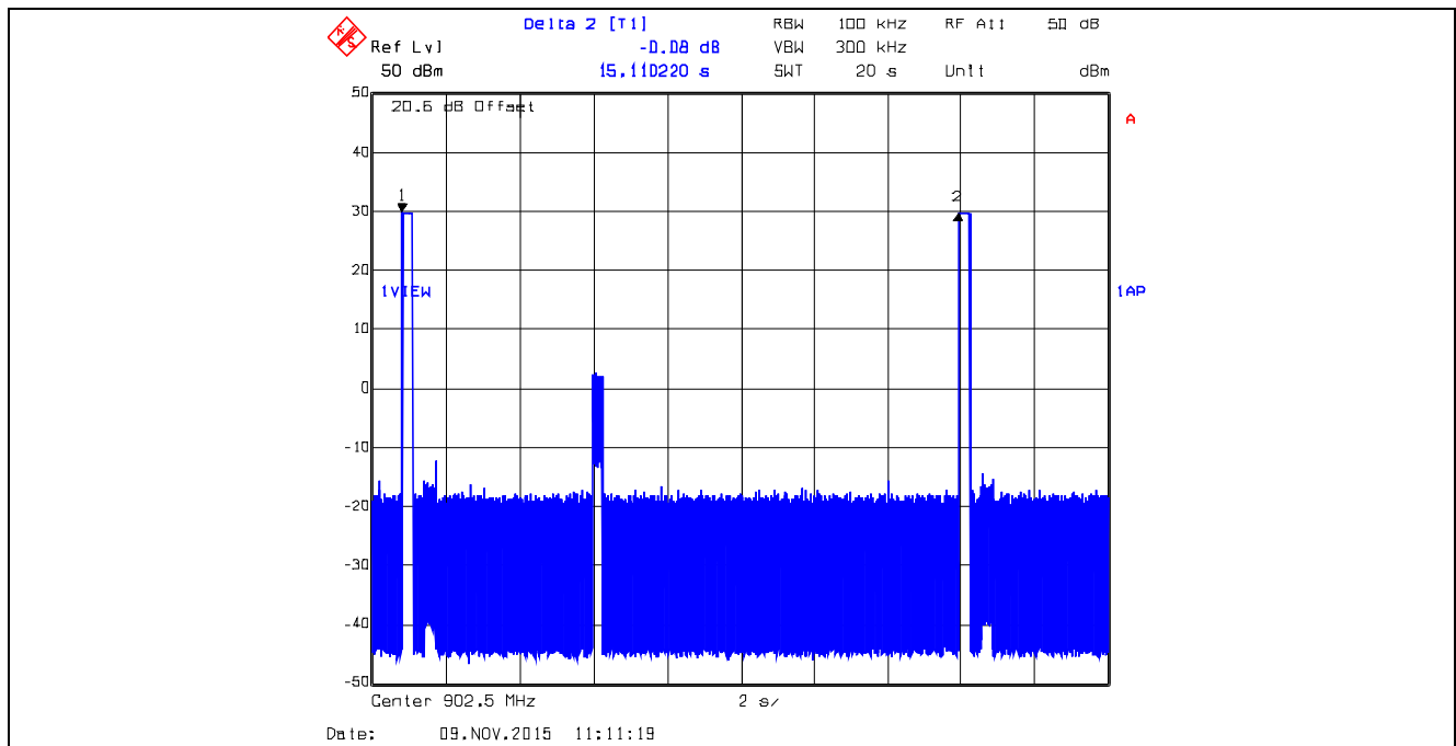
Plot 5.3.4.49. Time of Occupancy, 902.5 MHz XB0, Data Rate at 10 kbps Average time of occupancy = 20 \times (T_{\text{on}}) / (T_{\text{total}}) = 20 \times 0.3006012\text{s} / 15.1102\text{s} = 0.3979\text{s} < 0.4\text{s}
