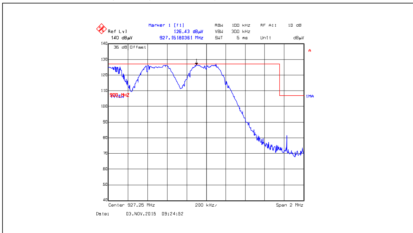
Plot 5.5.4.2.24. Band-Edge RF Radiated Emissions at 3 m, Vertical Polarization Pseudorandom Hopping Mode, High End of Frequency Band, 927.25 MHz, XB2, Data Rate at 250 kbps
