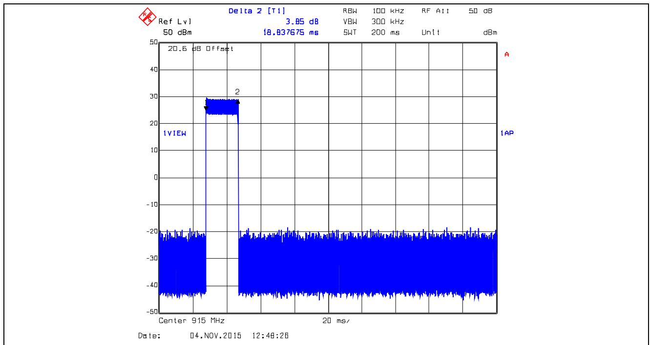
Plot 5.3.4.56. Time of Occupancy, 915.0 MHz, XB1, Data Rate at 110 kbps Dwell Time @ 915.00 MHz = 18.8377 ms
