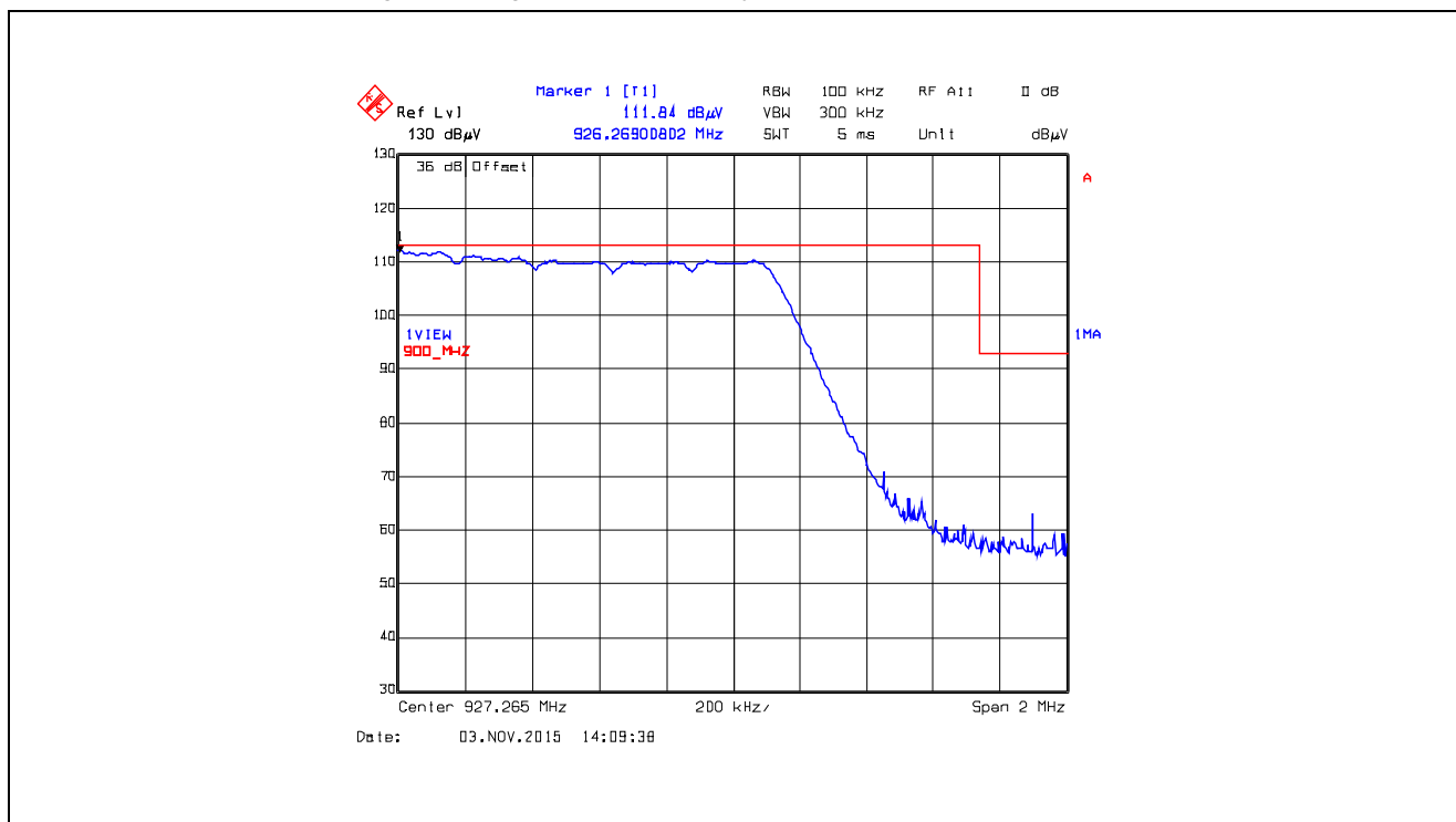
Plot 5.5.4.2.2.54. Band-Edge RF Radiated Emissions at 3 m, Horizontal Polarization Pseudorandom Hopping Mode, High End of Frequency Band, 927.265 MHz, XTCA1, Data Rate at 105kbps
