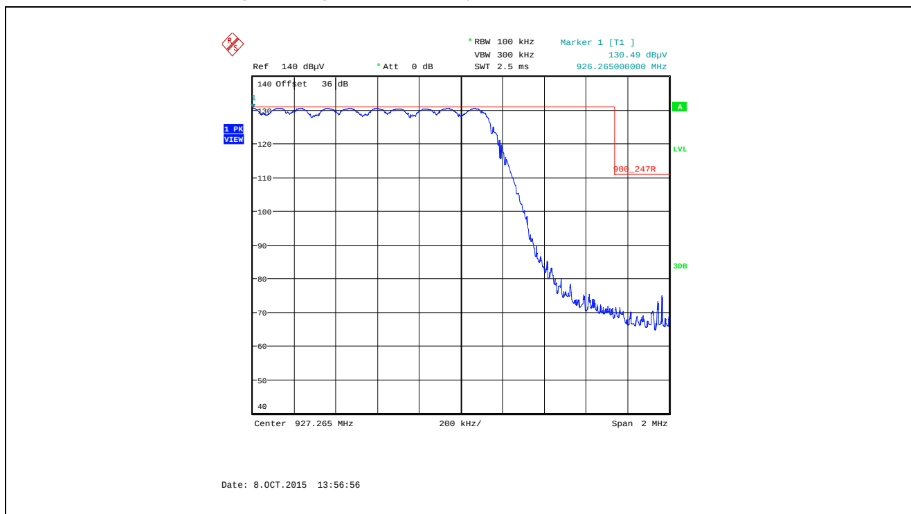
Plot 5.5.4.1.2.48. Band-Edge RF Radiated Emissions at 3 m, Vertical Polarization Pseudorandom Hopping Mode, High End of Frequency Band, 927.265 MHz, XTCA0, Data Rate at 10 kbps
