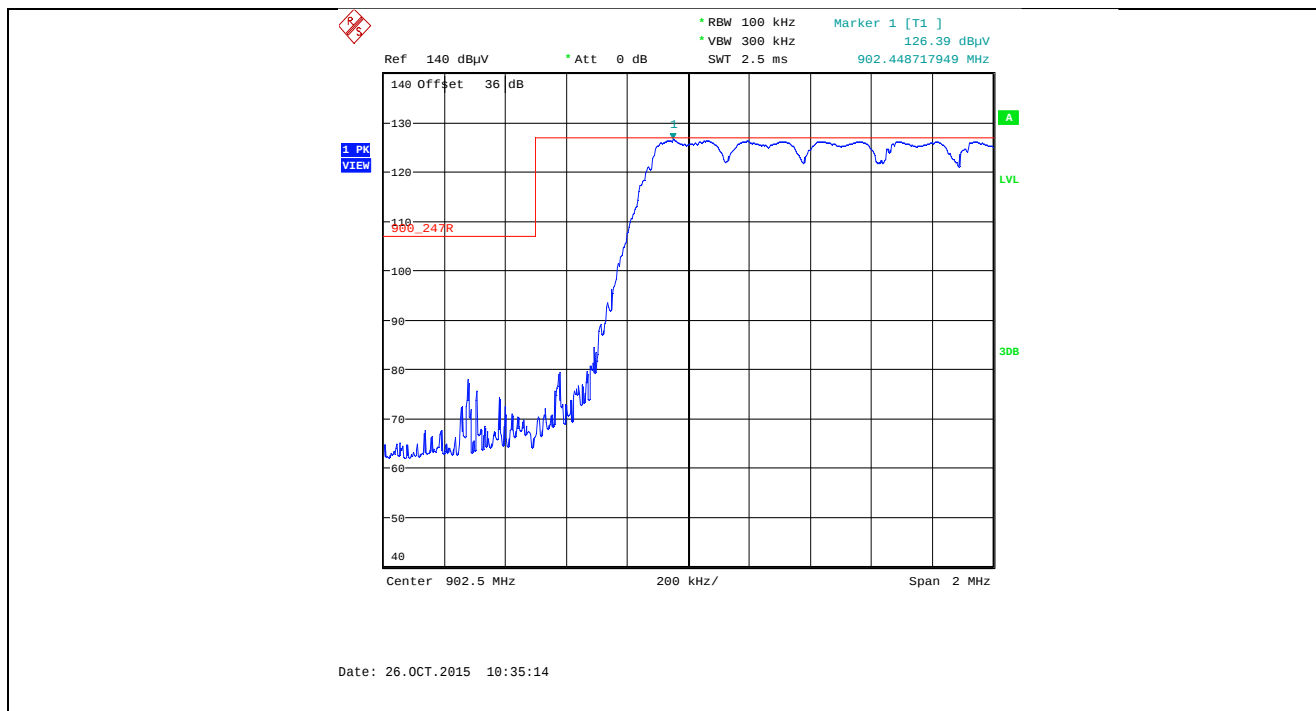
Plot 5.5.4.3.2.12. Band-Edge RF Radiated Emissions at 3 m, Vertical Polarization Pseudorandom Hopping Mode, Low End of Frequency Band, 902.5 MHz, XB1, Data Rate at 110 kbps
