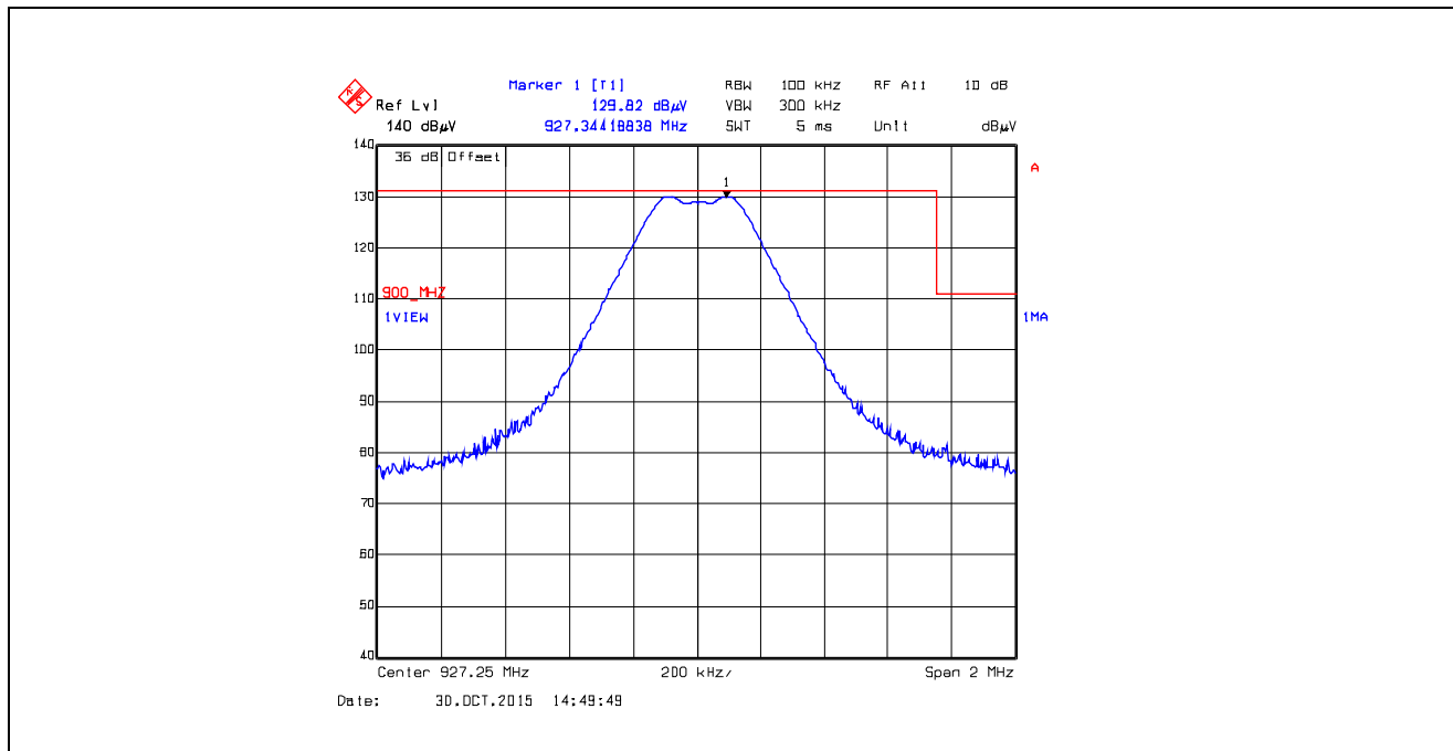
Plot 5.5.4.4.24. Band-Edge RF Radiated Emissions at 3 m, Vertical Polarization Pseudorandom Hopping Mode, High End of Frequency Band, 927.25 MHz, XB2, Data Rate at 250 kbps
