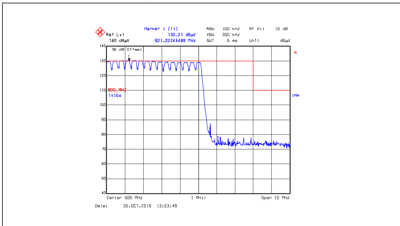
Plot 5.5.4.4.2.40. Band-Edge RF Radiated Emissions at 3 m, Vertical Polarization Pseudorandom Hopping Mode, High End of Frequency Band, 925.0 MHz, XTC1, Data Rate at 125 kbps
