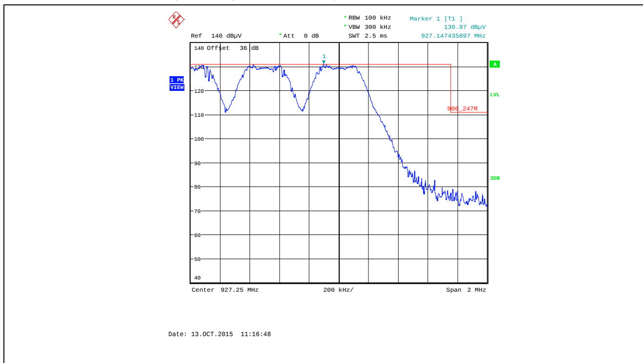
Plot 5.5.4.1.2.24. Band-Edge RF Radiated Emissions at 3 m, Vertical Polarization Pseudorandom Hopping Mode, High End of Frequency Band, 927.25 MHz, XB2, Data Rate at 250 kbps
