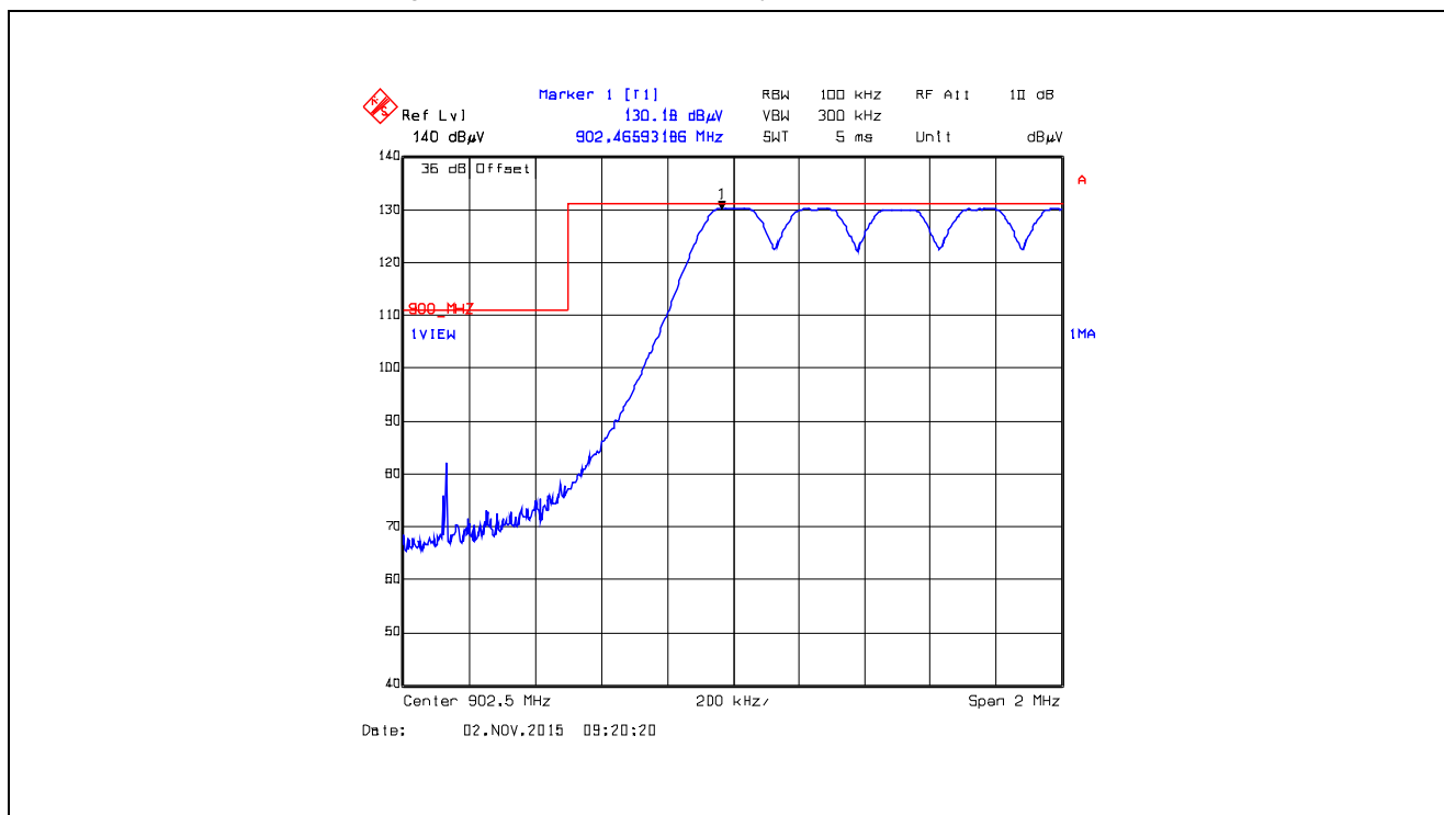
Plot 5.5.4.4.2.4. Band-Edge RF Radiated Emissions at 3 m, Vertical Polarization Pseudorandom Hopping Mode, Low End of Frequency Band, 902.5 MHz, XB0, Data Rate at 10 kbps
