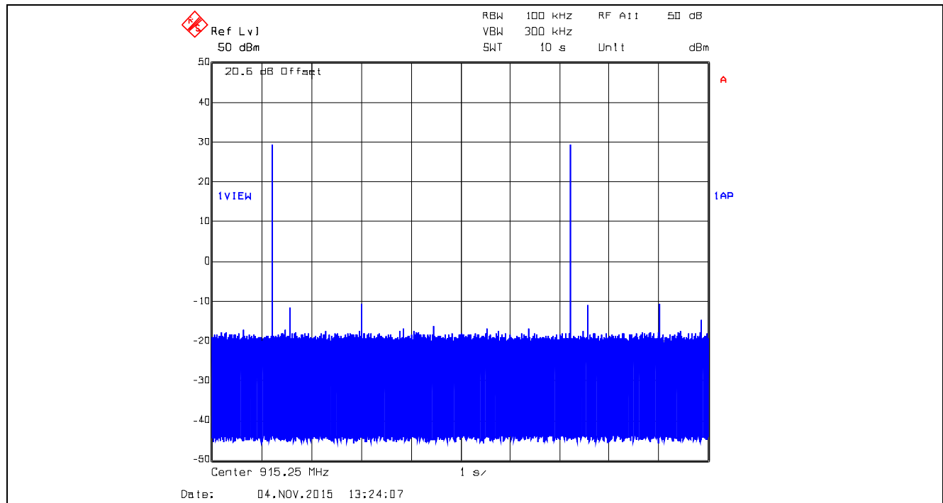
Plot 5.3.4.63. Time of Occupancy, 915.25 MHz, XB2, Data Rate at 250 kbps Average time of occupancy = (Dwell Time) x (number of hops) = 10.4208 ms x 2 = 20.8416 ms < 0.4 sec within 10 sec
