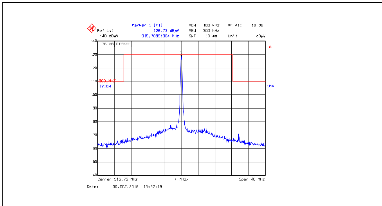
Plot 5.5.4.4.2.51. Band-Edge RF Radiated Emissions at 3 m, Vertical Polarization Single Frequency Mode, Low End of Frequency Band, 915.75 MHz, XTCA1, Data Rate at 105kbps
