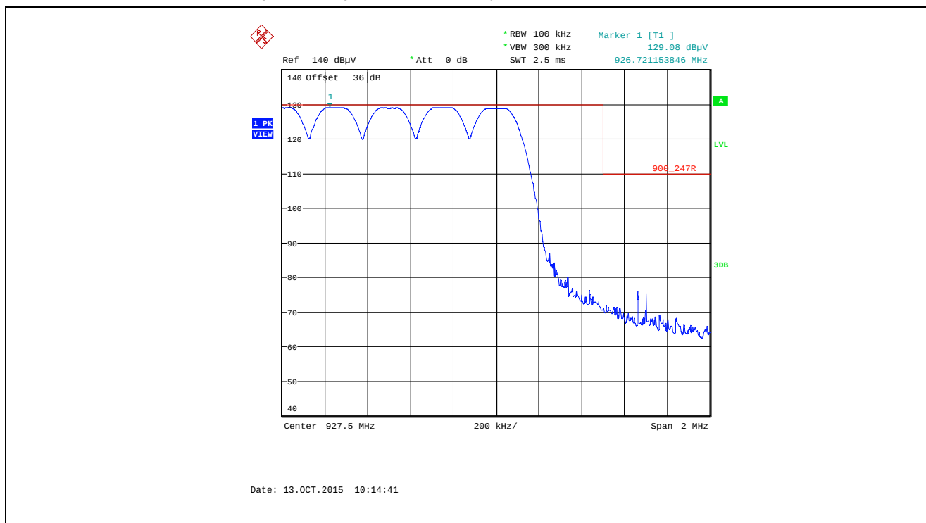
Plot 5.5.4.1.2.6. Band-Edge RF Radiated Emissions at 3 m, Horizontal Polarization Pseudorandom Hopping Mode, High End of Frequency Band, 927.5 MHz, XB0, Data Rate at 10 kbps
