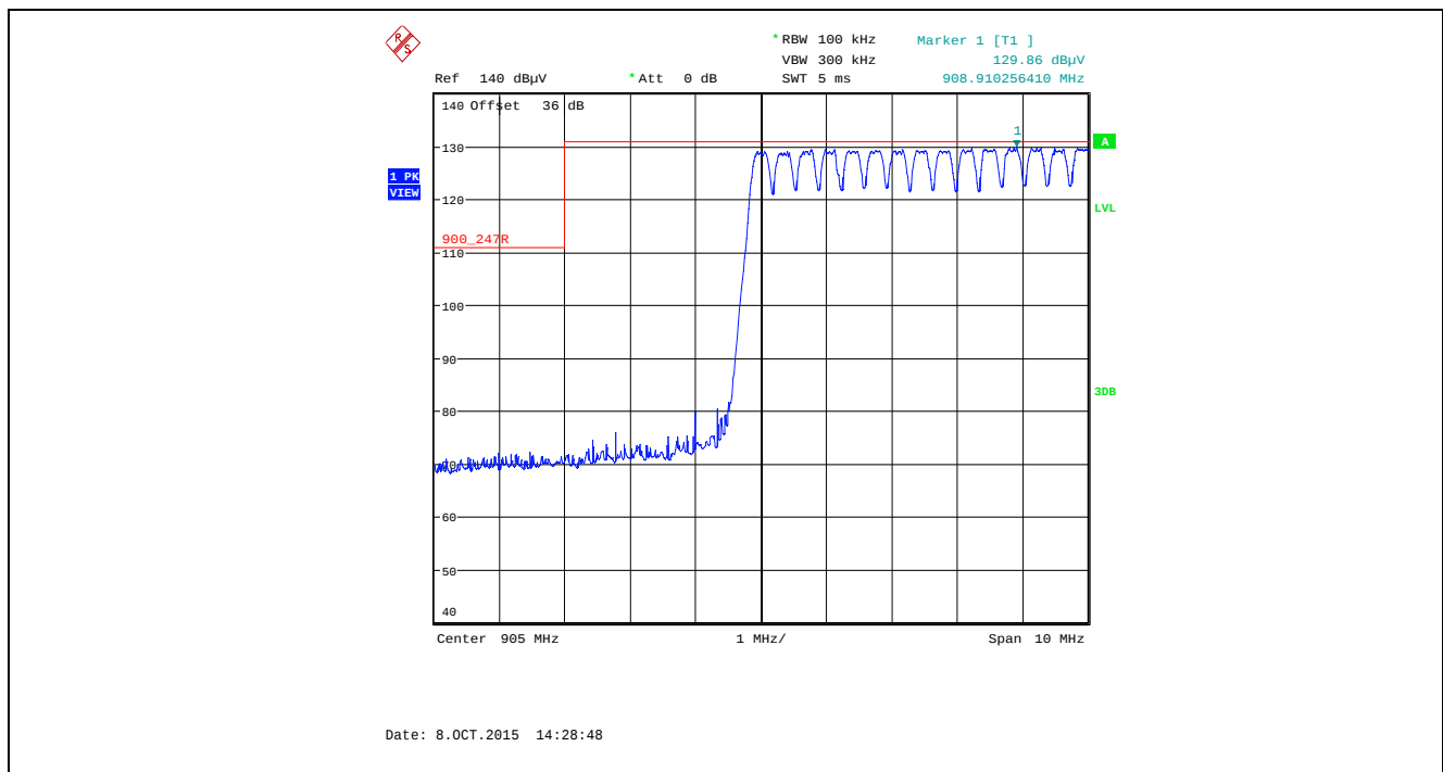
Plot 5.5.4.1.2.36. Band-Edge RF Radiated Emissions at 3 m, Vertical Polarization Pseudorandom Hopping Mode, Low End of Frequency Band, 905.0 MHz, XTC1, Data Rate at 125 kbps
