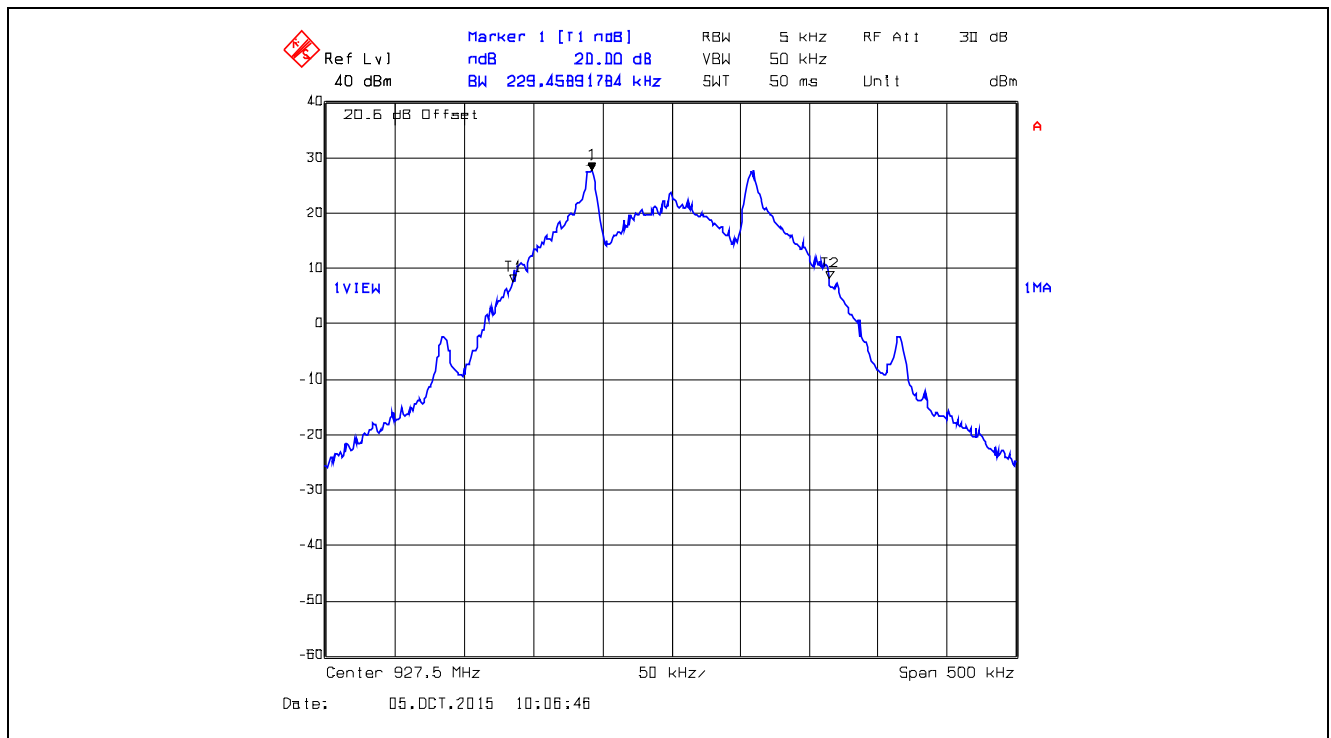
Plot 5.3.4.6. 20 dB Bandwidth, 927.5 MHz, XB1, Data Rate at 110 kbps
