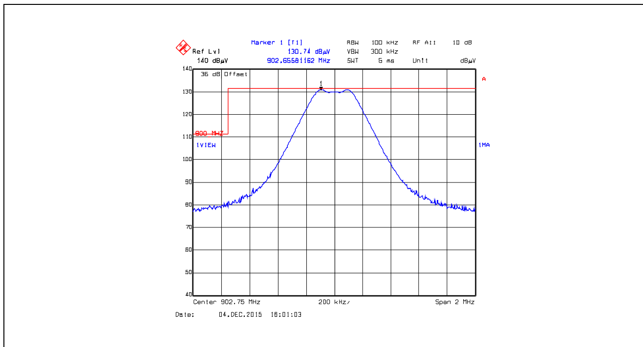
Plot 5.5.4.5.2.19. Band-Edge RF Radiated Emissions at 3 m, Vertical Polarization Single Frequency Mode, Low End of Frequency Band, 902.75 MHz, XB2, Data Rate at 250 kbps
