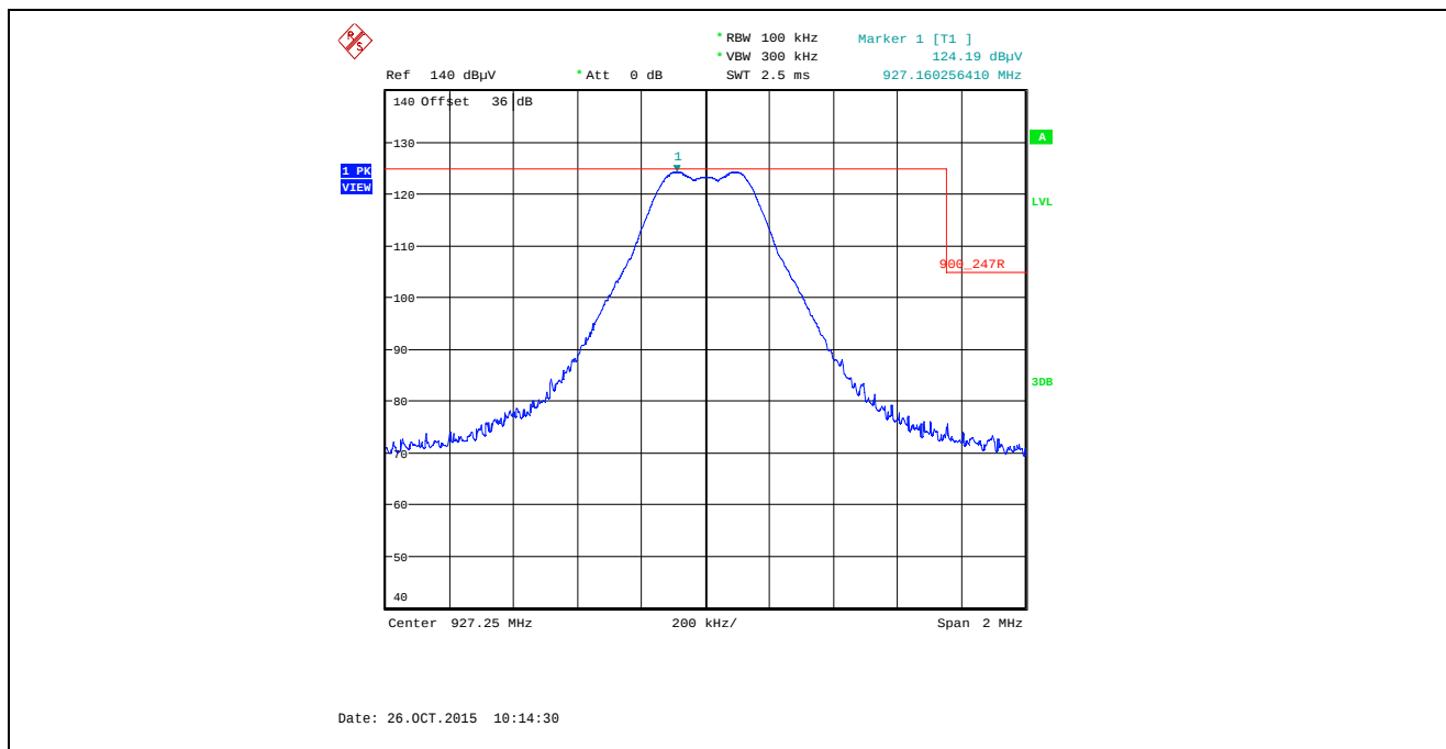
Plot 5.5.4.3.2.23. Band-Edge RF Radiated Emissions at 3 m, Vertical Polarization Single Frequency Mode, High End of Frequency Band, 927.25 MHz, XB2, Data Rate at 250 kbps
