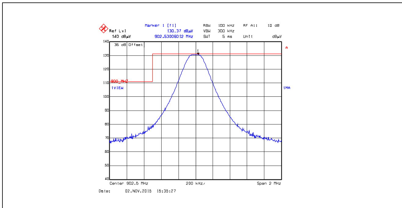
Plot 5.5.4.2.3. Band-Edge RF Radiated Emissions at 3 m, Vertical Polarization Single Frequency Mode, Low End of Frequency Band, 902.5 MHz, XB0, Data Rate at 10 kbps
