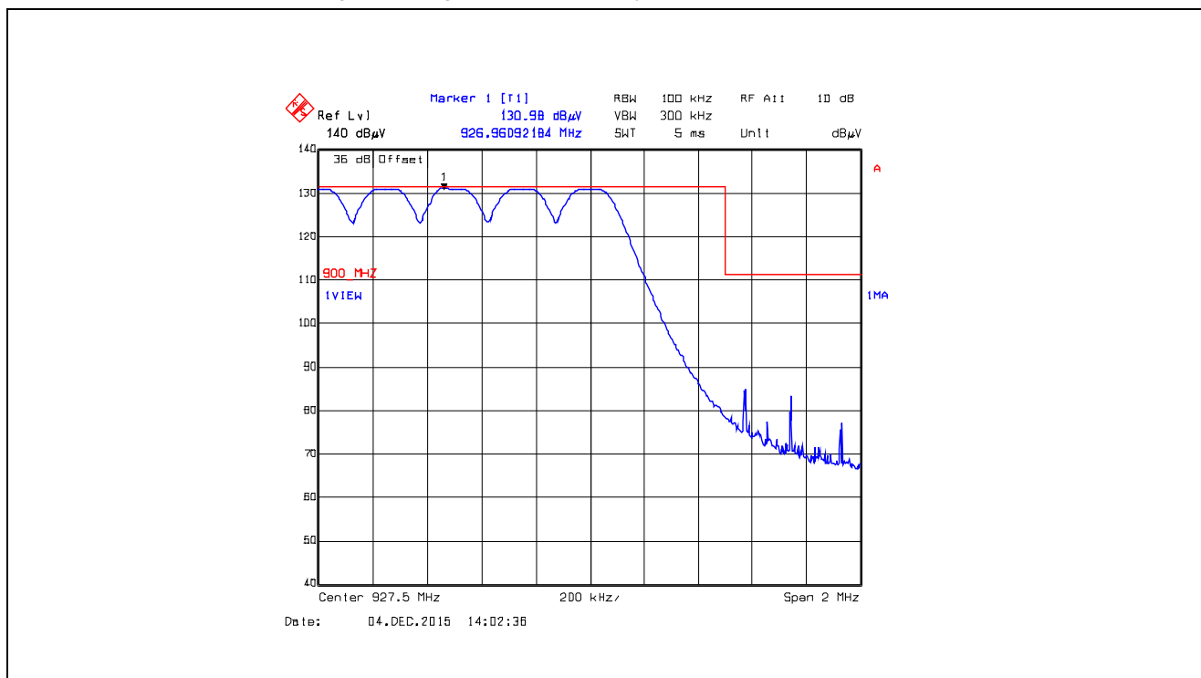
Plot 5.5.4.5.2.6. Band-Edge RF Radiated Emissions at 3 m, Horizontal Polarization Pseudorandom Hopping Mode, High End of Frequency Band, 927.5 MHz, XB0, Data Rate at 10 kbps
