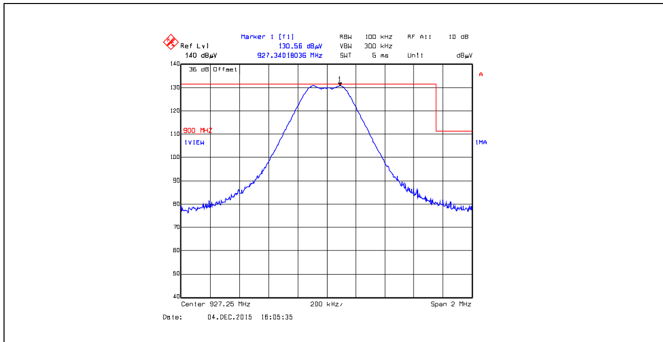
Plot 5.5.4.5.2.24. Band-Edge RF Radiated Emissions at 3 m, Vertical Polarization Pseudorandom Hopping Mode, High End of Frequency Band, 927.25 MHz, XB2, Data Rate at 250 kbps
