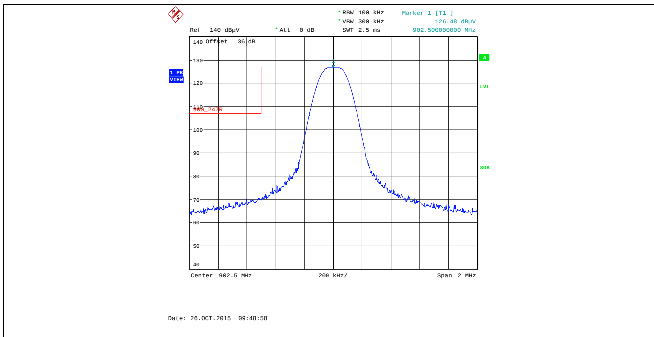
Plot 5.5.4.3.2.3. Band-Edge RF Radiated Emissions at 3 m, Vertical Polarization Single Frequency Mode, Low End of Frequency Band, 902.5 MHz, XB0, Data Rate at 10 kbps
