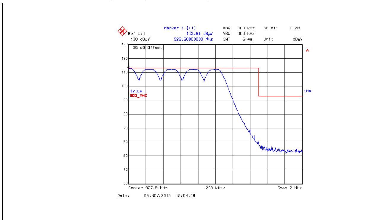
Plot 5.5.4.2.6. Band-Edge RF Radiated Emissions at 3 m, Horizontal Polarization Pseudorandom Hopping Mode, High End of Frequency Band, 927.5 MHz, XB0, Data Rate at 10 kbps
