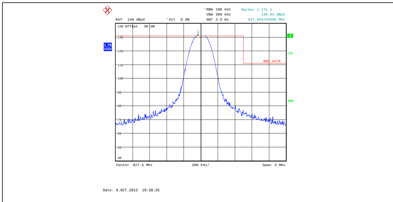
Plot 5.5.4.1.2.7. Band-Edge RF Radiated Emissions at 3 m, Vertical Polarization Single Frequency Mode, High End of Frequency Band, 927.5 MHz, XB0, Data Rate at 10 kbps
