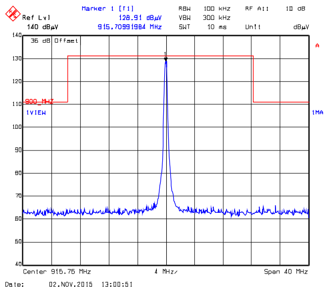
Plot 5.5.4.4.2.42. Band-Edge RF Radiated Emissions at 3 m, Horizontal Polarization Pseudorandom Hopping Mode, Low End of Frequency Band, 915.75 MHz, XTCA0, Data Rate at 10 kbps
