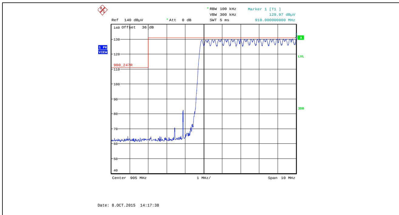
Plot 5.5.4.1.2.28. Band-Edge RF Radiated Emissions at 3 m, Vertical Polarization Pseudorandom Hopping Mode, Low End of Frequency Band, 905.0 MHz, XTC0, Data Rate at 10 kbps
