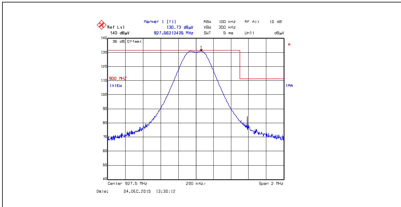
Plot 5.5.4.5.2.14. Band-Edge RF Radiated Emissions at 3 m, Horizontal Polarization Pseudorandom Hopping Mode, High End of Frequency Band, 927.5 MHz, XBX1, Data Rate at 110 kbps
