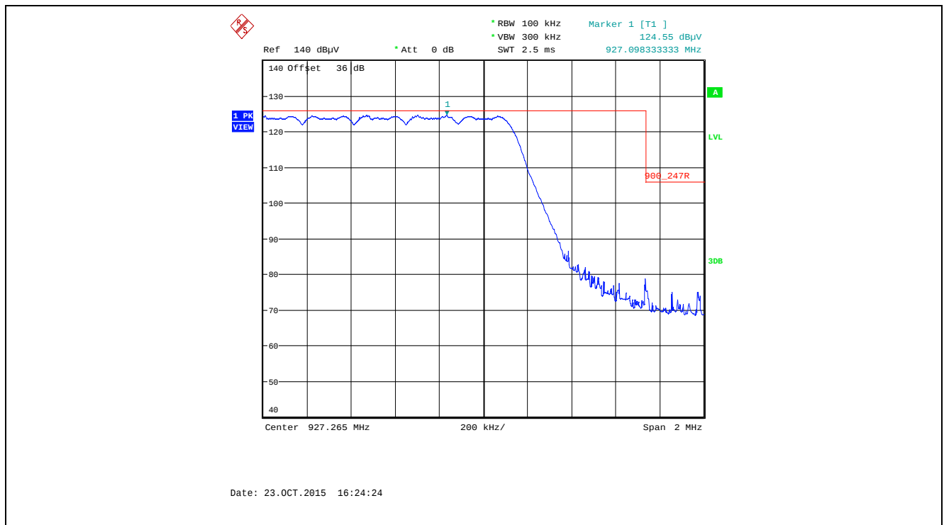
Plot 5.5.4.3.2.56. Band-Edge RF Radiated Emissions at 3 m, Vertical Polarization Pseudorandom Hopping Mode, High End of Frequency Band, 927.265 MHz, XTCA1, Data Rate at 105kbps
