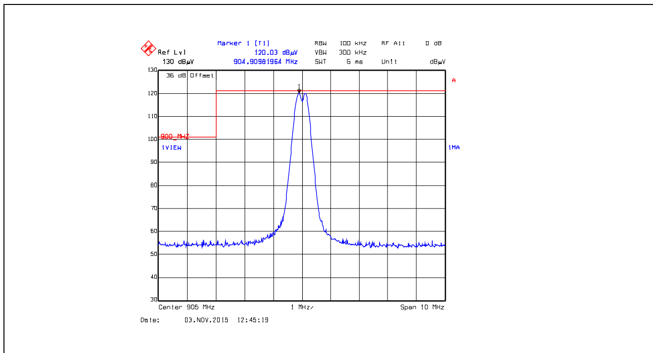
Plot 5.5.4.2.25. Band-Edge RF Radiated Emissions at 3 m, Horizontal Polarization Single Frequency Mode, Low End of Frequency Band, 905.0 MHz, XTC0, Data Rate at 10 kbps
