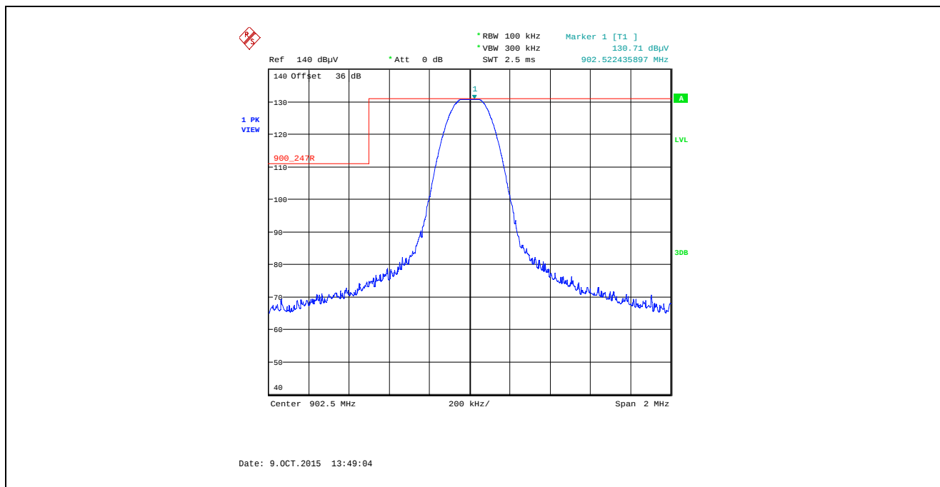
Plot 5.5.4.1.2.1. Band-Edge RF Radiated Emissions at 3 m, Horizontal Polarization Single Frequency Mode, Low End of Frequency Band, 902.5 MHz, XB0, Data Rate at 10 kbps
