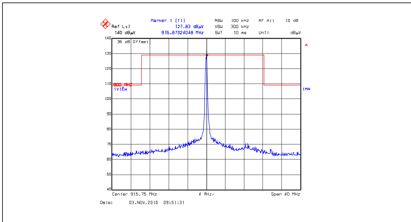
Plot 5.5.4.2.51. Band-Edge RF Radiated Emissions at 3 m, Vertical Polarization Single Frequency Mode, Low End of Frequency Band, 915.75 MHz, XTCA1, Data Rate at 105kbps
