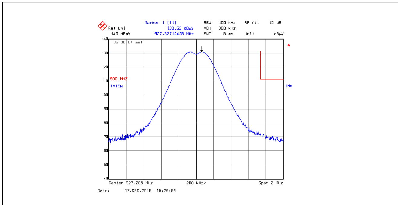
Plot 5.5.4.5.2.46. Band-Edge RF Radiated Emissions at 3 m, Horizontal Polarization Pseudorandom Hopping Mode, High End of Frequency Band, 927.265 MHz, XTCA0, Data Rate at 10 kbps
