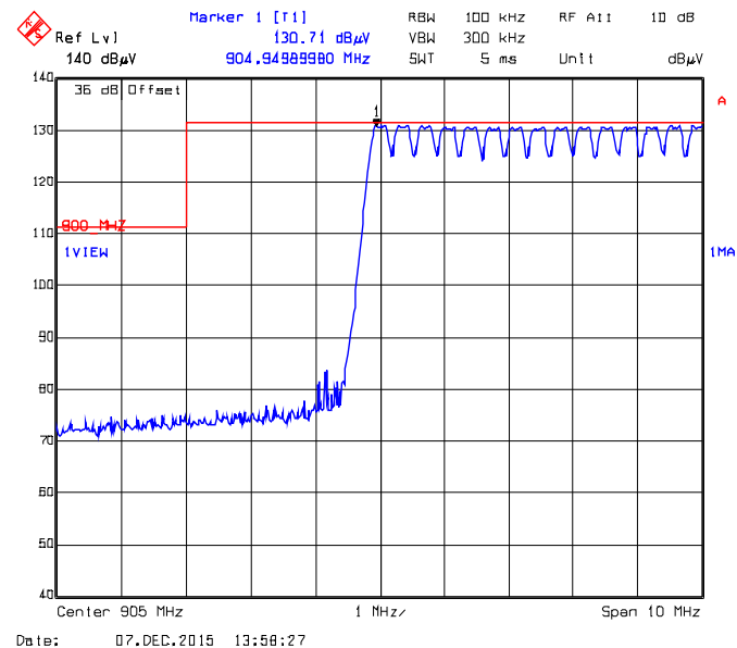
Plot 5.5.4.5.2.36. Band-Edge RF Radiated Emissions at 3 m, Vertical Polarization Pseudorandom Hopping Mode, Low End of Frequency Band, 905.0 MHz, XTC1, Data Rate at 125 kbps
