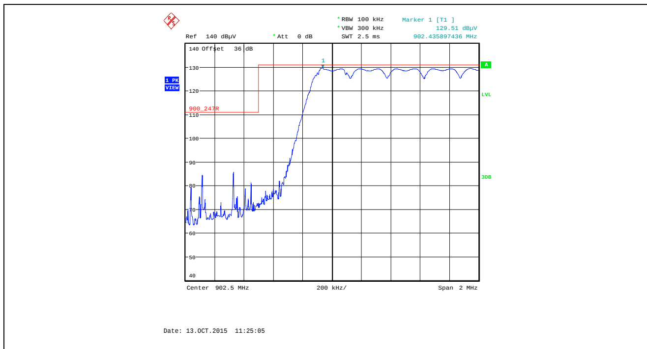
Plot 5.5.4.1.2.12. Band-Edge RF Radiated Emissions at 3 m, Vertical Polarization Pseudorandom Hopping Mode, Low End of Frequency Band, 902.5 MHz, XBX1, Data Rate at 110 kbps
