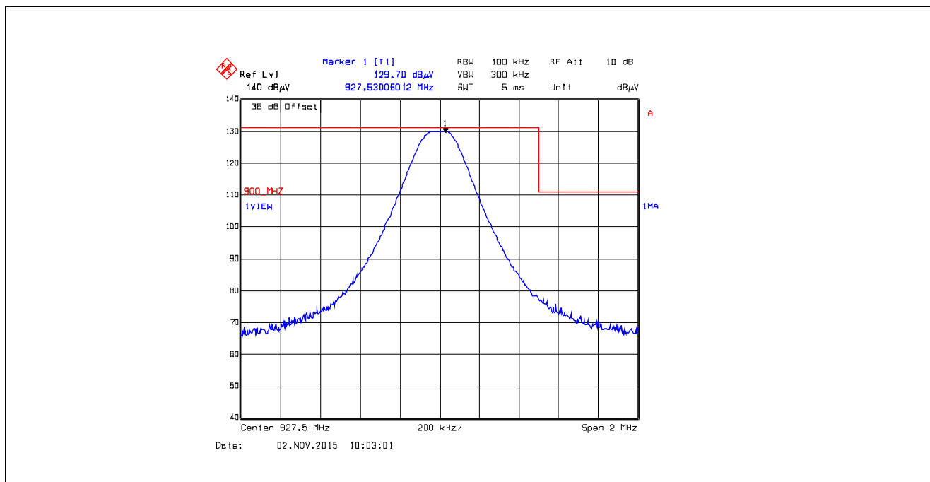
Plot 5.5.4.4.2.5. Band-Edge RF Radiated Emissions at 3 m, Horizontal Polarization Single Frequency Mode, High End of Frequency Band, 927.5 MHz, XB0, Data Rate at 10 kbps
