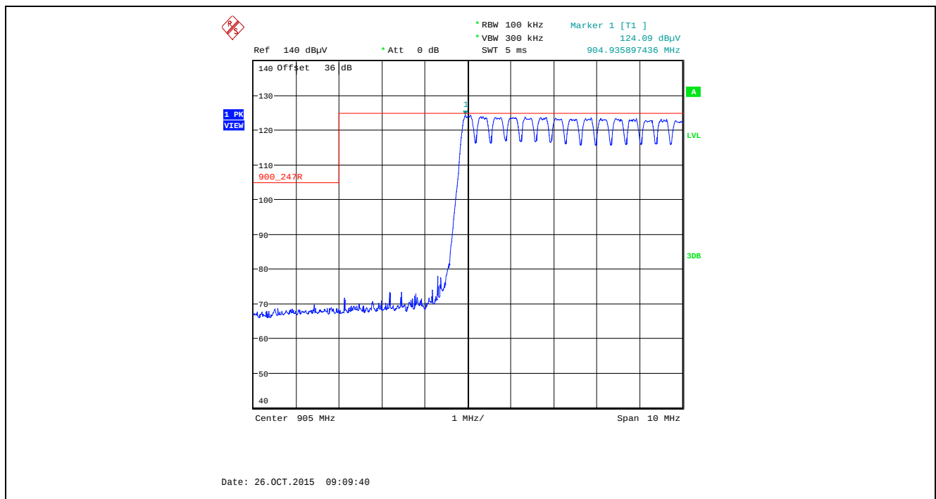
Plot 5.5.4.3.2.36. Band-Edge RF Radiated Emissions at 3 m, Vertical Polarization Pseudorandom Hopping Mode, Low End of Frequency Band, 905.0 MHz, XTC1, Data Rate at 125 kbps
