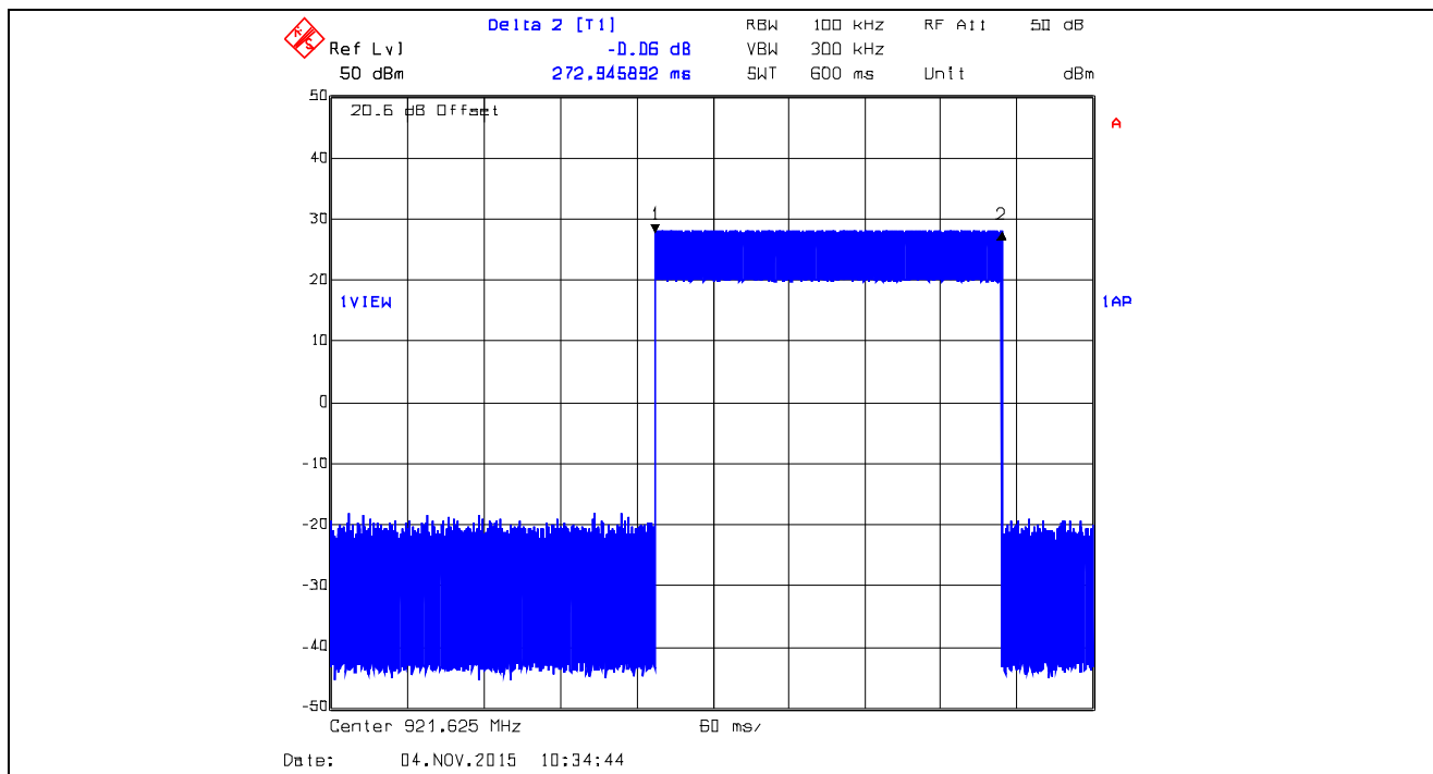
Plot 5.3.4.80. Time of Occupancy, 921.625 MHz, XTCA0, Data Rate at 10 kbps Dwell Time @ 921.625 MHz = 272.9459 ms
