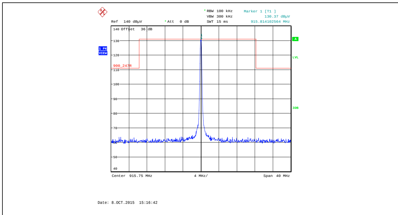
Plot 5.5.4.1.2.41. Band-Edge RF Radiated Emissions at 3 m, Horizontal Polarization Single Frequency Mode, Low End of Frequency Band, 915.75 MHz, XTCA0, Data Rate at 10 kbps
