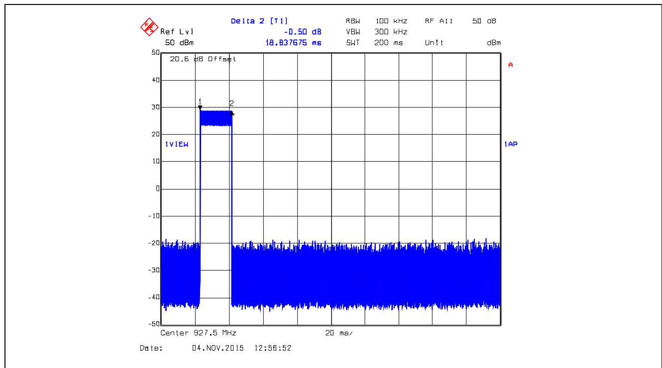
Plot 5.3.4.58. Time of Occupancy, 927.5 MHz, XBX1, Data Rate at 110 kbps
