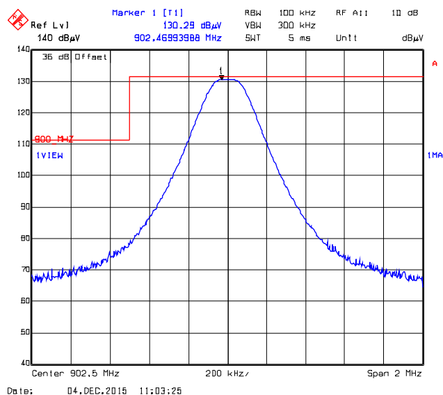
Plot 5.5.4.5.2.2. Band-Edge RF Radiated Emissions at 3 m, Horizontal Polarization Pseudorandom Hopping Mode, Low End of Frequency Band, 902.5 MHz, XB0, Data Rate at 10 kbps
