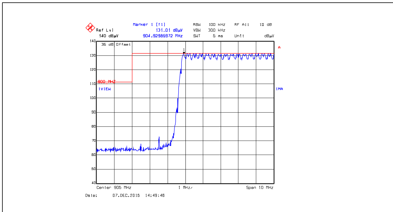
Plot 5.5.4.5.2.26. Band-Edge RF Radiated Emissions at 3 m, Horizontal Polarization Pseudorandom Hopping Mode, Low End of Frequency Band, 905.0 MHz, XTC0, Data Rate at 10 kbps
