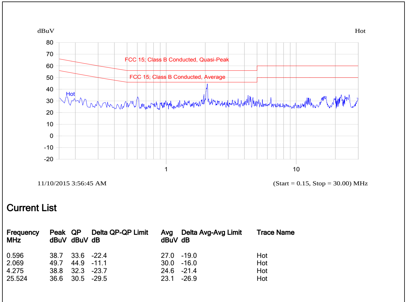
Plot 5.1.4.3. Power Line Conducted Emissions (Rx Mode) Line Voltage: 120 VAC; Line Tested: Hot
