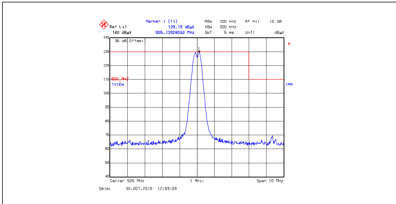
Plot 5.5.4.4.2.32. Band-Edge RF Radiated Emissions at 3 m, Vertical Polarization Pseudorandom Hopping Mode, High End of Frequency Band, 925.0 MHz, XTC0, Data Rate at 10 kbps
