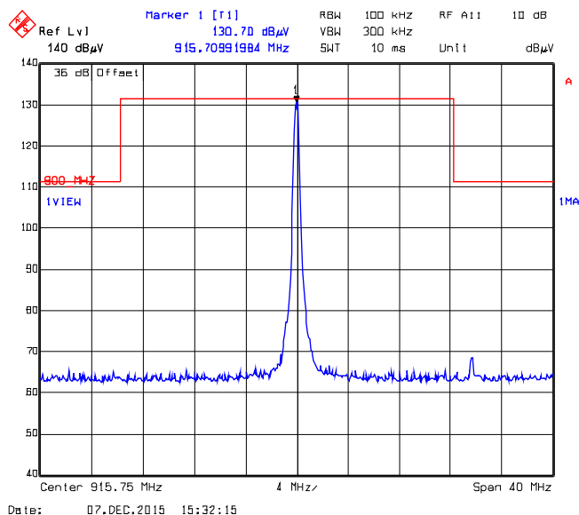
Plot 5.5.4.5.2.50. Band-Edge RF Radiated Emissions at 3 m, Horizontal Polarization Pseudorandom Hopping Mode, Low End of Frequency Band, 915.75 MHz, XTCA1, Data Rate at 105kbps
