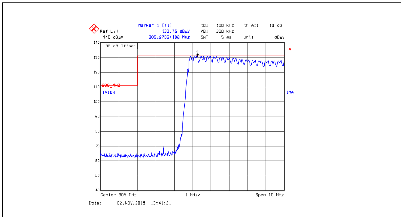
Plot 5.5.4.4.2.26. Band-Edge RF Radiated Emissions at 3 m, Horizontal Polarization Pseudorandom Hopping Mode, Low End of Frequency Band, 905.0 MHz, XTC0, Data Rate at 10 kbps
