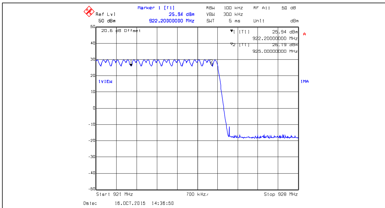
Plot 5.3.4.34. Number of Hopping Frequencies, XTC0, Data Rate at 10 kbps 9 Hopping Channels from 922 – 928 MHz
