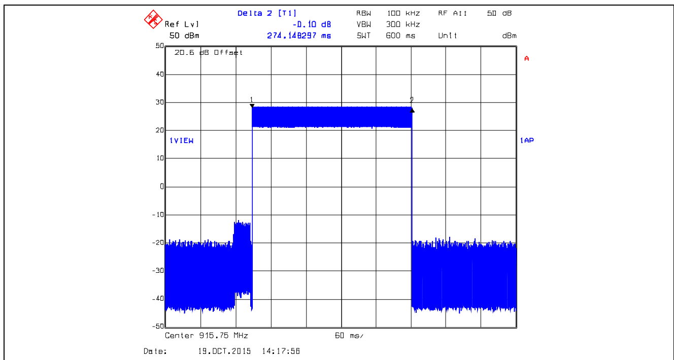
Plot 5.3.4.78. Time of Occupancy, 915.75 MHz, XTCA0, Data Rate at 10 kbps Dwell Time @ 915.75 MHz = 274.1483ms
