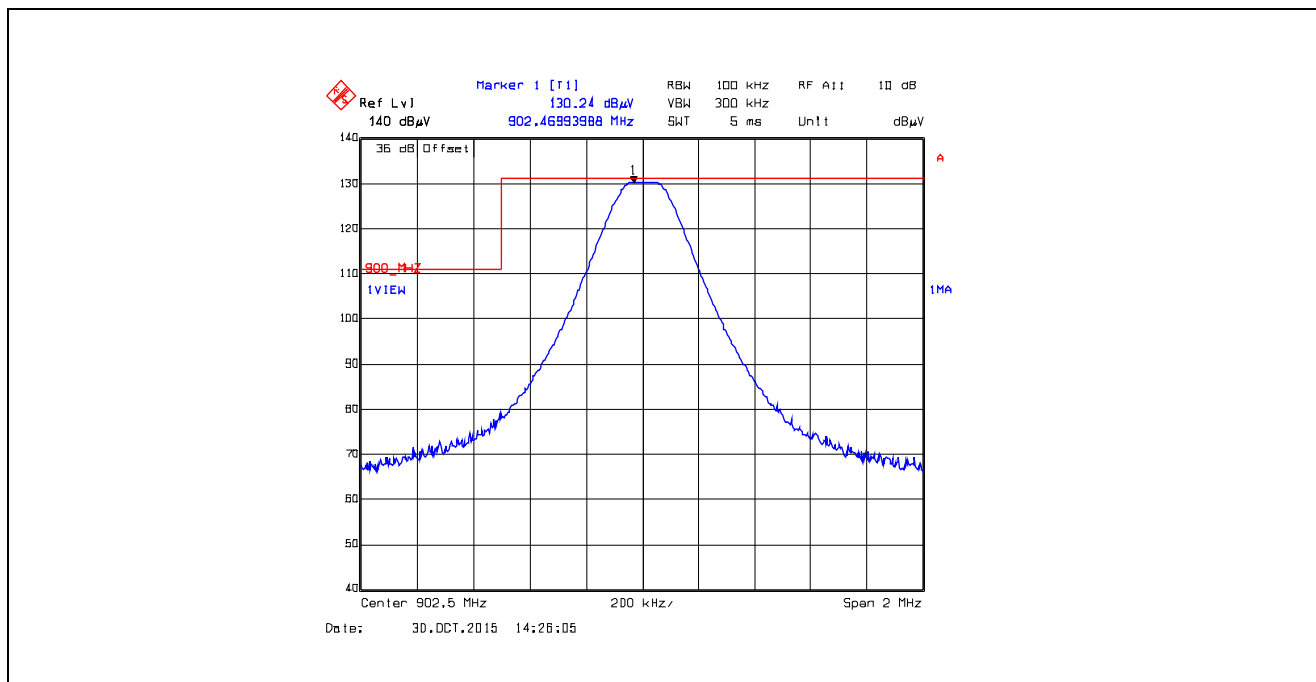
Plot 5.5.4.4.2.3. Band-Edge RF Radiated Emissions at 3 m, Vertical Polarization Single Frequency Mode, Low End of Frequency Band, 902.5 MHz, XB0, Data Rate at 10 kbps
