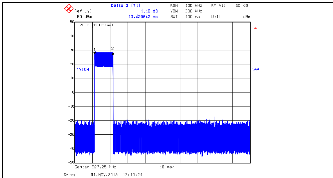
Plot 5.3.4.64. Time of Occupancy, 927.25 MHz, XB2, Data Rate at 250 kbps Dwell Time @ 927.25 MHz = 10.4208 ms
