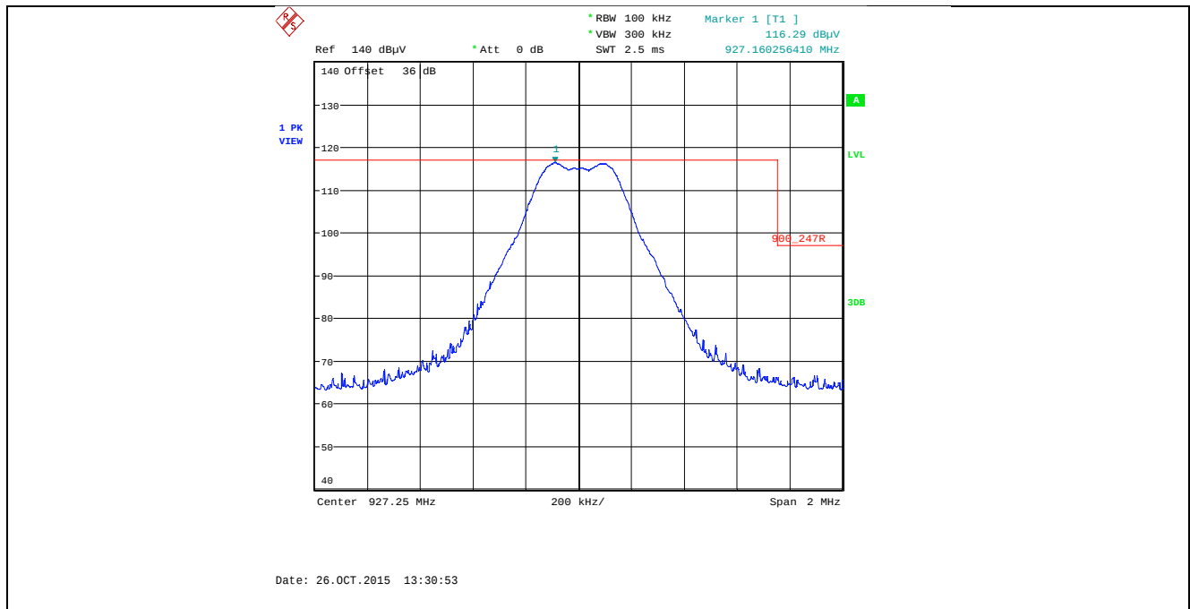
Plot 5.5.4.3.2.21. Band-Edge RF Radiated Emissions at 3 m, Horizontal Polarization Single Frequency Mode, High End of Frequency Band, 927.25 MHz, XB2, Data Rate at 250 kbps
