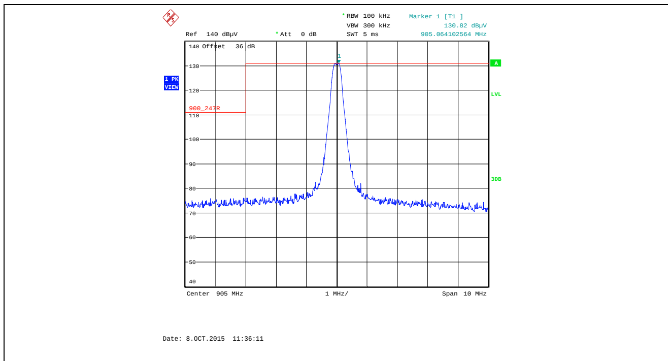
Plot 5.5.4.1.2.33. Band-Edge RF Radiated Emissions at 3 m, Horizontal Polarization Single Frequency Mode, Low End of Frequency Band, 905.0 MHz, XTC1, Data Rate at 125 kbps
