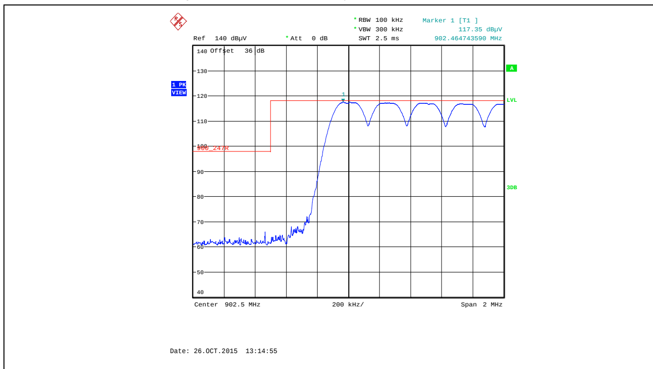
Plot 5.5.4.3.2.2. Band-Edge RF Radiated Emissions at 3 m, Horizontal Polarization Pseudorandom Hopping Mode, Low End of Frequency Band, 902.5 MHz, XB0, Data Rate at 10 kbps
