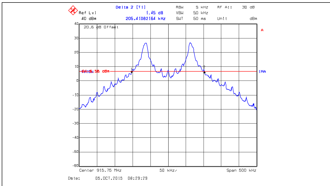
Plot 5.3.4.16. 20 dB Bandwidth, 915.75 MHz, XTCA0, Data Rate at 10 kbps
