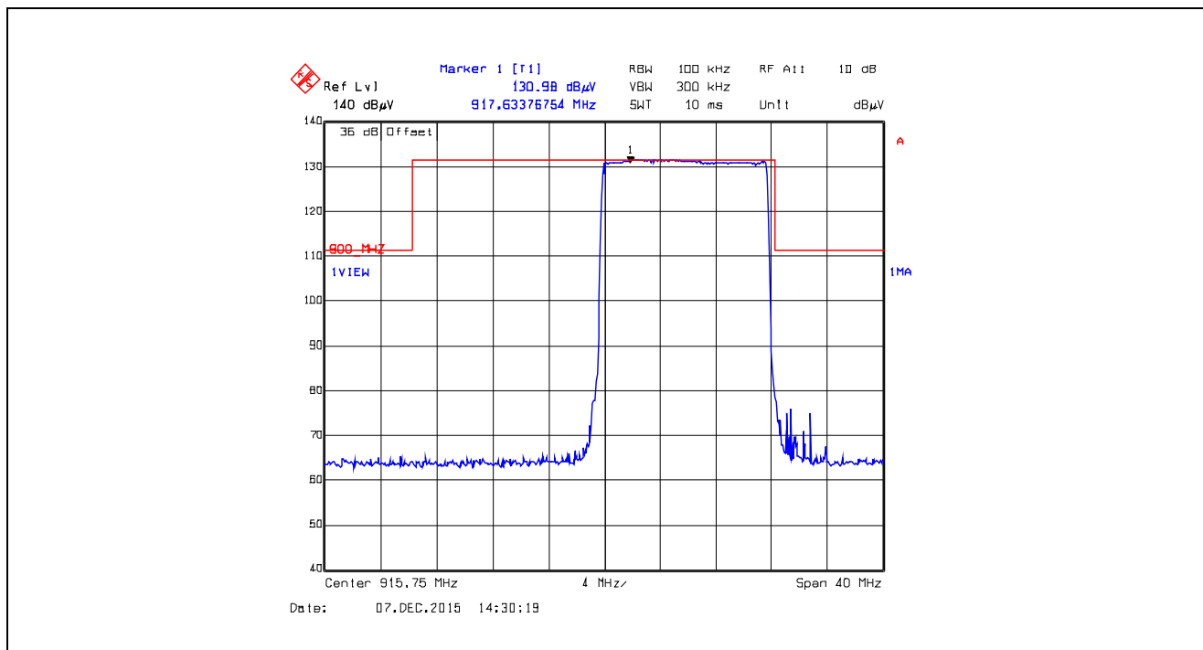
Plot 5.5.4.5.2.42. Band-Edge RF Radiated Emissions at 3 m, Horizontal Polarization Pseudorandom Hopping Mode, Low End of Frequency Band, 915.75 MHz, XTCA0, Data Rate at 10 kbps
