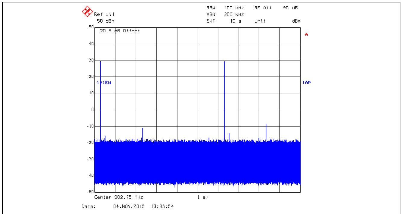
Plot 5.3.4.61. Time of Occupancy, 902.75 MHz, XB2, Data Rate at 250 kbps Average time of occupancy = (Dwell Time) x (number of hops) = 10.4208 ms x 2 = 20.8416 ms < 0.4 sec within 10 sec
