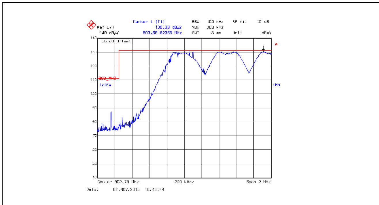
Plot 5.5.4.4.2.18. Band-Edge RF Radiated Emissions at 3 m, Horizontal Polarization Pseudorandom Hopping Mode, Low End of Frequency Band, 902.75 MHz, XBX2, Data Rate at 250 kbps
