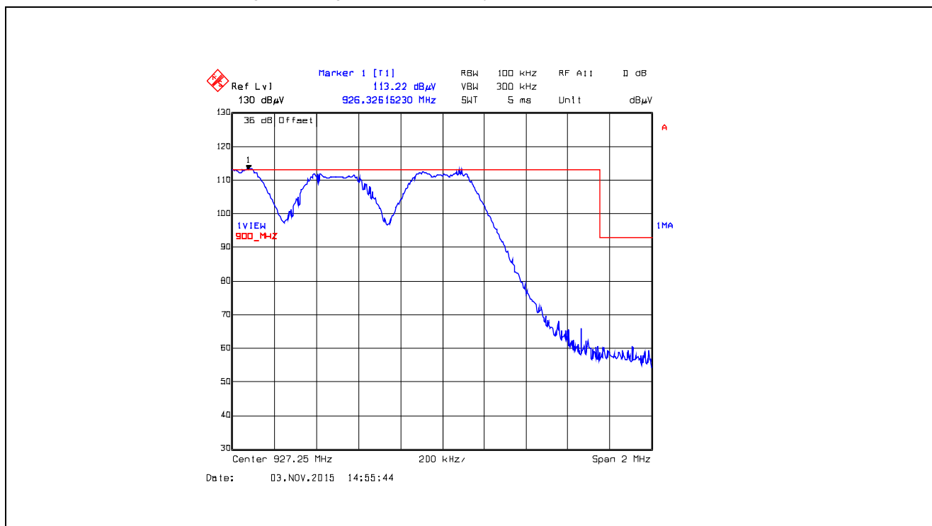
Plot 5.5.4.2.22. Band-Edge RF Radiated Emissions at 3 m, Horizontal Polarization Pseudorandom Hopping Mode, High End of Frequency Band, 927.25 MHz, XB2, Data Rate at 250 kbps
