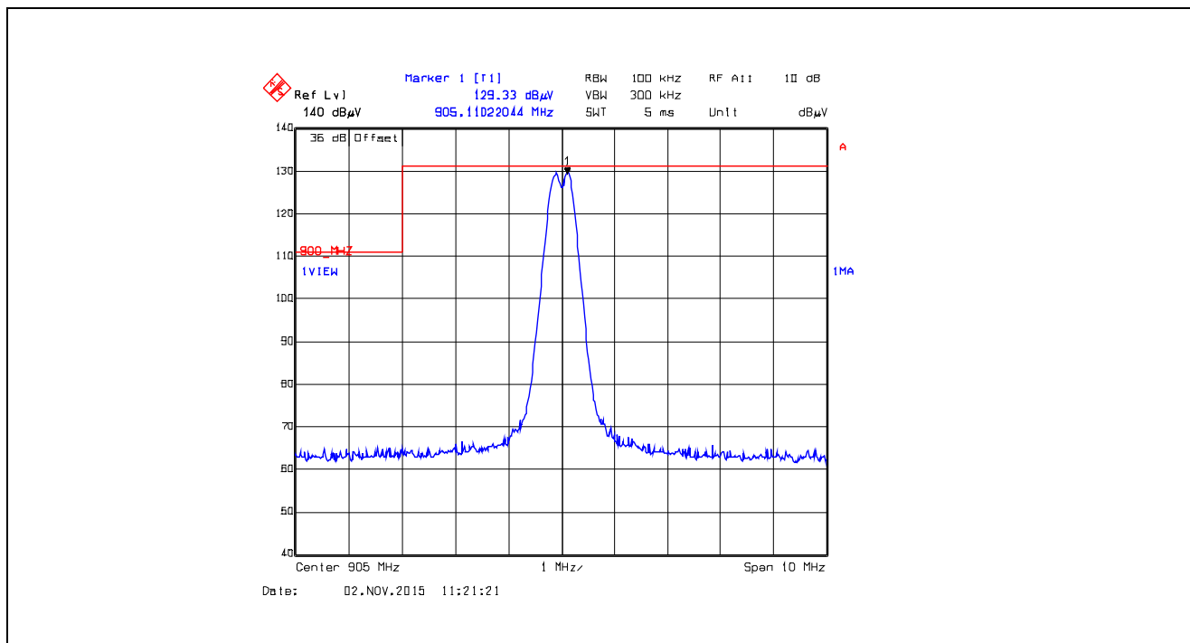
Plot 5.5.4.4.2.25. Band-Edge RF Radiated Emissions at 3 m, Horizontal Polarization Single Frequency Mode, Low End of Frequency Band, 905.0 MHz, XTC0, Data Rate at 10 kbps
