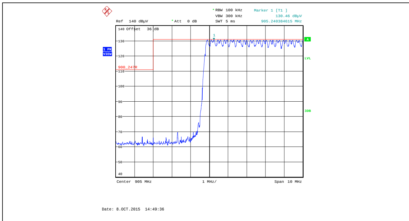
Plot 5.5.4.1.2.26. Band-Edge RF Radiated Emissions at 3 m, Horizontal Polarization Pseudorandom Hopping Mode, Low End of Frequency Band, 905.0 MHz, XTC0, Data Rate at 10 kbps
