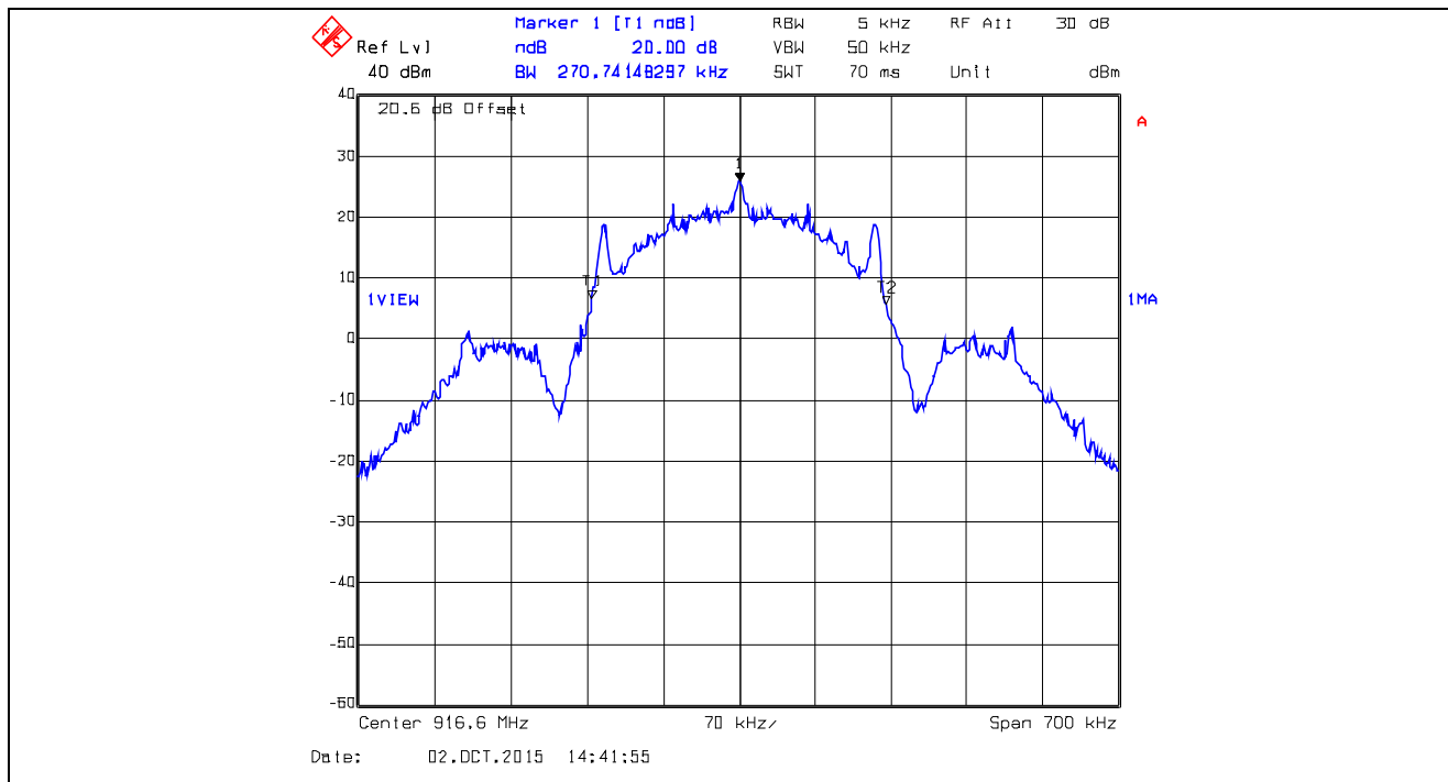
Plot 5.3.4.14. 20 dB Bandwidth, 916.6 MHz, XTC1, Data Rate at 125 kbps
