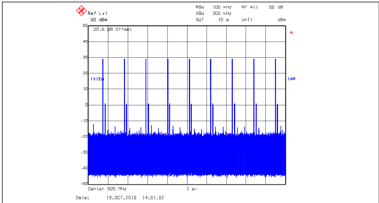
Plot 5.3.4.77. Time of Occupancy, 925.0 MHz, XTC1, Data Rate at 125 kbps Average time of occupancy = (Dwell Time) x (number of hops) = 19.2385ms x 9 = 173.15 ms < 0.4 sec within 10 sec
