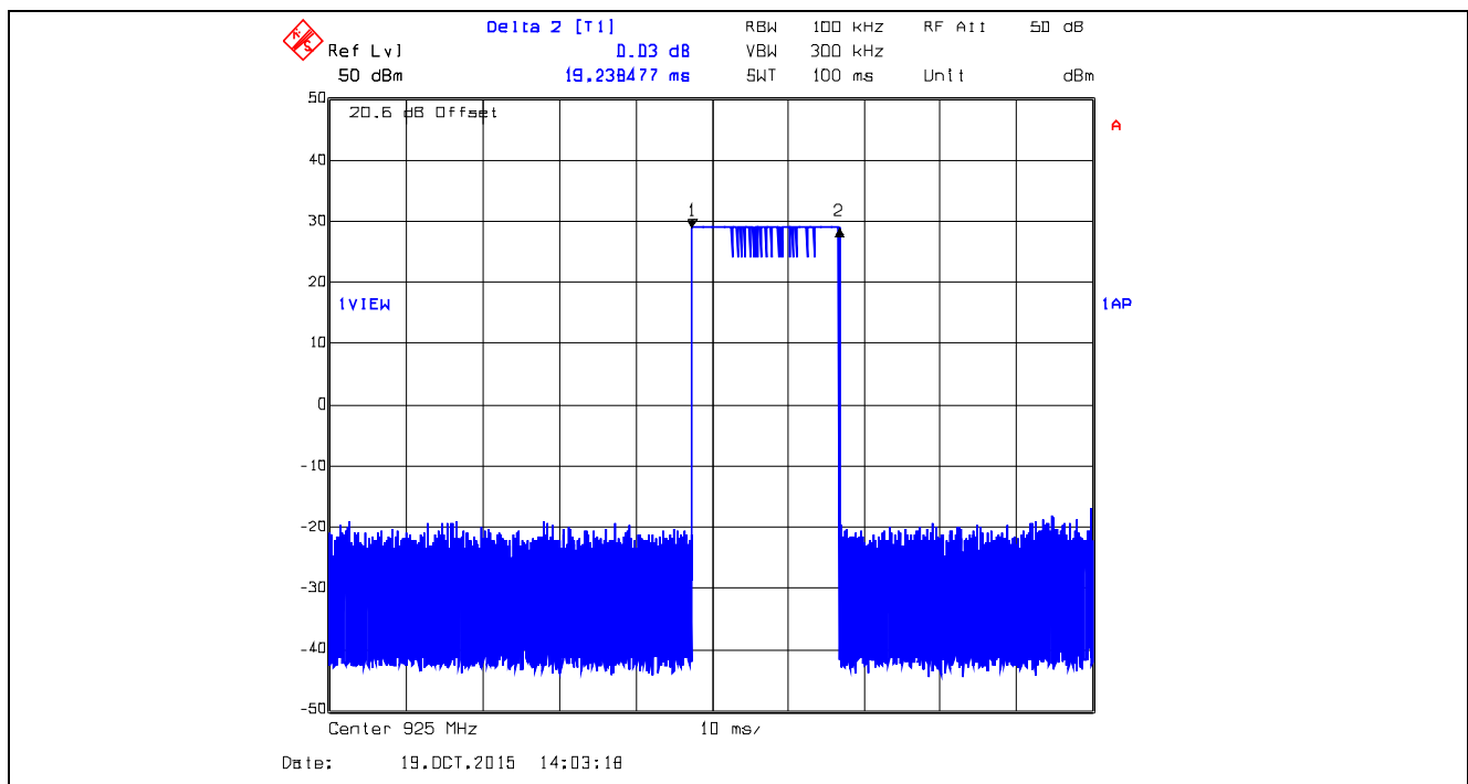
Plot 5.3.4.76. Time of Occupancy, 925.0 MHz, XTC1, Data Rate at 125 kbps Dwell Time @ 925.0 MHz = 19.2385 ms
