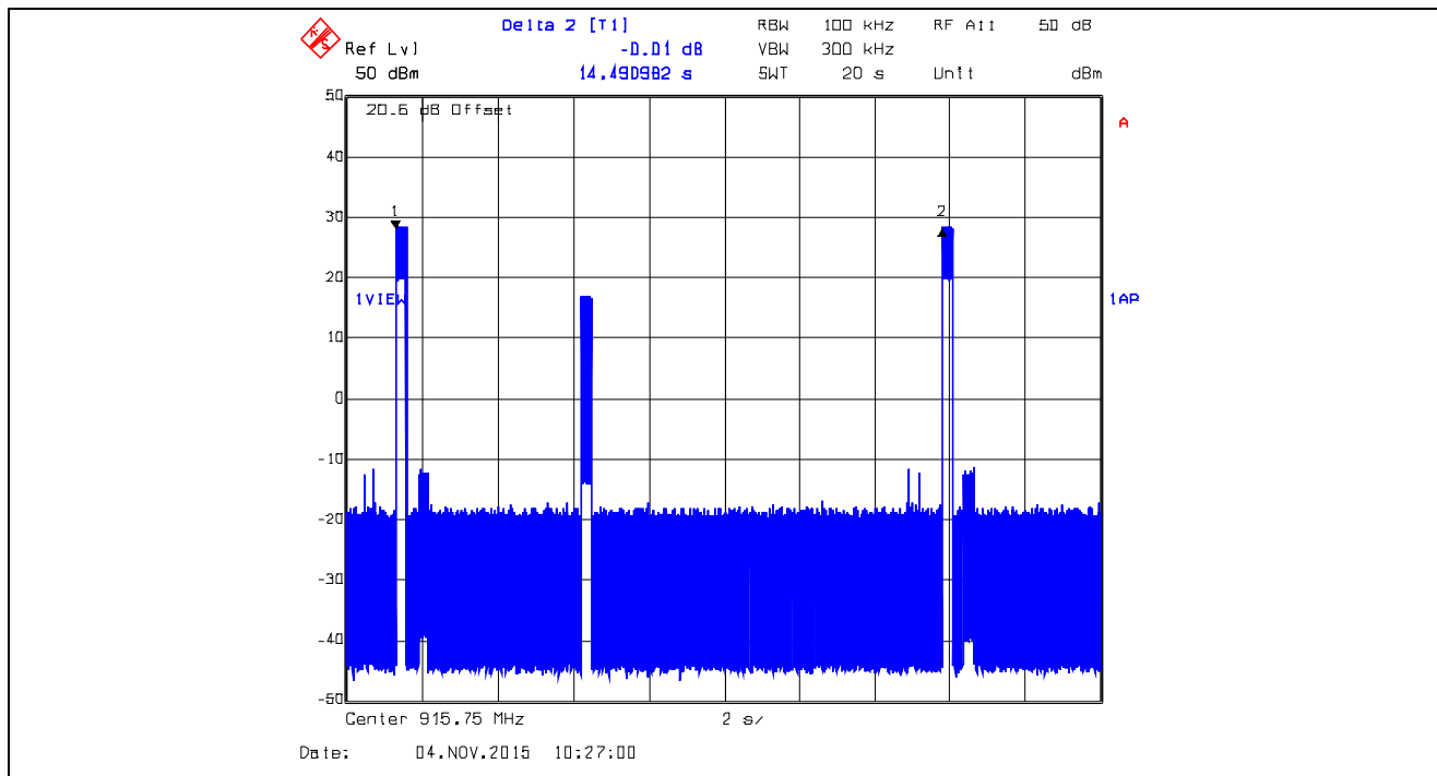
Plot 5.3.4.79. Time of Occupancy, 915.75 MHz XTCA0, Data Rate at 10 kbps Average time of occupancy = 20 \times (T_{\text{on}}) / (T_{\text{total}}) = 20 \times 0.2741483\text{s} / 14.4910\text{s} = 0.3783\text{s} < 0.4\text{s}
