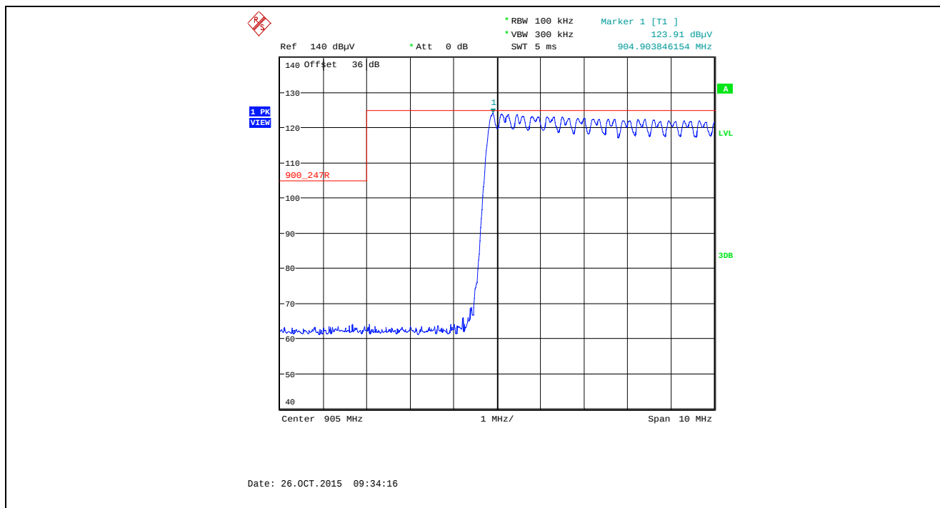
Plot 5.5.4.3.2.28. Band-Edge RF Radiated Emissions at 3 m, Vertical Polarization Pseudorandom Hopping Mode, Low End of Frequency Band, 905.0 MHz, XTC0, Data Rate at 10 kbps
