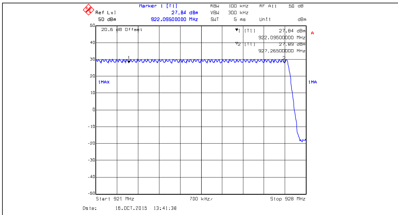
Plot 5.3.4.42. Number of Hopping Frequencies, XTCA0, Data Rate at 10 kbps 23 Hopping Channels from 922 – 928 MHz
