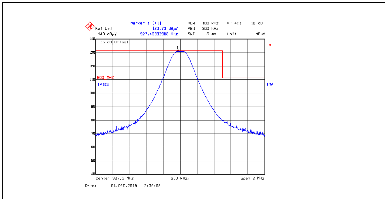
Plot 5.5.4.5.2.5. Band-Edge RF Radiated Emissions at 3 m, Horizontal Polarization Single Frequency Mode, High End of Frequency Band, 927.5 MHz, XB0, Data Rate at 10 kbps
