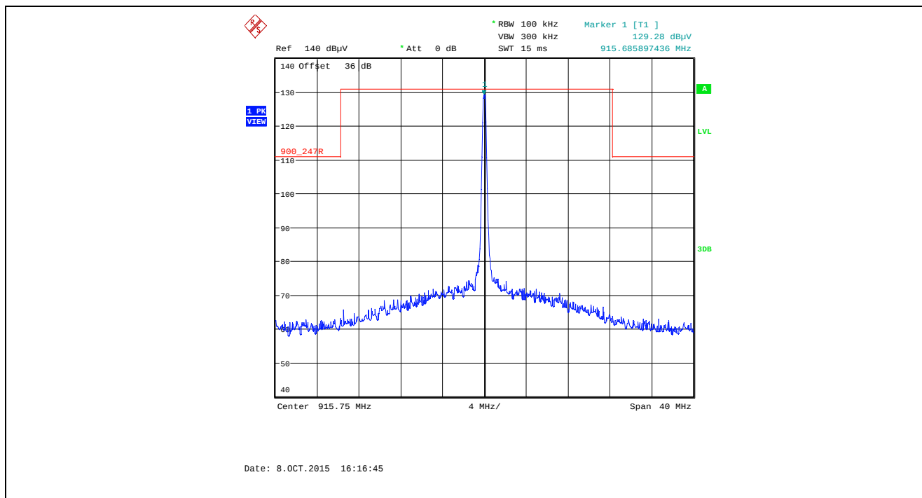
Plot 5.5.4.1.2.49. Band-Edge RF Radiated Emissions at 3 m, Horizontal Polarization Single Frequency Mode, Low End of Frequency Band, 915.75 MHz, XTCA1, Data Rate at 105kbps
