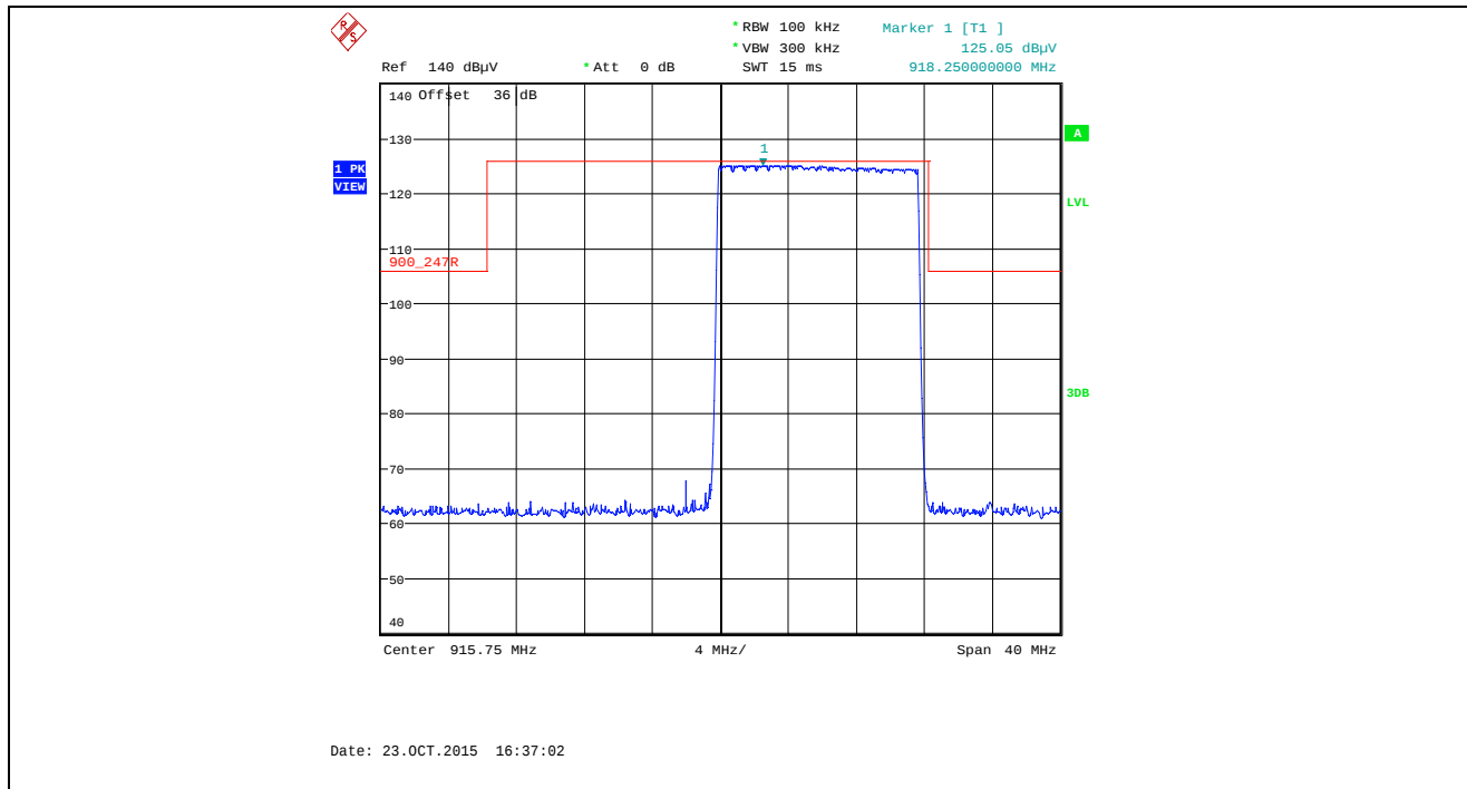
Plot 5.5.4.3.2.44. Band-Edge RF Radiated Emissions at 3 m, Vertical Polarization Pseudorandom Hopping Mode, Low End of Frequency Band, 915.75 MHz, XTCA0, Data Rate at 10 kbps
