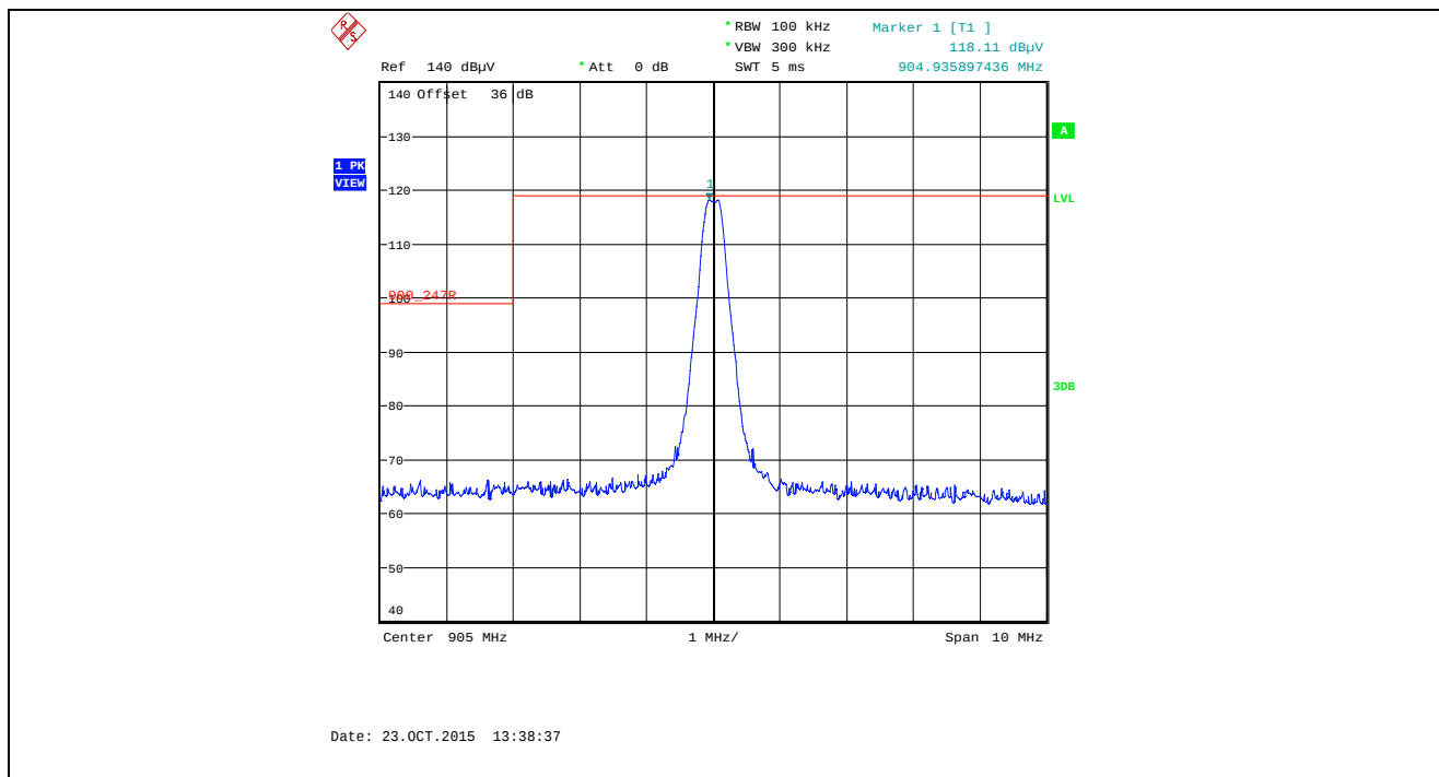
Plot 5.5.4.3.2.33. Band-Edge RF Radiated Emissions at 3 m, Horizontal Polarization Single Frequency Mode, Low End of Frequency Band, 905.0 MHz, XTC1, Data Rate at 125 kbps
