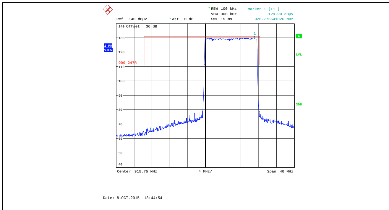
Plot 5.5.4.1.2.50. Band-Edge RF Radiated Emissions at 3 m, Horizontal Polarization Pseudorandom Hopping Mode, Low End of Frequency Band, 915.75 MHz, XTCA1, Data Rate at 105kbps
