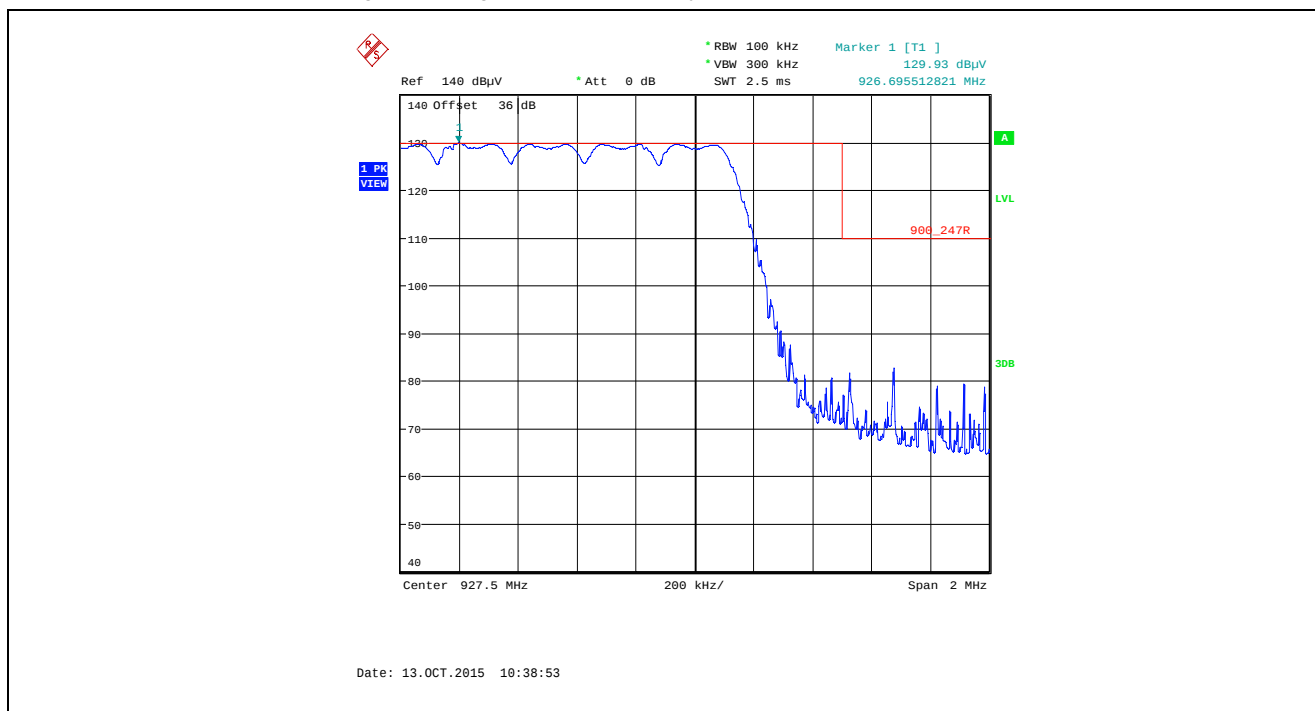
Plot 5.5.4.1.2.14. Band-Edge RF Radiated Emissions at 3 m, Horizontal Polarization Pseudorandom Hopping Mode, High End of Frequency Band, 927.5 MHz, XBX1, Data Rate at 110 kbps
