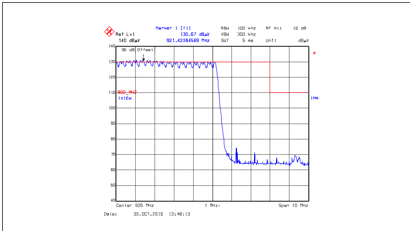
Plot 5.5.4.4.2.32. Band-Edge RF Radiated Emissions at 3 m, Vertical Polarization Pseudorandom Hopping Mode, High End of Frequency Band, 925.0 MHz, XTC0, Data Rate at 10 kbps
