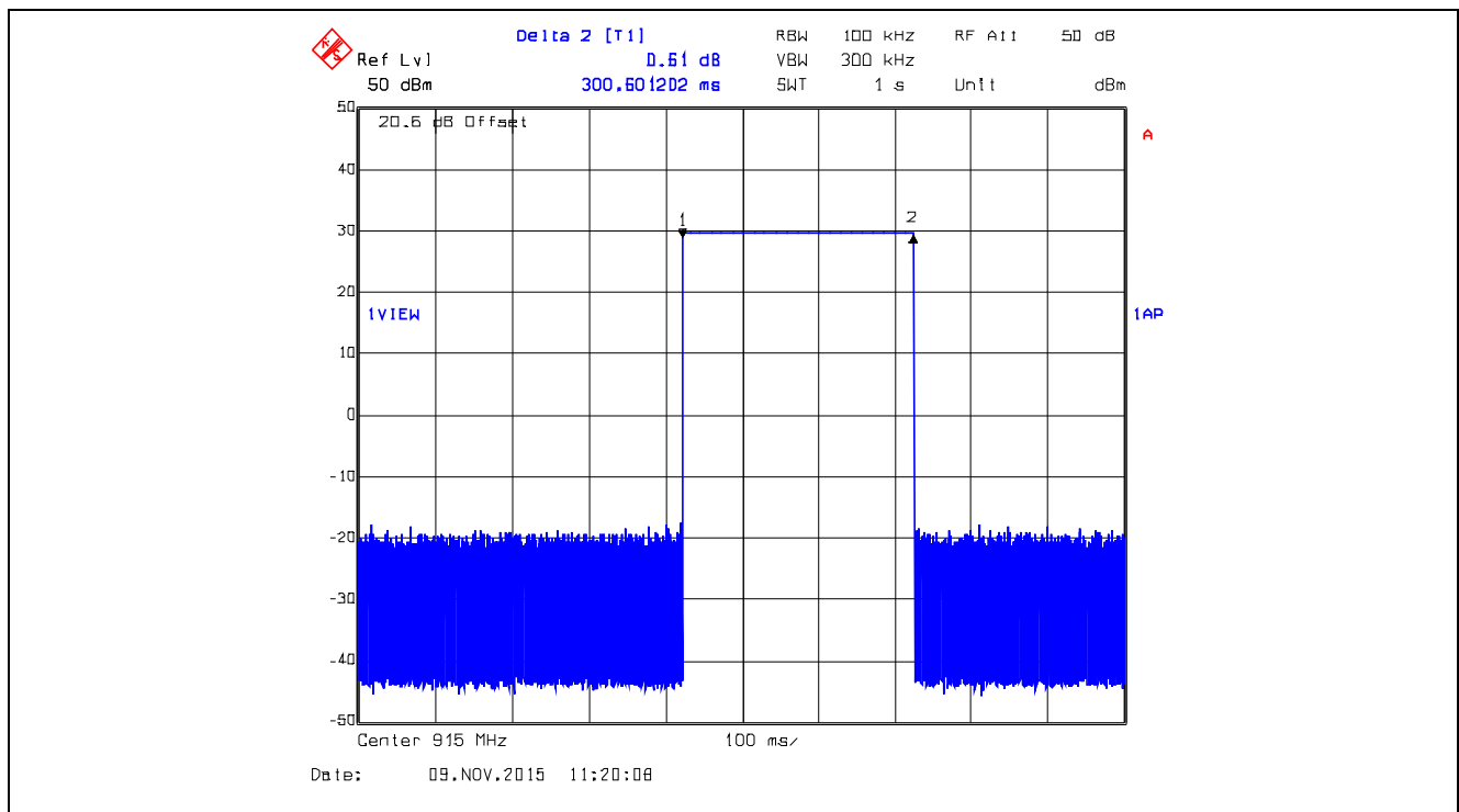
Plot 5.3.4.50. Time of Occupancy, 915 MHz, XB0, Data Rate at 10 kbps Dwell Time @ 915 MHz = 300.6012 ms
