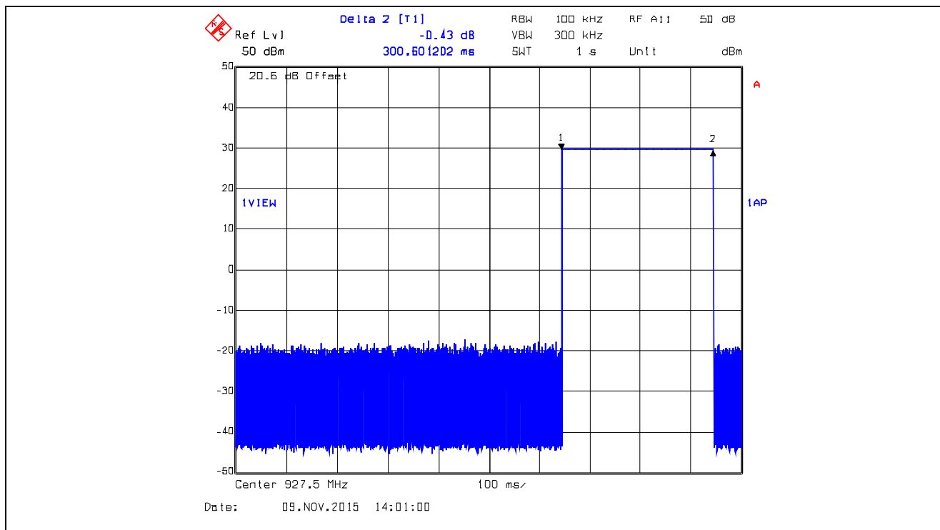
Plot 5.3.4.52. Time of Occupancy, 927.5 MHz, XBX0, Data Rate at 10 kbps Dwell Time @ 927.5 MHz = 300.6012 ms
