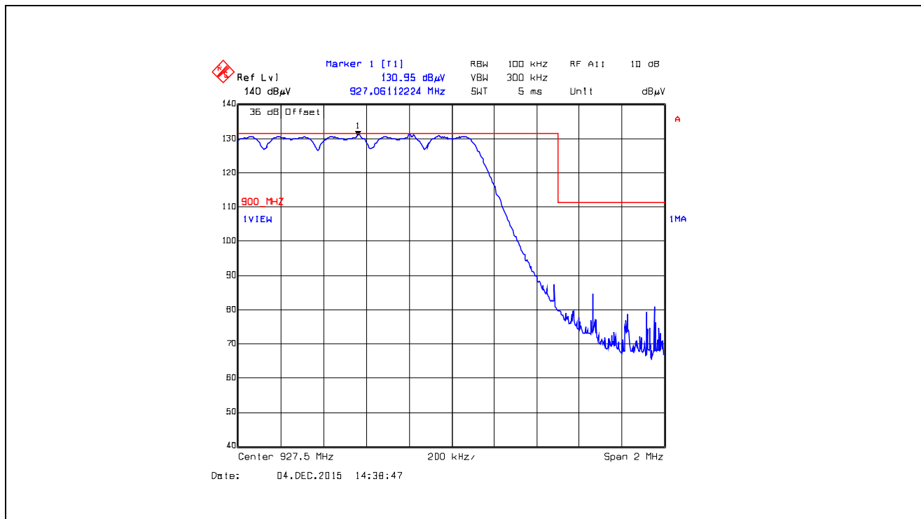
Plot 5.5.4.5.2.14. Band-Edge RF Radiated Emissions at 3 m, Horizontal Polarization Pseudorandom Hopping Mode, High End of Frequency Band, 927.5 MHz, XBX1, Data Rate at 110 kbps
