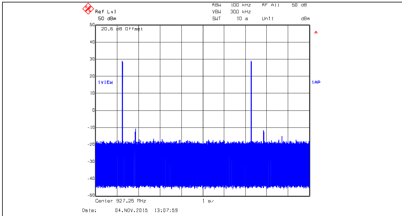
Plot 5.3.4.65. Time of Occupancy, 927.25 MHz, XB2, Data Rate at 250 kbps Average time of occupancy = (Dwell Time) x (number of hops) = 10.4208 ms x 2 = 20.8416 ms < 0.4 sec within 10 sec
