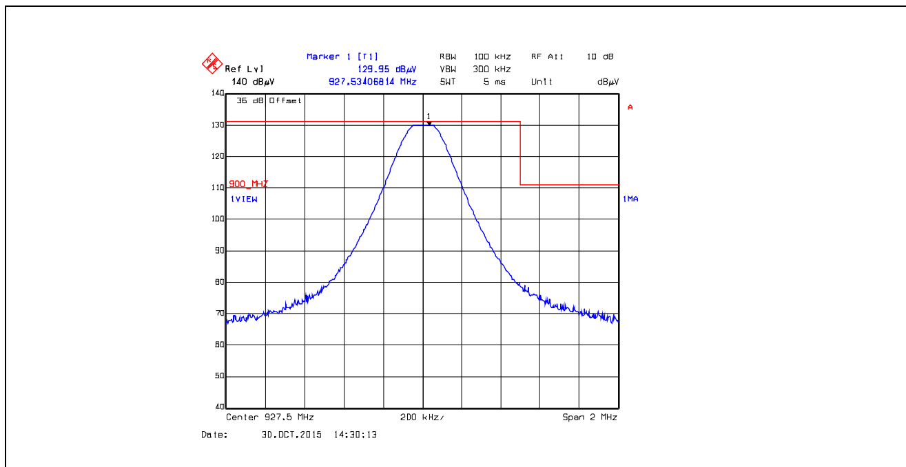
Plot 5.5.4.4.2.7. Band-Edge RF Radiated Emissions at 3 m, Vertical Polarization Single Frequency Mode, High End of Frequency Band, 927.5 MHz, XB0, Data Rate at 10 kbps
