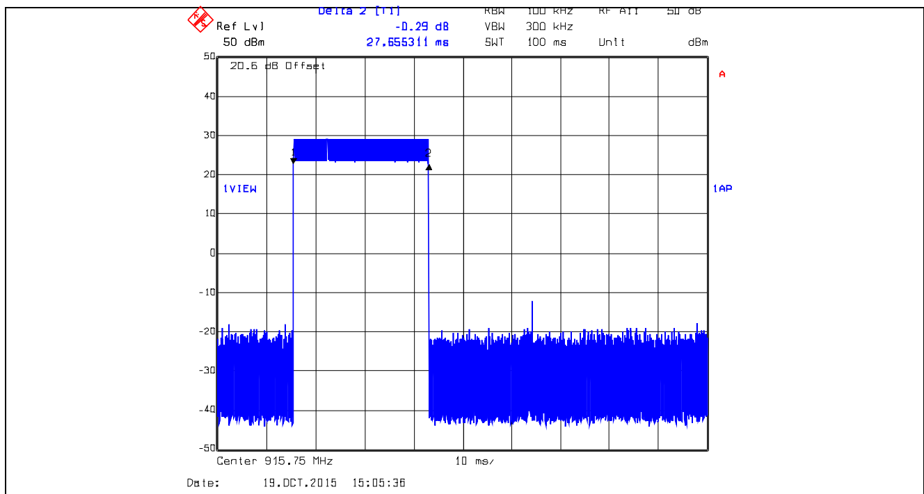
Plot 5.3.4.84. Time of Occupancy, 915.75 MHz XTCA1, Data Rate at 105 kbps Dwell Time @ 915.75 MHz = 27.655311 ms
