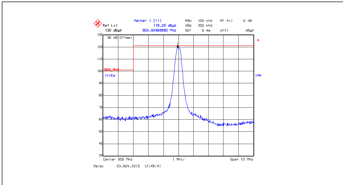
Plot 5.5.4.2.2.33. Band-Edge RF Radiated Emissions at 3 m, Horizontal Polarization Single Frequency Mode, Low End of Frequency Band, 905.0 MHz, XTC1, Data Rate at 125 kbps
