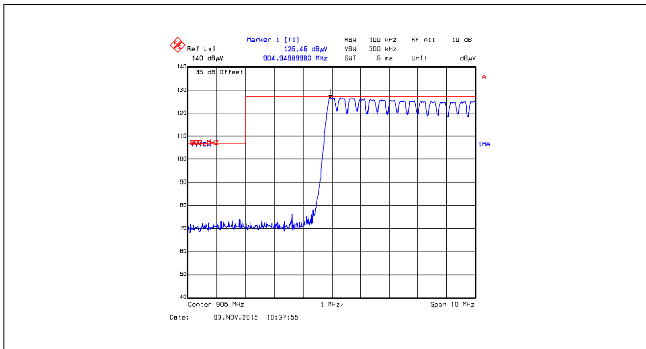
Plot 5.5.4.2.36. Band-Edge RF Radiated Emissions at 3 m, Vertical Polarization Pseudorandom Hopping Mode, Low End of Frequency Band, 905.0 MHz, XTC1, Data Rate at 125 kbps
