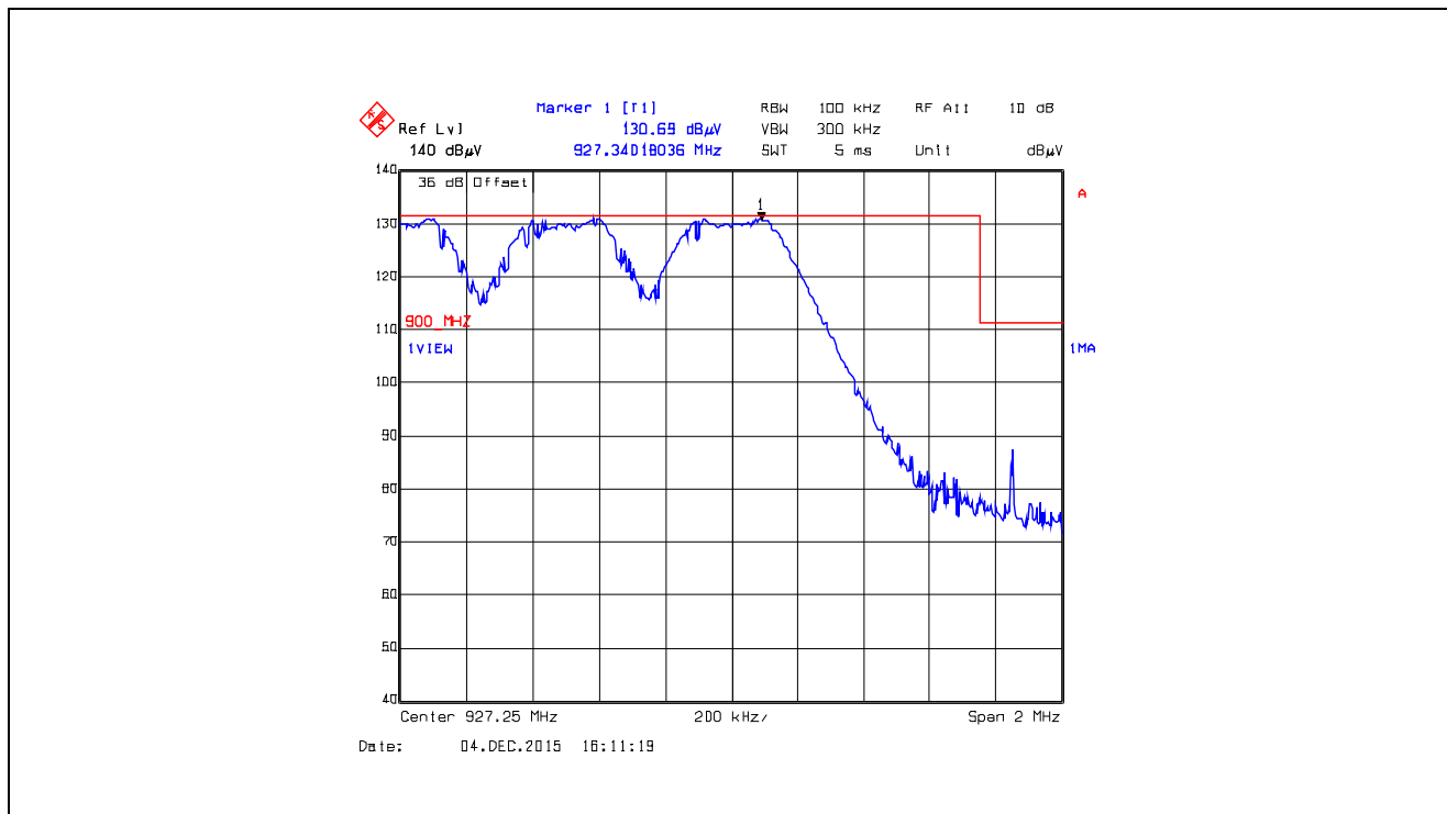
Plot 5.5.4.5.2.24. Band-Edge RF Radiated Emissions at 3 m, Vertical Polarization Pseudorandom Hopping Mode, High End of Frequency Band, 927.25 MHz, XB2, Data Rate at 250 kbps
