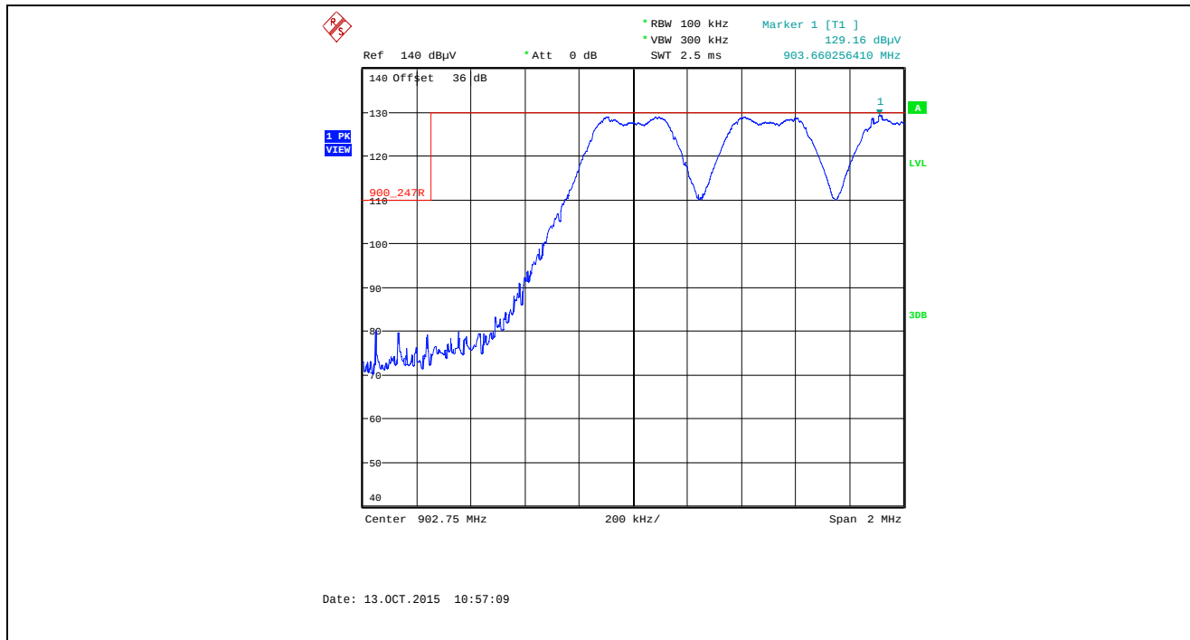
Plot 5.5.4.1.2.18. Band-Edge RF Radiated Emissions at 3 m, Horizontal Polarization Pseudorandom Hopping Mode, Low End of Frequency Band, 902.75 MHz, XBX2, Data Rate at 250 kbps
