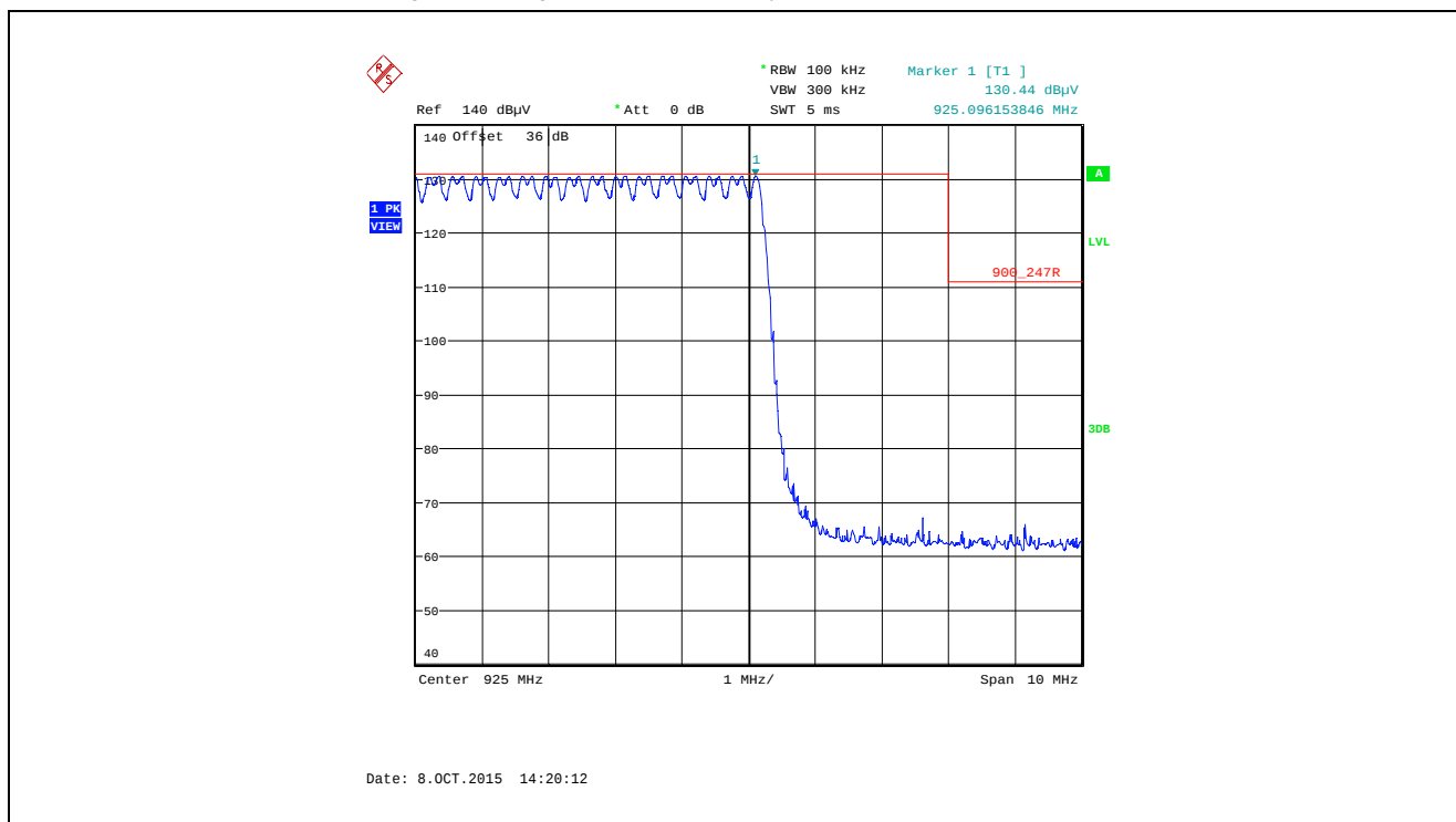
Plot 5.5.4.1.2.32. Band-Edge RF Radiated Emissions at 3 m, Vertical Polarization Pseudorandom Hopping Mode, High End of Frequency Band, 925.0 MHz, XTC0, Data Rate at 10 kbps
