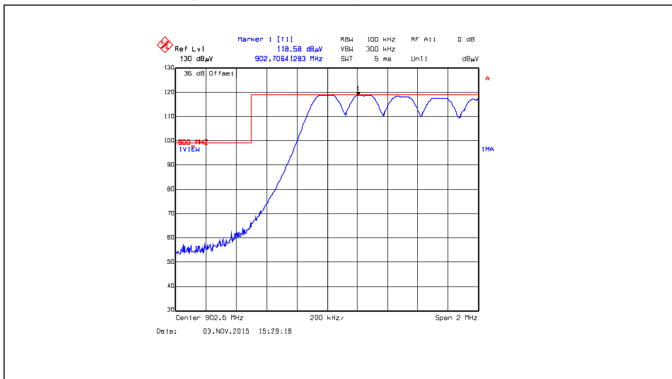
Plot 5.5.4.2.2.2. Band-Edge RF Radiated Emissions at 3 m, Horizontal Polarization Pseudorandom Hopping Mode, Low End of Frequency Band, 902.5 MHz, XB0, Data Rate at 10 kbps
