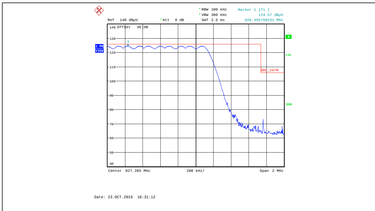
Plot 5.5.4.3.2.48. Band-Edge RF Radiated Emissions at 3 m, Vertical Polarization Pseudorandom Hopping Mode, High End of Frequency Band, 927.265 MHz, XTCA0, Data Rate at 10 kbps
