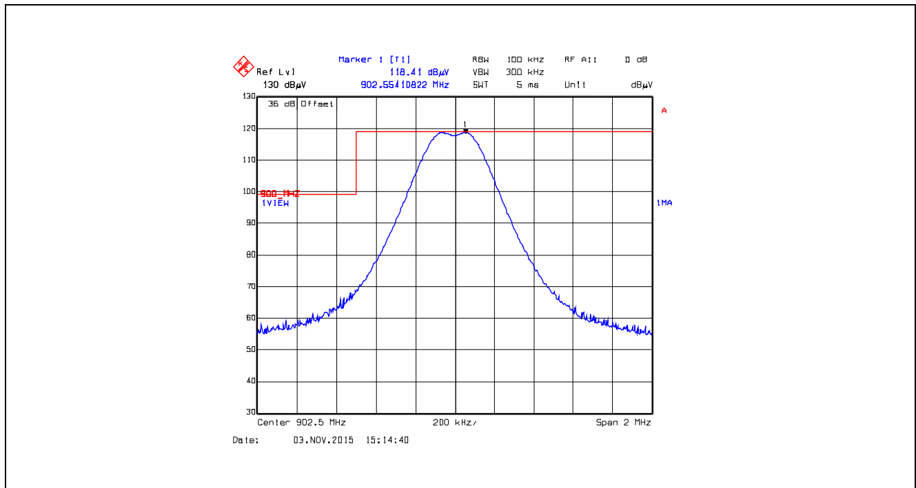
Plot 5.5.4.2.9. Band-Edge RF Radiated Emissions at 3 m, Horizontal Polarization Single Frequency Mode, Low End of Frequency Band, 902.5 MHz, XBX1, Data Rate at 110 kbps
