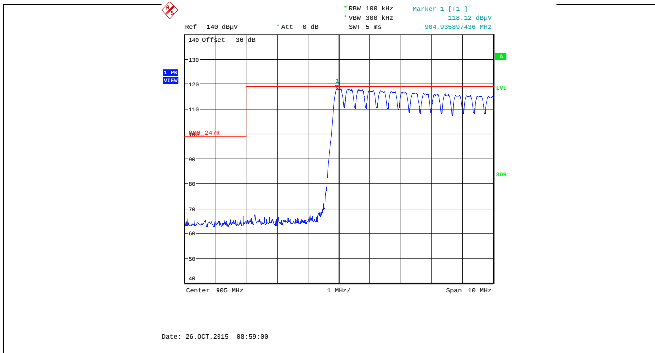
Plot 5.5.4.3.2.34. Band-Edge RF Radiated Emissions at 3 m, Horizontal Polarization Pseudorandom Hopping Mode, Low End of Frequency Band, 905.0 MHz, XTC1, Data Rate at 125 kbps
