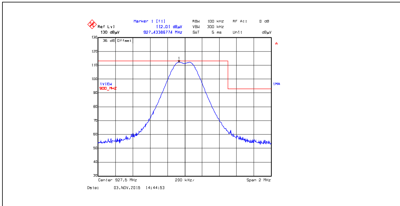
Plot 5.5.4.2.2.14. Band-Edge RF Radiated Emissions at 3 m, Horizontal Polarization Pseudorandom Hopping Mode, High End of Frequency Band, 927.5 MHz, XBX1, Data Rate at 110 kbps
