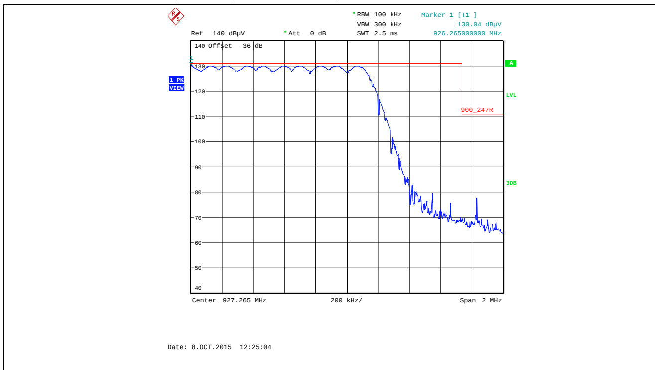
Plot 5.5.4.1.2.46. Band-Edge RF Radiated Emissions at 3 m, Horizontal Polarization Pseudorandom Hopping Mode, High End of Frequency Band, 927.265 MHz, XTCA0, Data Rate at 10 kbps
