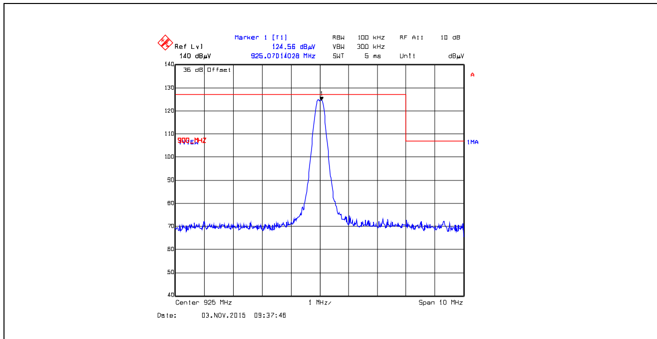
Plot 5.5.4.2.40. Band-Edge RF Radiated Emissions at 3 m, Vertical Polarization Pseudorandom Hopping Mode, High End of Frequency Band, 925.0 MHz, XTC1, Data Rate at 125 kbps
