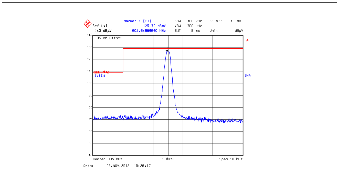
Plot 5.5.4.2.35. Band-Edge RF Radiated Emissions at 3 m, Vertical Polarization Single Frequency Mode, Low End of Frequency Band, 905.0 MHz, XTC1, Data Rate at 125 kbps
