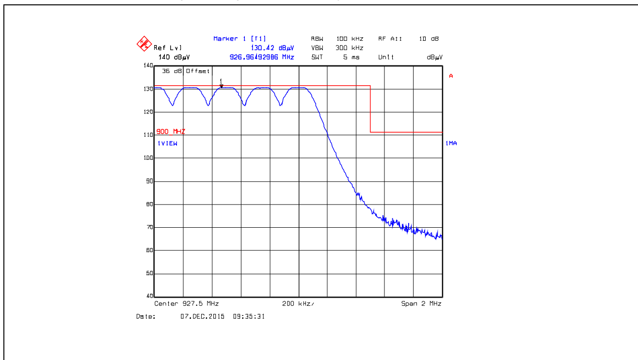
Plot 5.5.4.5.2.8. Band-Edge RF Radiated Emissions at 3 m, Vertical Polarization Pseudorandom Hopping Mode, High End of Frequency Band, 927.5 MHz, XB0, Data Rate at 10 kbps
