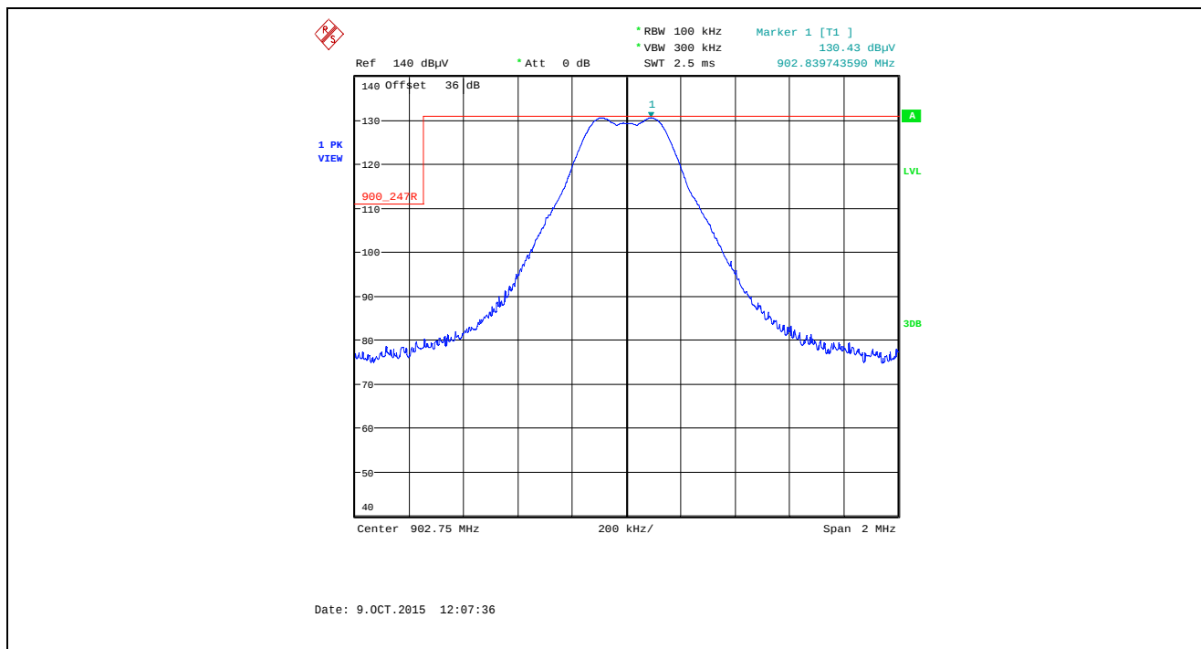
Plot 5.5.4.1.2.17. Band-Edge RF Radiated Emissions at 3 m, Horizontal Polarization Single Frequency Mode, Low End of Frequency Band, 902.75 MHz, XBX2, Data Rate at 250 kbps
