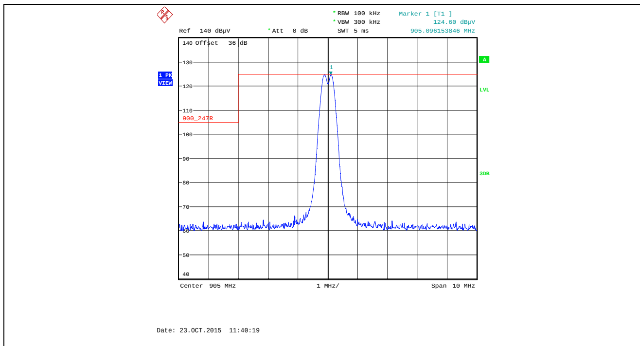
Plot 5.5.4.3.2.27. Band-Edge RF Radiated Emissions at 3 m, Vertical Polarization Single Frequency Mode, Low End of Frequency Band, 905.0 MHz, XTC0, Data Rate at 10 kbps
