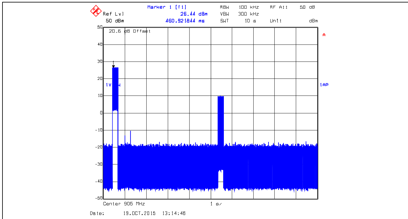
Plot 5.3.4.67. Time of Occupancy, 905 MHz, XTC0, Data Rate at 10 kbps Average time of occupancy = (Dwell Time) x (number of hops) = 272.75 ms x 1 = 272.75 ms < 0.4 sec within 10 sec
