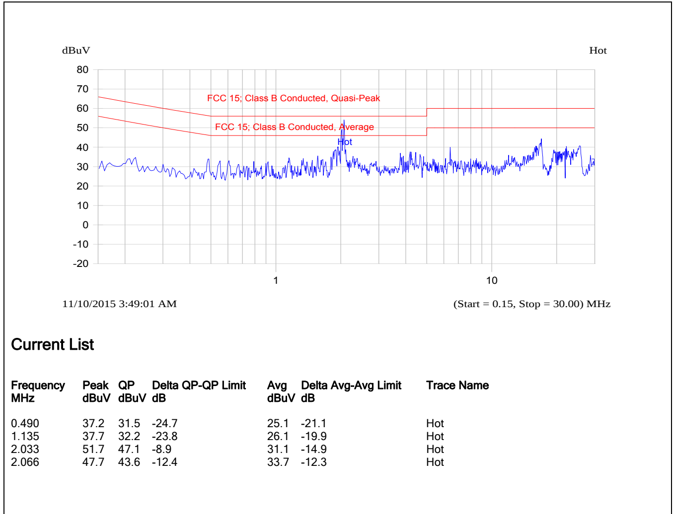
Plot 5.1.4.1. Power Line Conducted Emissions (Tx Mode) Line Voltage: 120 VAC; Line Tested: Hot
