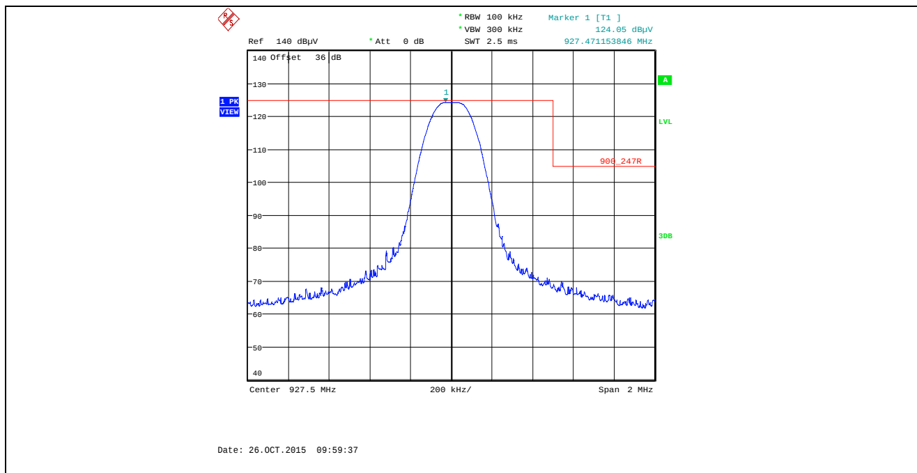
Plot 5.5.4.3.2.7. Band-Edge RF Radiated Emissions at 3 m, Vertical Polarization Single Frequency Mode, High End of Frequency Band, 927.5 MHz, XB0, Data Rate at 10 kbps
