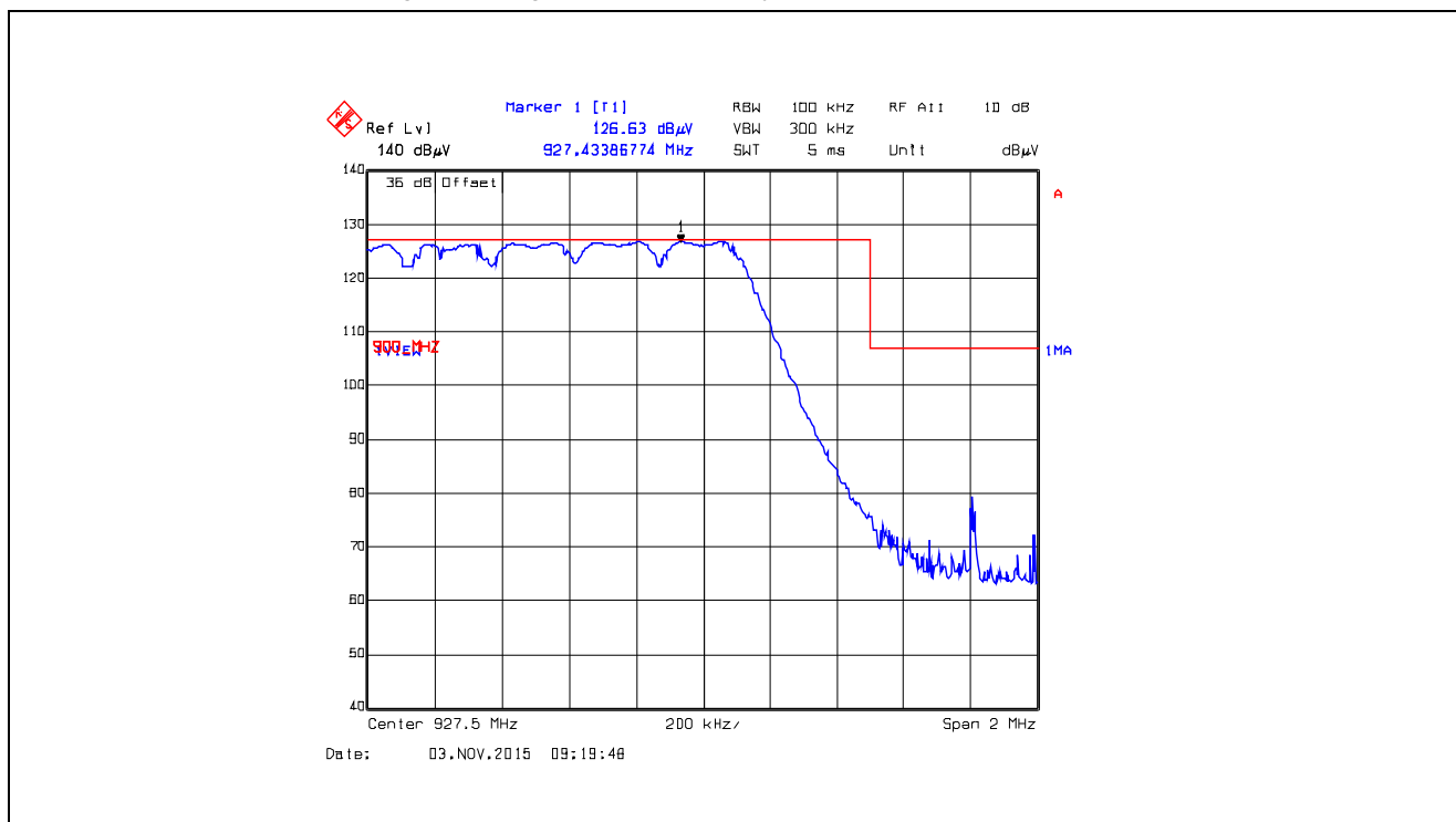
Plot 5.5.4.2.16. Band-Edge RF Radiated Emissions at 3 m, Vertical Polarization Pseudorandom Hopping Mode, High End of Frequency Band, 927.5 MHz, XBX1, Data Rate at 110 kbps
