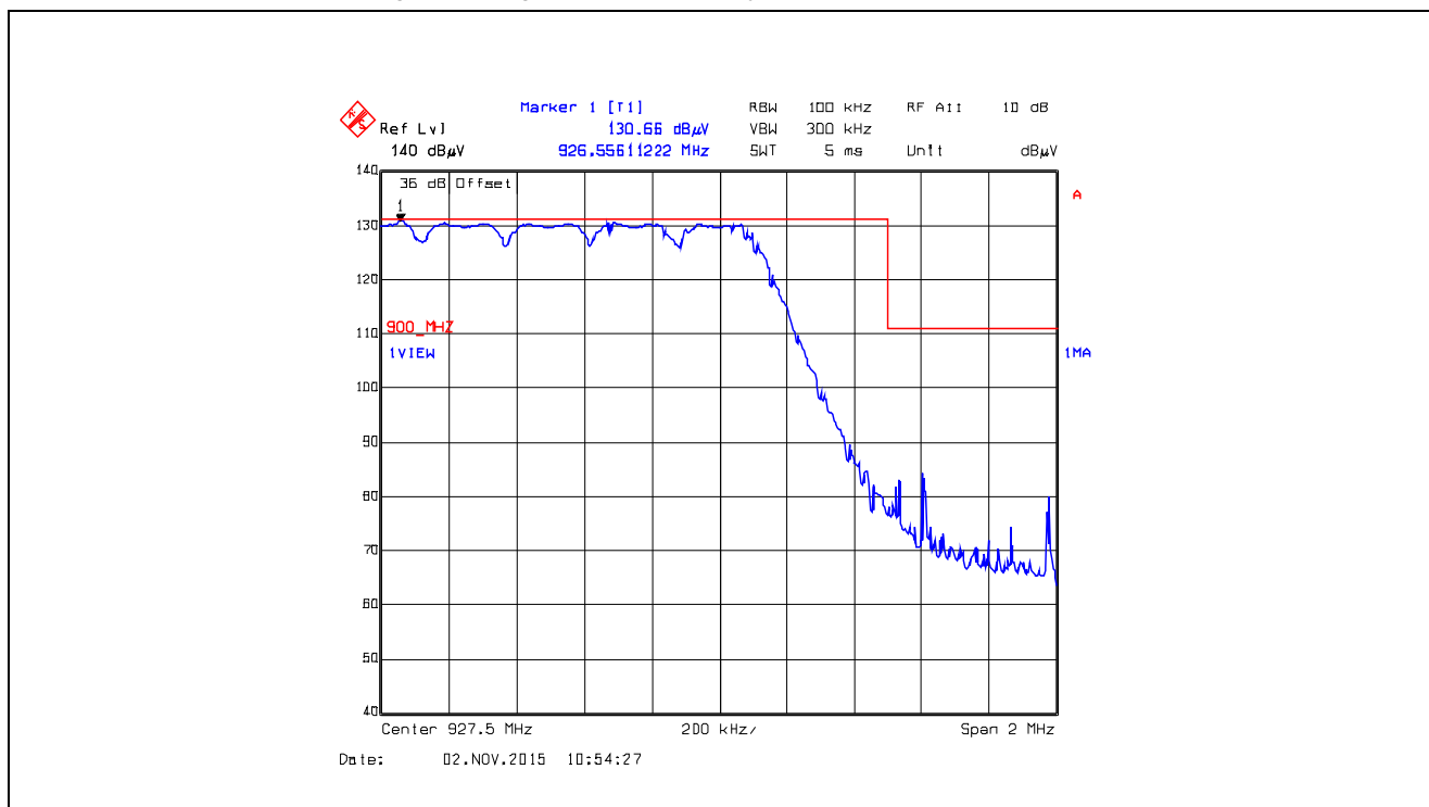
Plot 5.5.4.4.2.14. Band-Edge RF Radiated Emissions at 3 m, Horizontal Polarization Pseudorandom Hopping Mode, High End of Frequency Band, 927.5 MHz, XBX1, Data Rate at 110 kbps
