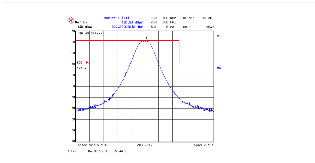
Plot 5.5.4.5.2.7. Band-Edge RF Radiated Emissions at 3 m, Vertical Polarization Single Frequency Mode, High End of Frequency Band, 927.5 MHz, XB0, Data Rate at 10 kbps
