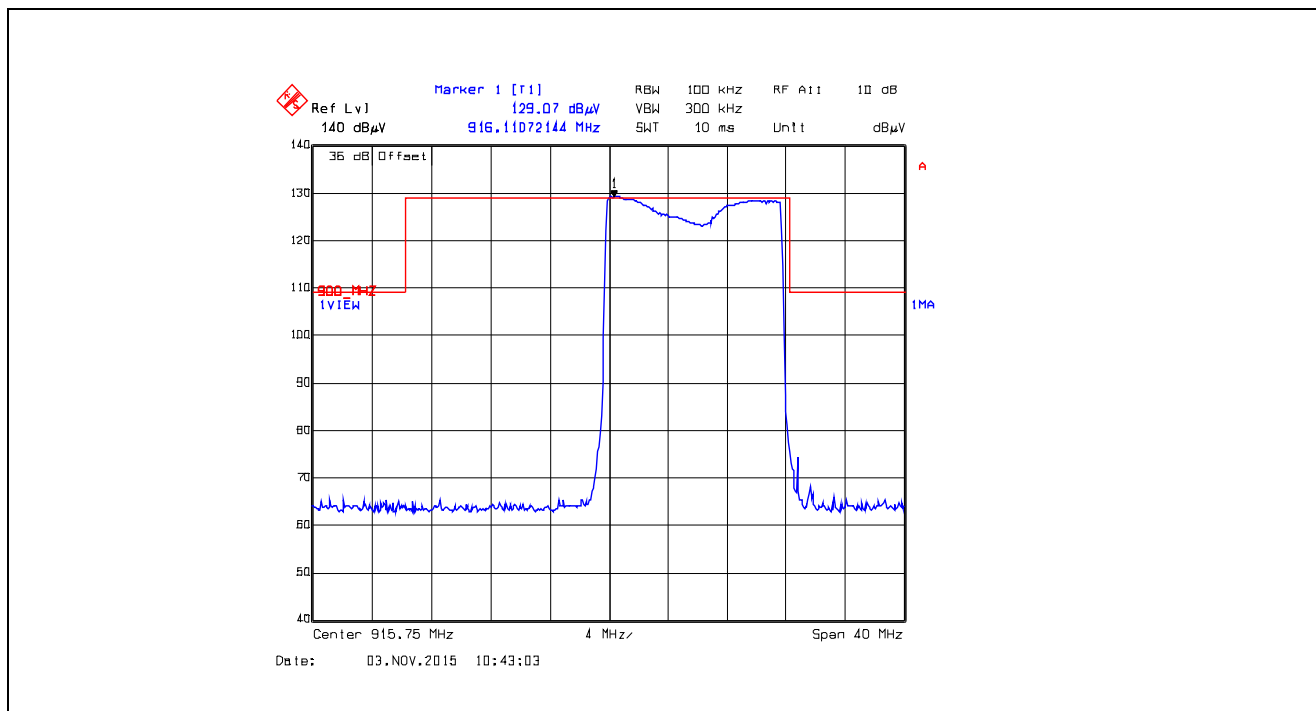
Plot 5.5.4.2.2.44. Band-Edge RF Radiated Emissions at 3 m, Vertical Polarization Pseudorandom Hopping Mode, Low End of Frequency Band, 915.75 MHz, XTCA0, Data Rate at 10 kbps
