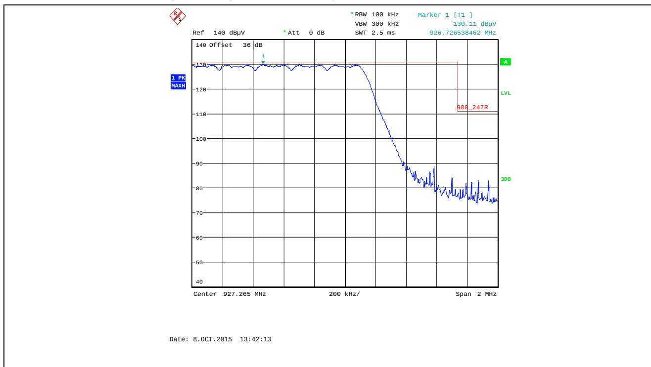
Plot 5.5.4.1.2.54. Band-Edge RF Radiated Emissions at 3 m, Horizontal Polarization Pseudorandom Hopping Mode, High End of Frequency Band, 927.265 MHz, XTCA1, Data Rate at 105kbps
