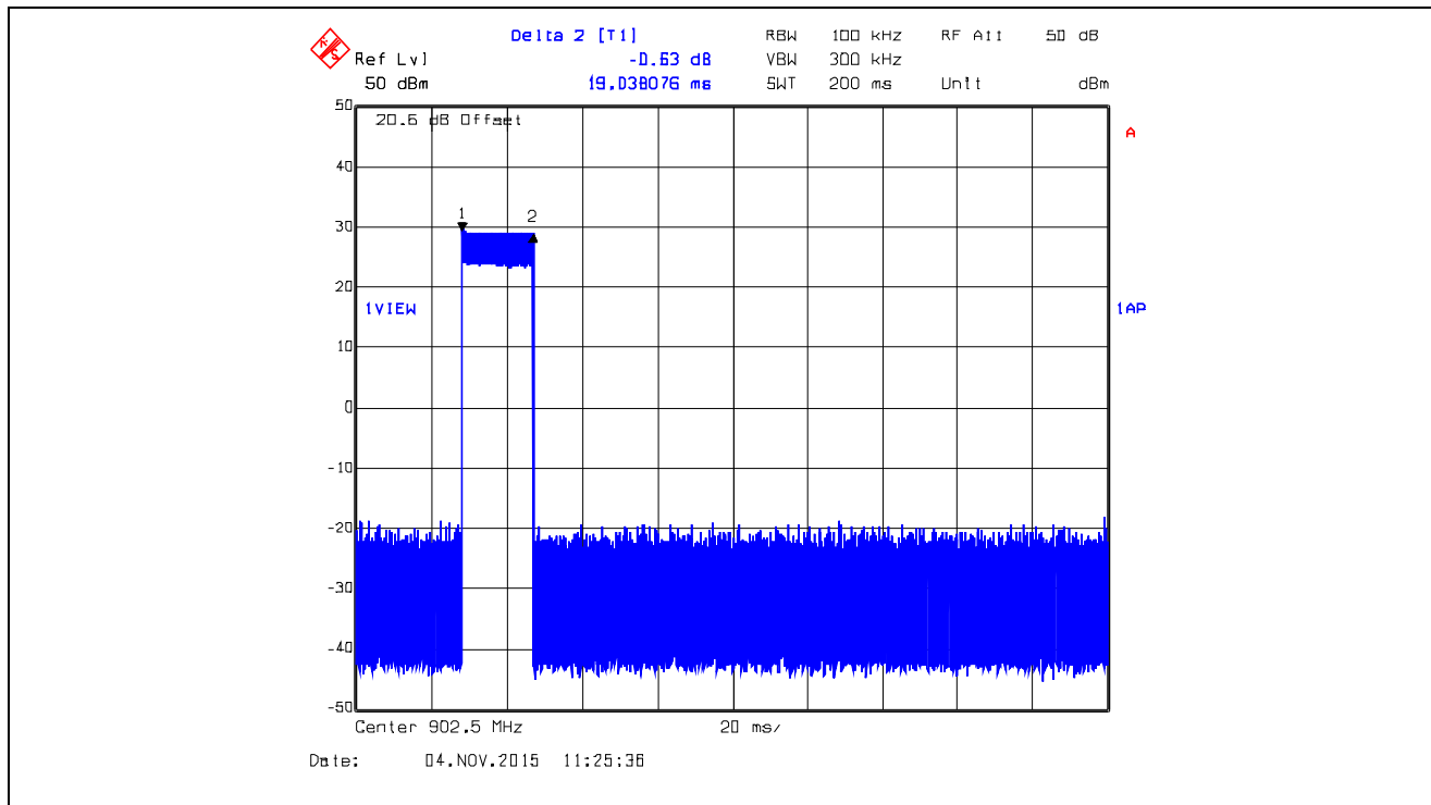
Plot 5.3.4.54. Time of Occupancy, 902.5 MHz, XB1, Data Rate at 110 kbps Dwell Time @ 902.5 MHz = 19.0381 ms
