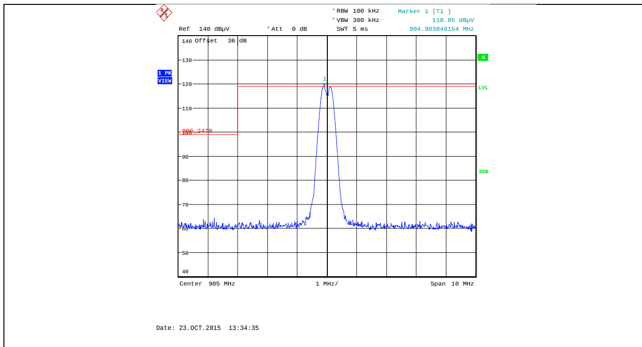
Plot 5.5.4.3.2.25. Band-Edge RF Radiated Emissions at 3 m, Horizontal Polarization Single Frequency Mode, Low End of Frequency Band, 905.0 MHz, XTC0, Data Rate at 10 kbps
