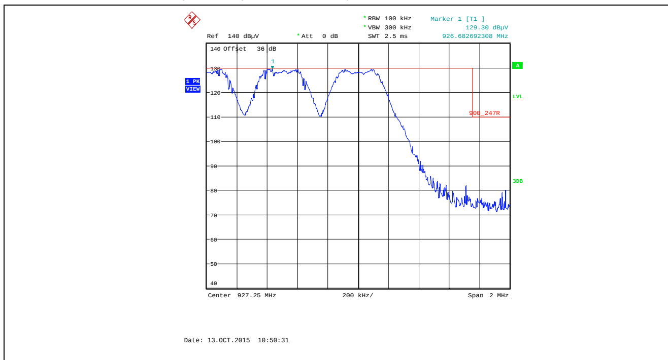
Plot 5.5.4.1.2.22. Band-Edge RF Radiated Emissions at 3 m, Horizontal Polarization Pseudorandom Hopping Mode, High End of Frequency Band, 927.25 MHz, XB2, Data Rate at 250 kbps
