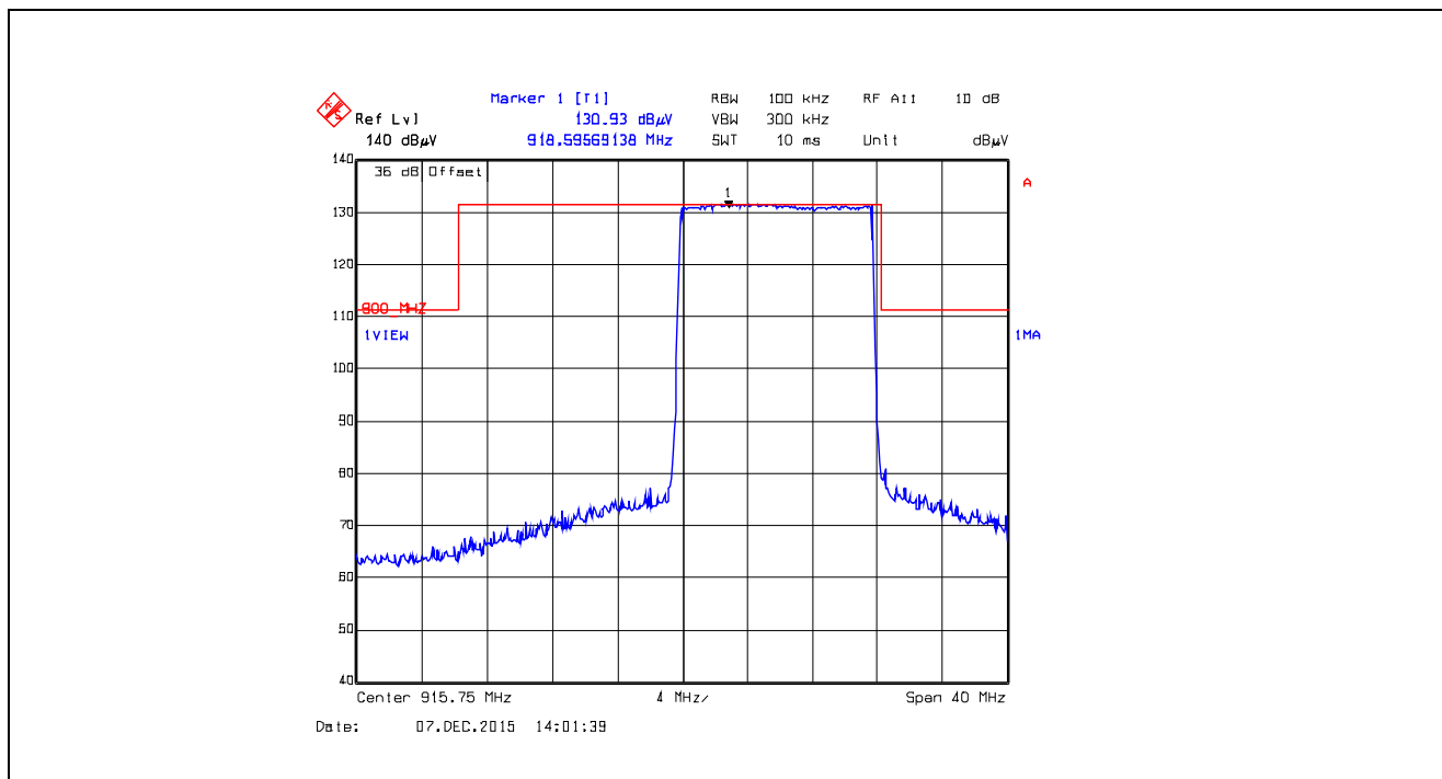
Plot 5.5.4.5.2.52. Band-Edge RF Radiated Emissions at 3 m, Vertical Polarization Pseudorandom Hopping Mode, Low End of Frequency Band, 915.75 MHz, XTCA1, Data Rate at 105kbps
