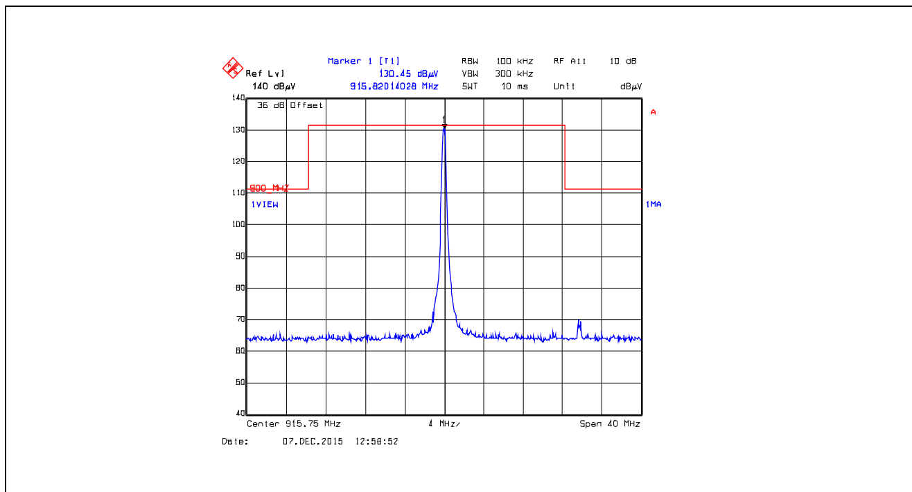
Plot 5.5.4.5.2.43. Band-Edge RF Radiated Emissions at 3 m, Vertical Polarization Single Frequency Mode, Low End of Frequency Band, 915.75 MHz, XTCA0, Data Rate at 10 kbps
