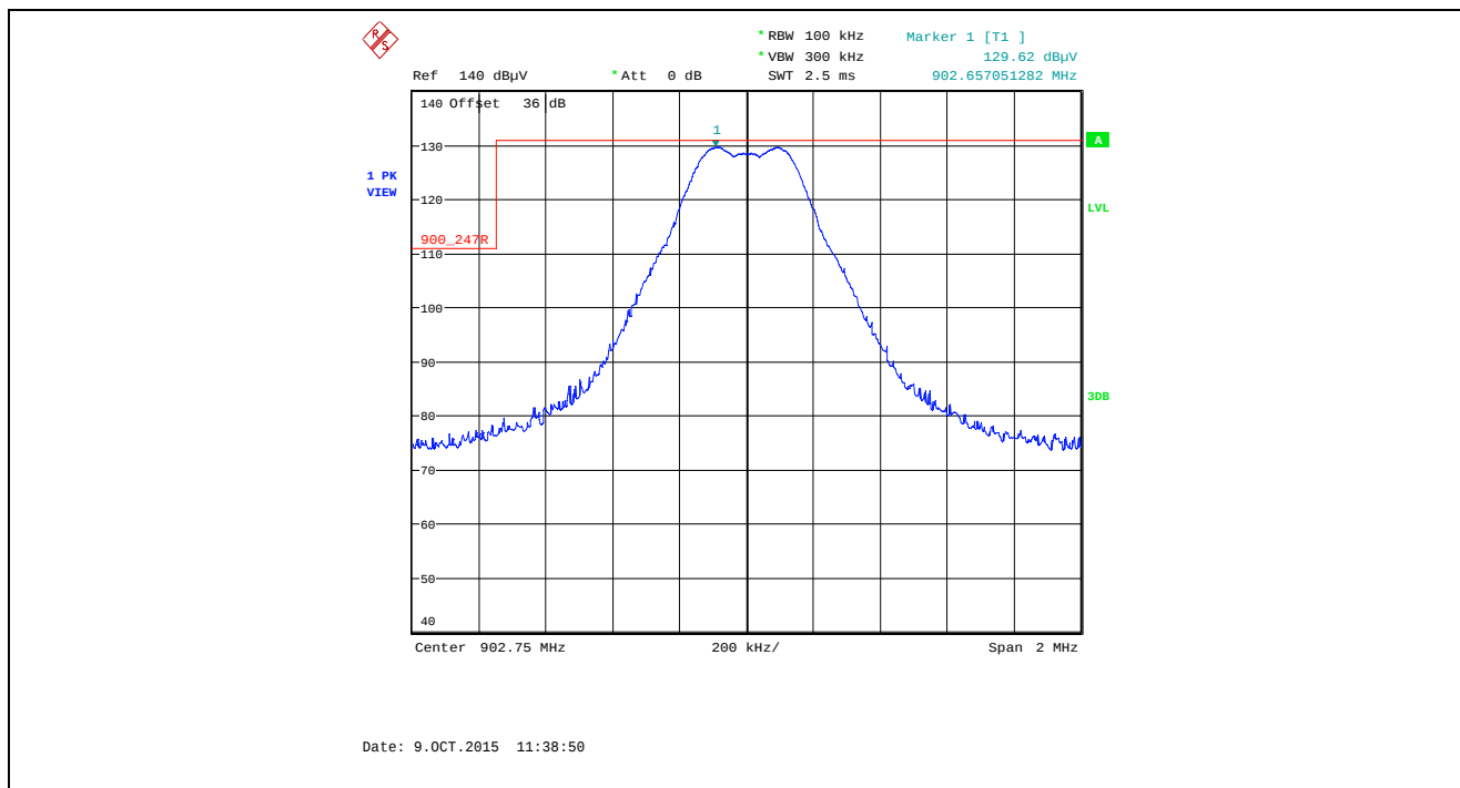
Plot 5.5.4.1.2.19. Band-Edge RF Radiated Emissions at 3 m, Vertical Polarization Single Frequency Mode, Low End of Frequency Band, 902.75 MHz, XB2, Data Rate at 250 kbps
