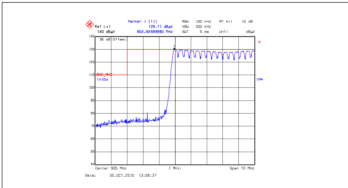
Plot 5.5.4.4.2.36. Band-Edge RF Radiated Emissions at 3 m, Vertical Polarization Pseudorandom Hopping Mode, Low End of Frequency Band, 905.0 MHz, XTC1, Data Rate at 125 kbps
