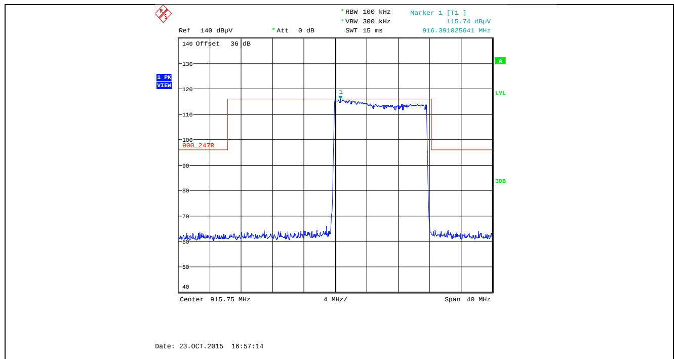
Plot 5.5.4.3.2.50. Band-Edge RF Radiated Emissions at 3 m, Horizontal Polarization Pseudorandom Hopping Mode, Low End of Frequency Band, 915.75 MHz, XTCA1, Data Rate at 105kbps
