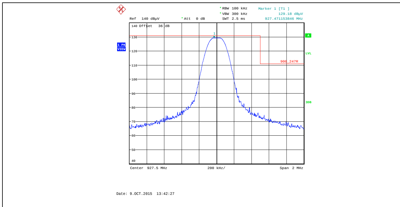
Plot 5.5.4.1.2.5. Band-Edge RF Radiated Emissions at 3 m, Horizontal Polarization Single Frequency Mode, High End of Frequency Band, 927.5 MHz, XB0, Data Rate at 10 kbps
