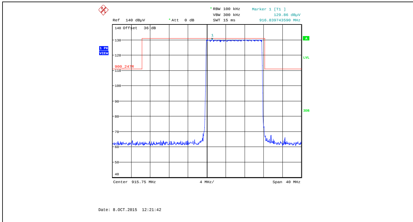
Plot 5.5.4.1.2.42. Band-Edge RF Radiated Emissions at 3 m, Horizontal Polarization Pseudorandom Hopping Mode, Low End of Frequency Band, 915.75 MHz, XTCA0, Data Rate at 10 kbps
