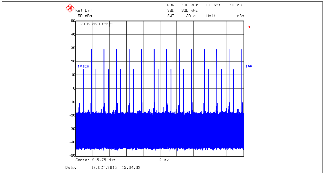
Plot 5.3.4.85. Time of Occupancy, 915.75 MHz XTCA1, Data Rate at 105 kbps Average time of occupancy = (Dwell Time) x (number of hops) = 27.6553 ms x 14 = 387.1742 ms < 0.4 sec within 20 sec
