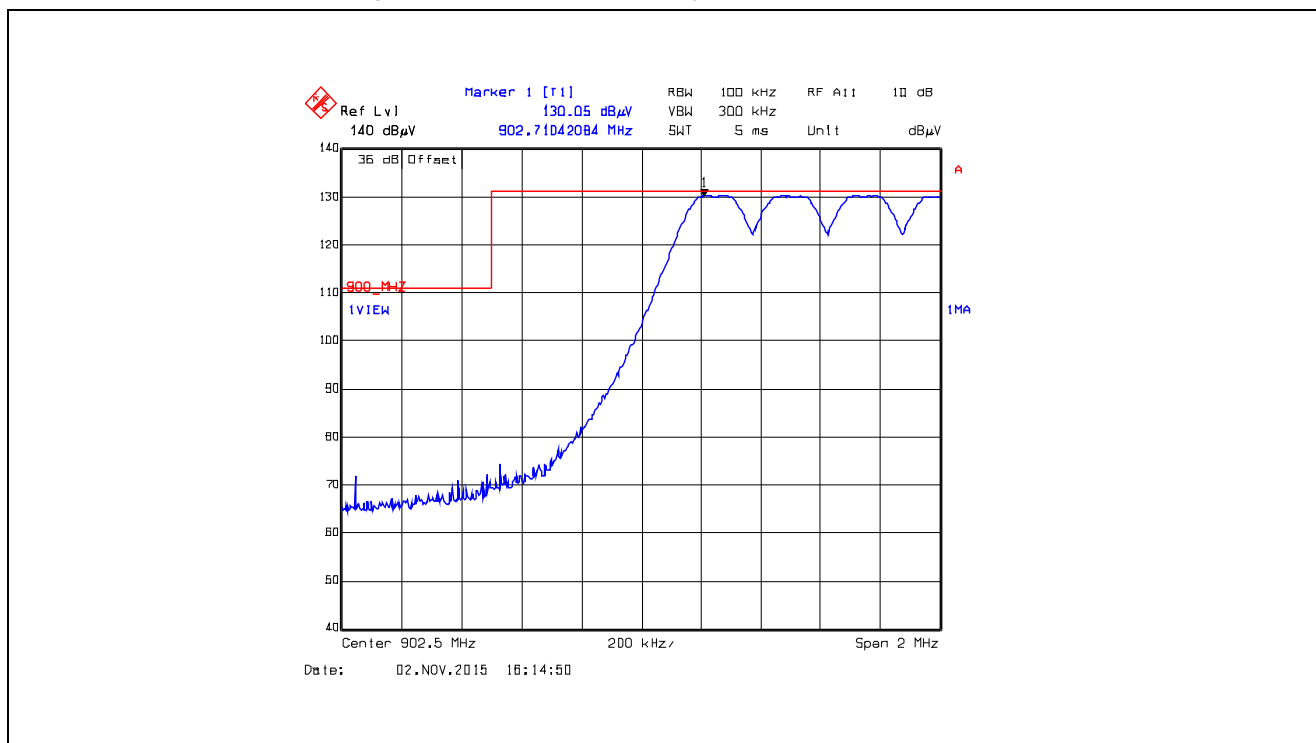
Plot 5.5.4.2.4. Band-Edge RF Radiated Emissions at 3 m, Vertical Polarization Pseudorandom Hopping Mode, Low End of Frequency Band, 902.5 MHz, XB0, Data Rate at 10 kbps
