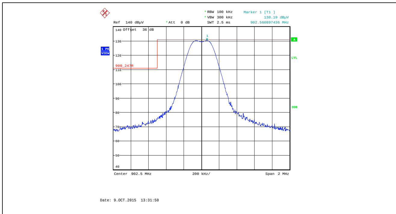
Plot 5.5.4.1.2.9. Band-Edge RF Radiated Emissions at 3 m, Horizontal Polarization Single Frequency Mode, Low End of Frequency Band, 902.5 MHz, XB1, Data Rate at 110 kbps
