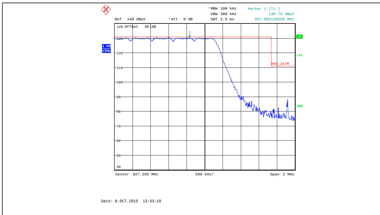
Plot 5.5.4.1.2.56. Band-Edge RF Radiated Emissions at 3 m, Vertical Polarization Pseudorandom Hopping Mode, High End of Frequency Band, 927.265 MHz, XTCA1, Data Rate at 105kbps
