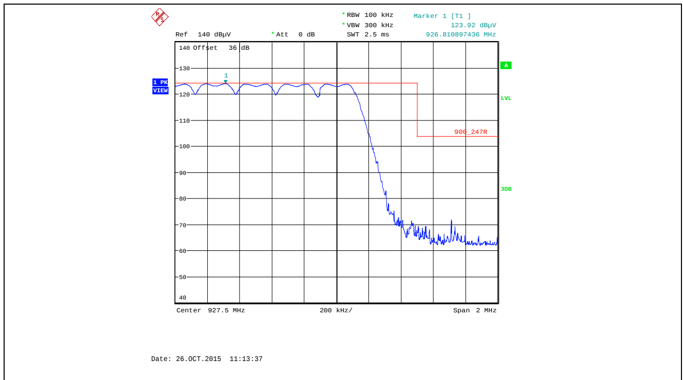
Plot 5.5.4.3.2.16. Band-Edge RF Radiated Emissions at 3 m, Vertical Polarization Pseudorandom Hopping Mode, High End of Frequency Band, 927.5 MHz, XBX1, Data Rate at 110 kbps
