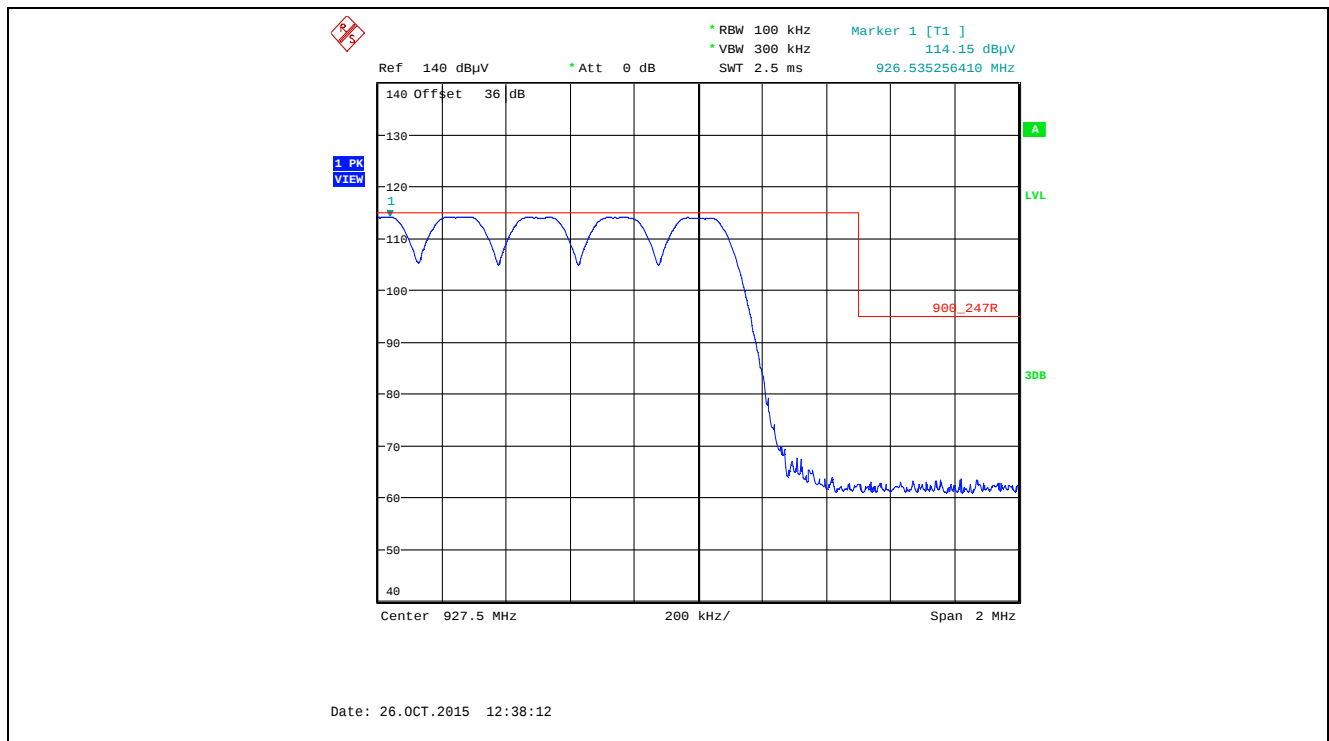
Plot 5.5.4.3.2.6. Band-Edge RF Radiated Emissions at 3 m, Horizontal Polarization Pseudorandom Hopping Mode, High End of Frequency Band, 927.5 MHz, XB0, Data Rate at 10 kbps
