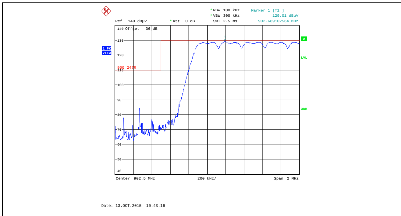
Plot 5.5.4.1.2.10. Band-Edge RF Radiated Emissions at 3 m, Horizontal Polarization Pseudorandom Hopping Mode, Low End of Frequency Band, 902.5 MHz, XB1, Data Rate at 110 kbps
