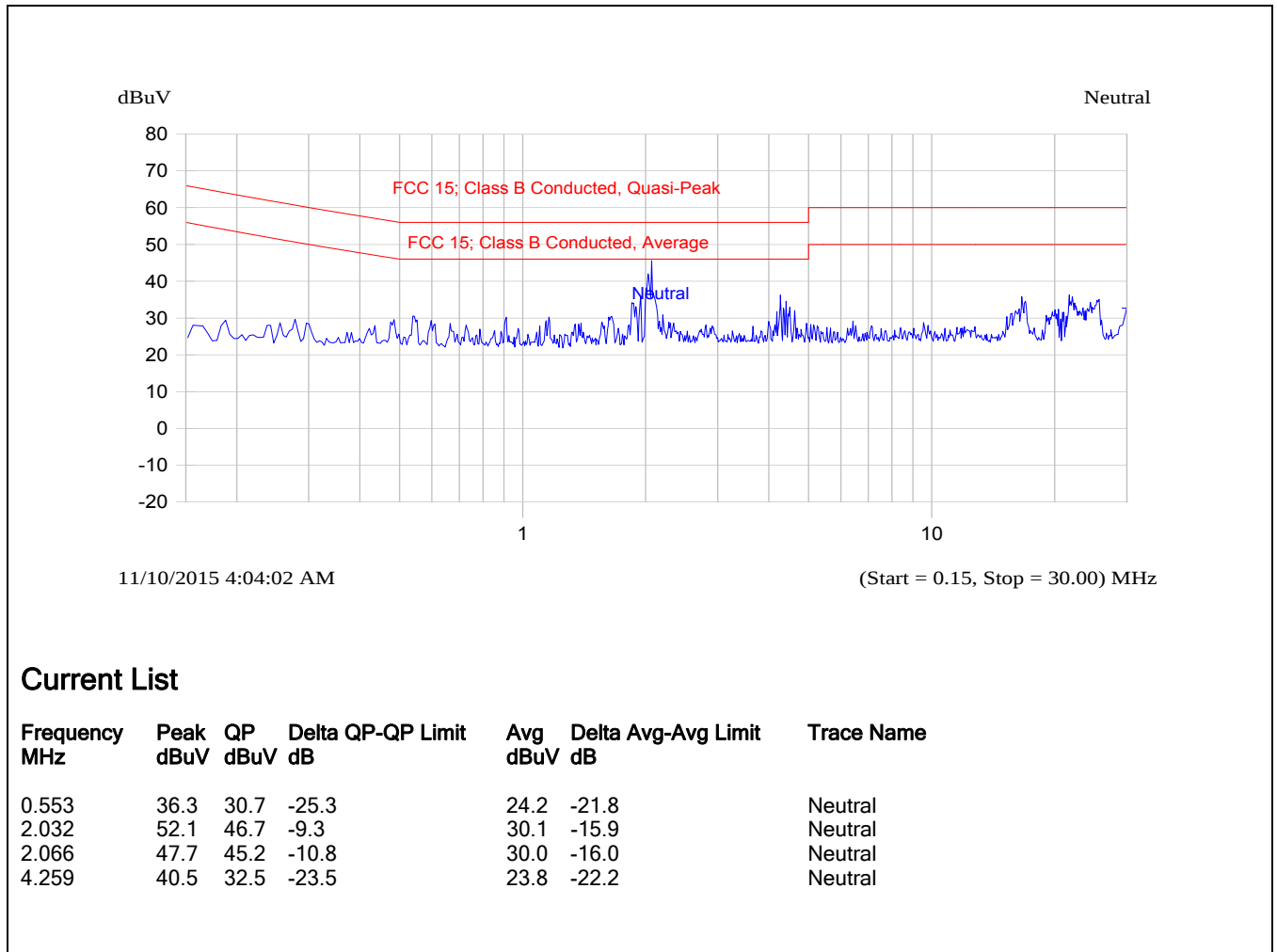
Plot 5.1.4.4. Power Line Conducted Emissions (Rx Mode) Line Voltage: 120 VAC; Line Tested: Neutral
