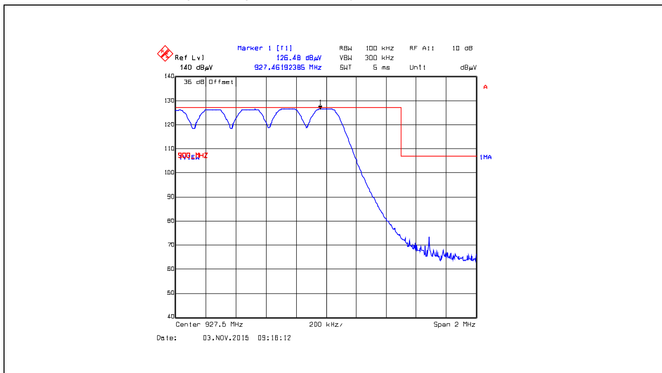
Plot 5.5.4.2.8. Band-Edge RF Radiated Emissions at 3 m, Vertical Polarization Pseudorandom Hopping Mode, High End of Frequency Band, 927.5 MHz, XB0, Data Rate at 10 kbps
