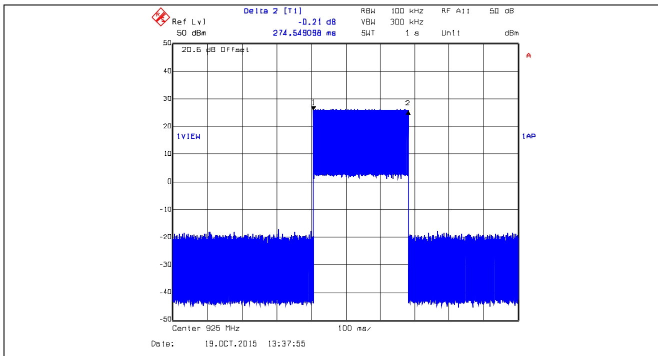
Plot 5.3.4.70. Time of Occupancy, 925.0 MHz, XTC0, Data Rate at 10 kbps Dwell Time @ 925.0 MHz = 274.55 ms
