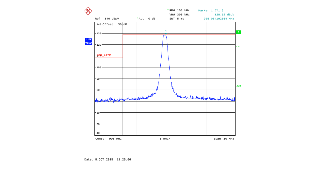
Plot 5.5.4.1.2.35. Band-Edge RF Radiated Emissions at 3 m, Vertical Polarization Single Frequency Mode, Low End of Frequency Band, 905.0 MHz, XTC1, Data Rate at 125 kbps
