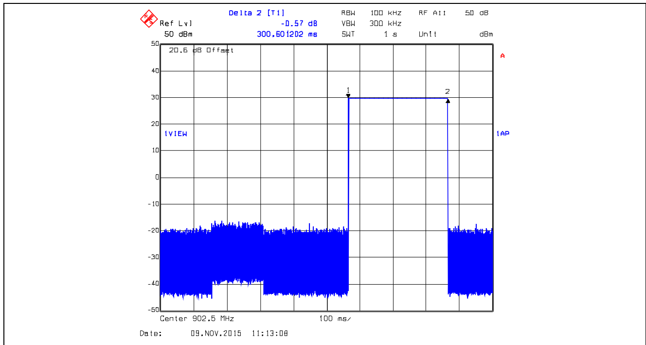
Plot 5.3.4.48. Time of Occupancy, 902.5 MHz, XB0, Data Rate at 10 kbps Dwell Time @ 902.5 MHz = 300.601202 ms
