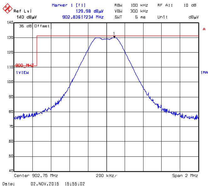
Plot 5.5.4.2.20. Band-Edge RF Radiated Emissions at 3 m, Vertical Polarization Pseudorandom Hopping Mode, Low End of Frequency Band, 902.75 MHz, XB2, Data Rate at 250 kbps
