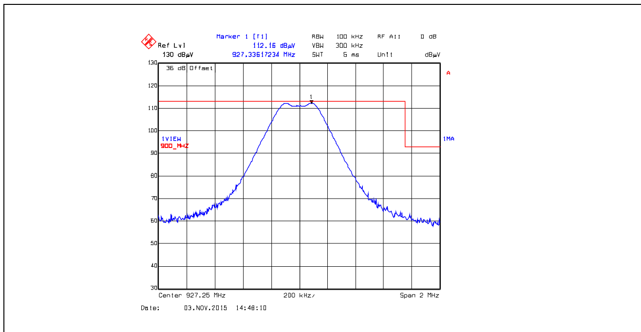
Plot 5.5.4.2.21. Band-Edge RF Radiated Emissions at 3 m, Horizontal Polarization Single Frequency Mode, High End of Frequency Band, 927.25 MHz, XB2, Data Rate at 250 kbps
