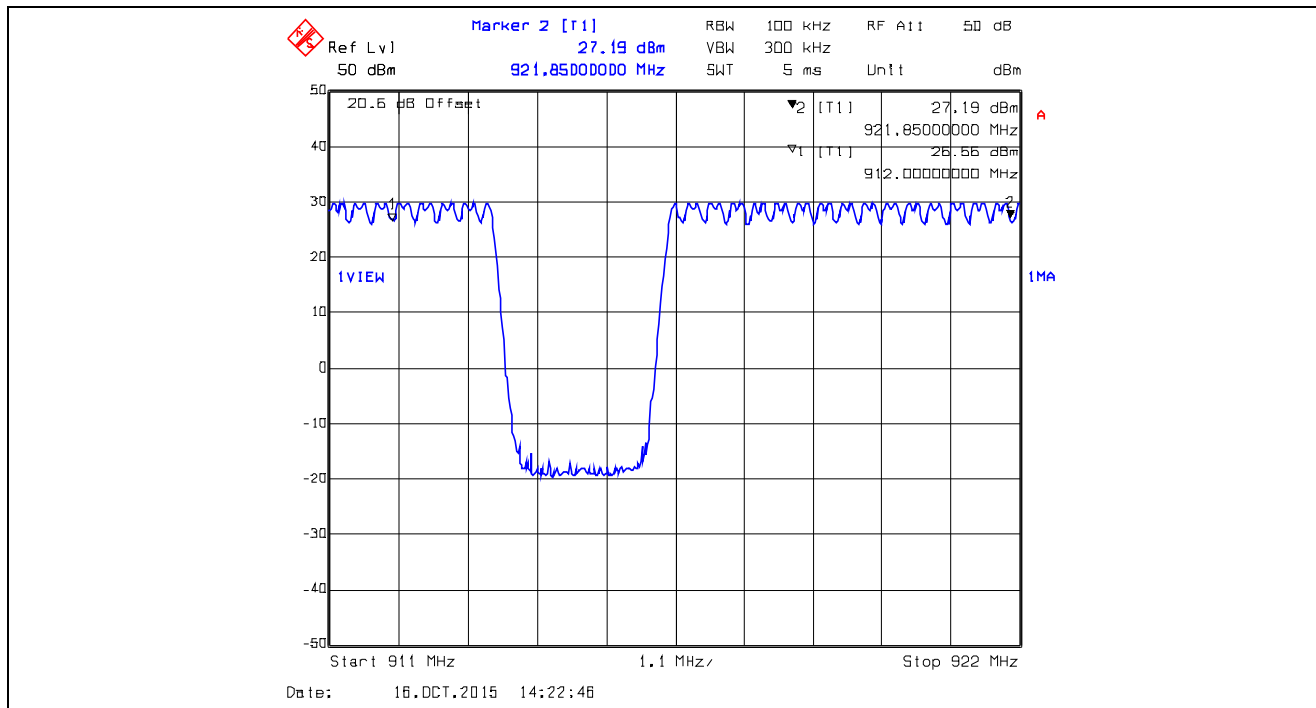
Plot 5.3.4.33. Number of Hopping Frequencies, XTC0, Data Rate at 10 kbps 21 Hopping Channels from 912 – 922 MHz
