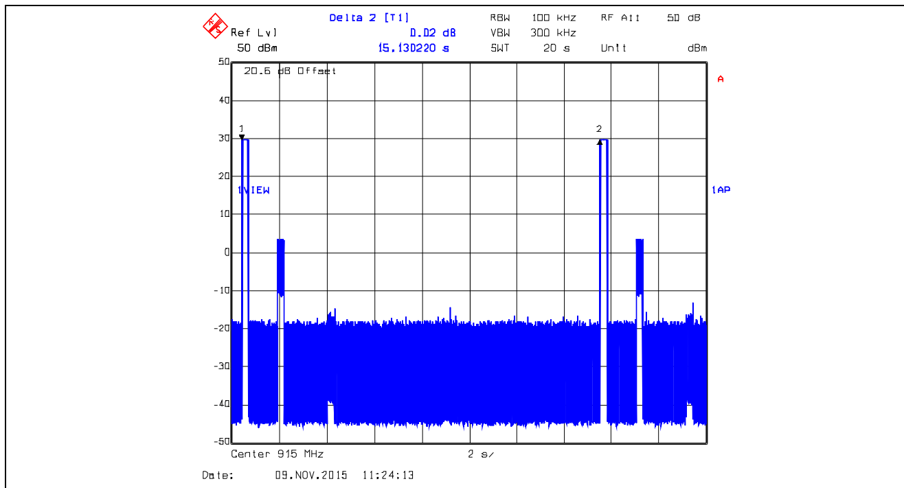
Plot 5.3.4.51. Time of Occupancy, 915 MHz XBX0, Data Rate at 10 kbps Average time of occupancy = 20 \times (T_{\text{on}}) / (T_{\text{total}}) = 20 \times 0.3006012\text{s} / 15.1302\text{s} = 0.3974\text{s} < 0.4\text{s}
