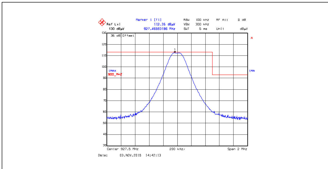
Plot 5.5.4.2.5. Band-Edge RF Radiated Emissions at 3 m, Horizontal Polarization Single Frequency Mode, High End of Frequency Band, 927.5 MHz, XB0, Data Rate at 10 kbps
