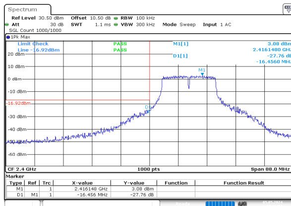
g_2412MHz_Chain 0
