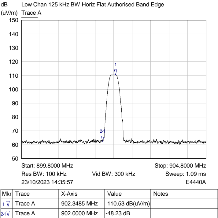
Low channel 125kHz BW Authorised Band edge plot
