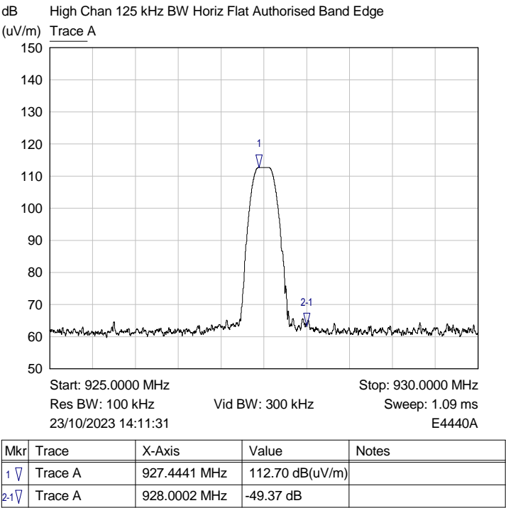
High channel 125kHz BW Authorised Band edge plot
