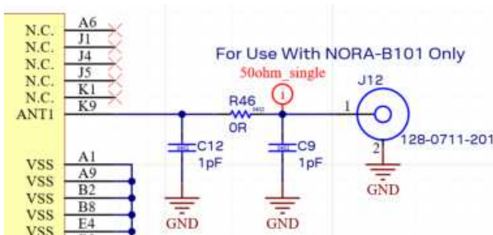
Figure 19: NORA-B101 ANT pin U.FL schematic
