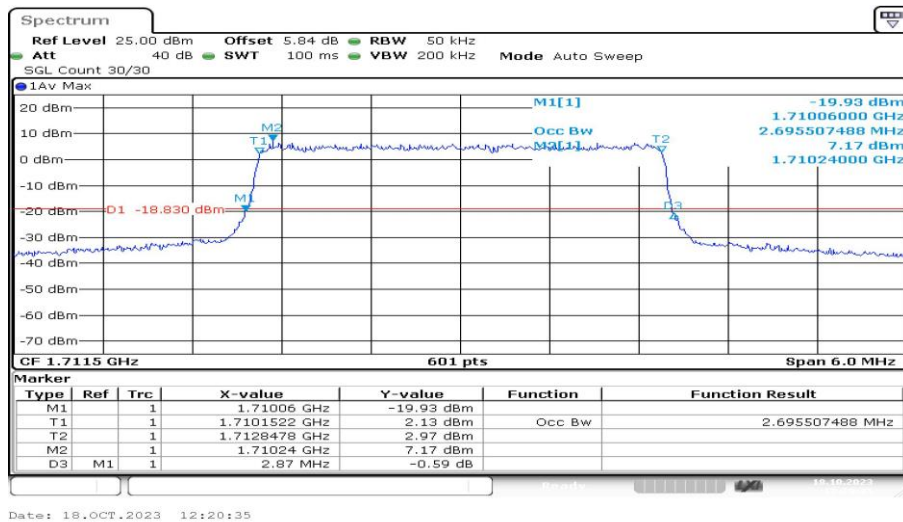
Band4-3MHz-QPSK-19965-15RB#0-PASS
