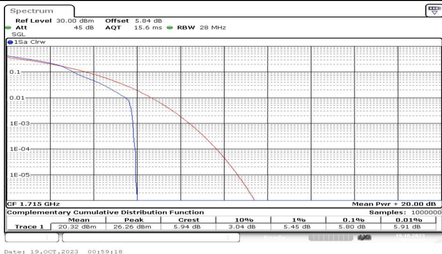
Band4-10MHz-16QAM-20000-1RB#0-PASS
