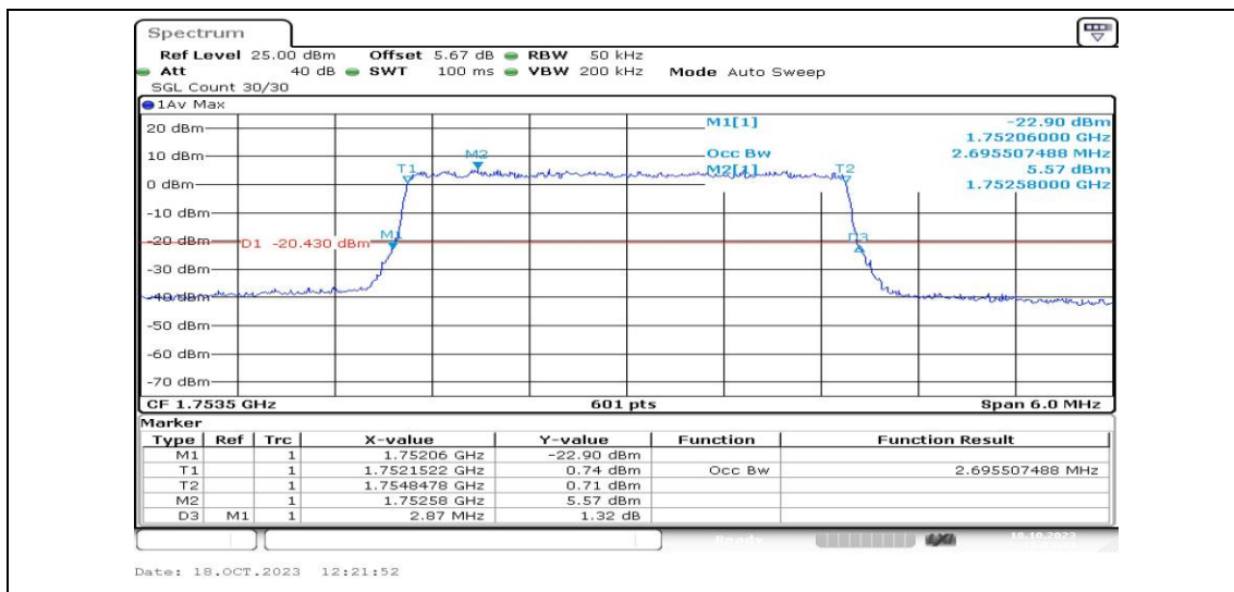
Band4-3MHz-16QAM-20385-15RB#0-PASS
