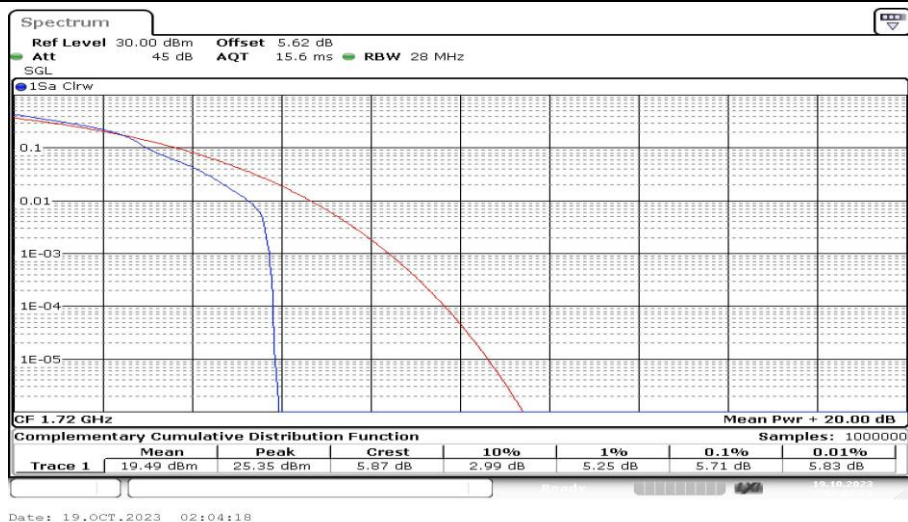
Band4-20MHz-16QAM-20050-1RB#0-PASS
