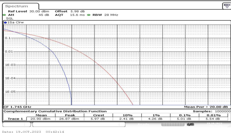
Band4-20MHz-QPSK-20300-100RB#0-PASS
