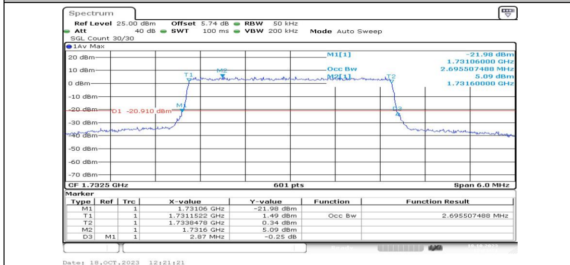
Band4-3MHz-16QAM-20175-15RB#0-PASS
