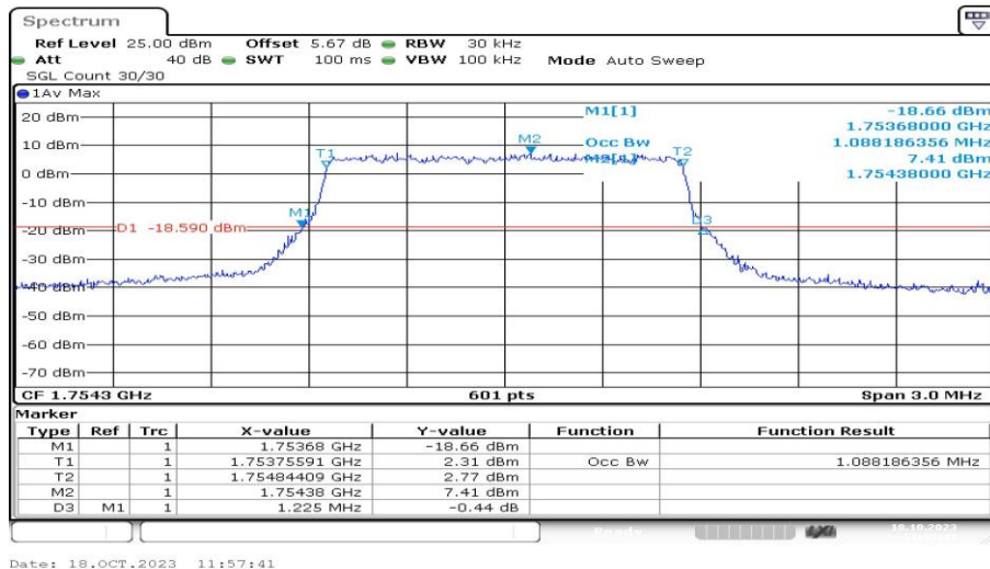
Band4-1.4MHz-16QAM-20393-6RB#0-PASS
