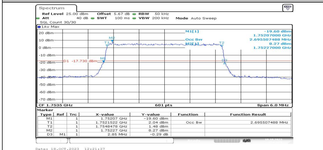
Band4-3MHz-QPSK-20385-15RB#0-PASS
