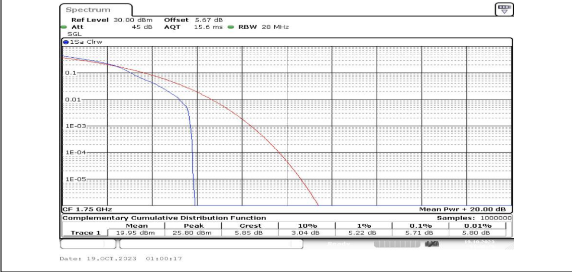
Band4-10MHz-16QAM-20350-1RB#0-PASS
