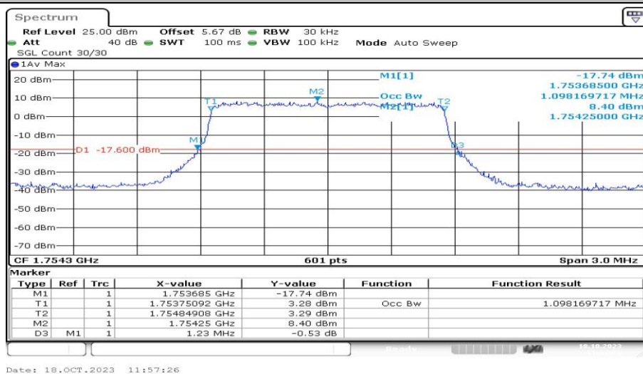
Band4-1.4MHz-QPSK-20393-6RB#0-PASS
