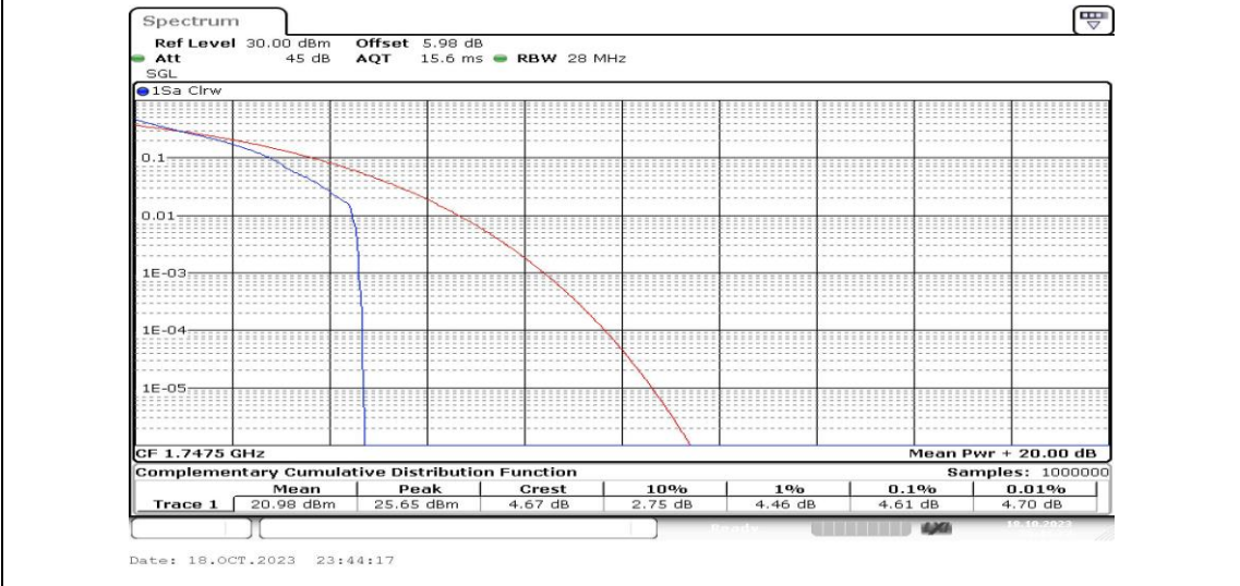
Band4-15MHz-QPSK-20325-1RB#0-PASS
