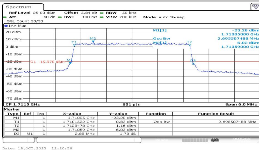
Band4-3MHz-16QAM-19965-15RB#0-PASS
