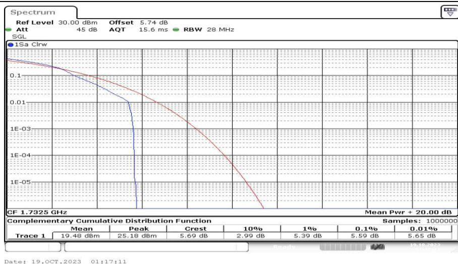
Band4-15MHz-16QAM-20175-1RB#0-PASS
