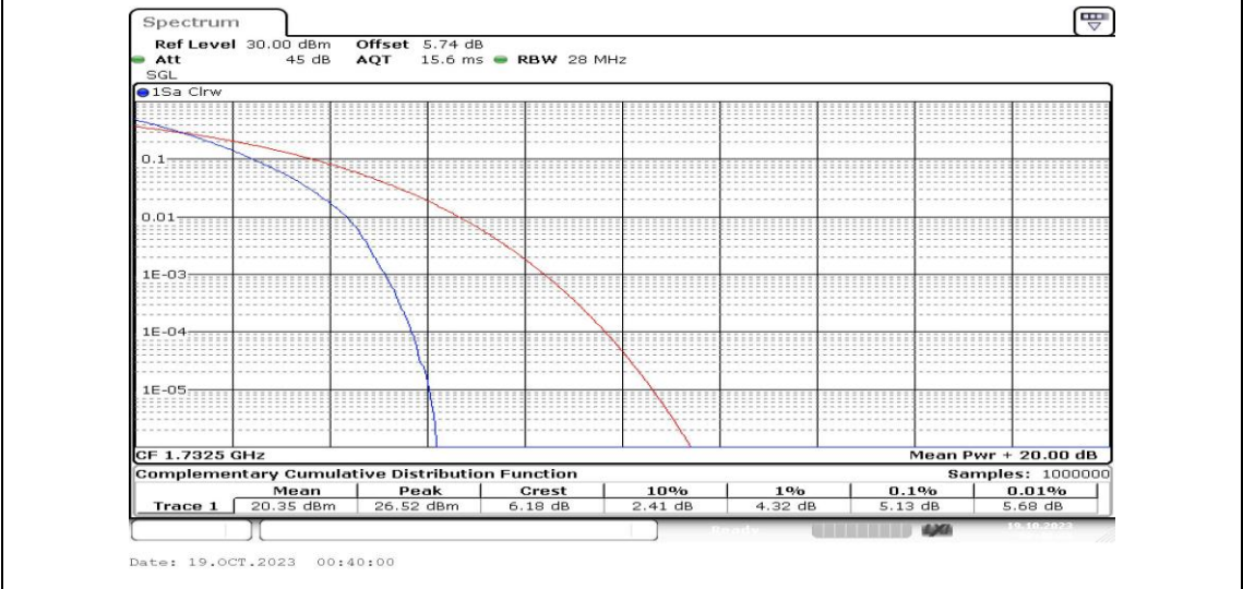
Band4-20MHz-QPSK-20175-100RB#0-PASS
