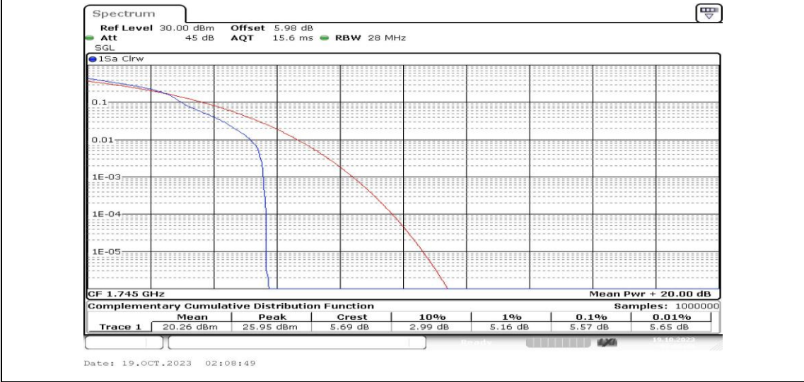
Band4-20MHz-16QAM-20300-1RB#0-PASS
