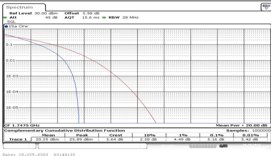
Band4-15MHz-QPSK-20325-75RB#0-PASS
