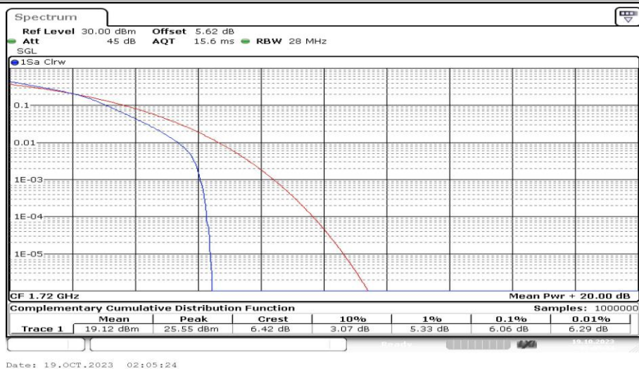
Band4-20MHz-16QAM-20050-25RB#0-PASS
