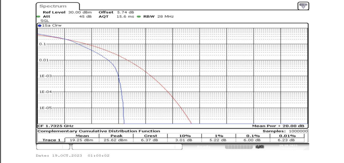
Band4-10MHz-16QAM-20175-25RB#0-PASS
