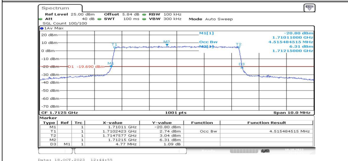
Band4-5MHz-16QAM-19975-25RB#0-PASS
