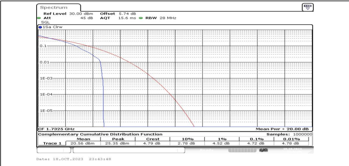
Band4-15MHz-QPSK-20175-1RB#0-PASS
