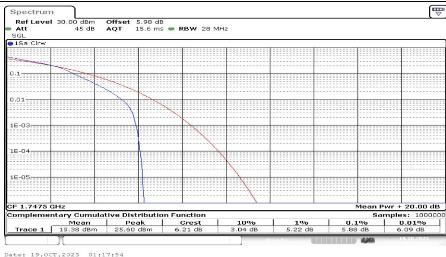
Band4-15MHz-16QAM-20325-25RB#0-PASS
