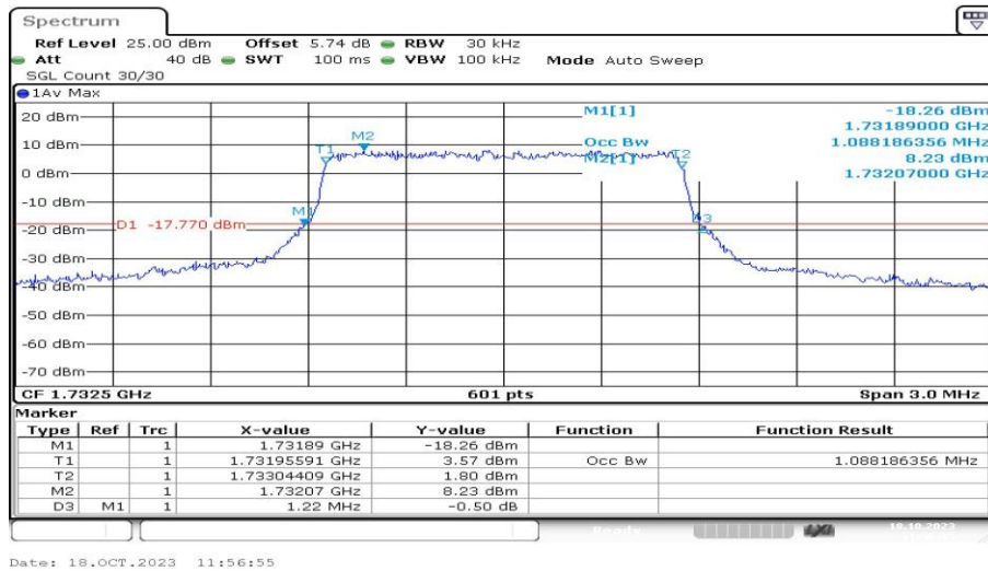
Band4-1.4MHz-QPSK-20175-6RB#0-PASS
