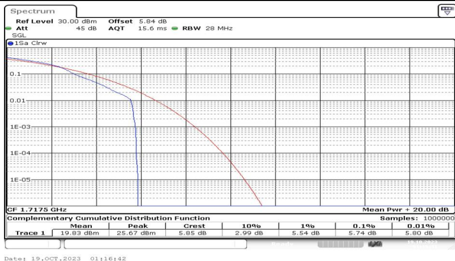
Band4-15MHz-16QAM-20025-1RB#0-PASS
