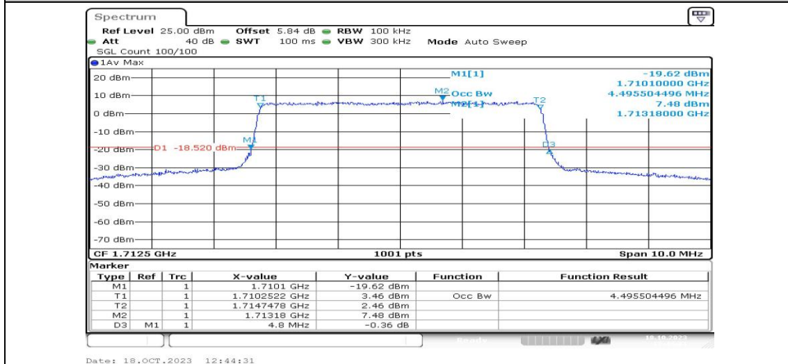
Band4-5MHz-QPSK-19975-25RB#0-PASS
