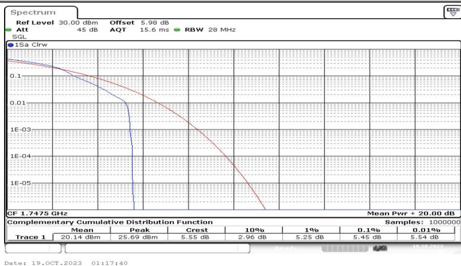
Band4-15MHz-16QAM-20325-1RB#0-PASS
