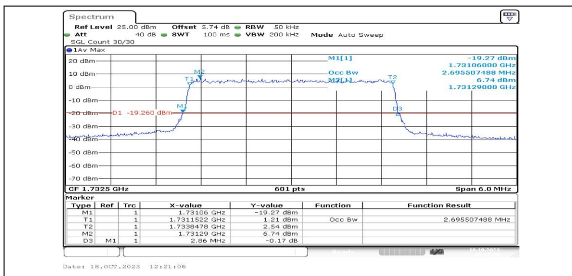
Band4-3MHz-QPSK-20175-15RB#0-PASS
