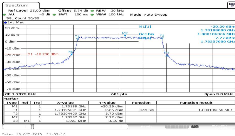
Band4-1.4MHz-16QAM-20175-6RB#0-PASS
