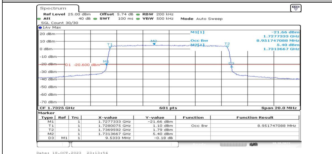
Band4-10MHz-QPSK-20175-50RB#0-PASS
