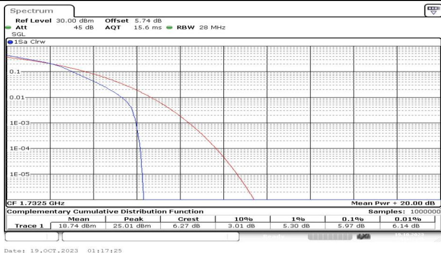
Band4-15MHz-16QAM-20175-25RB#0-PASS
