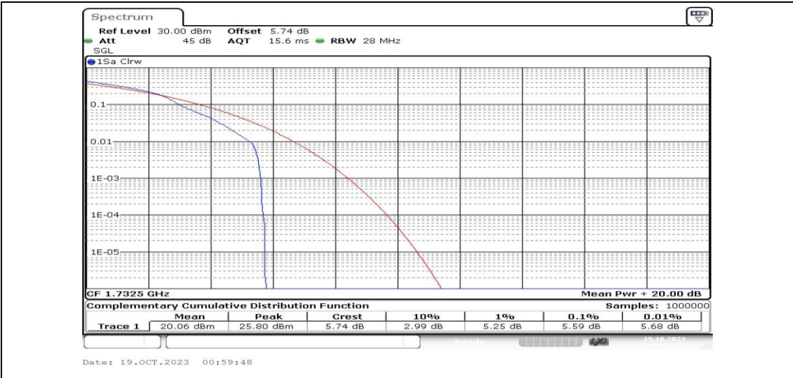
Band4-10MHz-16QAM-20175-1RB#0-PASS
