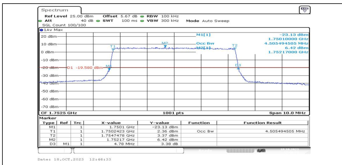
Band4-5MHz-16QAM-20375-25RB#0-PASS
