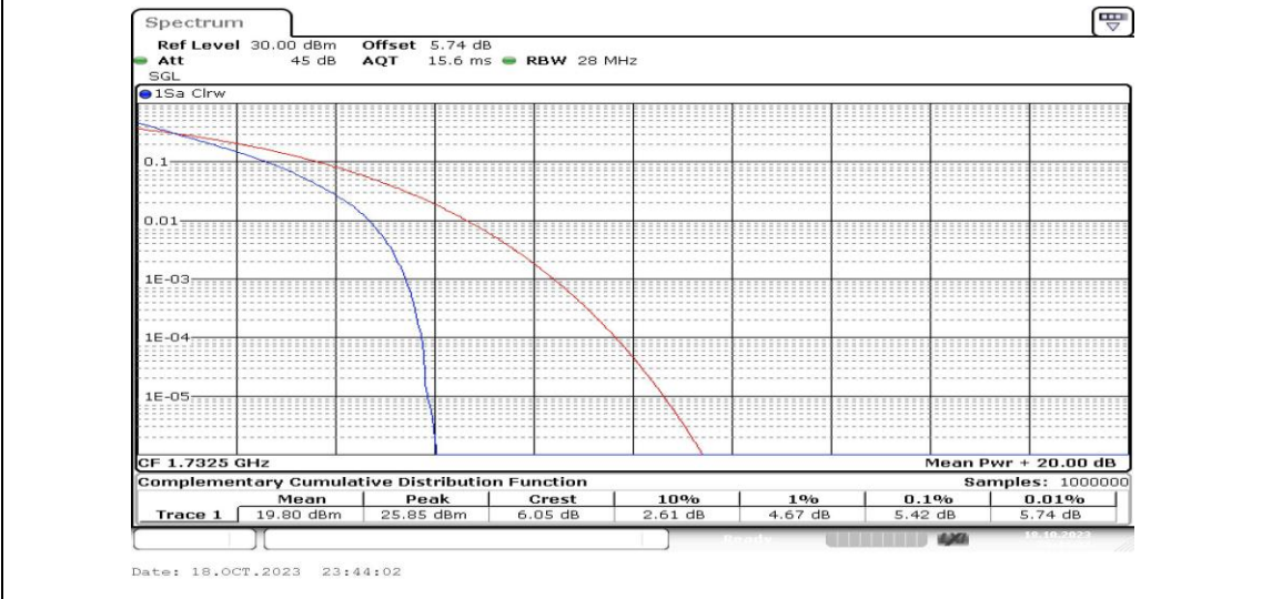
Band4-15MHz-QPSK-20175-75RB#0-PASS
