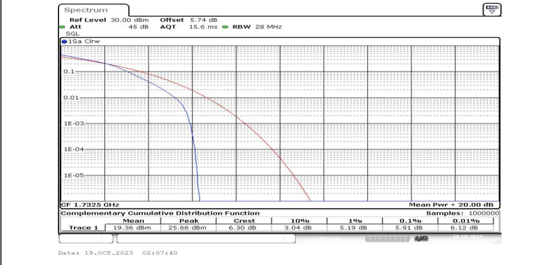
Band4-20MHz-16QAM-20175-25RB#0-PASS
