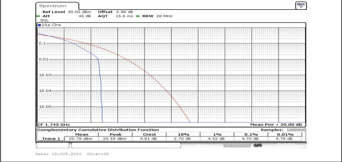
Band4-20MHz-QPSK-20300-1RB#0-PASS
