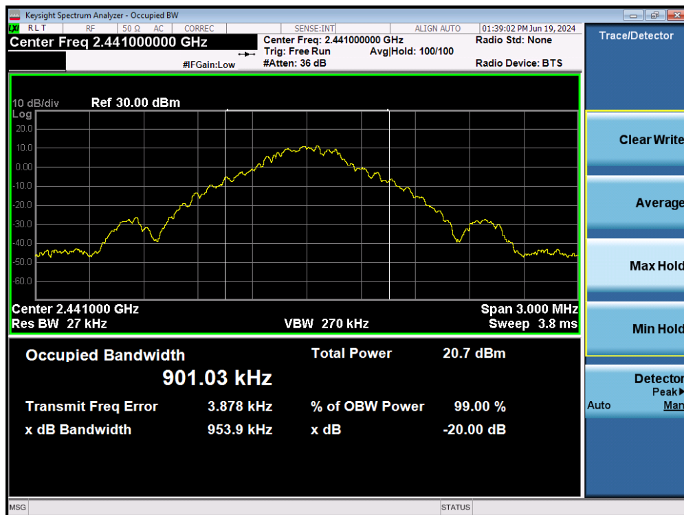
Plot 7-12. 20dB Bandwidth Plot (Bluetooth, 1Mbps – Ch. 39) – Ant 2
