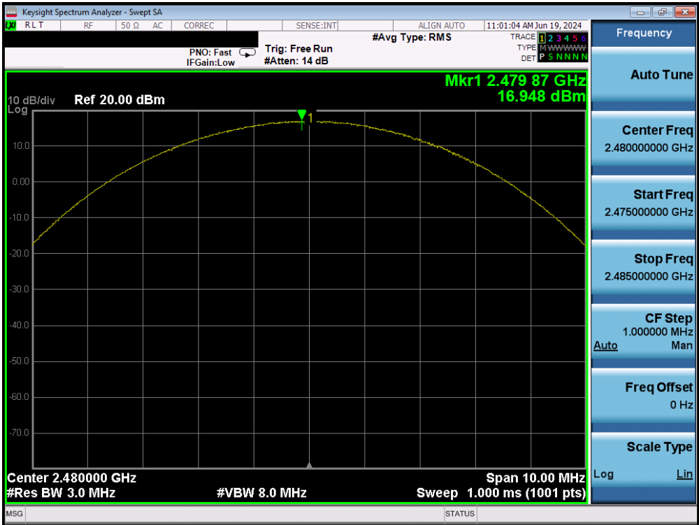
Plot 7-46. Peak Conducted Power (3Mbps – Ch. 78) – Ant 2
