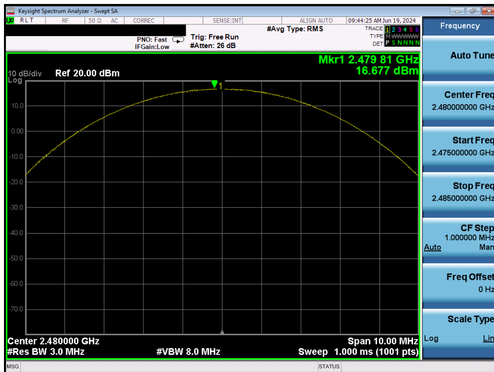
Plot 7-25. Peak Conducted Power (2Mbps – Ch. 78) – Ant 1
