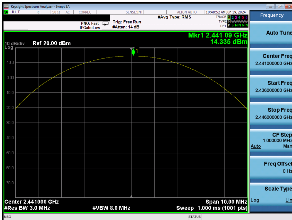
Plot 7-39. Peak Conducted Power (1Mbps – Ch. 39) – Ant 2
