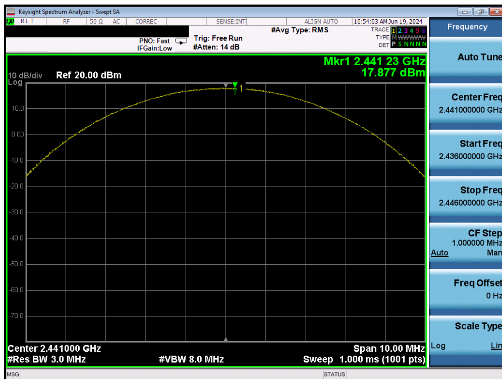
Plot 7-42. Peak Conducted Power (2Mbps – Ch. 39) – Ant 2
