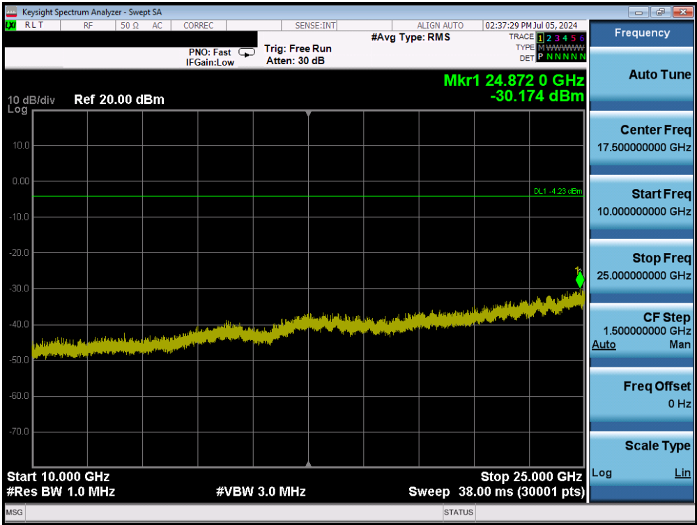
Plot 7-73. Conducted Spurious Plot (Bluetooth, 1Mbps – Ch. 0) – Ant1
