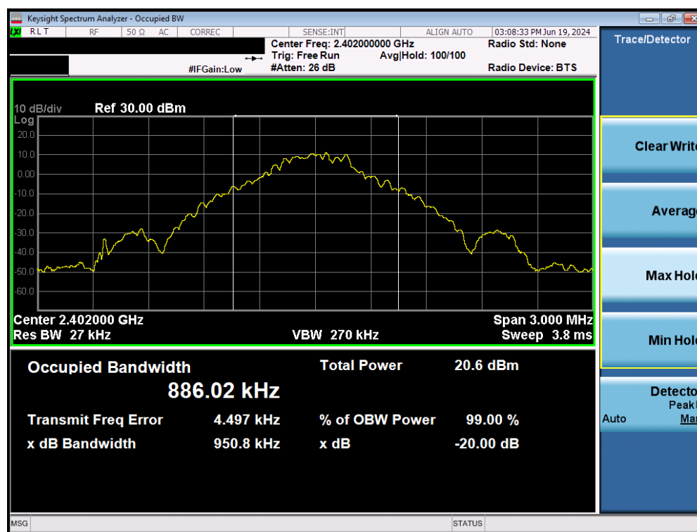
Plot 7-2. 20dB Bandwidth Plot (Bluetooth, 1Mbps – Ch. 0) – Ant 1
