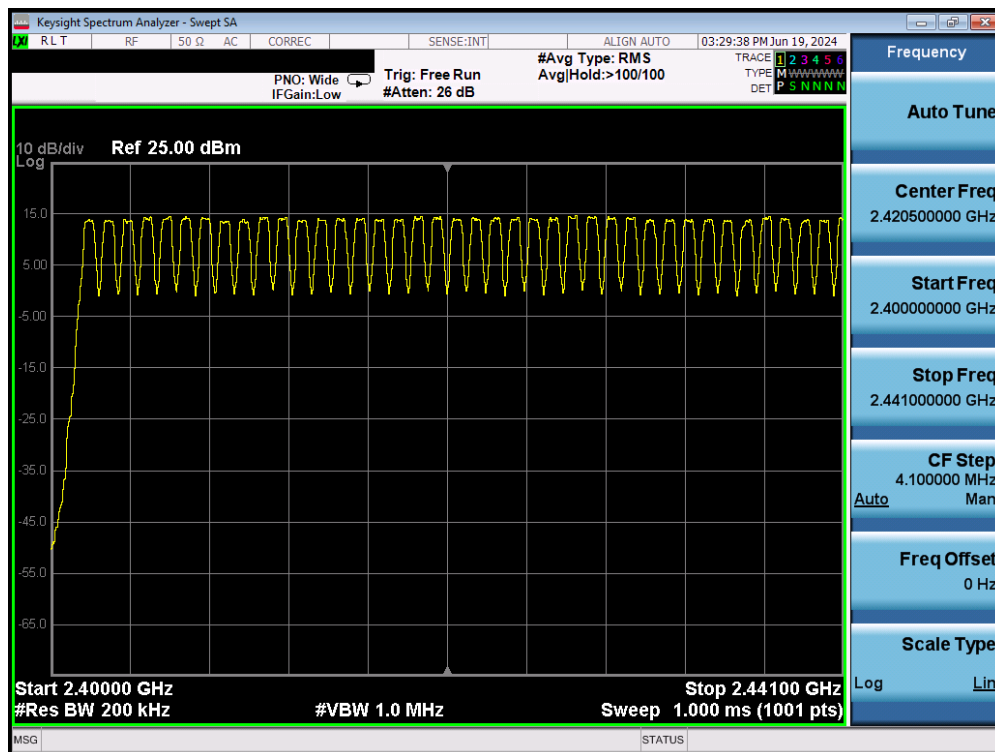
Plot 7-68. Low End Spectrum Channel Hopping Plot (Bluetooth) – Ant1
