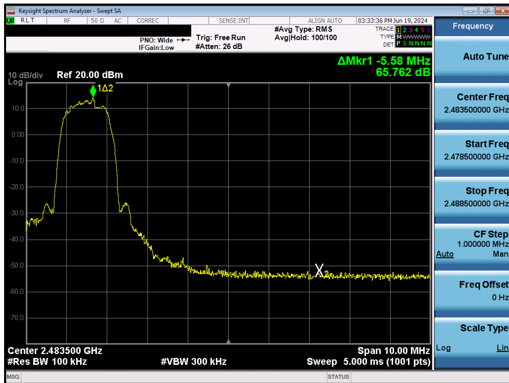
Plot 7-57. Band Edge Plot (Bluetooth with Hopping Disabled, 3 Mbps – Ch. 78) – Ant1
