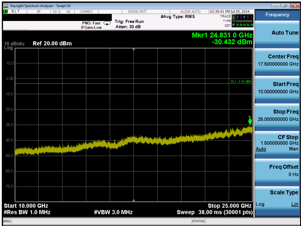
Plot 7-79. Conducted Spurious Plot (Bluetooth, 1Mbps – Ch. 0) – Ant2
