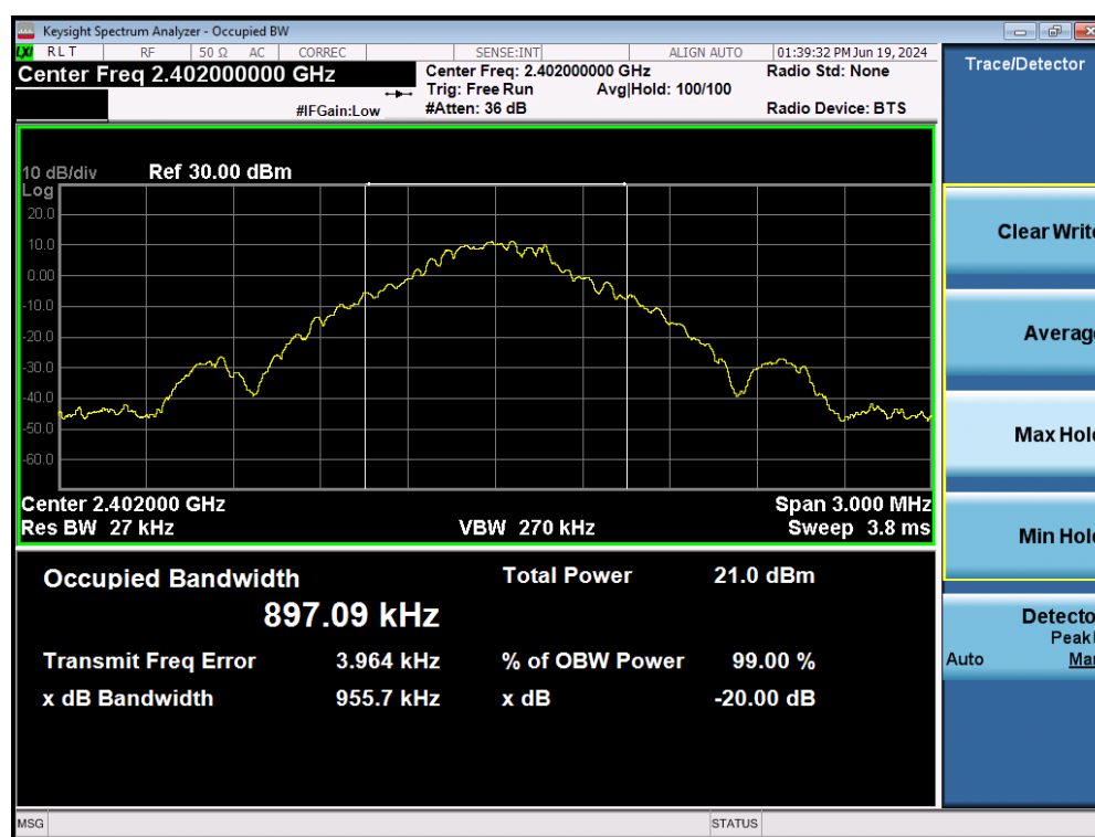
Plot 7-11. 20dB Bandwidth Plot (Bluetooth, 1Mbps – Ch. 0) – Ant 2
