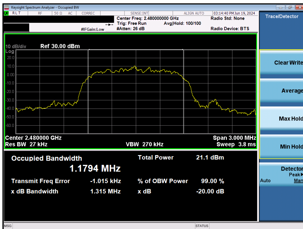
Plot 7-7. 20dB Bandwidth Plot (Bluetooth, 2Mbps – Ch. 78) – Ant 1
