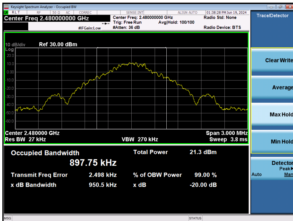
Plot 7-13. 20dB Bandwidth Plot (Bluetooth, 1Mbps – Ch. 78) – Ant 2
