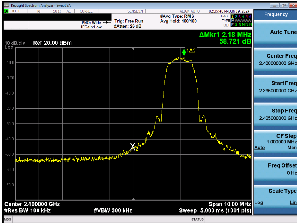
Plot 7-60. Band Edge Plot (Bluetooth with Hopping Disabled, 3 Mbps – Ch. 0) – Ant2
