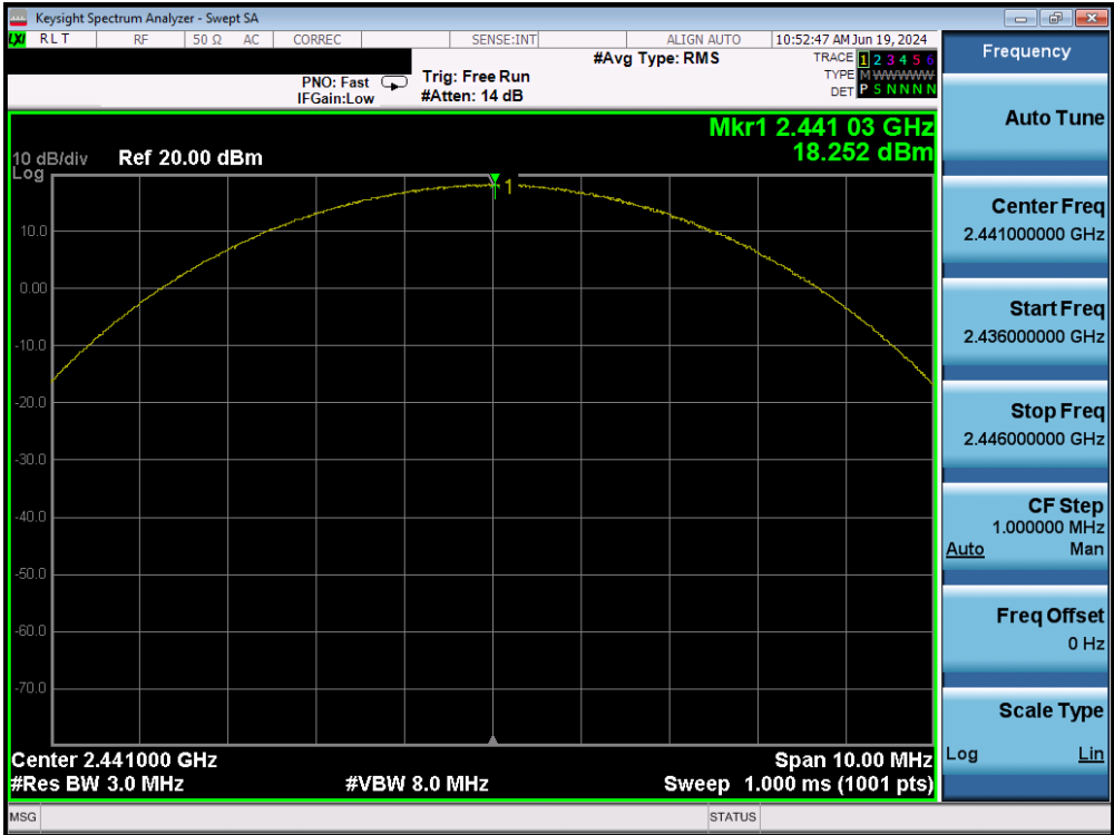
Plot 7-45. Peak Conducted Power (3Mbps – Ch. 39) – Ant 2
