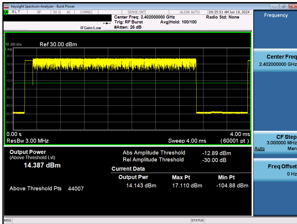
Plot 7-32. Average Conducted Power (2Mbps – Ch. 0) – Ant 1
