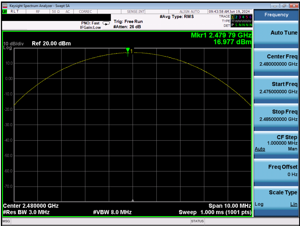
Plot 7-28. Peak Conducted Power (3Mbps – Ch. 78) – Ant 1
