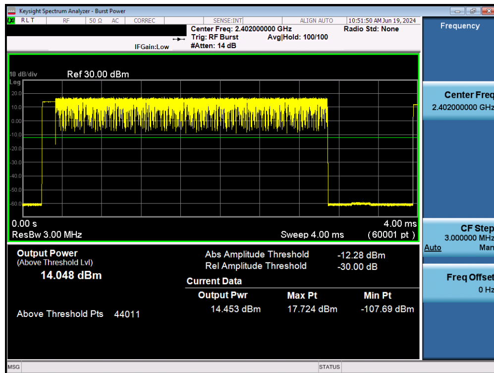
Plot 7-53. Average Conducted Power (3Mbps – Ch. 0) – Ant 2
