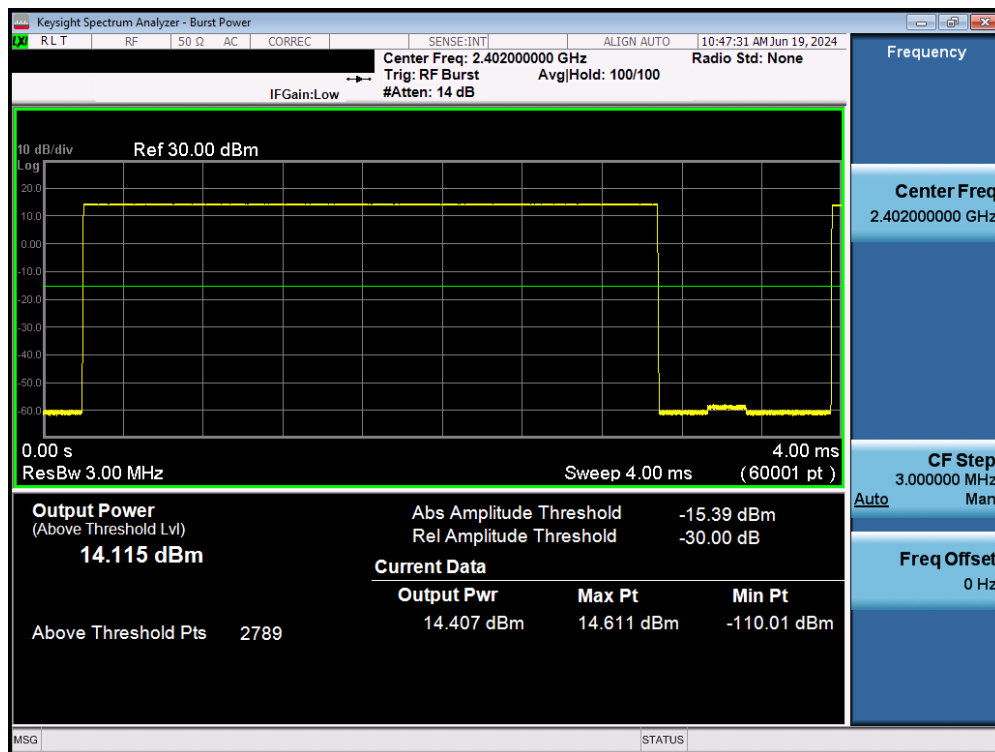
Plot 7-47. Average Conducted Power (1Mbps – Ch. 0) – Ant 2
