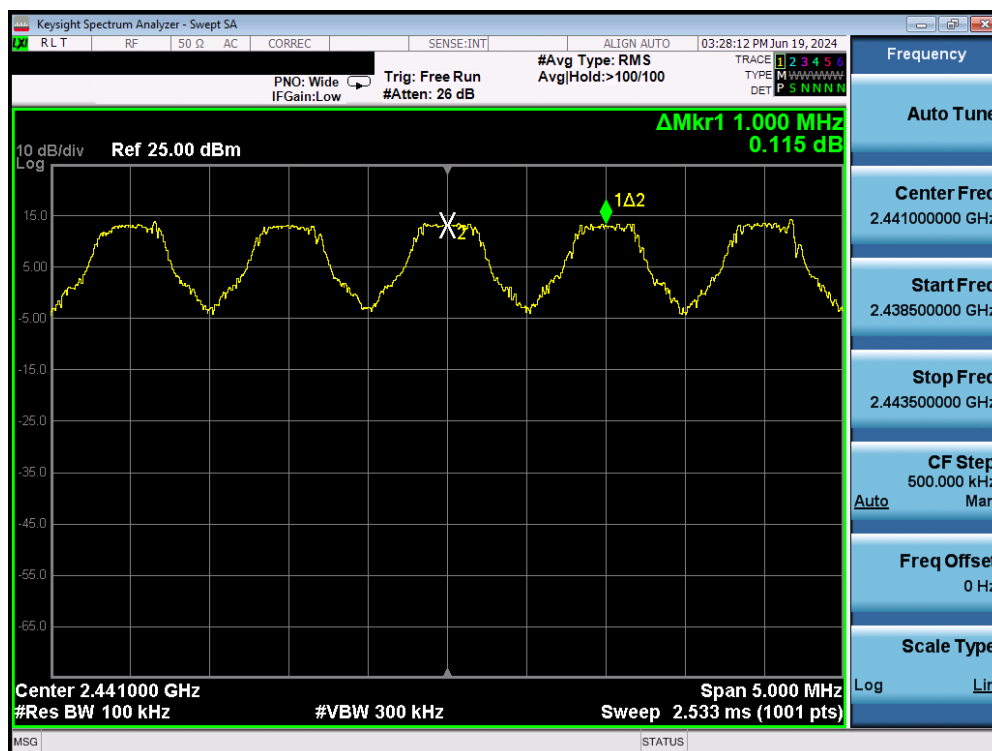
Plot 7-64. Channel Spacing Plot (Bluetooth) – Ant1
