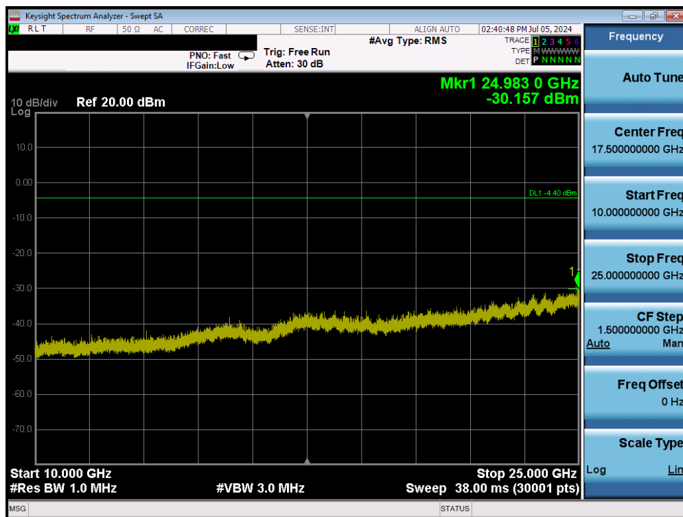
Plot 7-83. Conducted Spurious Plot (Bluetooth, 1Mbps – Ch. 78) – Ant2
