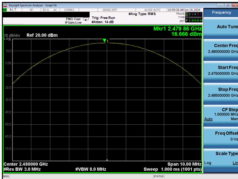
Plot 7-43. Peak Conducted Power (2Mbps – Ch. 78) – Ant 2
