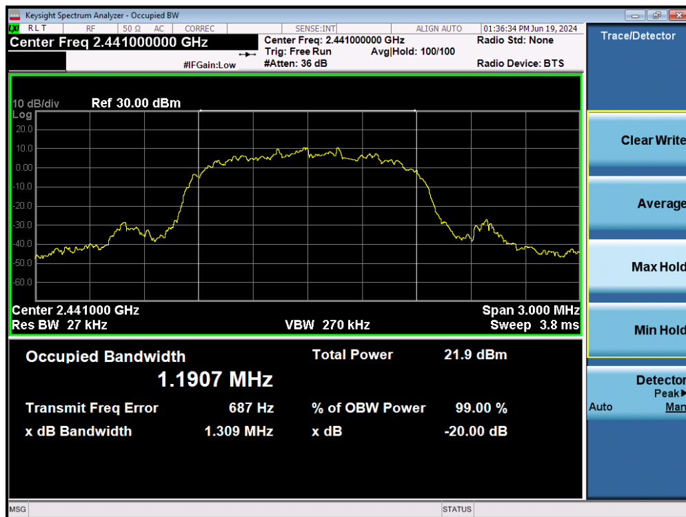
Plot 7-18. 20dB Bandwidth Plot (Bluetooth, 3Mbps – Ch. 39) – Ant 2
