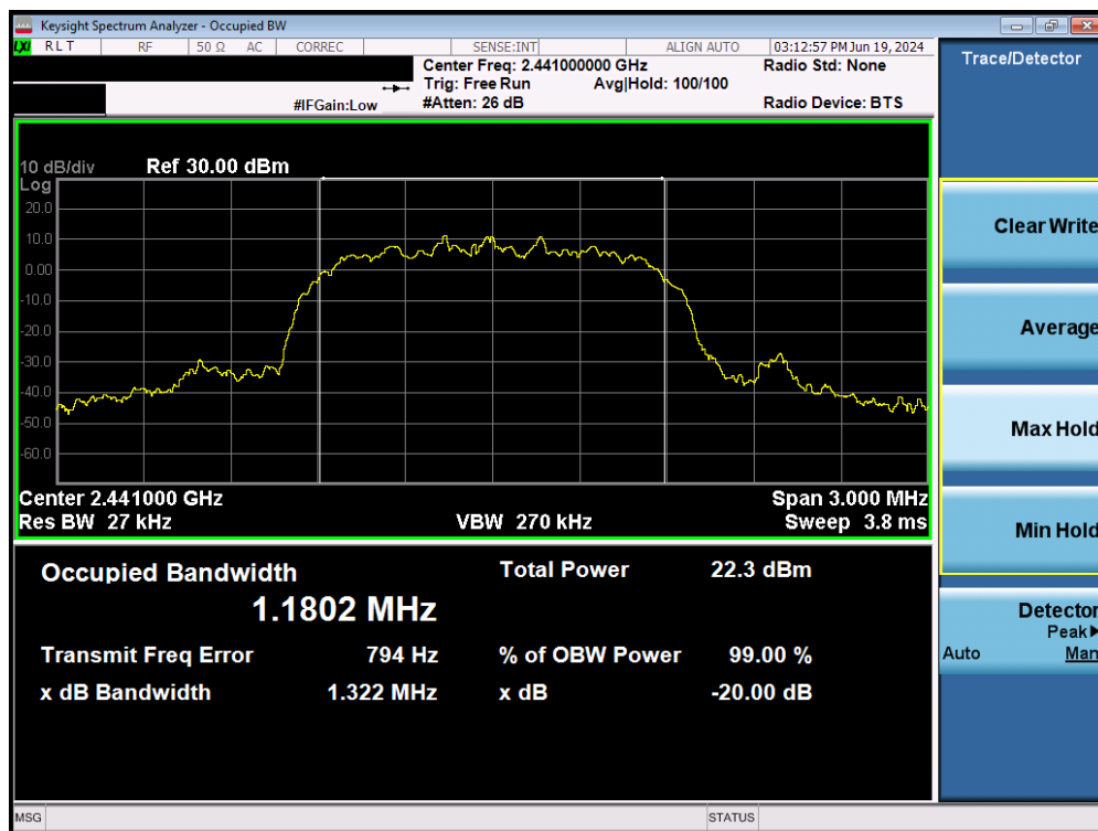
Plot 7-6. 20dB Bandwidth Plot (Bluetooth, 2Mbps – Ch. 39) – Ant 1
