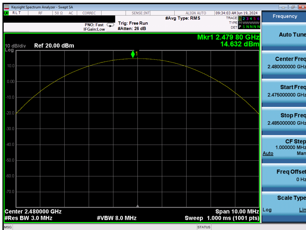
Plot 7-22. Peak Conducted Power (1Mbps – Ch. 78) – Ant 1
