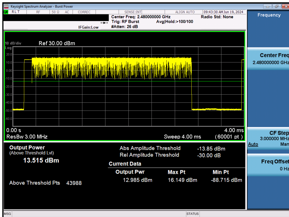
Plot 7-37. Average Conducted Power (3Mbps – Ch. 78) – Ant 1
