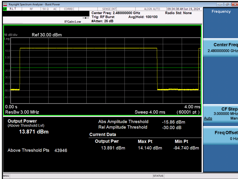
Plot 7-31. Average Conducted Power (1Mbps – Ch. 78) – Ant 1
