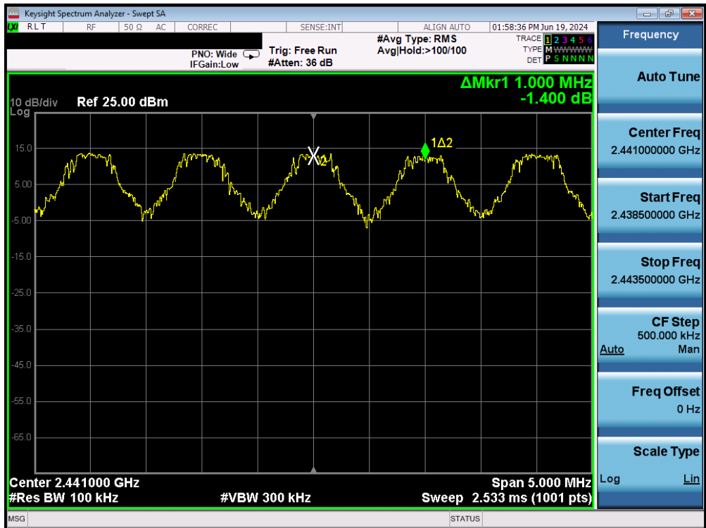
Plot 7-65. Channel Spacing Plot (Bluetooth) – Ant2
