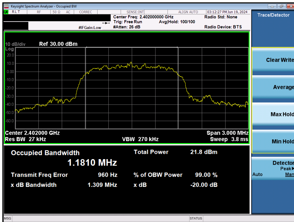
Plot 7-5. 20dB Bandwidth Plot (Bluetooth, 2Mbps – Ch. 0) – Ant 1
