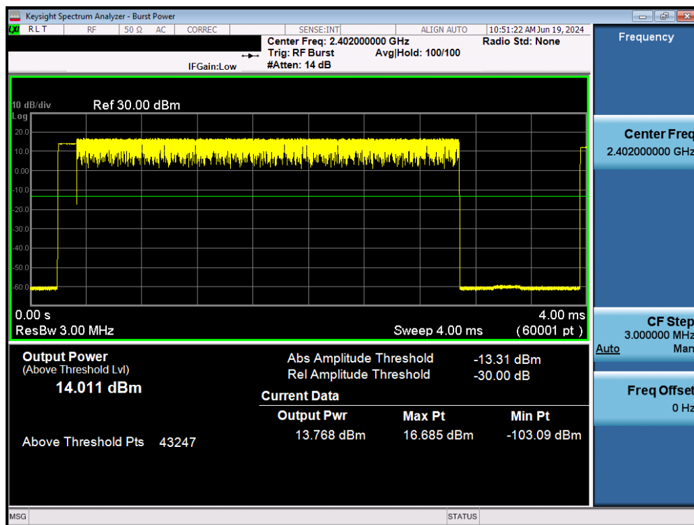
Plot 7-50. Average Conducted Power (2Mbps – Ch. 0) – Ant 2
