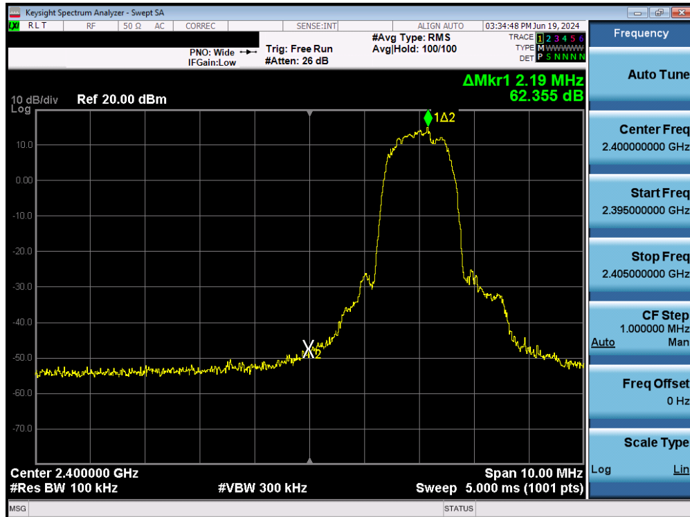
Plot 7-56. Band Edge Plot (Bluetooth with Hopping Disabled, 3 Mbps – Ch. 0) – Ant1
