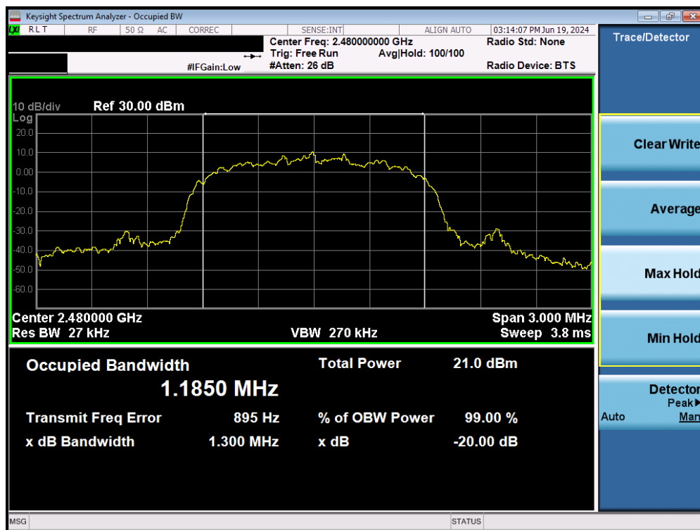
Plot 7-10. 20dB Bandwidth Plot (Bluetooth, 3Mbps – Ch. 78) – Ant 1
