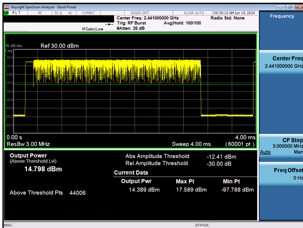
Plot 7-36. Average Conducted Power (3Mbps – Ch. 39) – Ant 1
