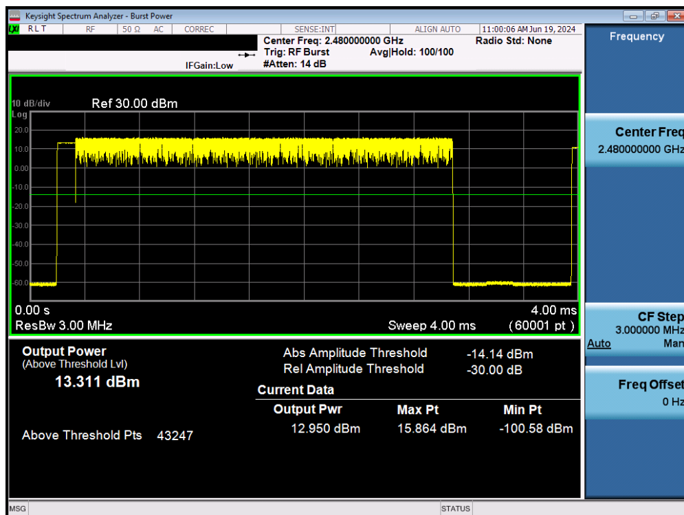
Plot 7-52. Average Conducted Power (2Mbps – Ch. 78) – Ant 2
