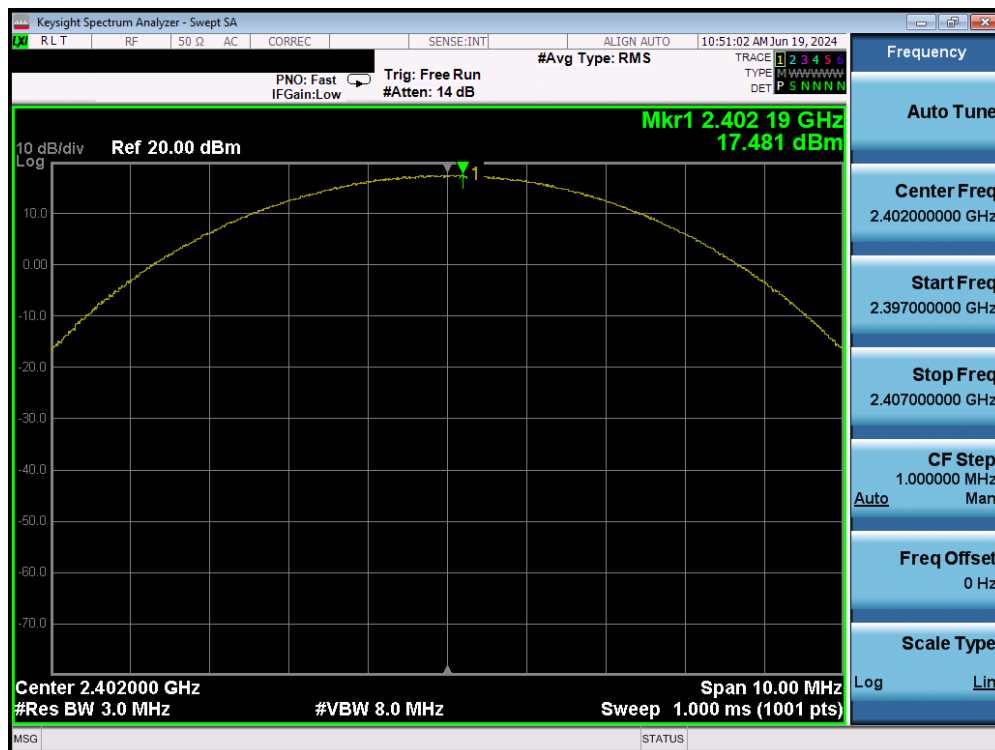
Plot 7-41. Peak Conducted Power (2Mbps – Ch. 0) – Ant 2
