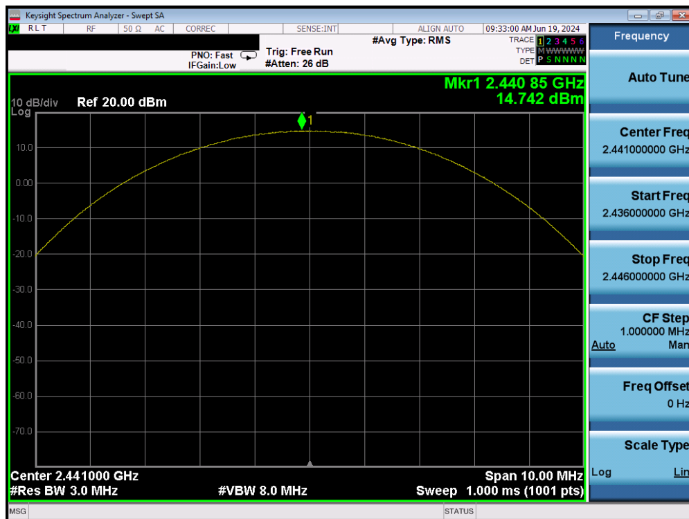
Plot 7-21. Peak Conducted Power (1Mbps – Ch. 39) – Ant 1
