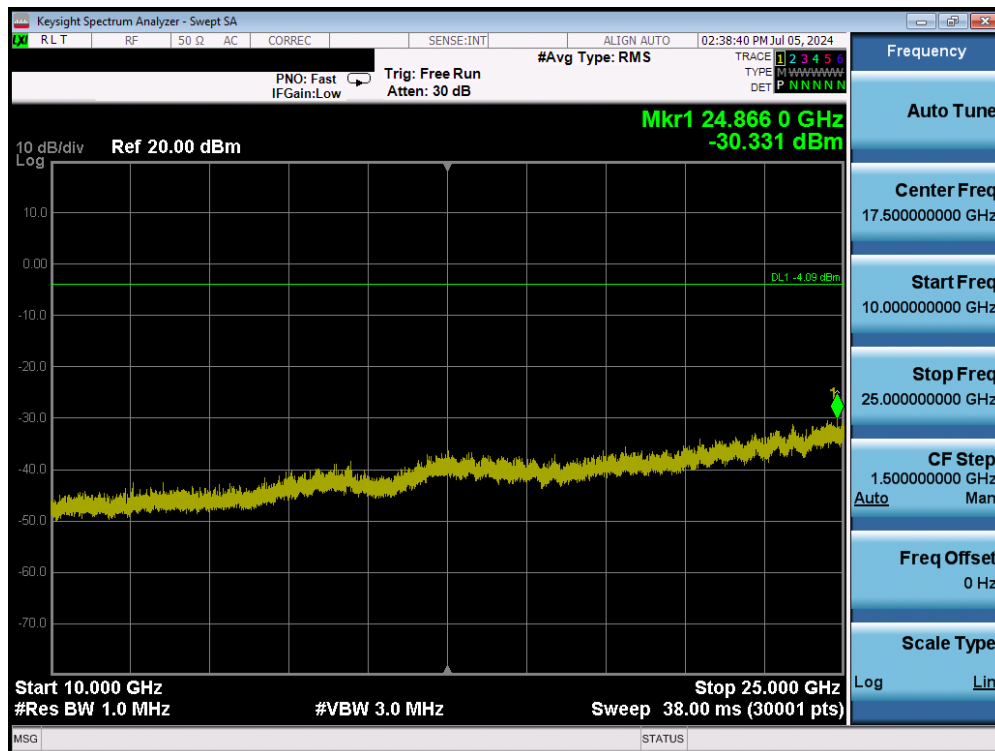
Plot 7-77. Conducted Spurious Plot (Bluetooth, 1Mbps – Ch. 78) – Ant1
