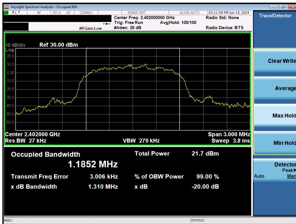
Plot 7-8. 20dB Bandwidth Plot (Bluetooth, 3Mbps – Ch. 0) – Ant 1
