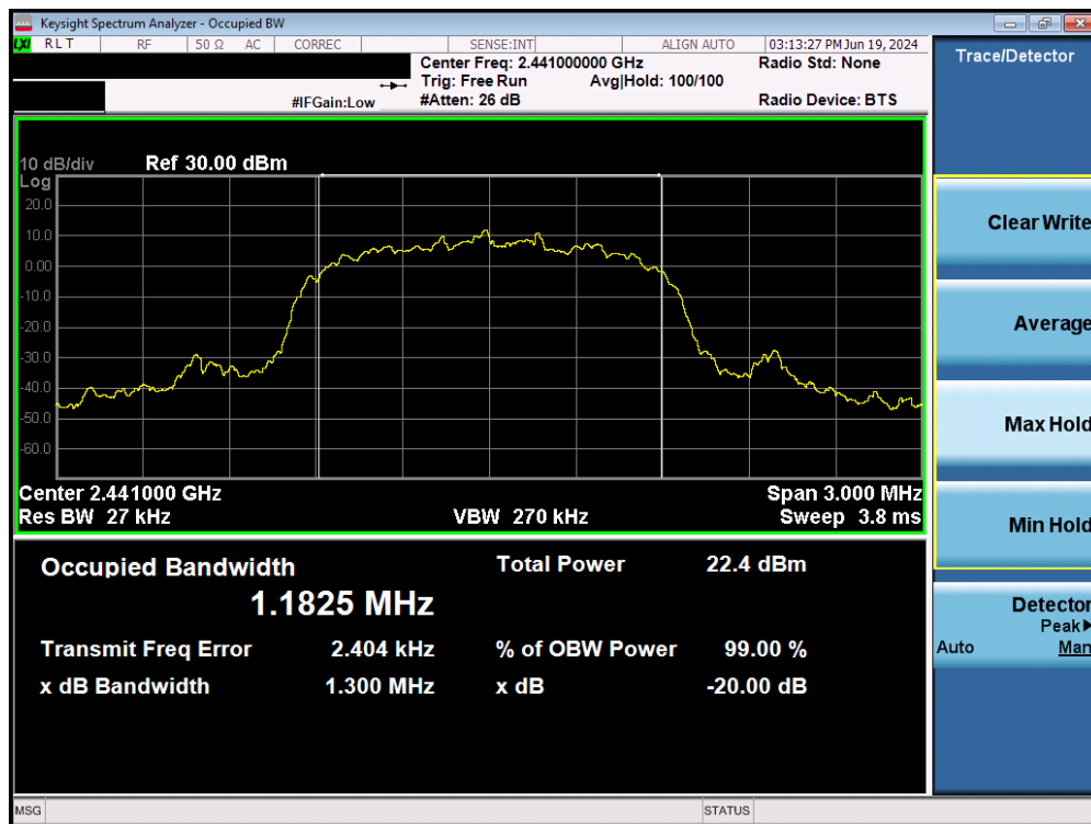
Plot 7-9. 20dB Bandwidth Plot (Bluetooth, 3Mbps – Ch. 39) – Ant 1
