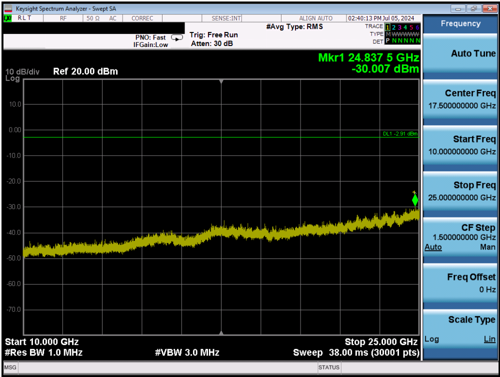
Plot 7-81. Conducted Spurious Plot (Bluetooth, 1Mbps – Ch. 39) – Ant2
