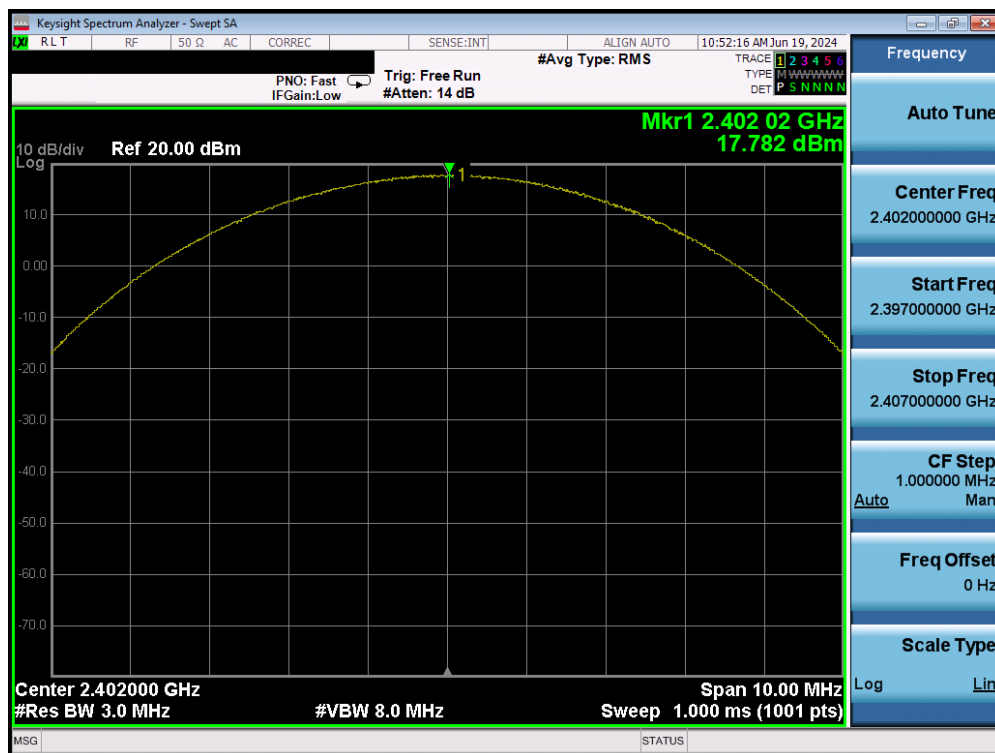
Plot 7-44. Peak Conducted Power (3Mbps – Ch. 0) – Ant 2
