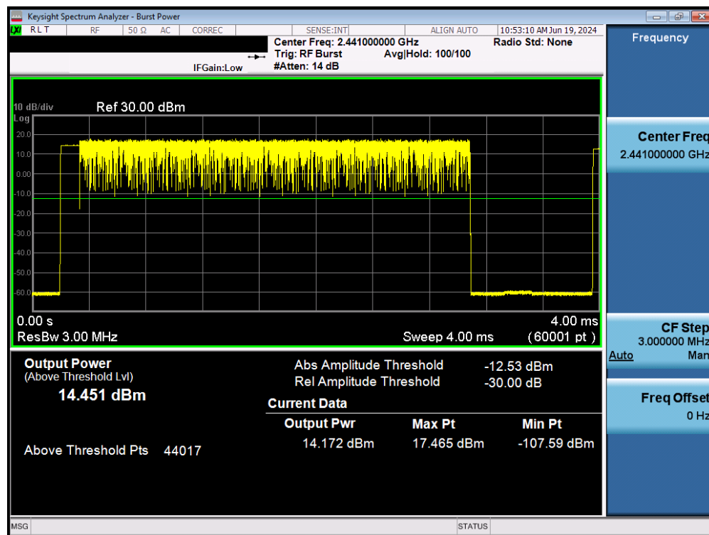
Plot 7-54. Average Conducted Power (3Mbps – Ch. 39) – Ant 2
