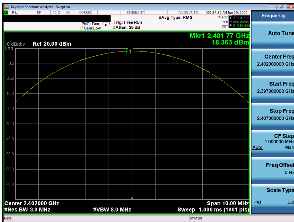
Plot 7-26. Peak Conducted Power (3Mbps – Ch. 0) – Ant 1
