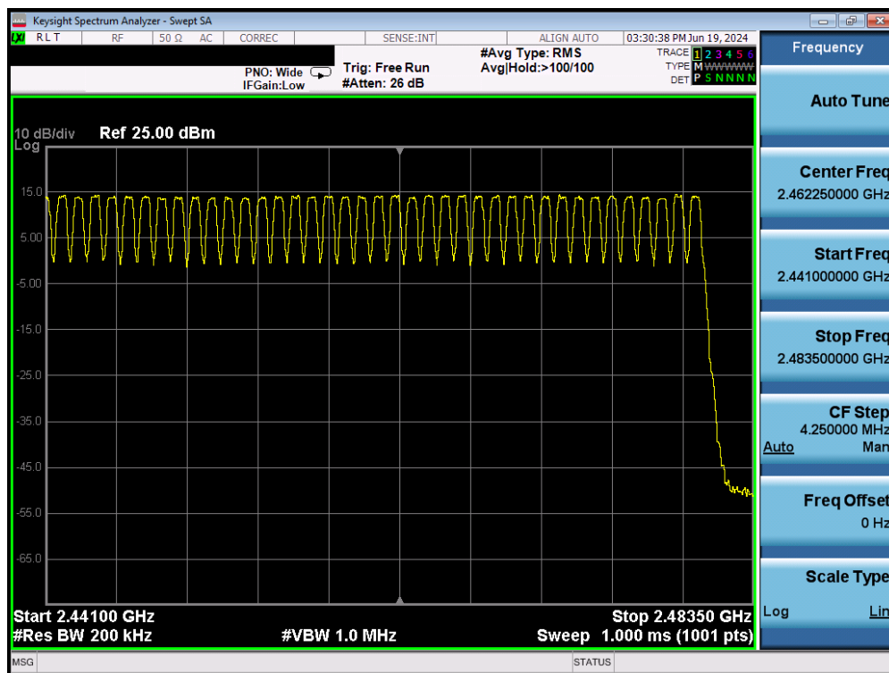
Plot 7-69. High End Spectrum Channel Hopping Plot (Bluetooth) – Ant1
