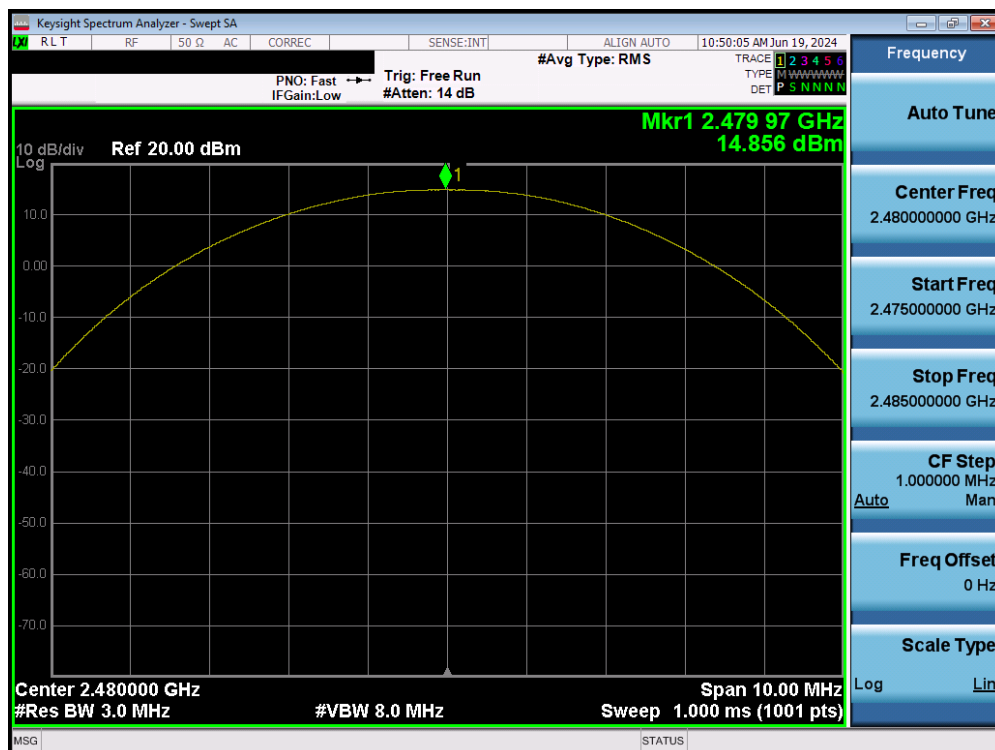
Plot 7-40. Peak Conducted Power (1Mbps – Ch. 78) – Ant 2
