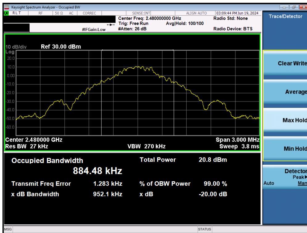
Plot 7-4. 20dB Bandwidth Plot (Bluetooth, 1Mbps – Ch. 78) – Ant 1
