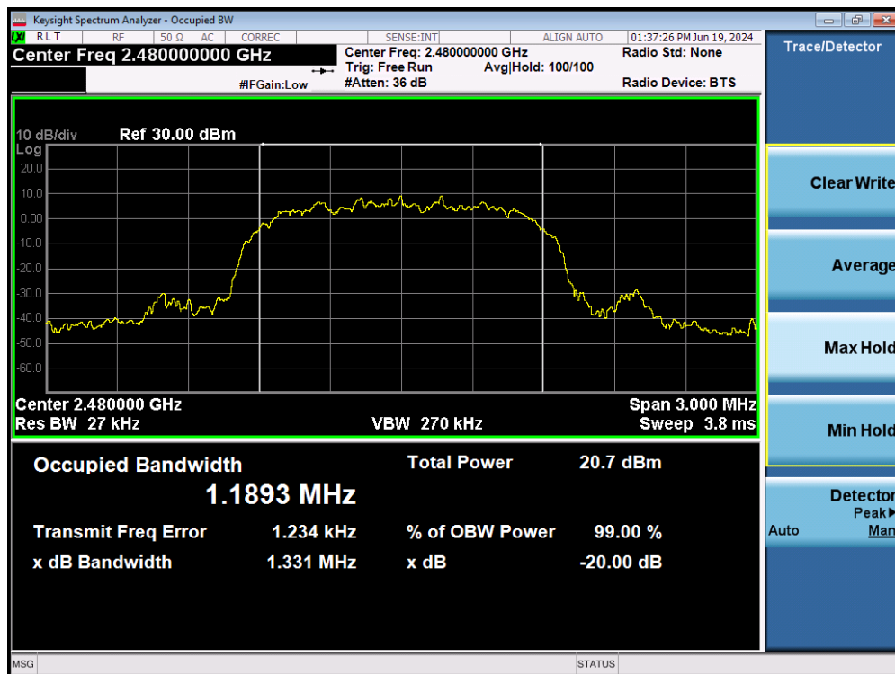
Plot 7-16. 20dB Bandwidth Plot (Bluetooth, 2Mbps – Ch. 78) – Ant 2
