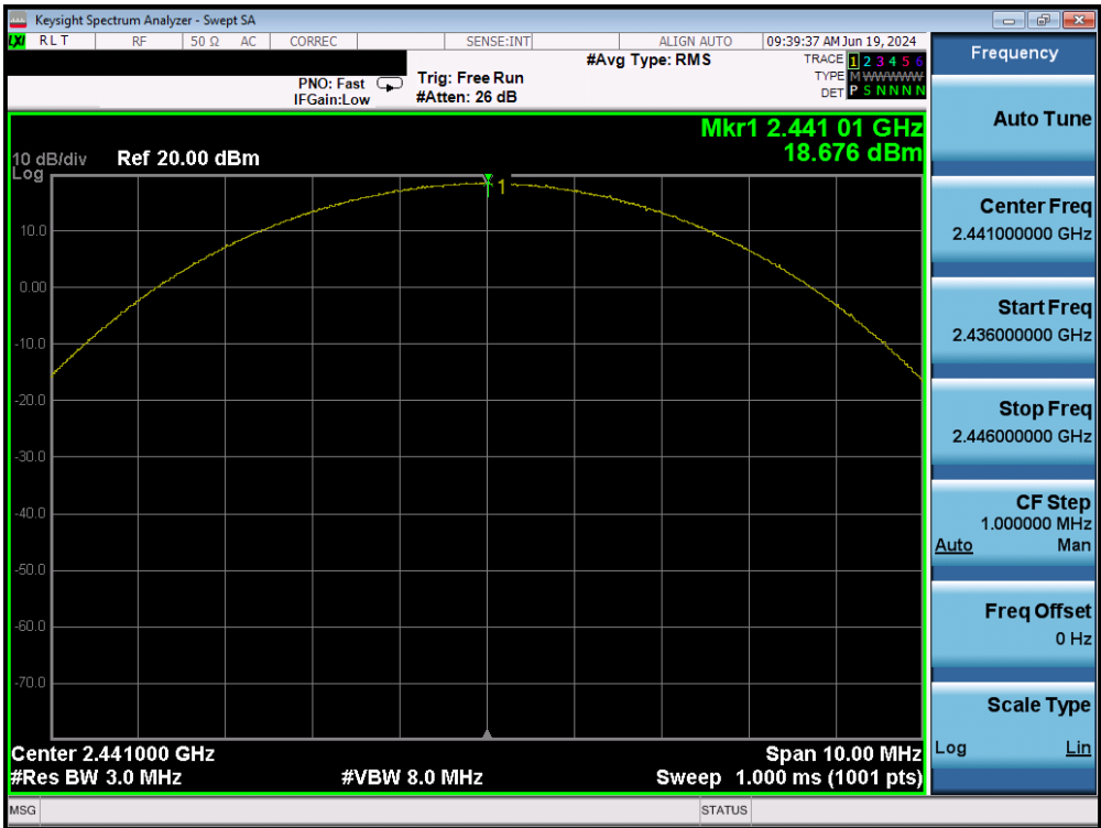
Plot 7-27. Peak Conducted Power (3Mbps – Ch. 39) – Ant 1
