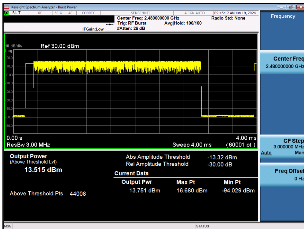
Plot 7-34. Average Conducted Power (2Mbps – Ch. 78) – Ant 1
