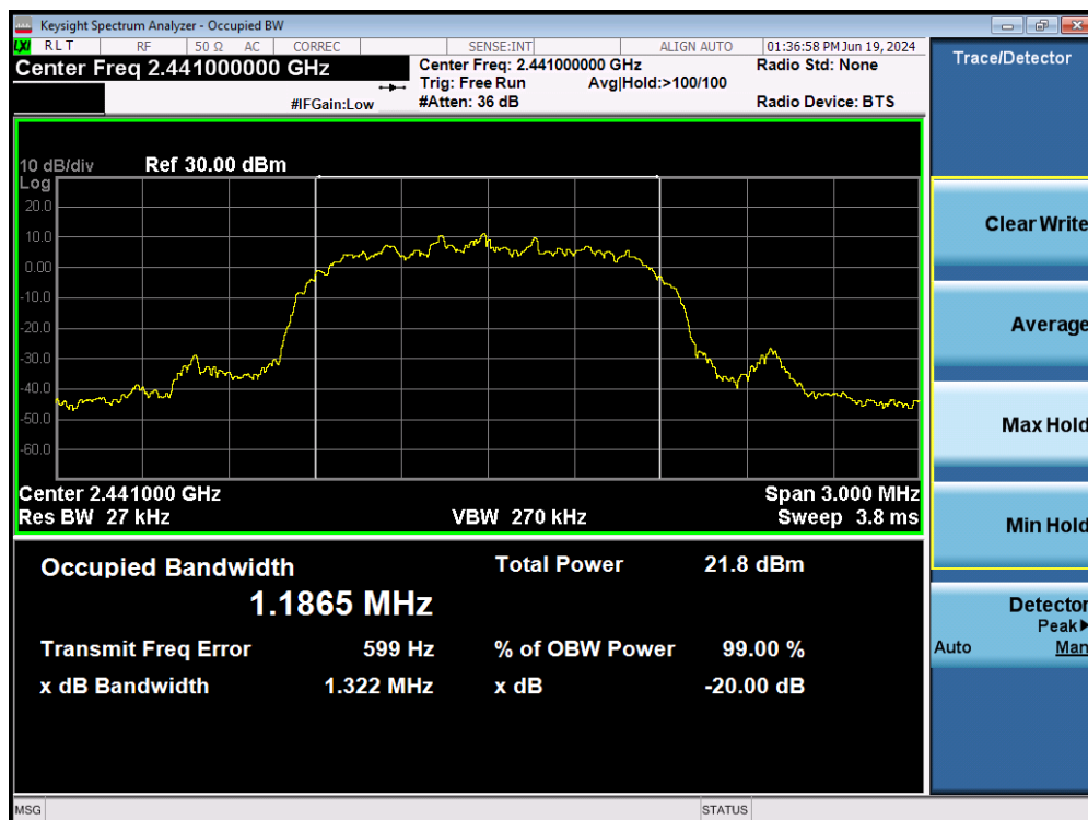
Plot 7-15. 20dB Bandwidth Plot (Bluetooth, 2Mbps – Ch. 39) – Ant 2
