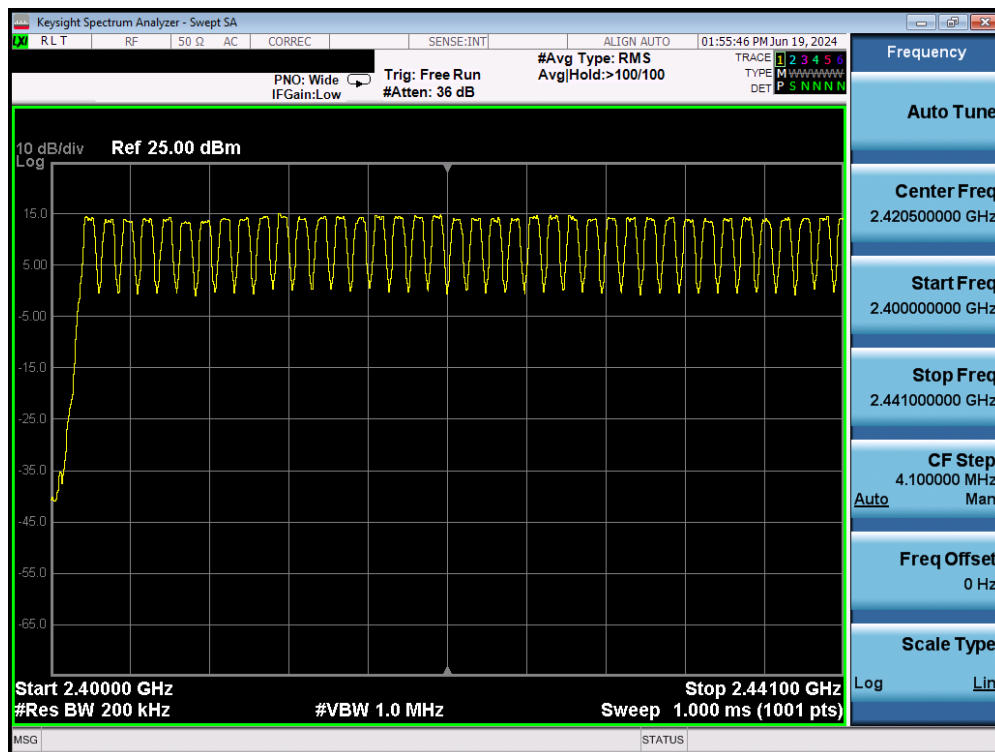
Plot 7-70. Low End Spectrum Channel Hopping Plot (Bluetooth) – Ant2
