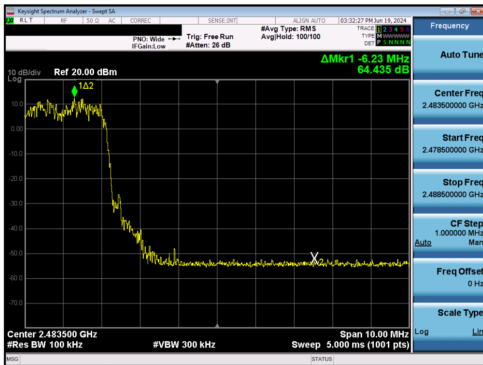
Plot 7-59. Band Edge Plot (Bluetooth with Hopping Enabled, 3 Mbps) – Ant1
