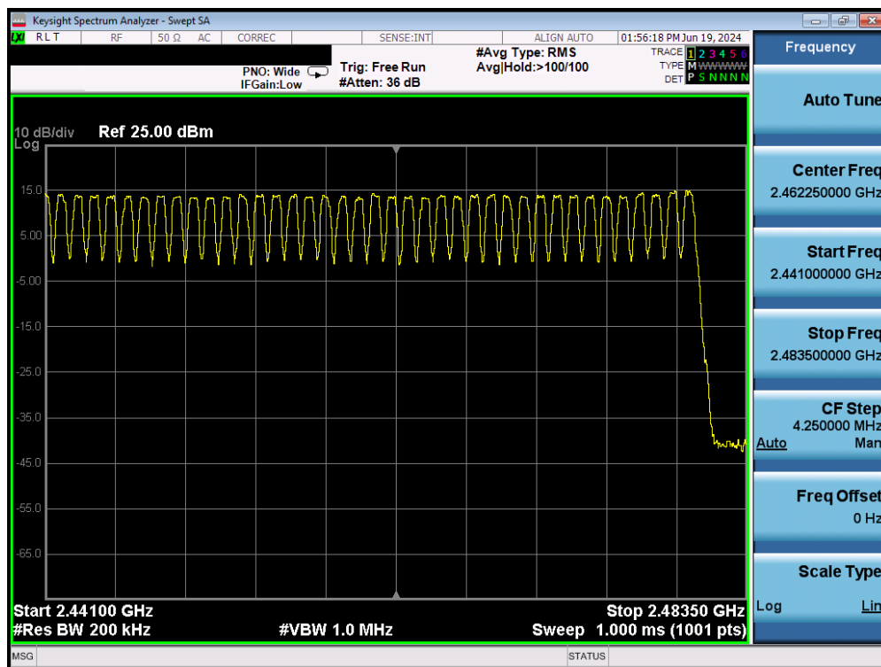
Plot 7-71. High End Spectrum Channel Hopping Plot (Bluetooth) – Ant2
