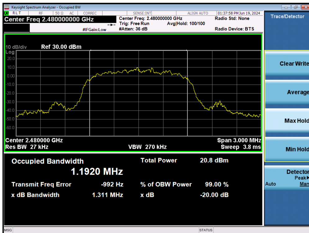
Plot 7-19. 20dB Bandwidth Plot (Bluetooth, 3Mbps – Ch. 78) – Ant 2
