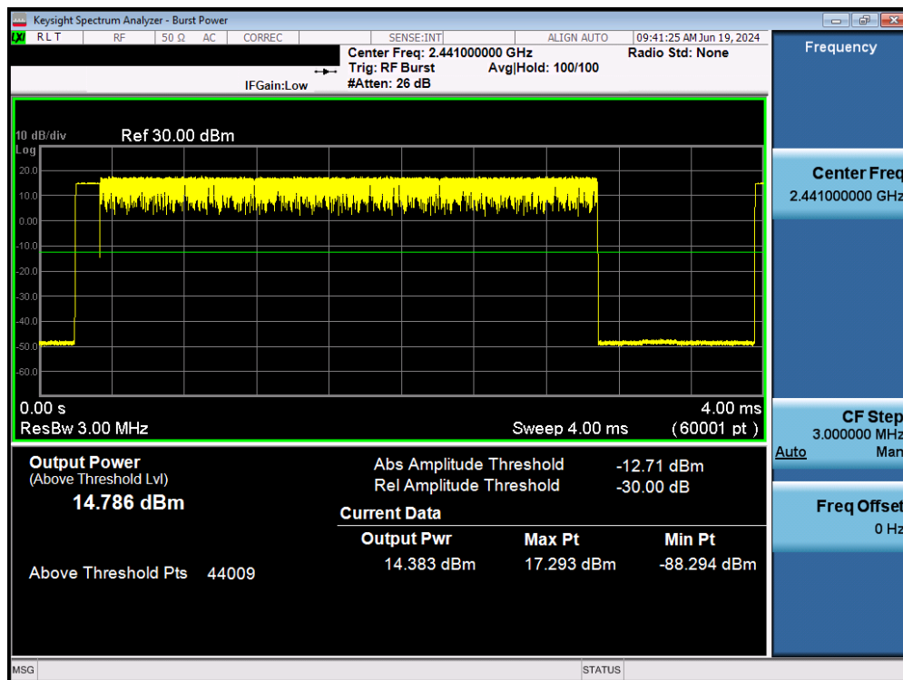
Plot 7-33. Average Conducted Power (2Mbps – Ch. 39) – Ant 1
