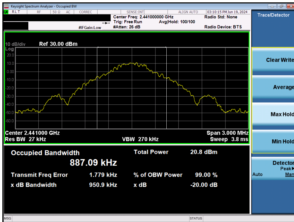
Plot 7-3. 20dB Bandwidth Plot (Bluetooth, 1Mbps – Ch. 39) – Ant 1
