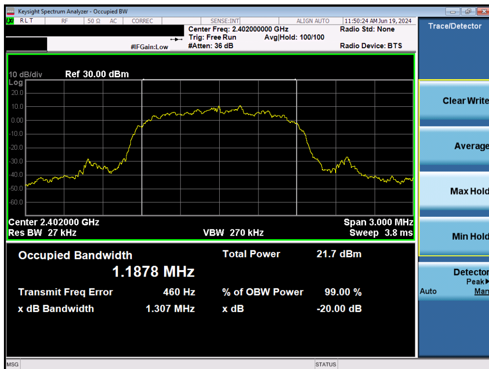
Plot 7-17. 20dB Bandwidth Plot (Bluetooth, 3Mbps – Ch. 0) – Ant 2
