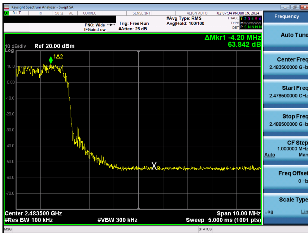
Plot 7-63. Band Edge Plot (Bluetooth with Hopping Enabled, 3 Mbps) – Ant2
