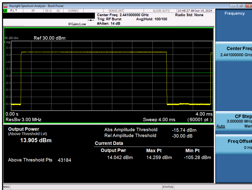
Plot 7-48. Average Conducted Power (1Mbps – Ch. 39) – Ant 2
