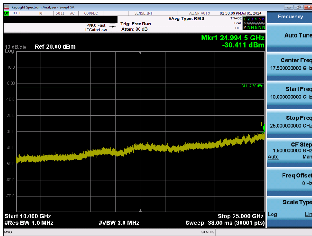
Plot 7-75. Conducted Spurious Plot (Bluetooth, 1Mbps – Ch. 39) – Ant1
