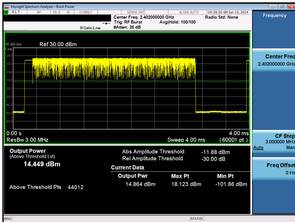
Plot 7-35. Average Conducted Power (3Mbps – Ch. 0) – Ant 1
