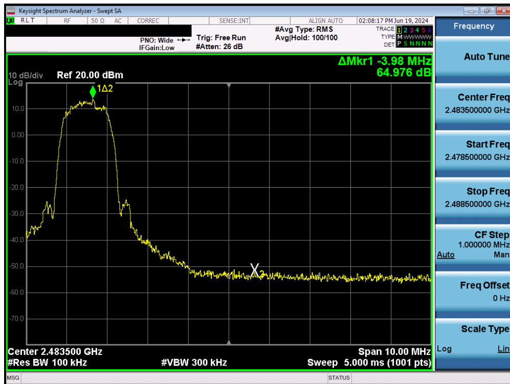
Plot 7-61. Band Edge Plot (Bluetooth with Hopping Disabled, 3 Mbps – Ch. 78) – Ant2
