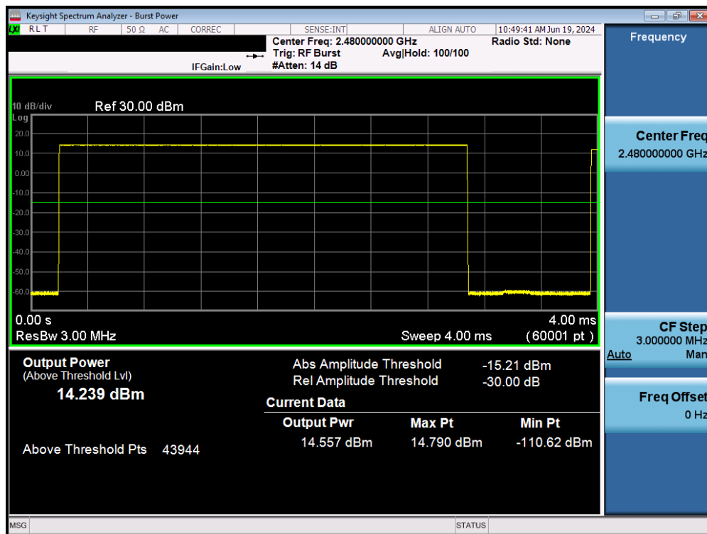
Plot 7-49. Average Conducted Power (1Mbps – Ch. 78) – Ant 2
