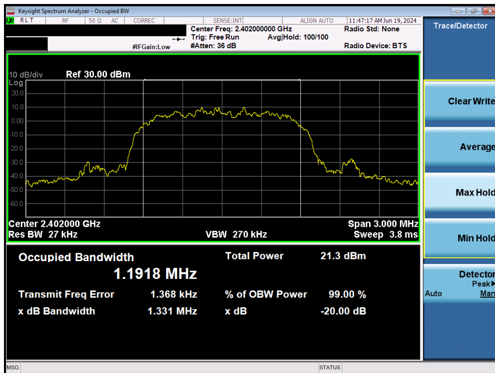
Plot 7-14. 20dB Bandwidth Plot (Bluetooth, 2Mbps – Ch. 0) – Ant 2
