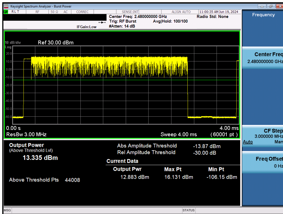
Plot 7-55. Average Conducted Power (3Mbps – Ch. 78) – Ant 2
