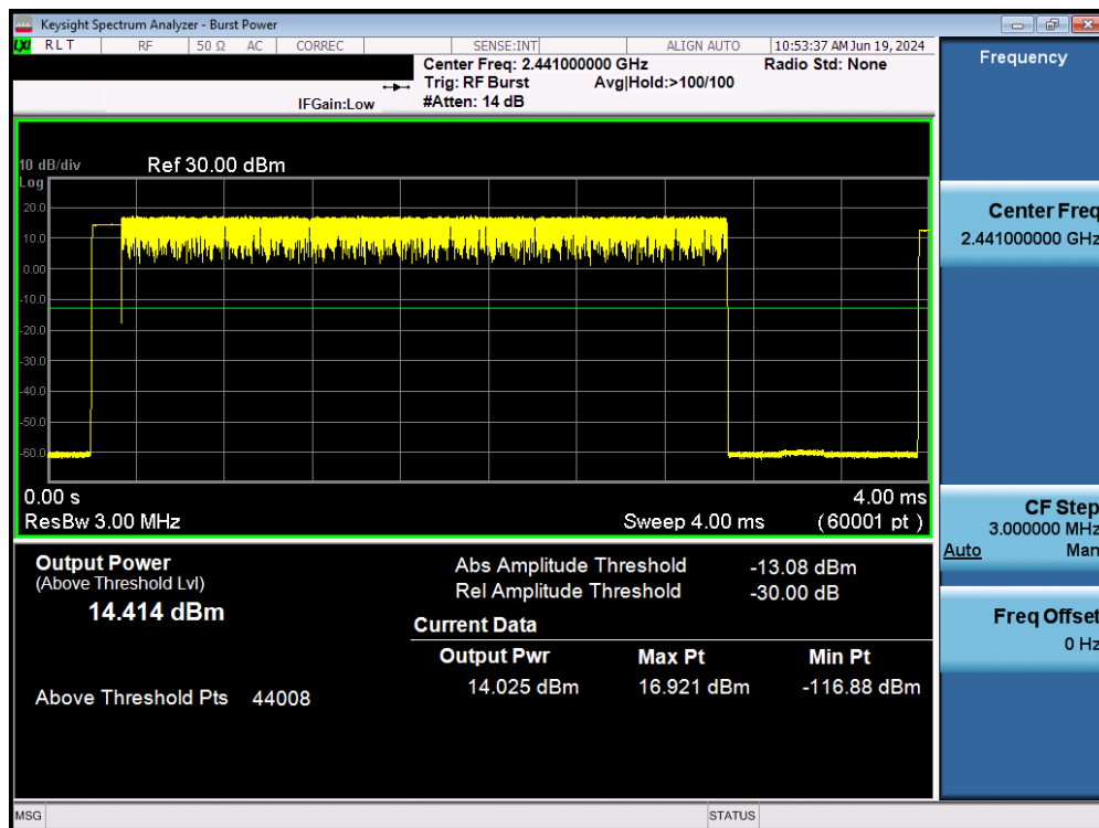
Plot 7-51. Average Conducted Power (2Mbps – Ch. 39) – Ant 2
