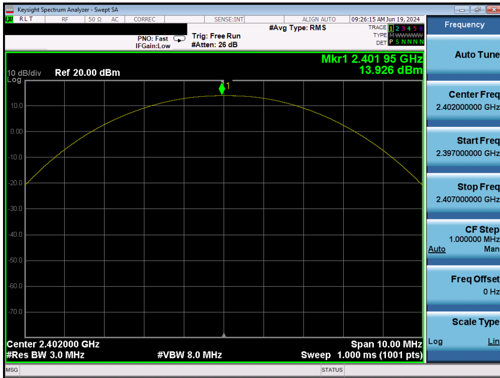
Plot 7-20. Peak Conducted Power (1Mbps – Ch. 0) – Ant 1
