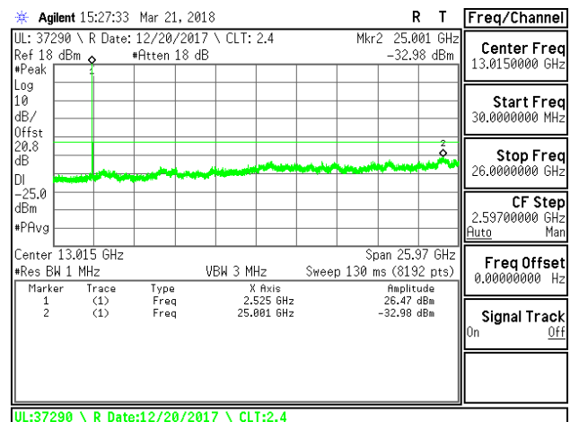
LTE B7 20MHz 16QAM Middle Channel RB1-0
