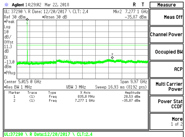
LTE B5 1.4MHz 16QAM Middle Channel B1-0
