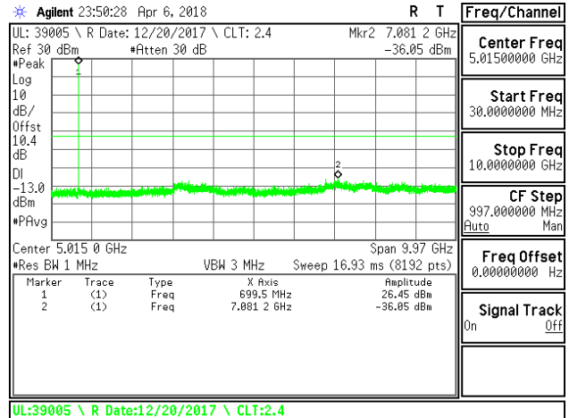
LTE B12 5MHz 16QAM Low Channel RB1-0
