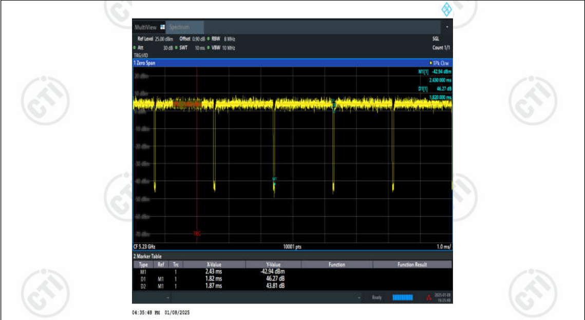
NTNV-11N40MIMO-Ant2-5230
