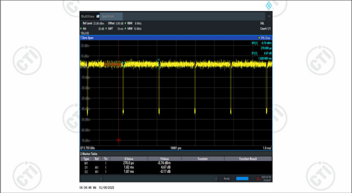
NTNV-11N40MIMO-Ant2-5755
