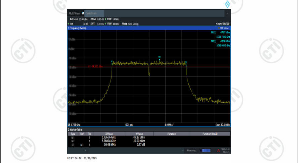
11AC40SISO-Ant2-5755-PASS
