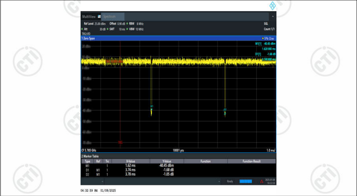
NTNV-11N20MIMO-Ant2-5785
