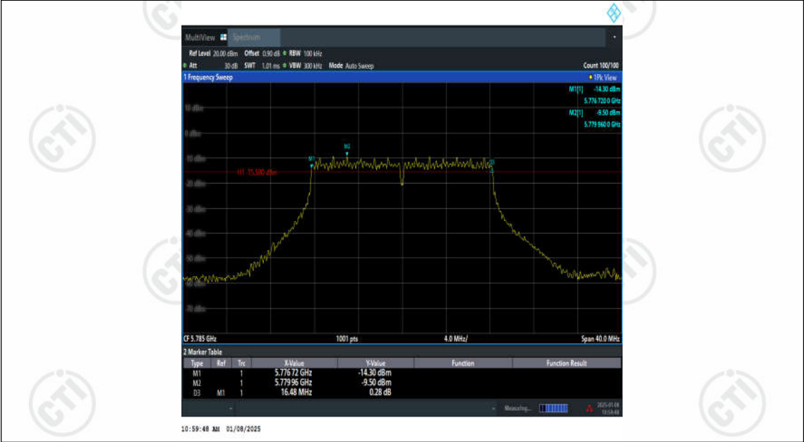
11A-Ant2-5785-PASS
