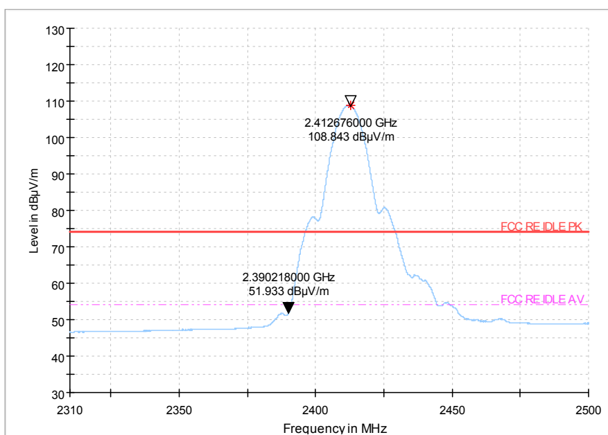
Fig 82. Radiated emission (Power): 802.11b, low channel
