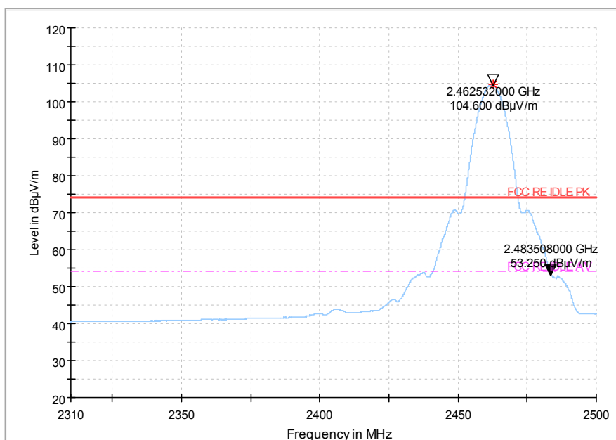
Fig 78. Radiated emission (Power): 802.11b, high channel
