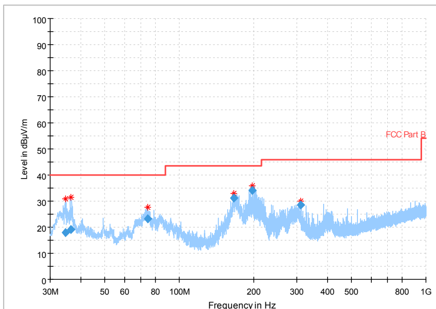
Fig 79. Radiated Spurious Emission (802.11b,Ch11,30MHz~1GHz)
