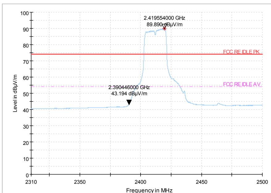
Fig 67. Radiated emission (Power): 802.11n, low channel
