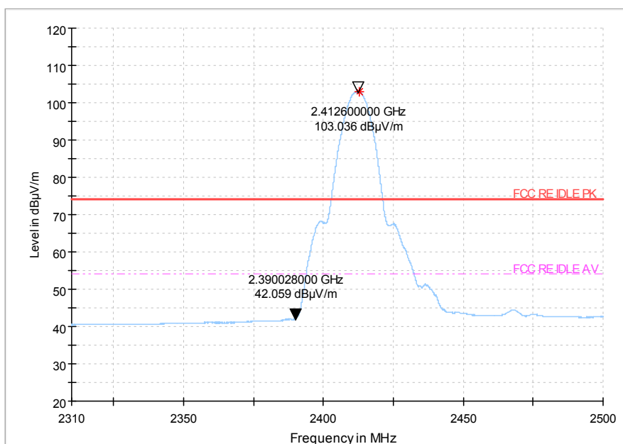
Fig 77. Radiated emission (Power): 802.11b, low channel
