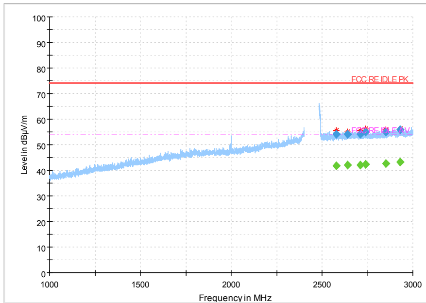
Fig 80. Radiated Spurious Emission (802.11b,Ch11,1GHz~3GHz)
