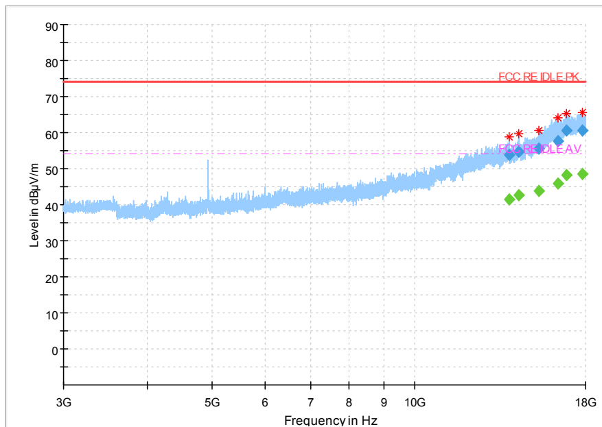
Fig 81. Radiated Spurious Emission (802.11b,Ch11,3GHz~18GHz)
