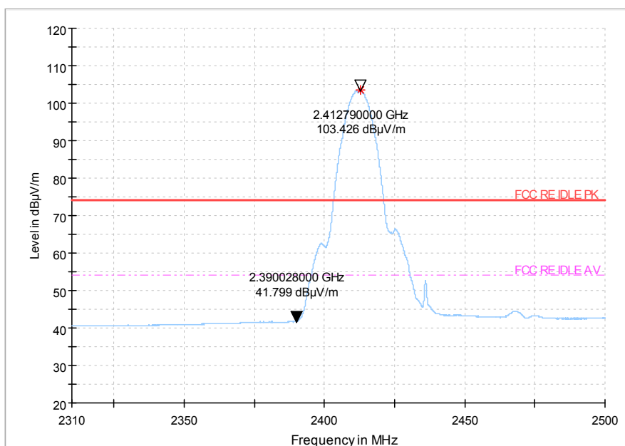
Fig 57. Radiated emission (Power): 802.11b, low channel
