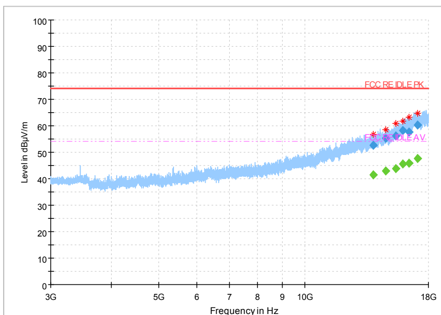
Fig 76. Radiated Spurious Emission (802.11 n-40MHz, Ch3, 3GHz~18GHz)
