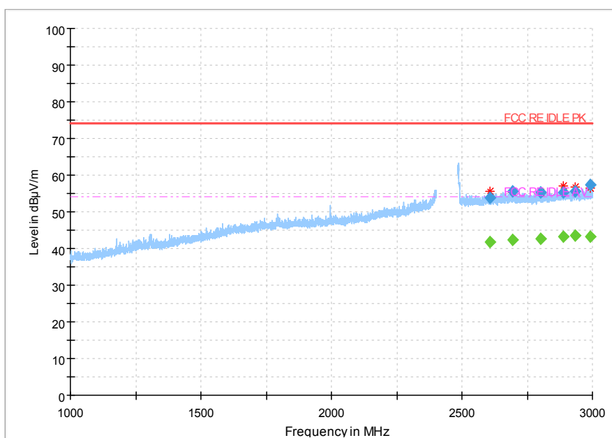
Fig 85. Radiated Spurious Emission (802.11b,Ch11,1GHz~3GHz)
