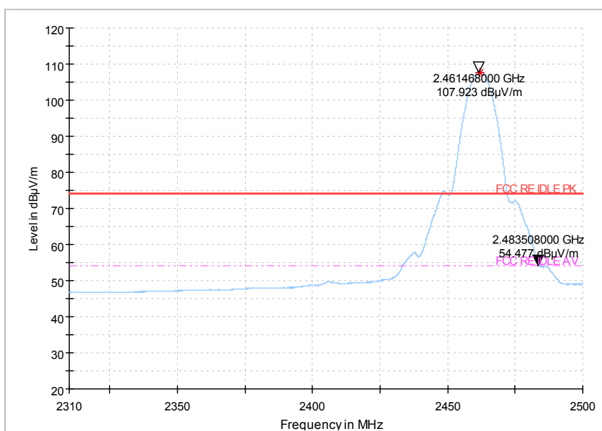
Fig 83. Radiated emission (Power): 802.11b, high channel
