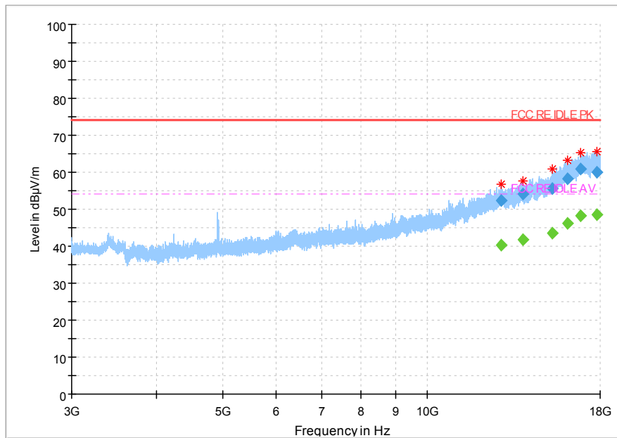
Fig 86. Radiated Spurious Emission (802.11b,Ch11,3GHz~18GHz)
