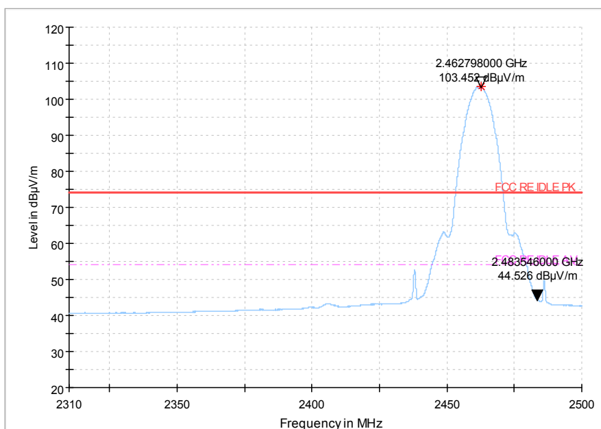
Fig 58. Radiated emission (Power): 802.11b, high channel
