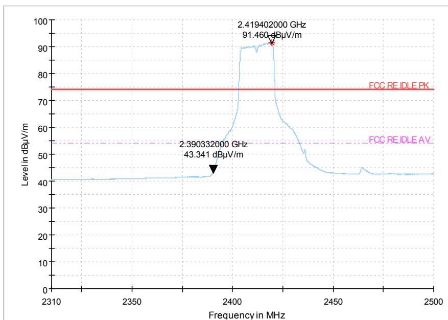
Fig 62. Radiated emission (Power): 802.11g, low channel
