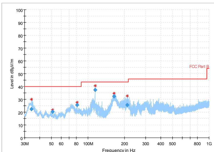
Fig 84. Radiated Spurious Emission (802.11b,Ch11,30MHz~1GHz)
