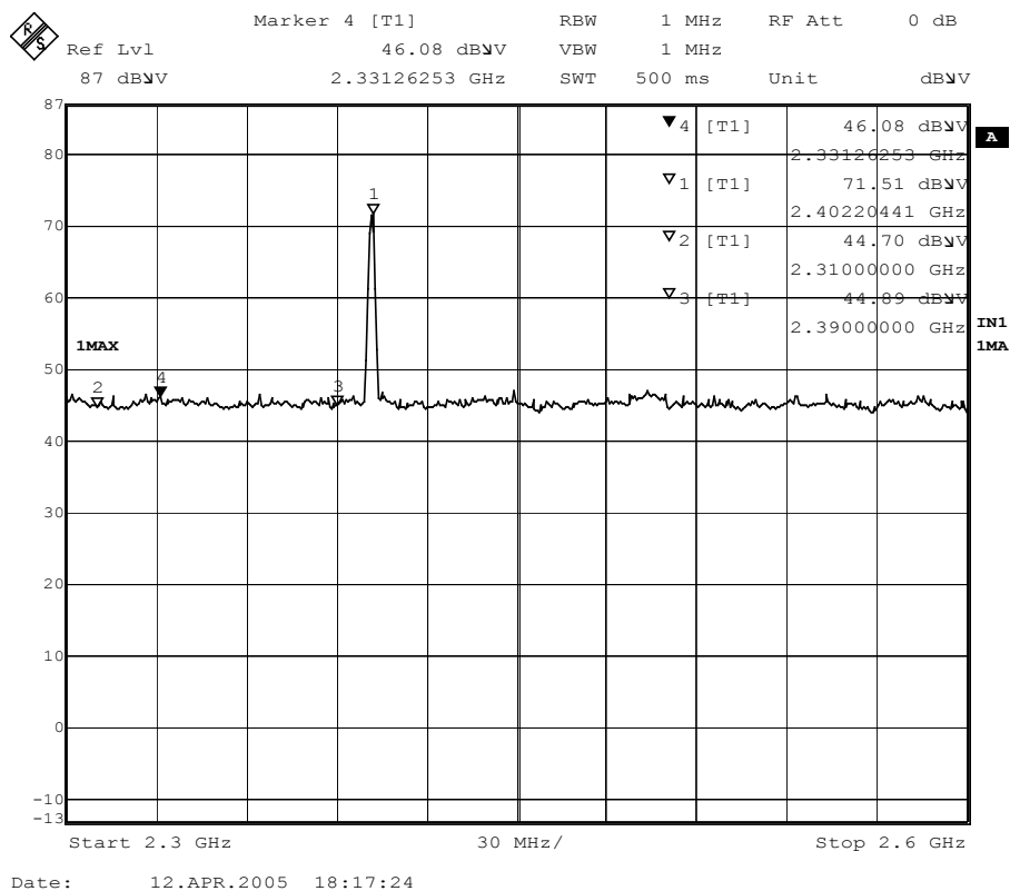
Figure Channel 00: (Horizontal)
