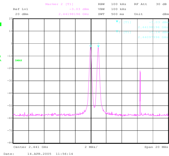
Channel 39 2441MHz
