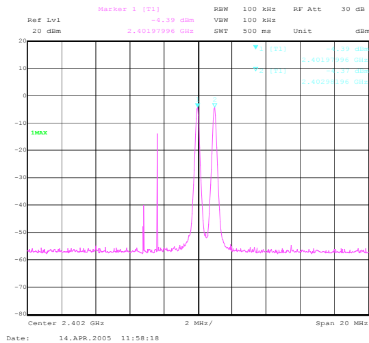
Channel 00 2402MHz
