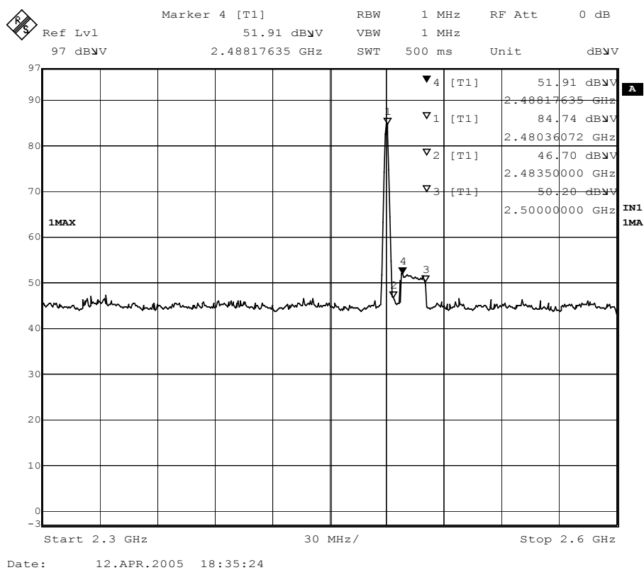
Figure Channel 78: (Vertical)
