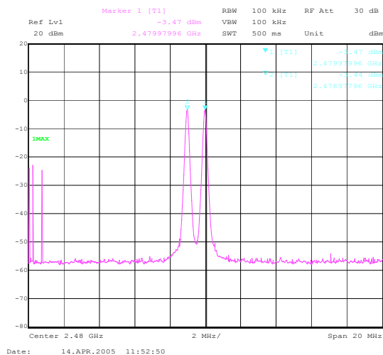
Channel 78 2480 MHz
