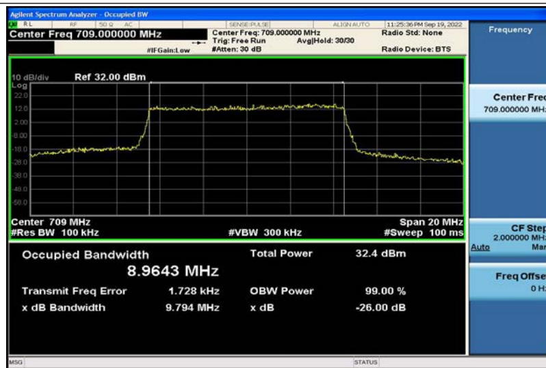
Band17-10MHz-QPSK-23780-50RB#0-8.9643
