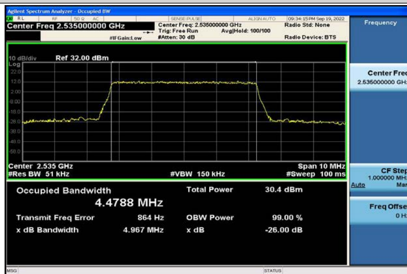
Band7-5MHz-16QAM-21100-25RB#0-4.4788
