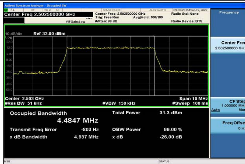
Band7-5MHz-QPSK-20775-25RB#0-4.4847
