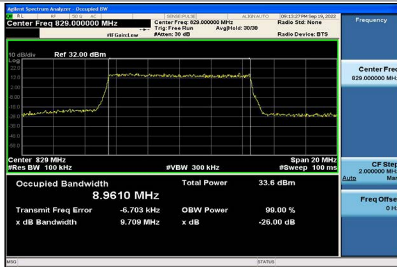
Band5-10MHz-16QAM-20450-50RB#0-8.9610
