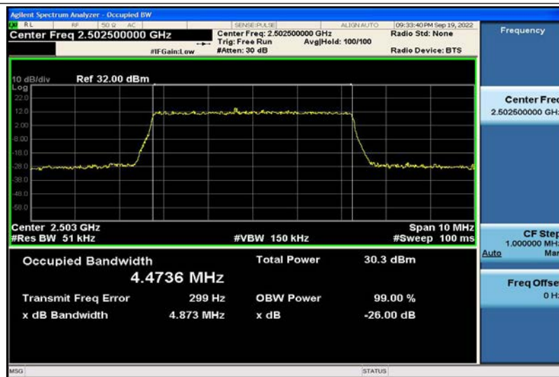
Band7-5MHz-16QAM-20775-25RB#0-4.4736
