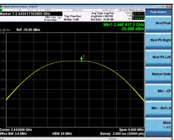
Output Power, Channel 19, neg40dBm
