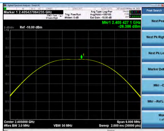
Output Power, Channel 11, neg40dBm
