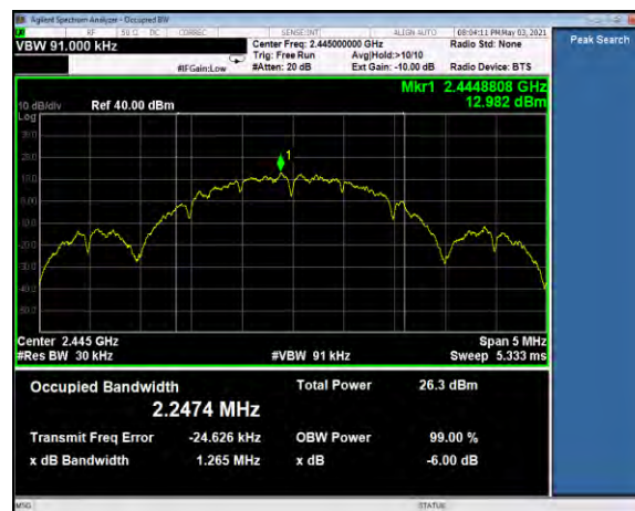
99% BW, Channel 19, neg4dBm
