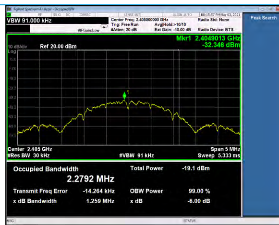
99% BW, Channel 11, neg40dBm
