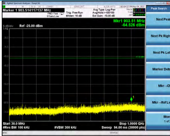
Conducted TX Spurious 30-1000 MHz Channel 25, neg4dBm
