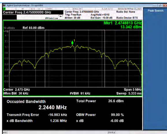
99% BW Channel 25, neg4dBm
