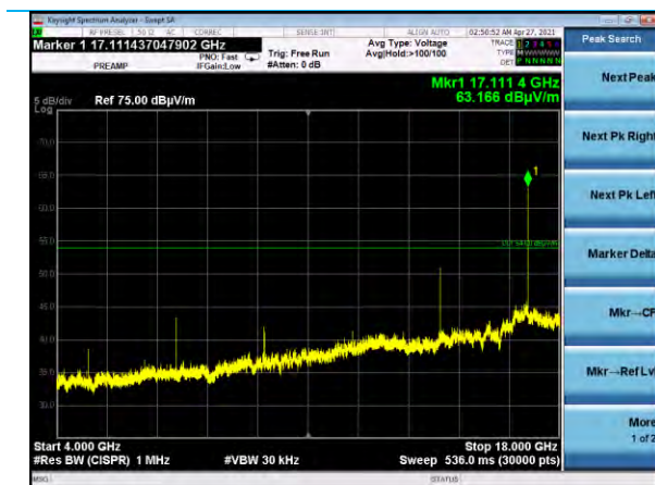
4-18 GHz, Horizontal Antenna Vertical EUT, Channel 19
