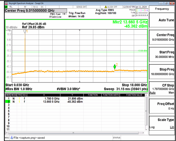
13A_n66 (30MHz-18GHz) 15M DFT-s-OFDM BPSK Inner_1RB_Right High
