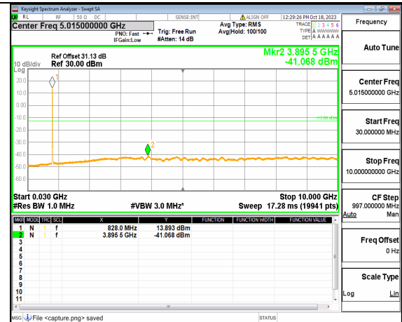
2A_n5 (30MHz-10GHz) 10M DFT-s-OFDM QPSK Outer_Full Low
