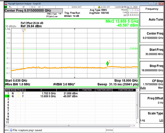
13A_n66 (30MHz-18GHz) 15M DFT-s-OFDM QPSK Inner_1RB_Right Mid
