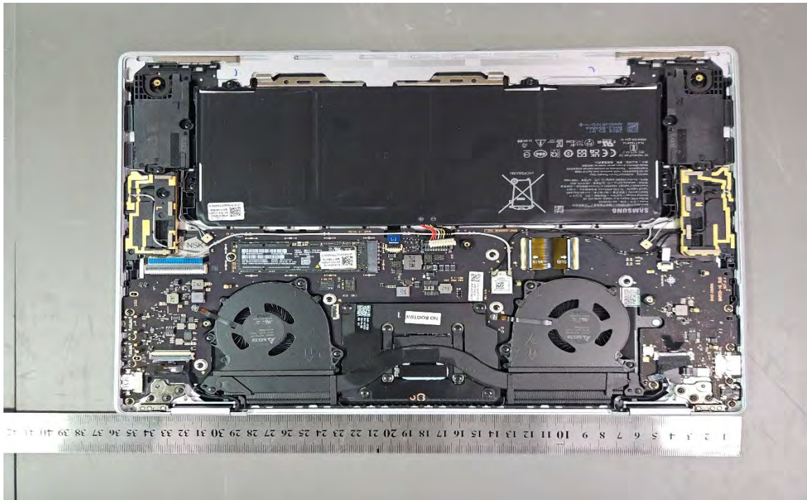
Internal EUT#10
