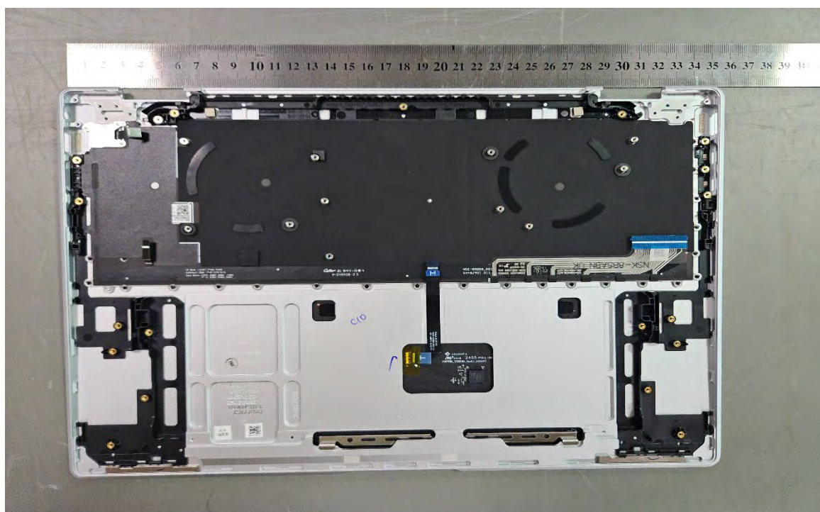
Internal EUT#9
