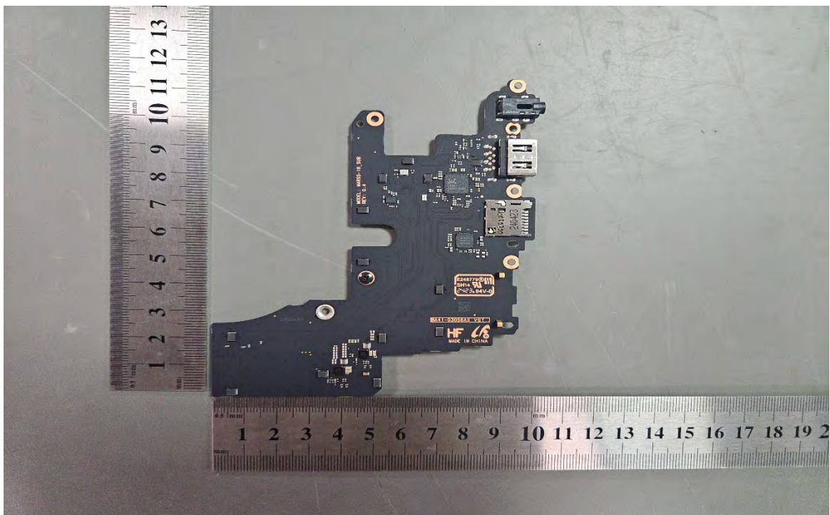
Internal EUT#21
