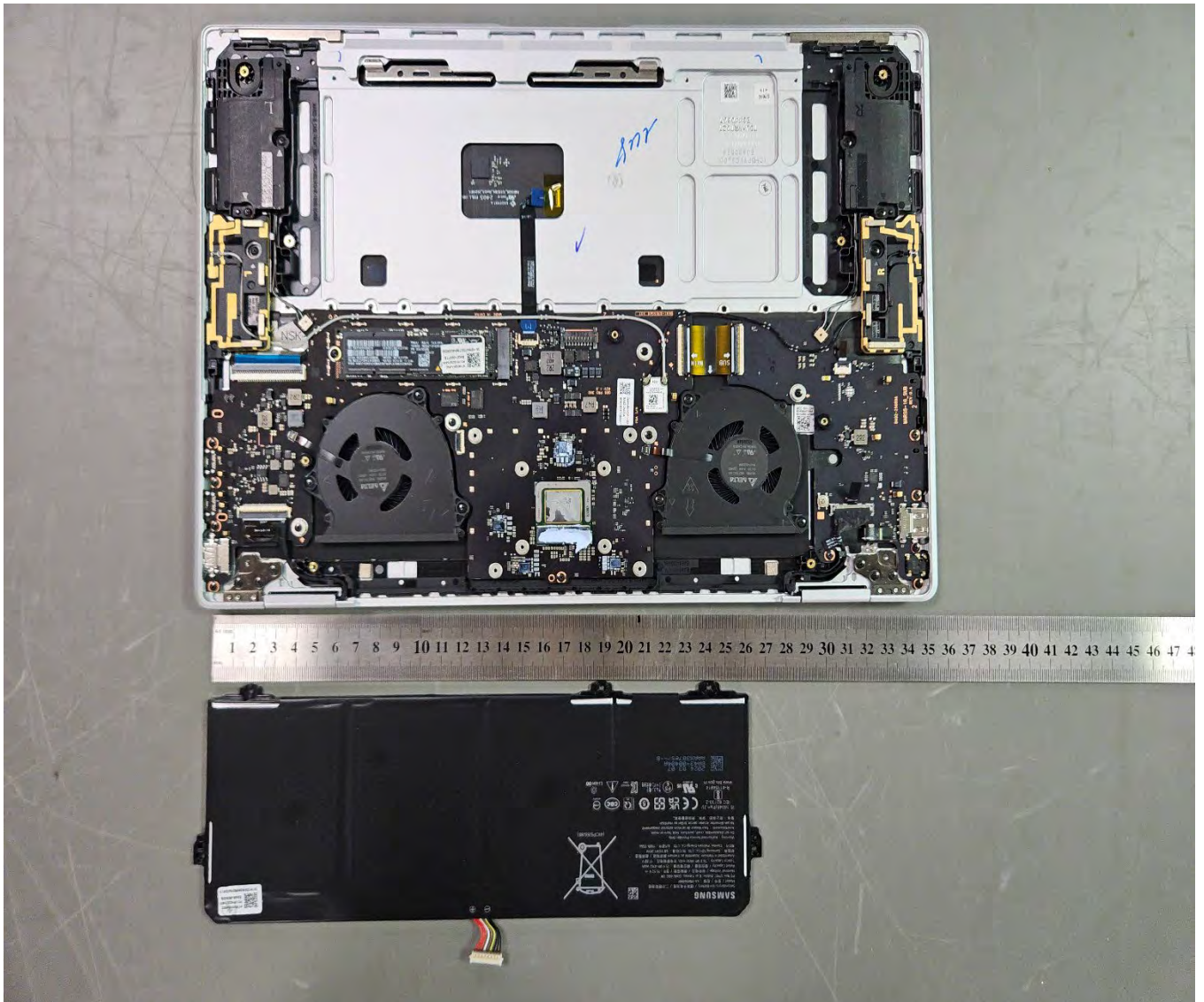
Internal EUT#15
