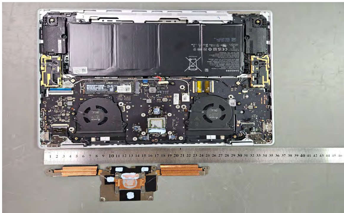
Internal EUT#1
