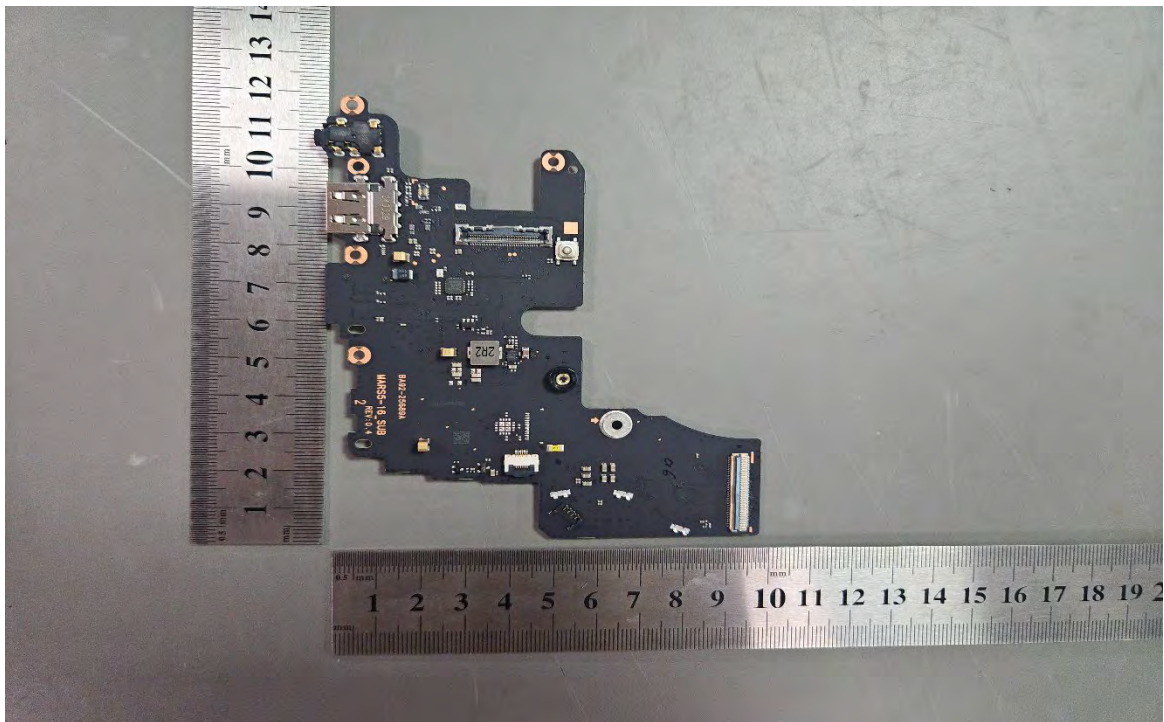
Internal EUT#20
