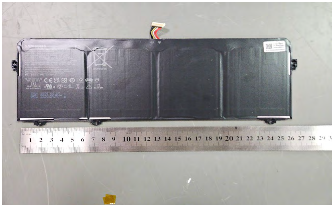
Internal EUT#18
