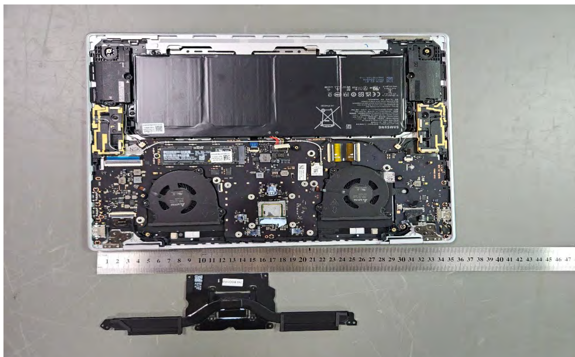
Internal EUT#2
