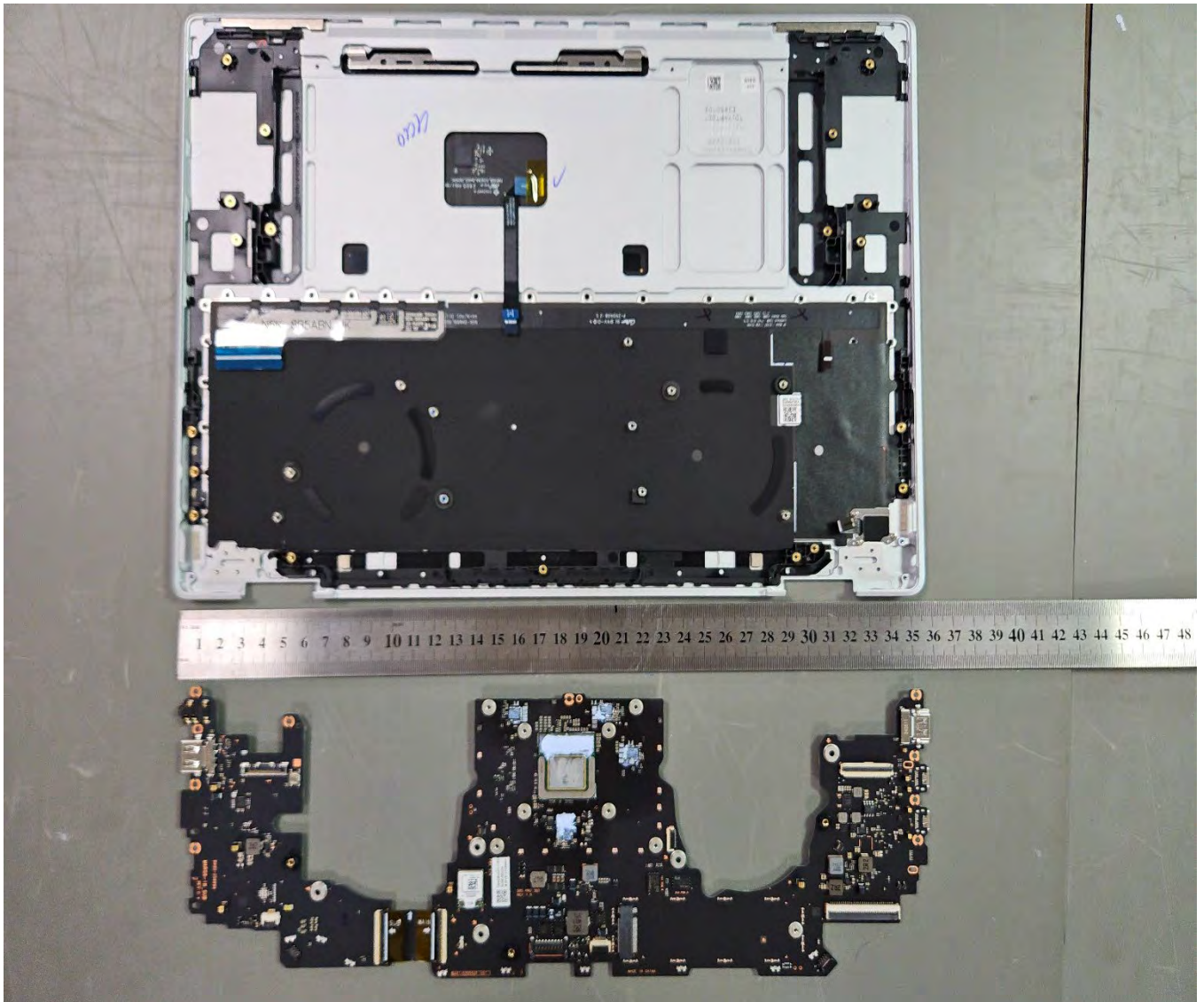
Internal EUT#24
