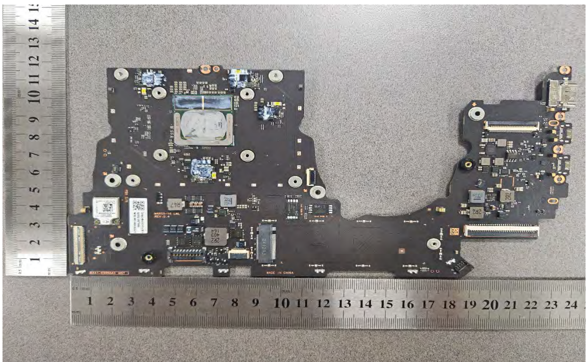
Internal EUT#29
