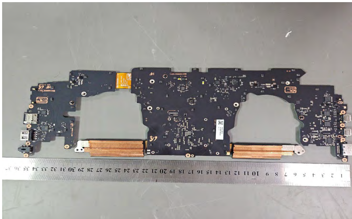
Internal EUT#8
