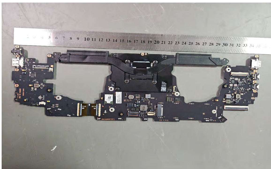
Internal EUT#6
