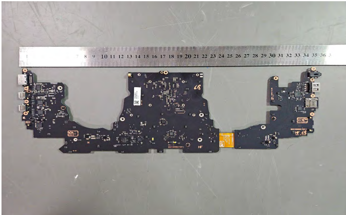
Internal EUT#25
