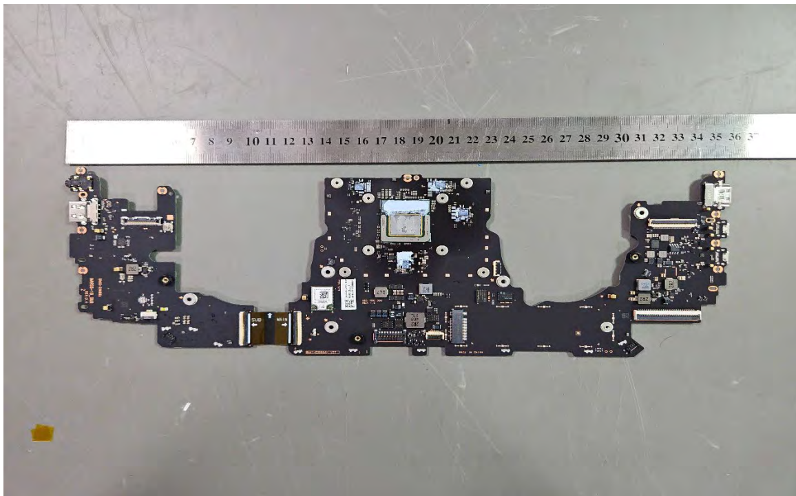
Internal EUT#22
