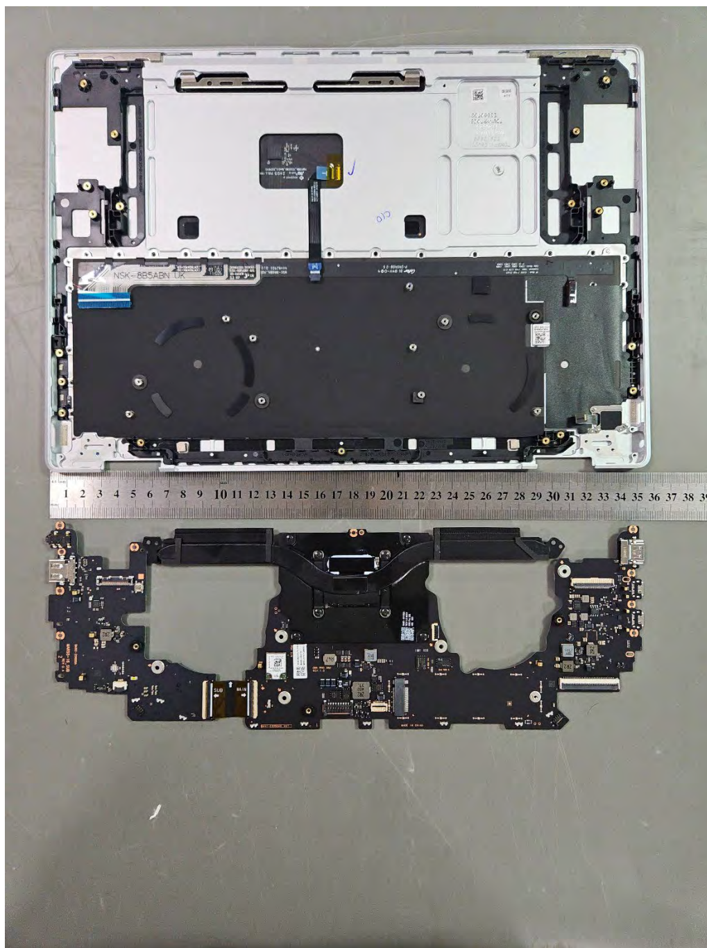
Internal EUT#7
