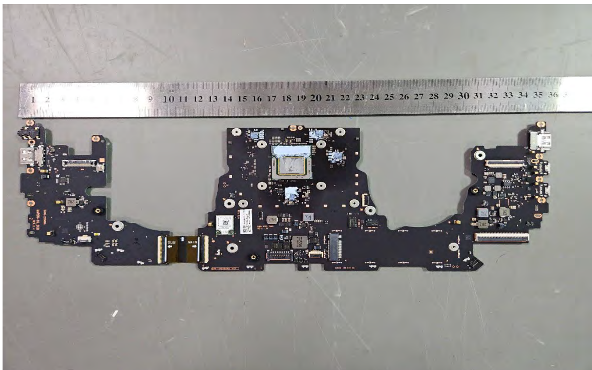
Internal EUT#23
