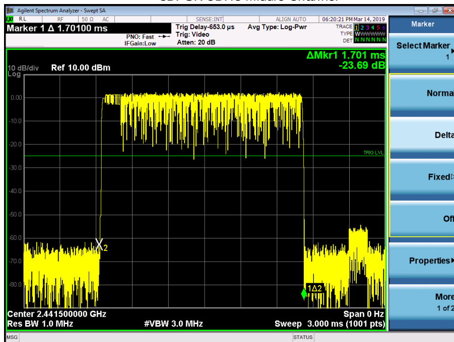
8DPSK 3DH3 Middle Channel
