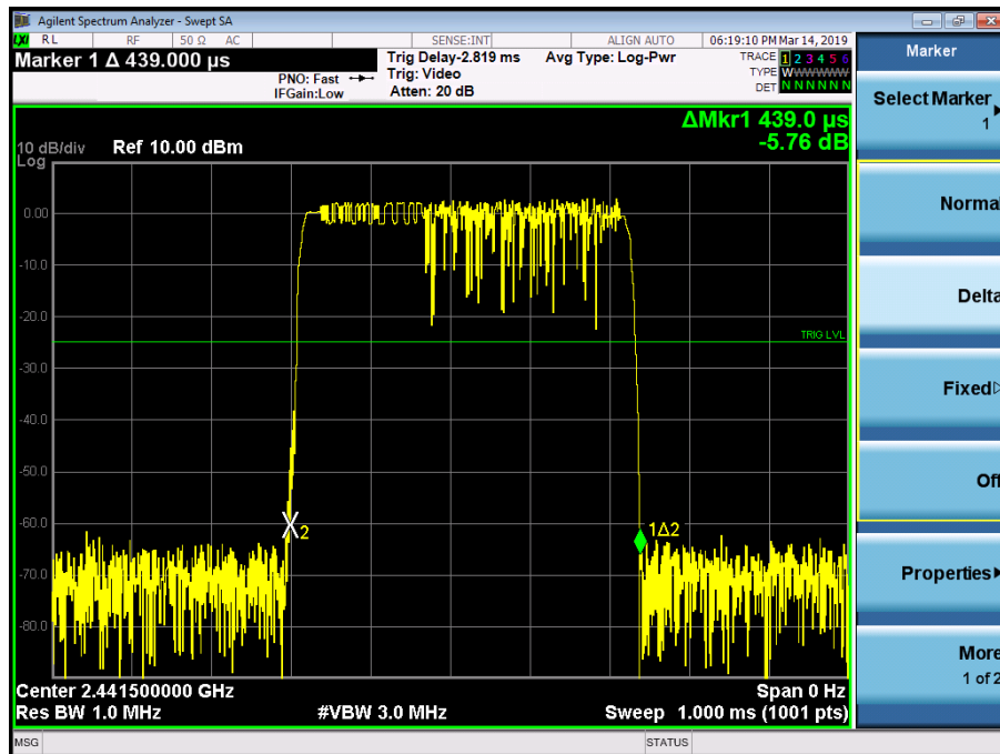
8DPSK 3DH1 Middle Channel
