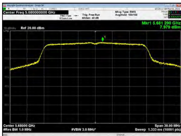
U-NII-2C, 802.11ac VHT20, Channel No.: 136
