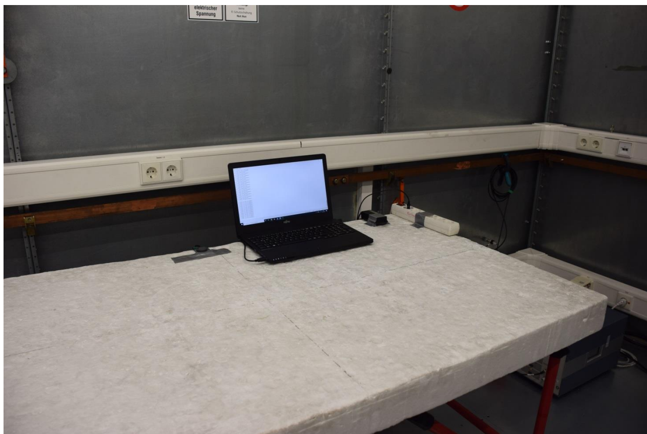
Picture 7: Test setup AC power line conducted emissions (front view)
