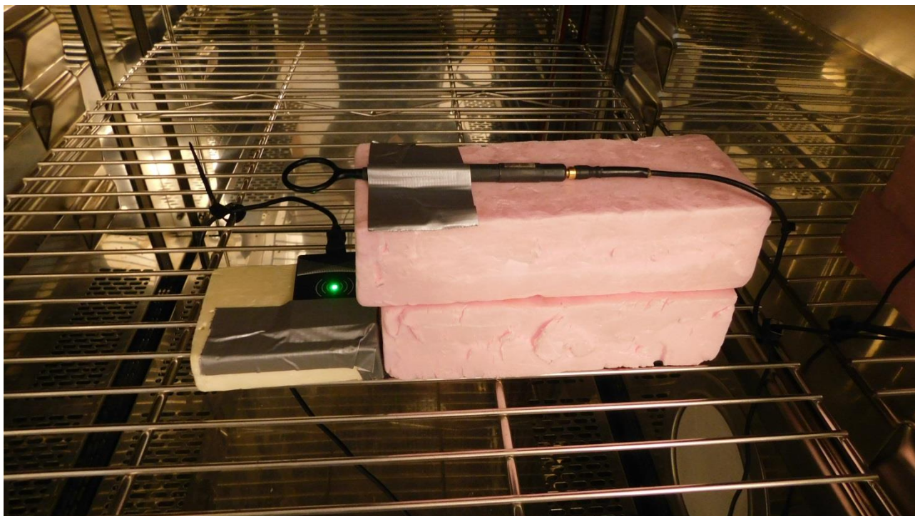
Picture 9: Climatic tests and bandwidth measurements
