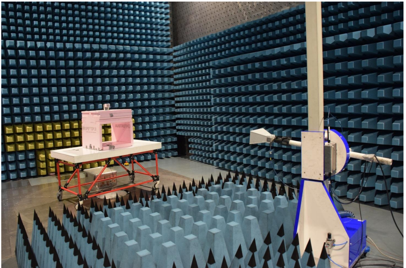
Picture 6: SAC, radiated emission test 1 GHz – 2 GHz (rear view)
