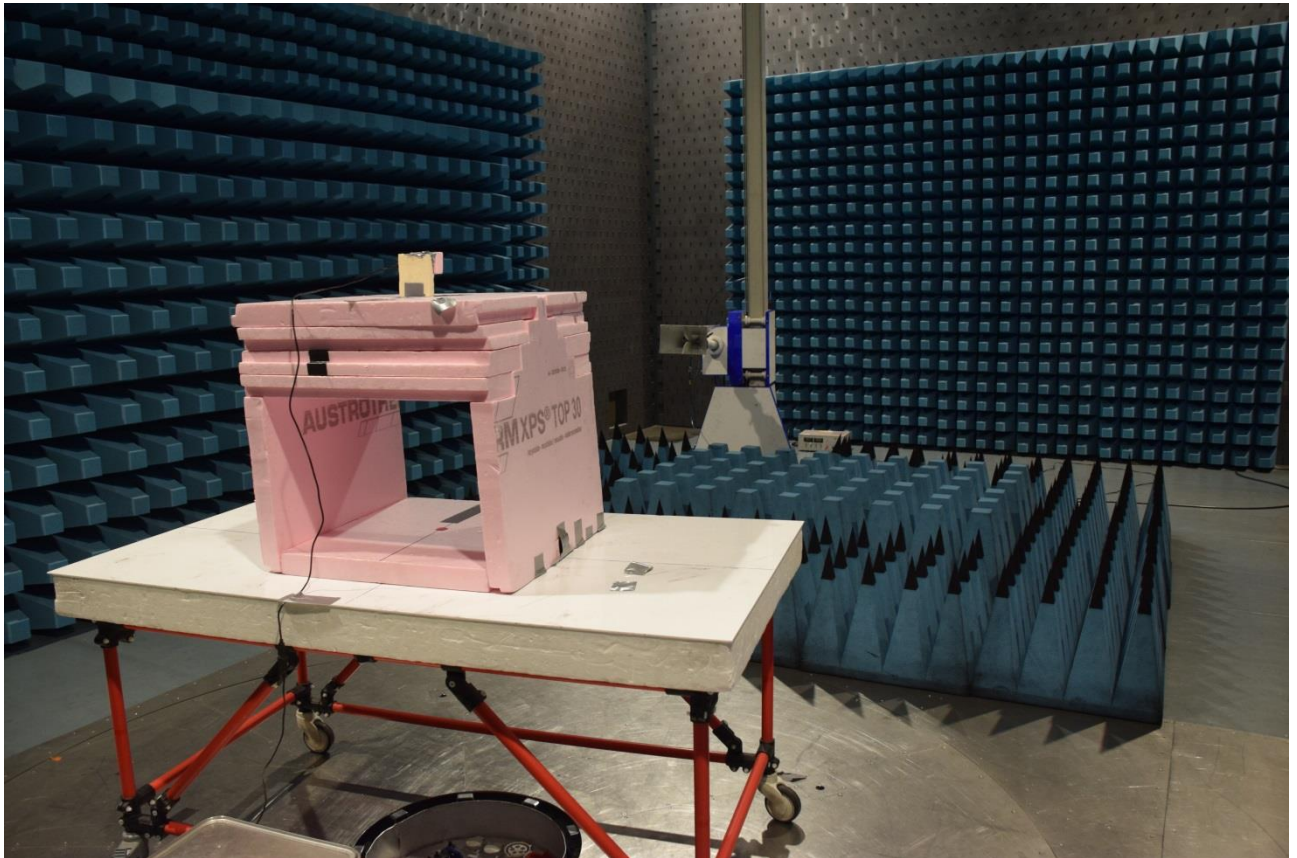
Picture 5: SAC, radiated emission test 1 GHz – 2 GHz (front view)
