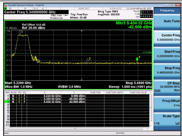
11N40SISO-Ant1-5230-PASS
