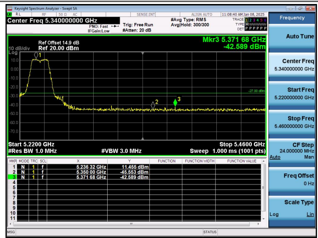
11N20SISO-Ant1-5240-PASS
