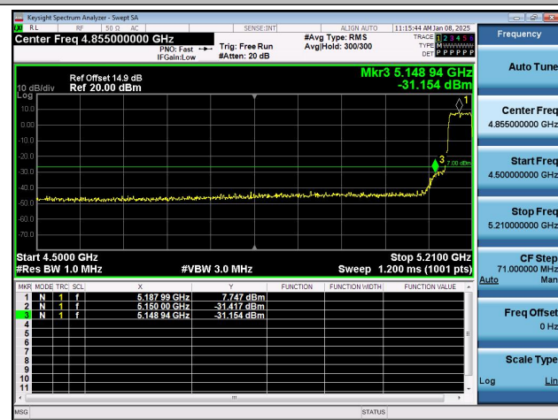
11N40SISO-Ant1-5190-PASS
