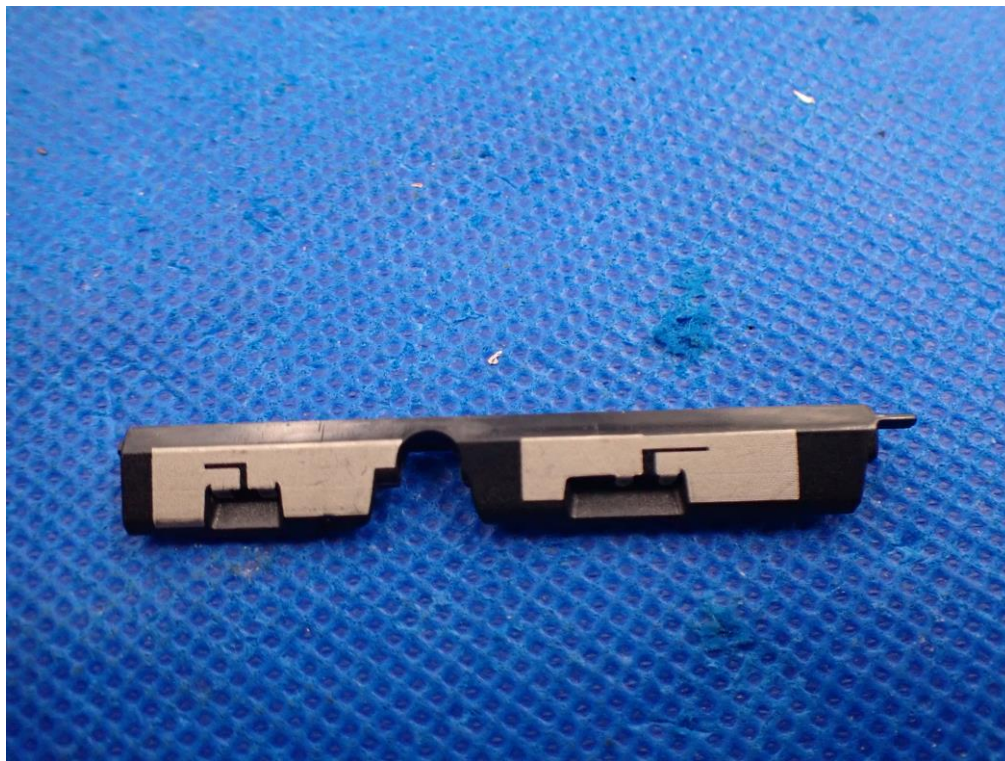
n41:TRX0&amp; n78:RX1 ANTENNA
