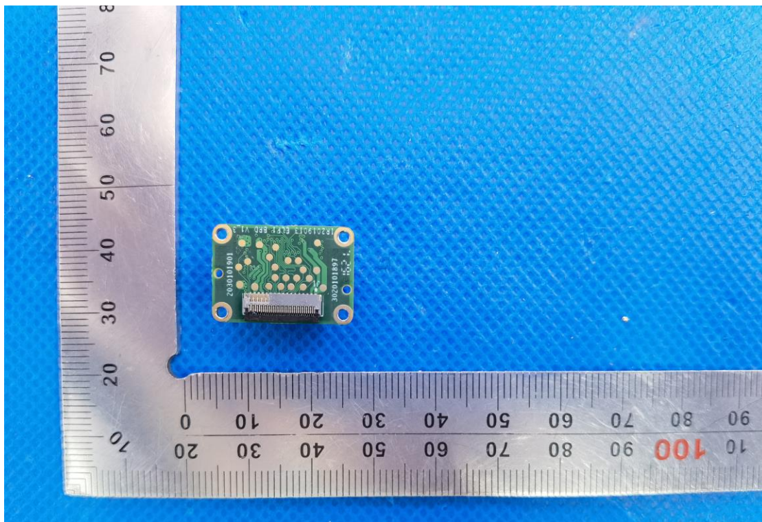
INTERNAL VIEW OF EUT(FIGURE 14)
