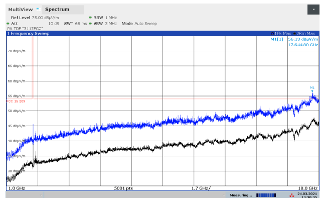
Radiated Emissions 1 - 18 GHz, 2441 MHz, GFSK, VP
