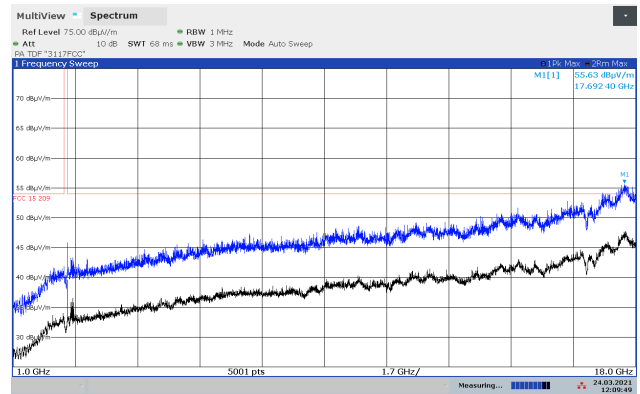
Radiated Emissions 1 - 18 GHz, 2480 MHz, GFSK, VP
