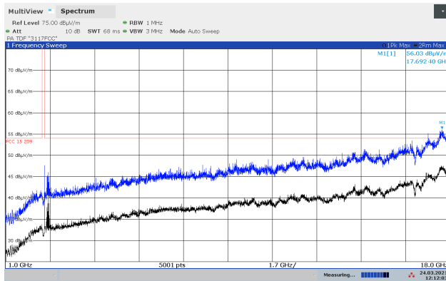
Radiated Emissions 1 - 18 GHz, 2480 MHz, GFSK, HP
