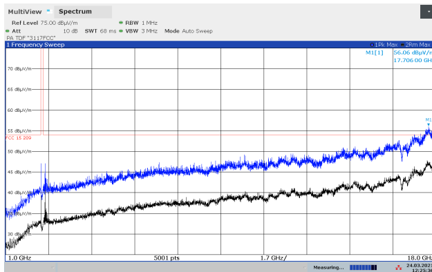
Radiated Emissions 1 - 18 GHz, 2402 MHz, GFSK, HP
