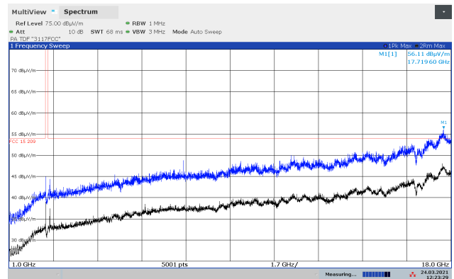
Radiated Emissions 1 - 18 GHz, 2402 MHz, GFSK, VP
