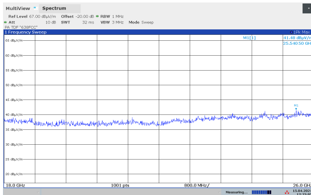
Pre-scan 18 - 26 GHz, 2441 MHz, GFSK, @approx. 10cm
