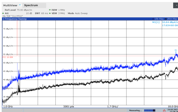
Radiated Emissions 1 - 18 GHz, 2441 MHz, GFSK, HP
