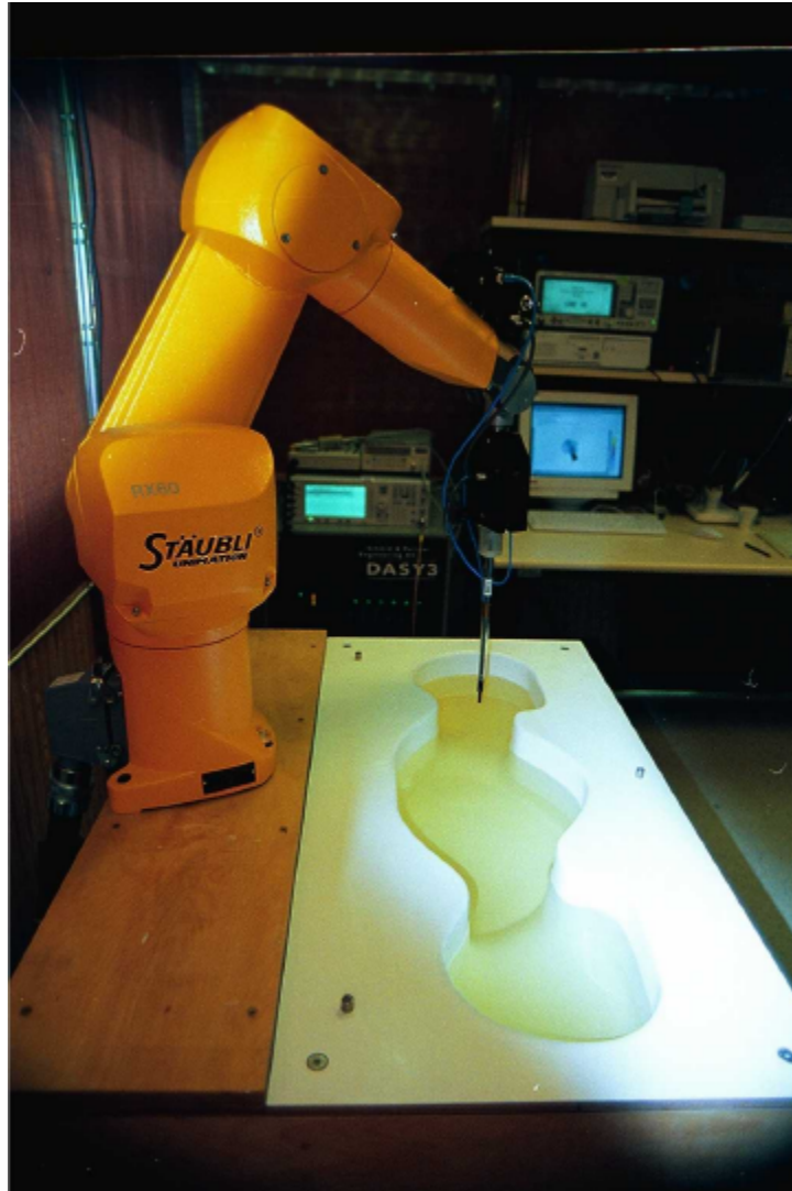
Photo 1 – DASY3 System
