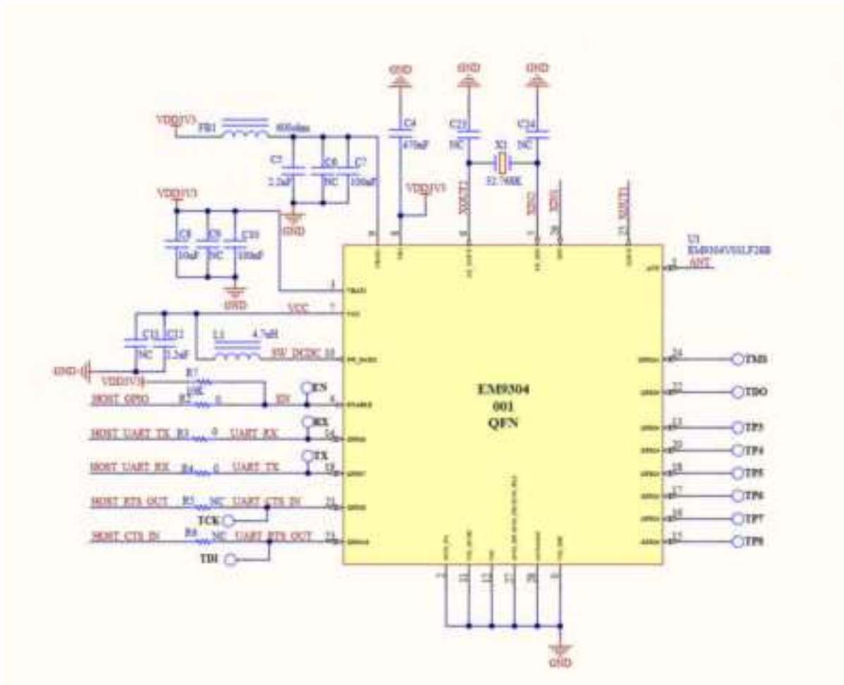
Figure 7:Chip Configurationt
