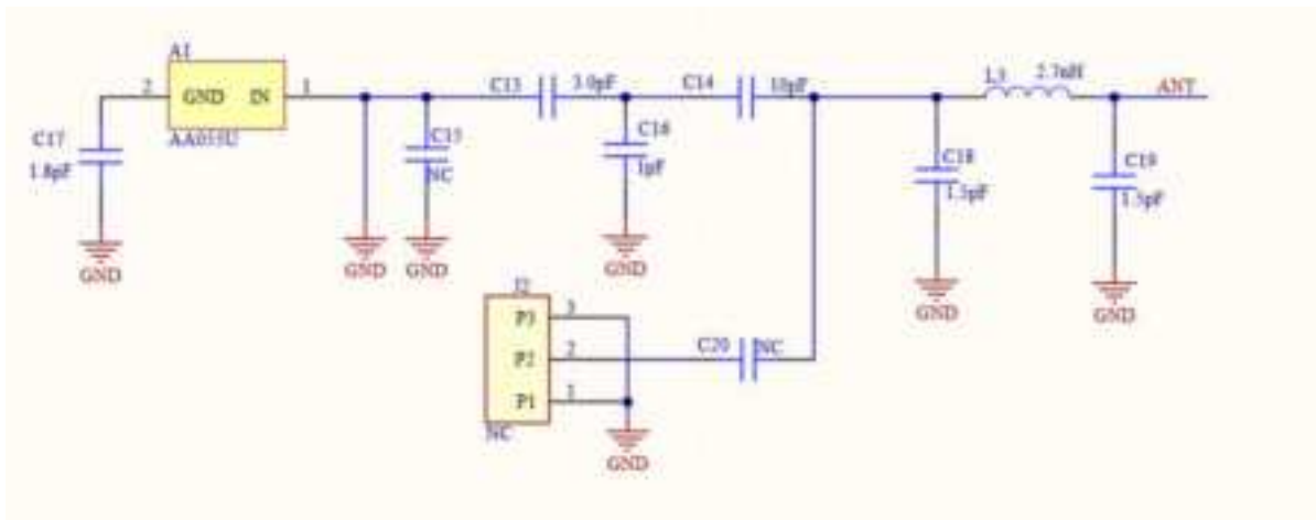
Figure 8: Matching Circuit
