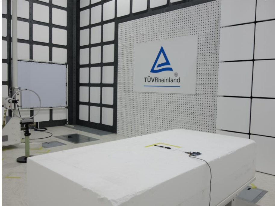
Photograph 27: Test Setup for Spurious Emissions (Back View 1, WiFi)
