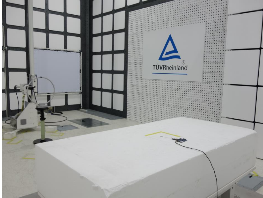
Photograph 11: Test Setup for Spurious Emissions (Back View 1, WiFi)
