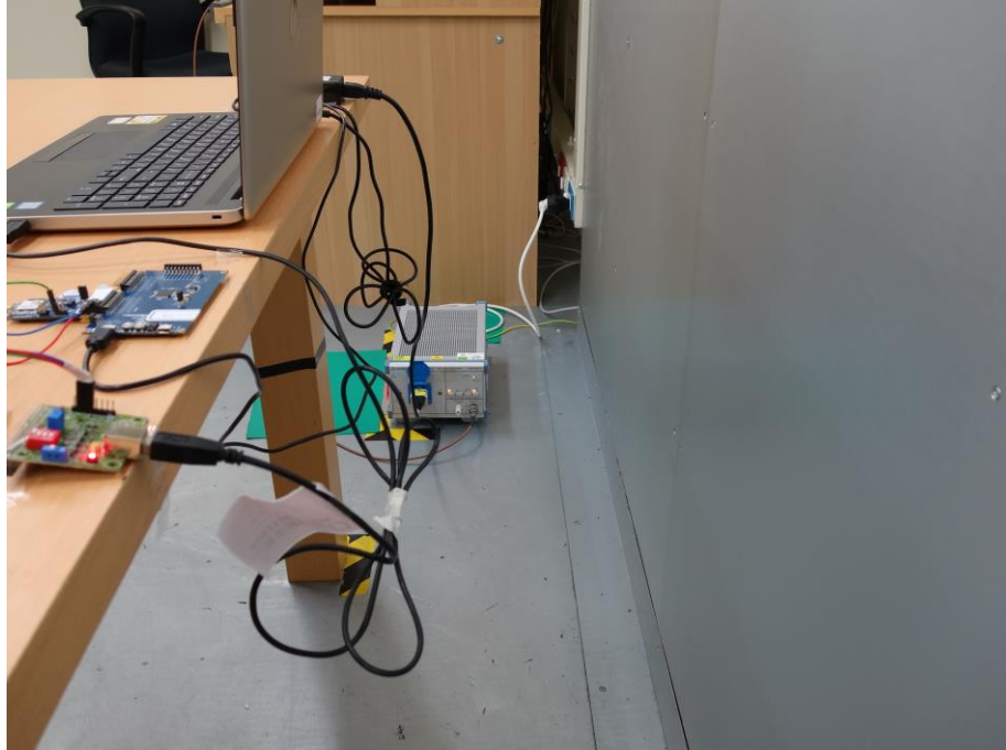
Photograph 24: Test Setup for Mains Conducted Emissions (Back View, BLE)
