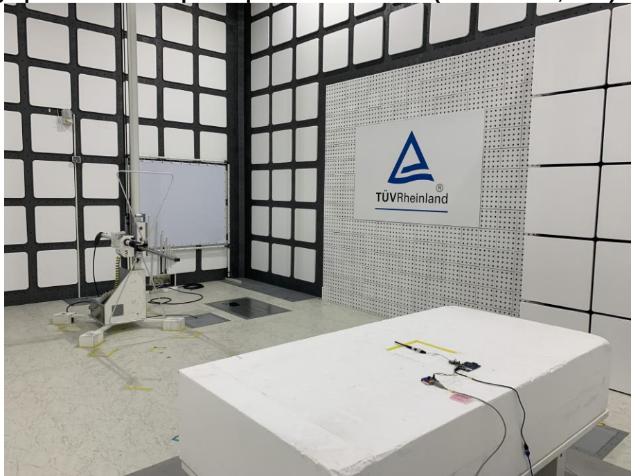
Photograph 20: Test Setup for Spurious Emissions (Back View 2, BLE)
