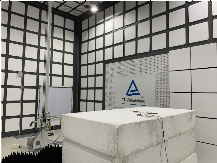
Photograph 22: Test Setup for Spurious Emissions (Back View 4, BLE)
