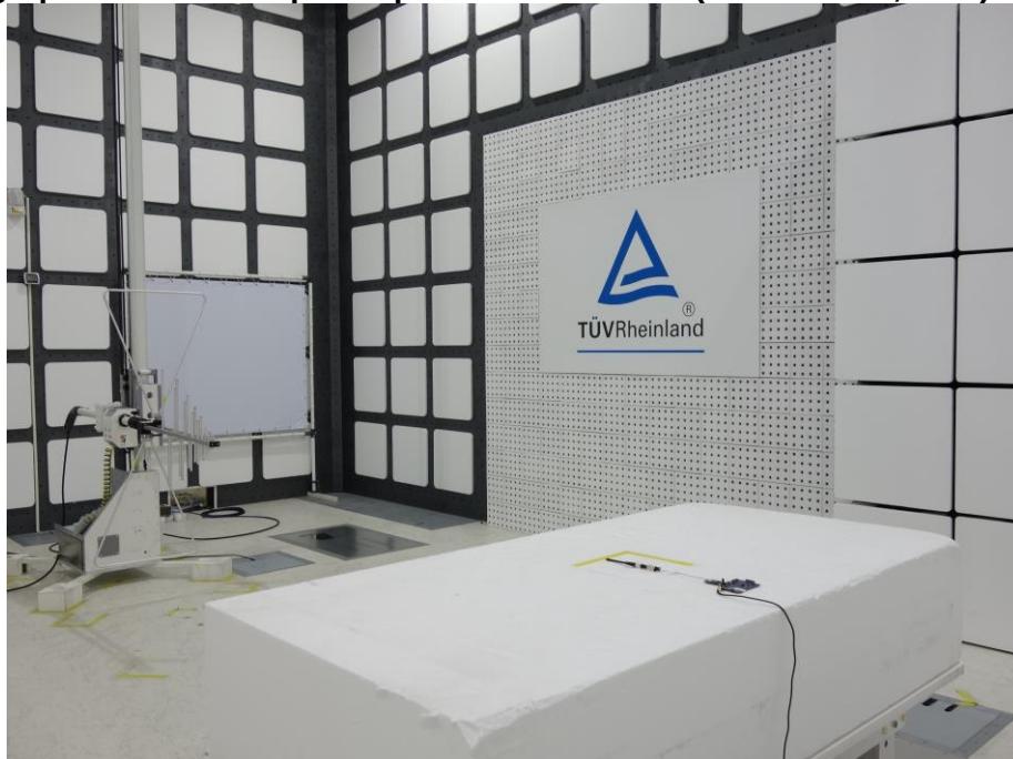
Photograph 28: Test Setup for Spurious Emissions (Back View 2, WiFi)
