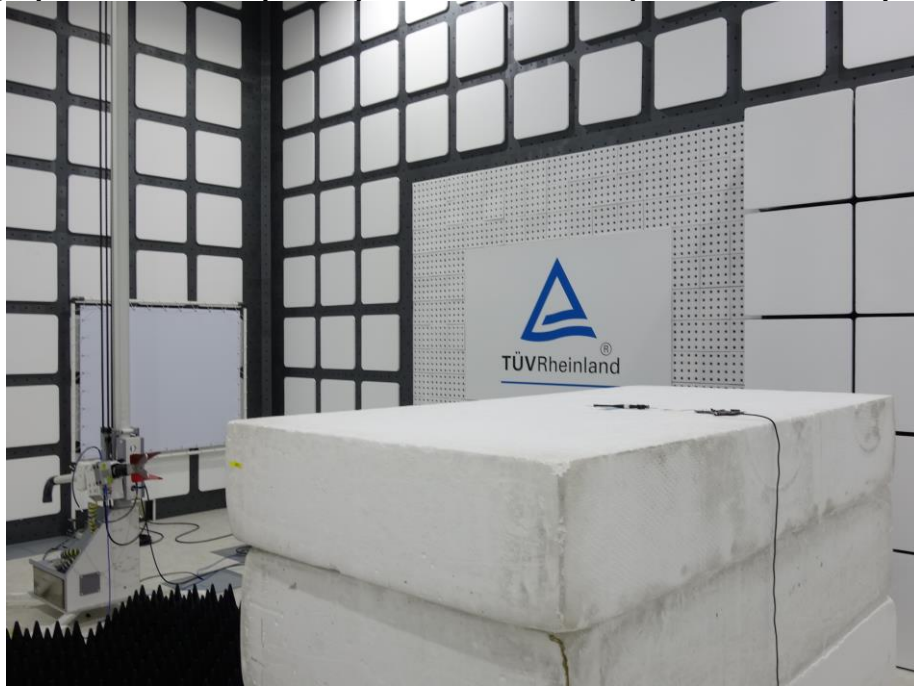
Photograph 29: Test Setup for Spurious Emissions (Back View 3, WiFi)
