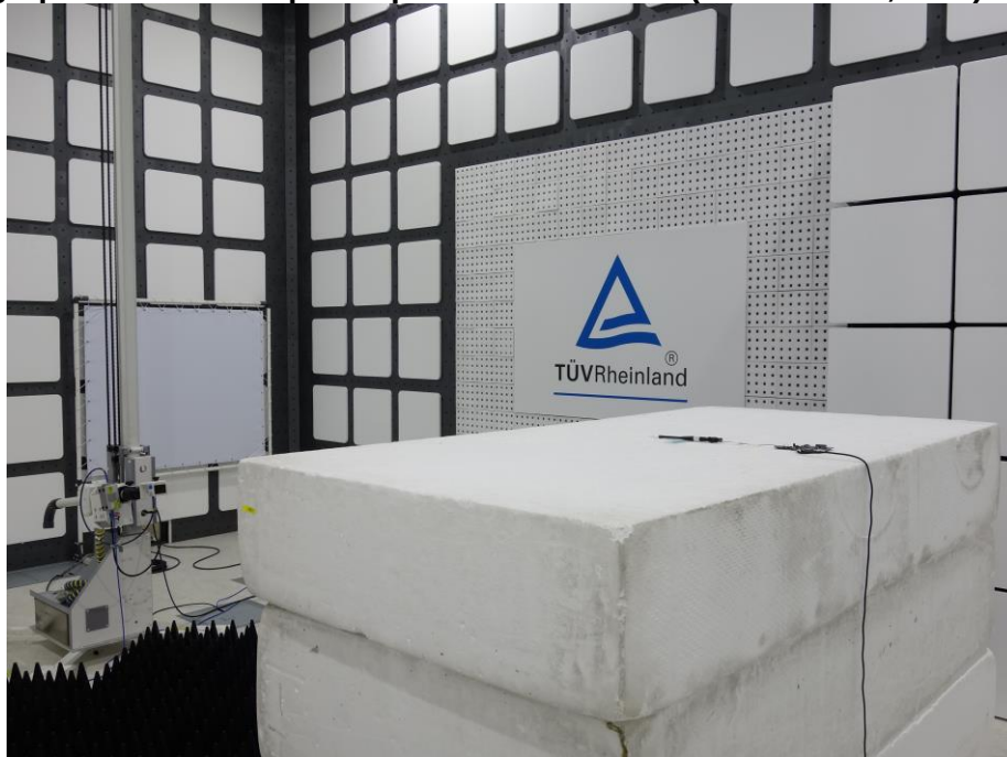
Photograph 30: Test Setup for Spurious Emissions (Back View 4, WiFi)
