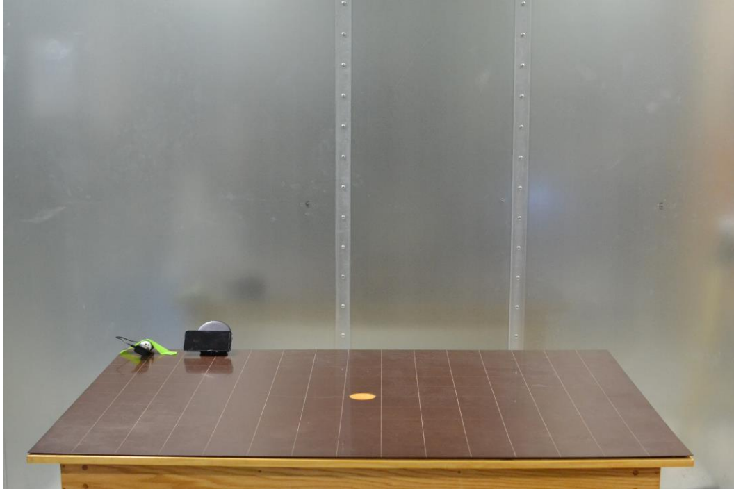
Figure 7. Test Setup – ACLC WCP – <30MHz
