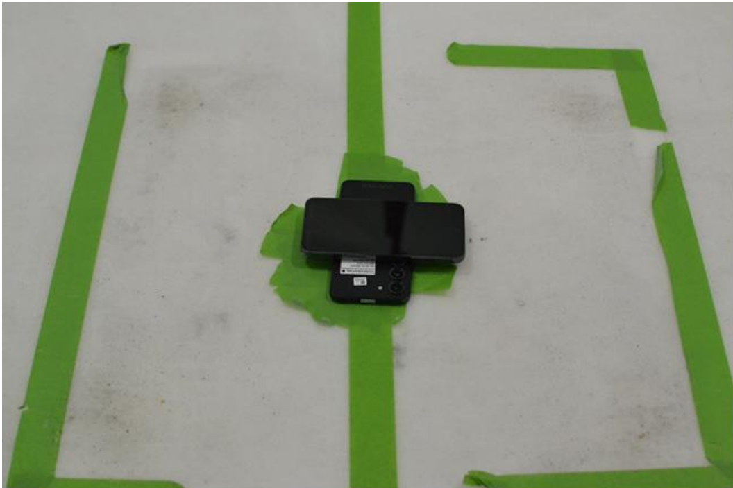
Figure 24. Test Setup – WPT Position – 30Hz-1GHz
