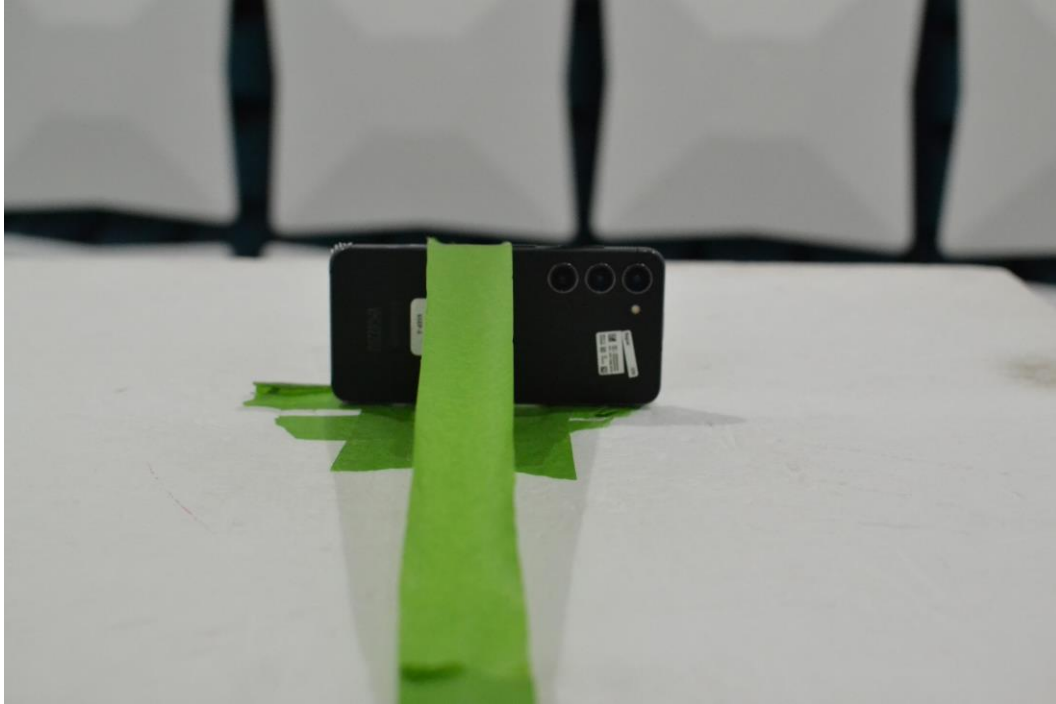
Figure 11. Test Setup – Y Position – 1GHz-18GHz
