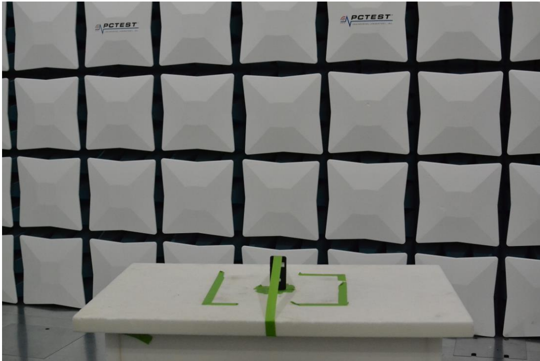
Figure 19. Test Setup – Z Position – 30MHz-1GHz
