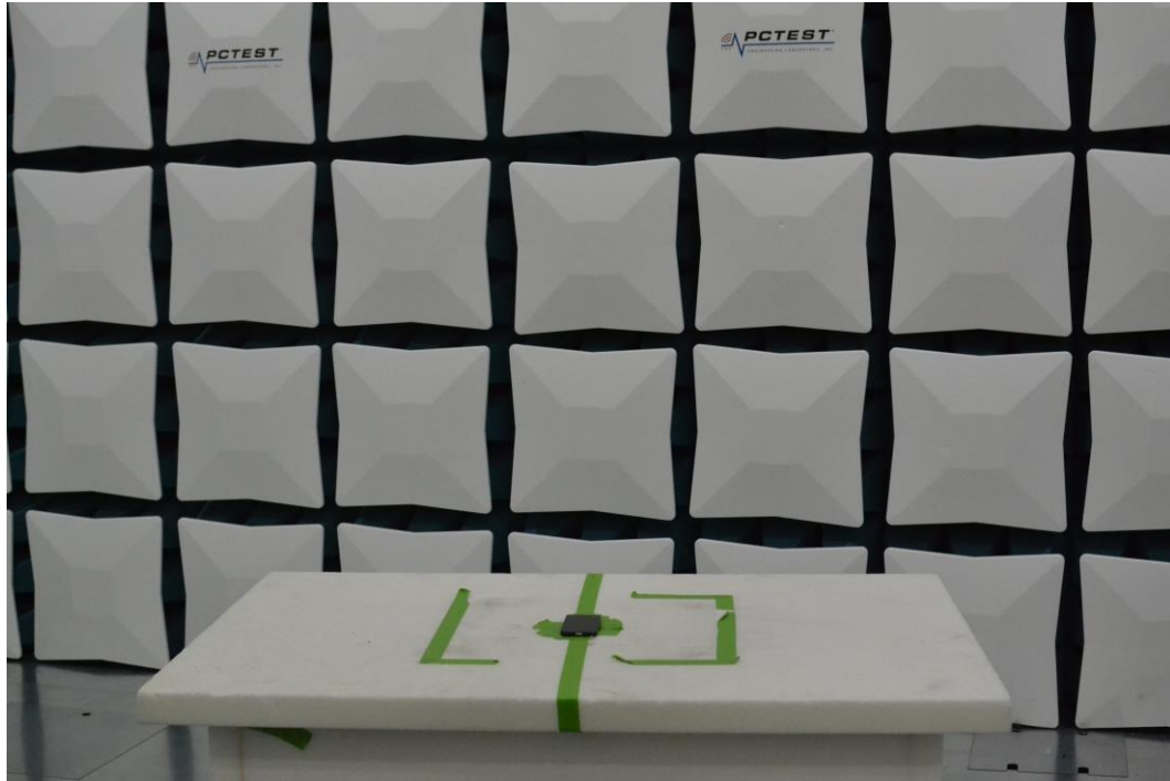
Figure 17. Test Setup – X Position – 30MHz-1GHz
