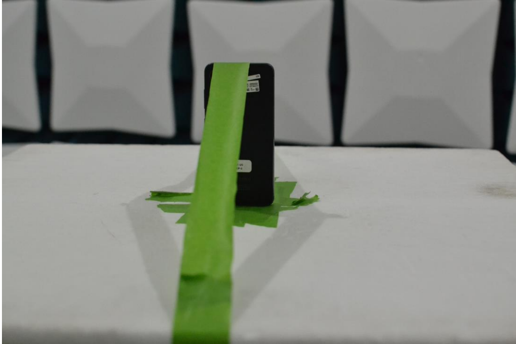
Figure 13. Test Setup – Z Position – 1GHz-18GHz
