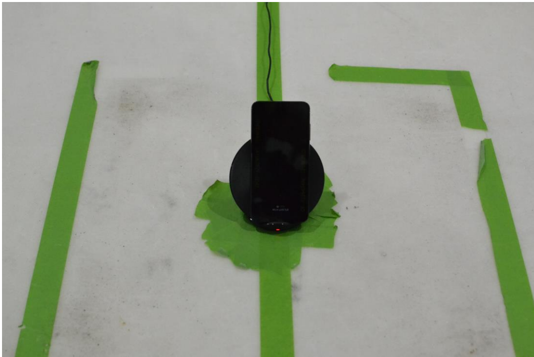
Figure 20. Test Setup – WCP Position – 30MHz-1GHz
