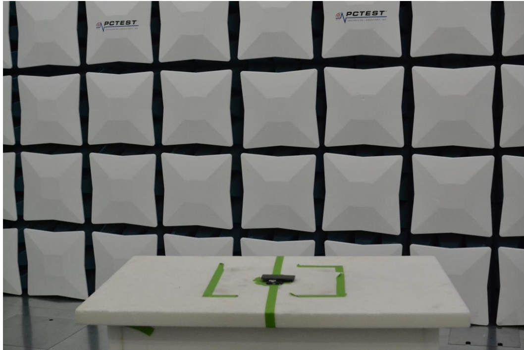
Figure 25. Test Setup – WPT Position – 30Hz-1GHz
