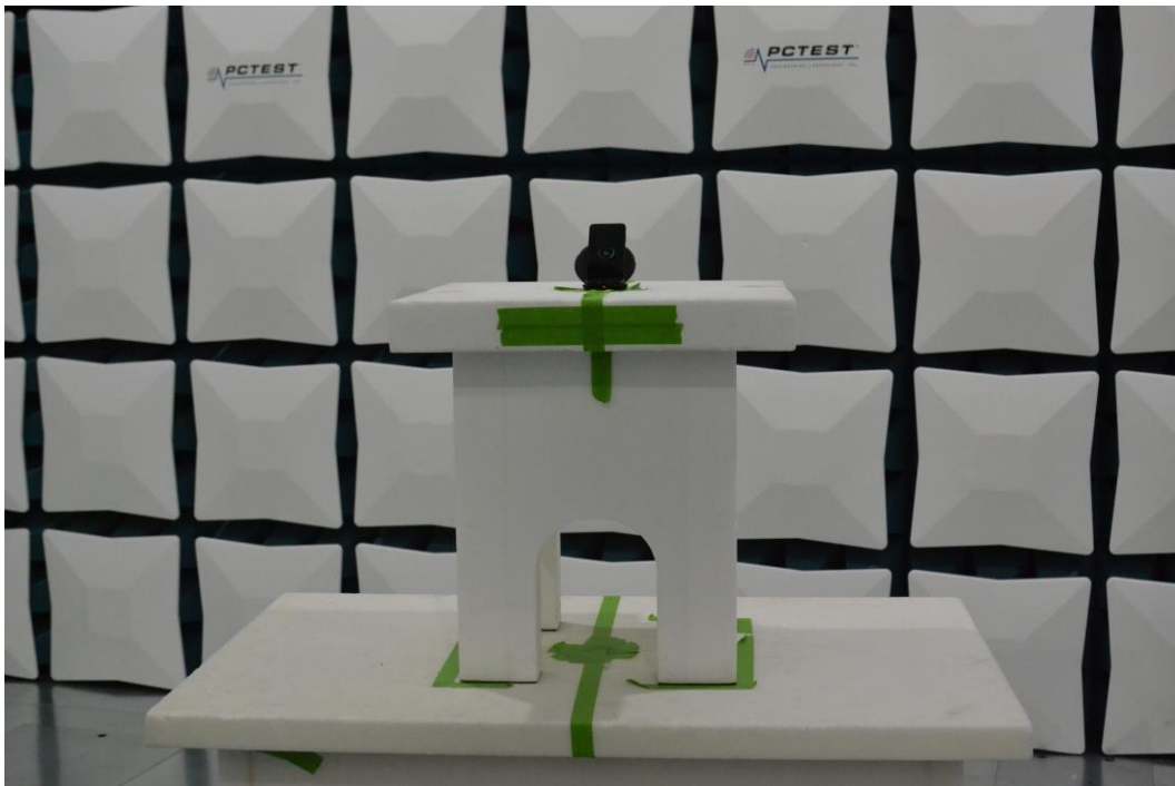
Figure 16. Test Setup – WCP Position – 1GHz-18GHz
