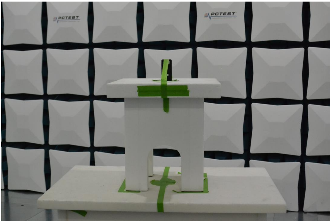
Figure 14. Test Setup – Z Position – 1GHz-18GHz
