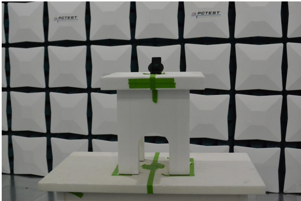
Figure 22. Test Setup – WPT Position – 1GHz-18GHz
