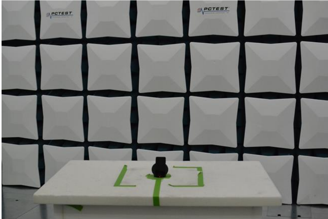
Figure 21. Test Setup – WCP Position – 30MHz-1GHz
