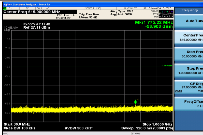
Band4-10MHz-16QAM-20000-1RB#0-30~1000MHz
