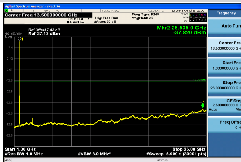
Band4-15MHz-QPSK-20175-1RB#0-1000~26000MHz
