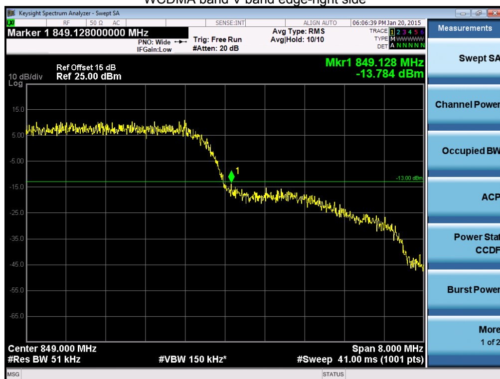
WCDMA band V band edge-right side
