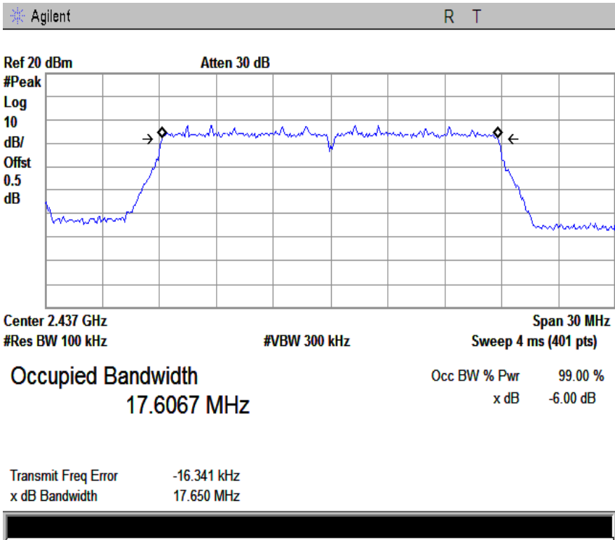
N20-6 6dB
