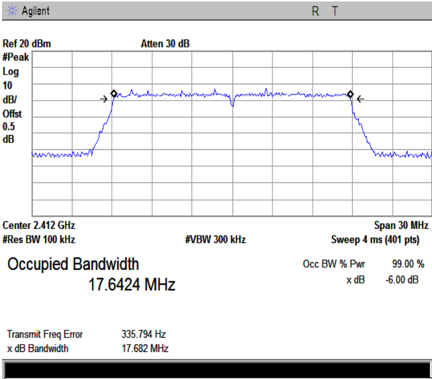
N20-1 6dB
