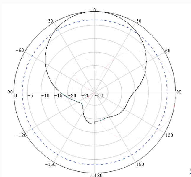
E Plane
