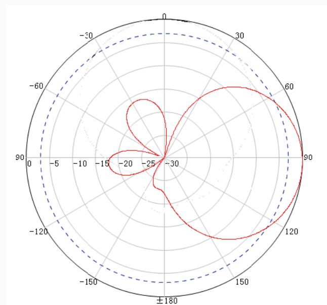
H Plane
