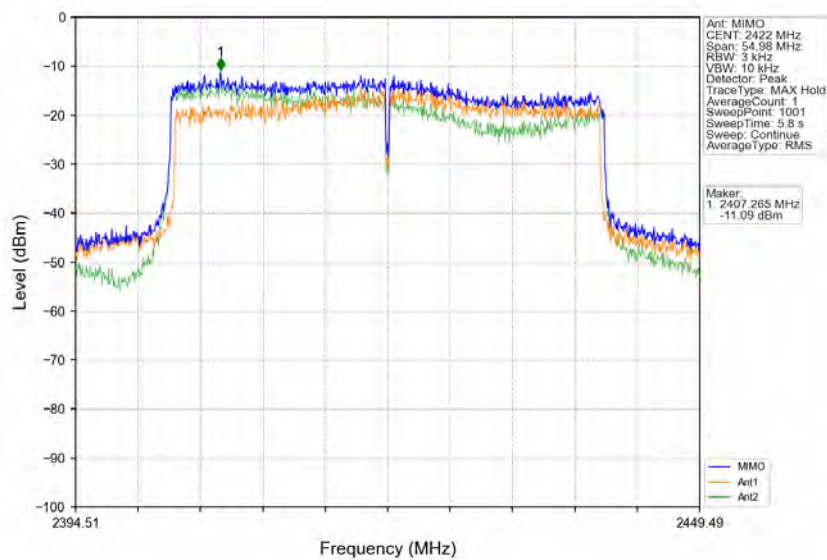
802.11ax(HEW40)_LCH_2422MHz_RU484_Left_MIMO_NTNV
