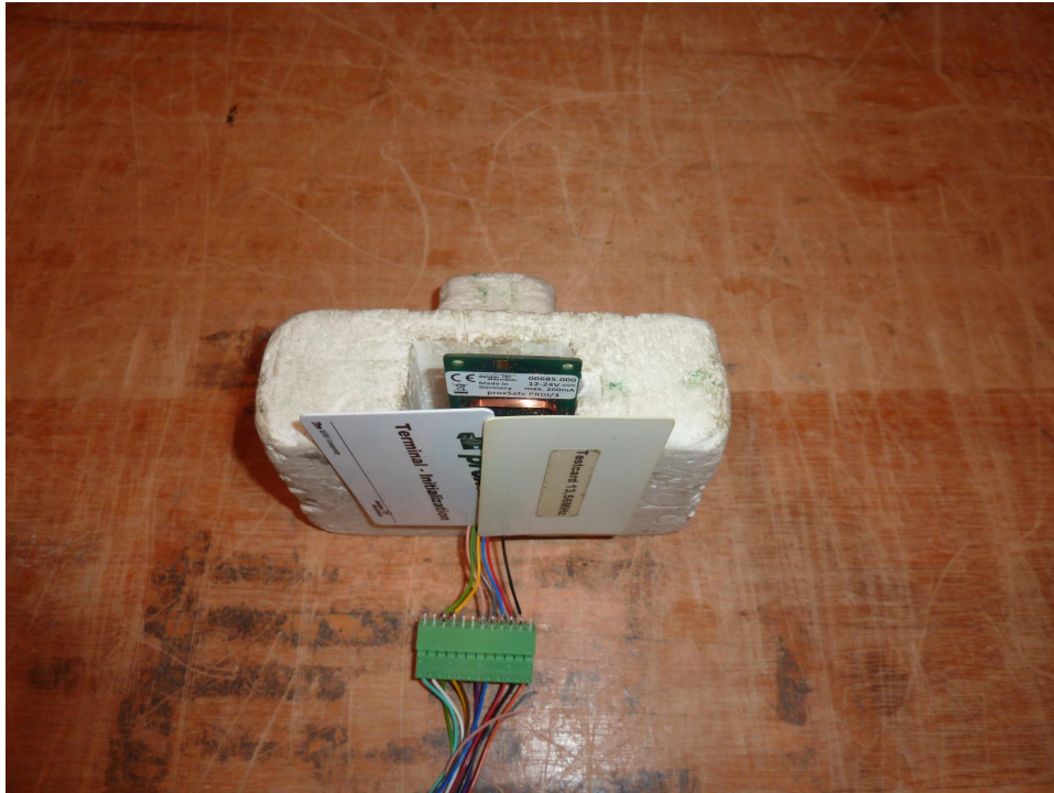
170664ah3: EUT setup
