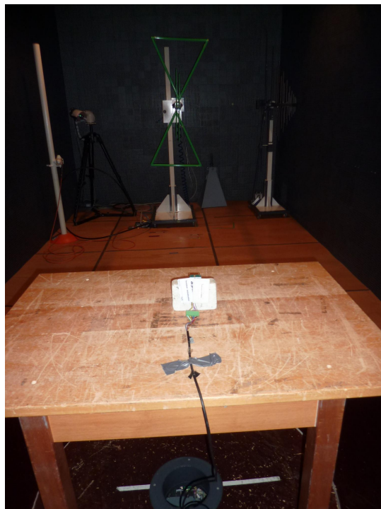
170664ah2: Preliminary radiated measurement anechoic chamber 30MHz to 1000 MHz
