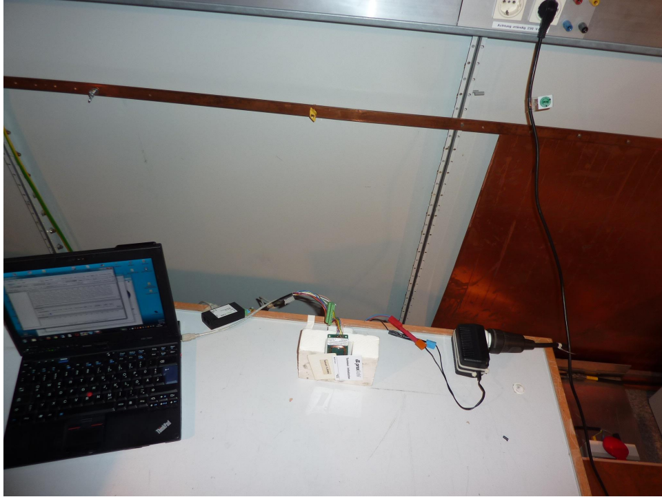
170664con1: Conducted measurement 1
