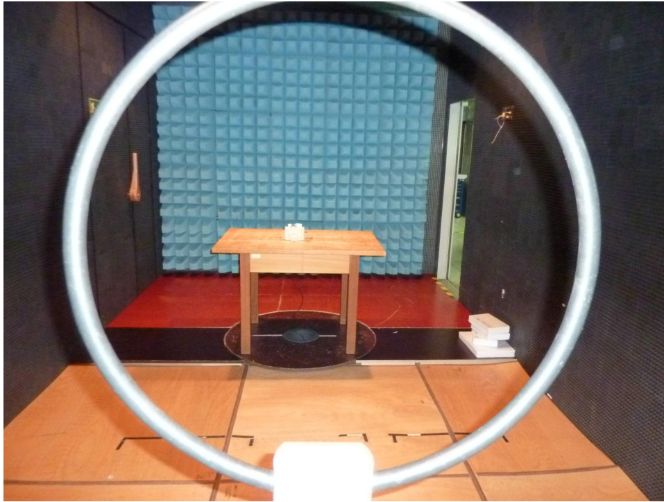
170664ah1: Preliminary radiated measurement anechoic chamber 9 kHz to 30 MHz
