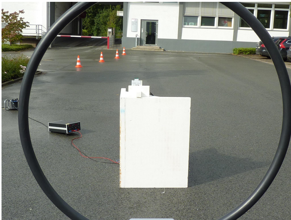
170664outdoor: Final radiated measurement outdoor test site 9 kHz to 30 MHz
