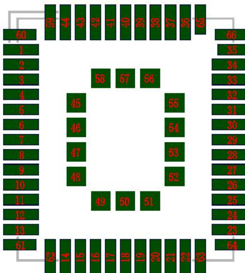
Figure 3- 1 Pin configuration diagram
