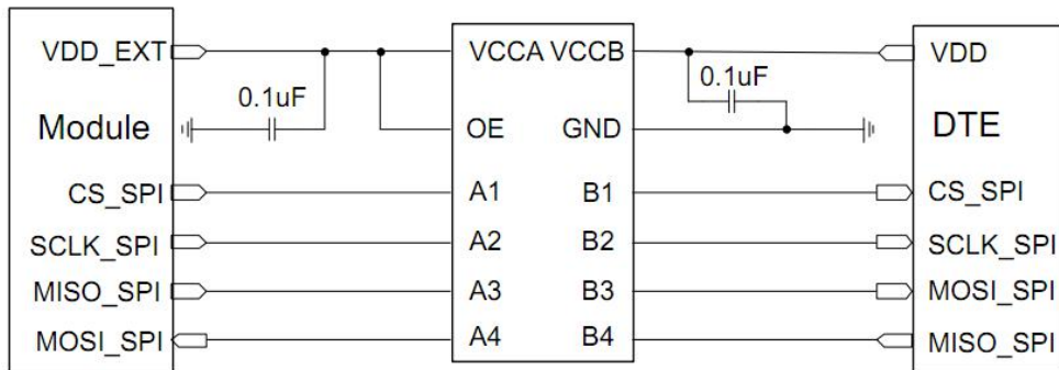
Figure 3-4 Reference circuit
