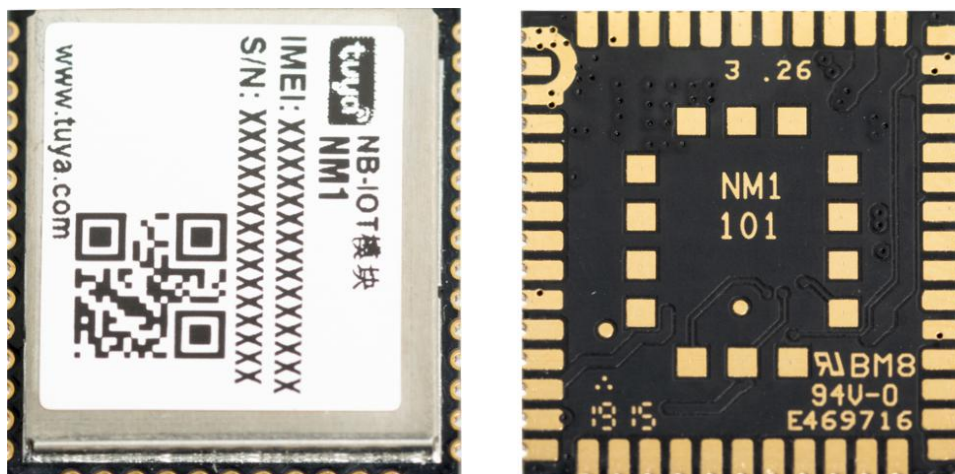
Figure 2-1 Product appearance
