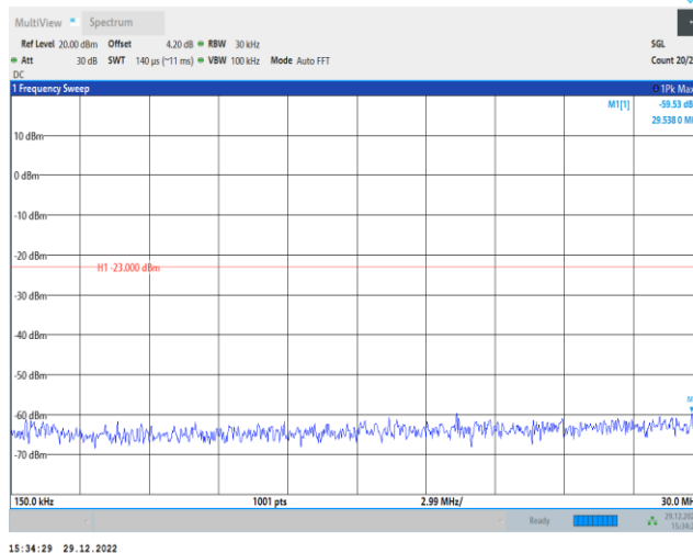
Band4-1312-0.15~30MHz
