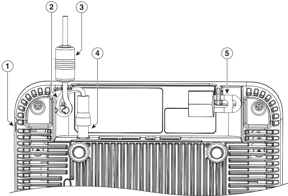
Figure 5 Routing the DC Power Cable
