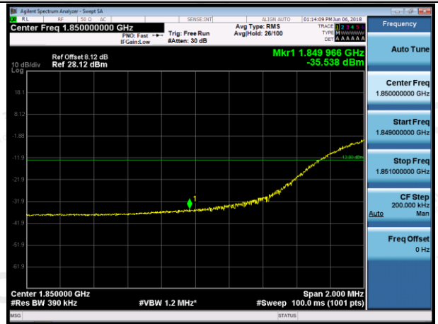
LCH_16QAM_100RB#0
