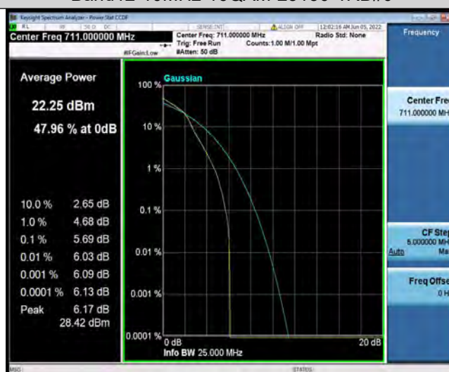
Band12-10MHz-16QAM-23130-27RB#0
