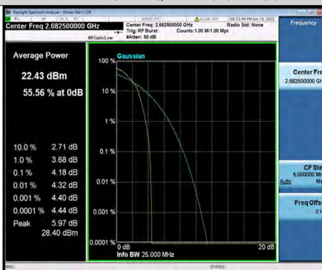
Band41-15MHz-QPSK-41515-75RB#0
