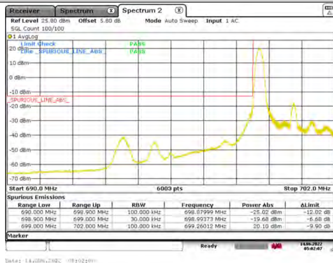
Band12-3MHz-QPSK-23025-15RB#0
