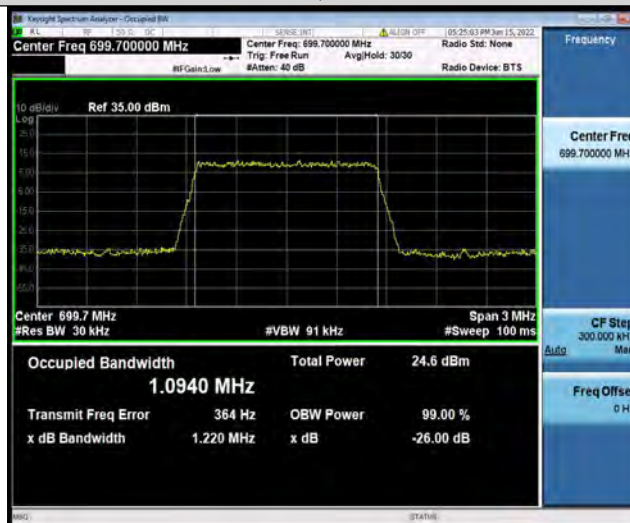
Band12-1.4MHz-QPSK-23095-6RB#0
