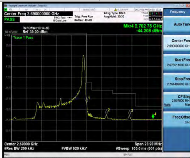
Band41-10MHz-16QAM-41540-27RB#23
