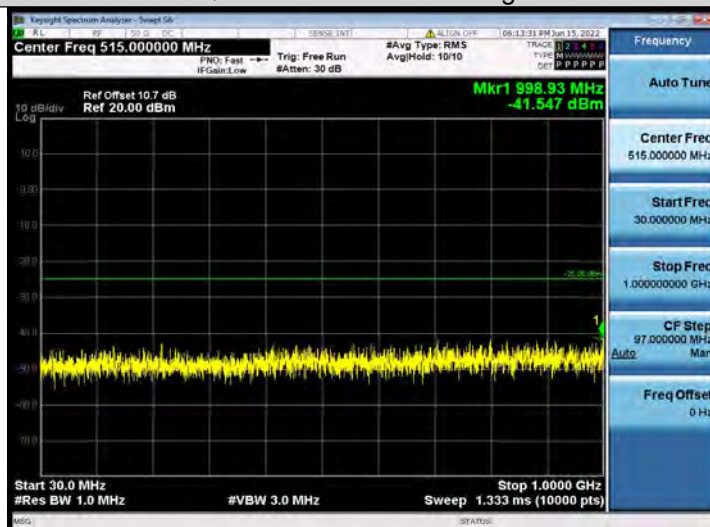
Band41-5MHz-QPSK-40620-1RB#0-Range1:30~1000MHz
