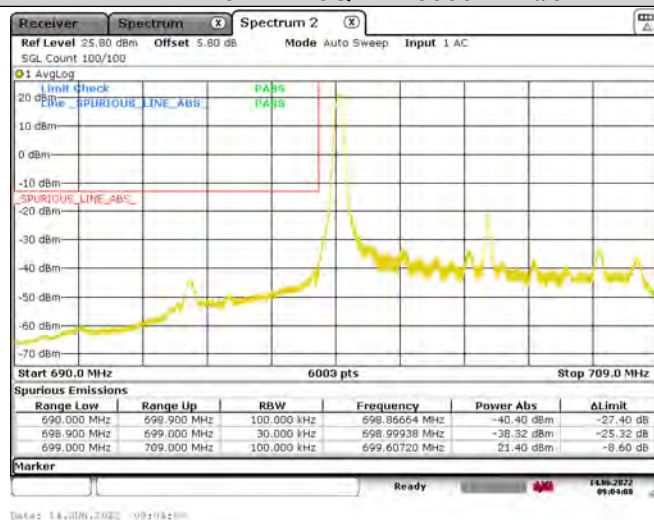
Band12-10MHz-16QAM-23060-27RB#0
