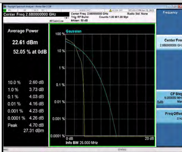
Band41-20MHz-16QAM-41490-27RB#0
