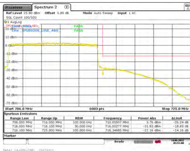
Band12-10MHz-16QAM-23060-1RB#0
