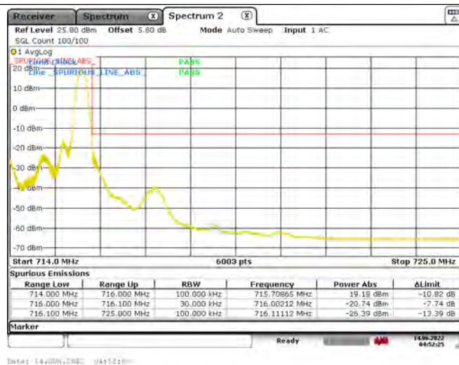
Band12-1.4MHz-16QAM-23173-6RB#0
