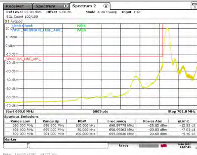
Band12-1.4MHz-QPSK-23017-6RB#0
