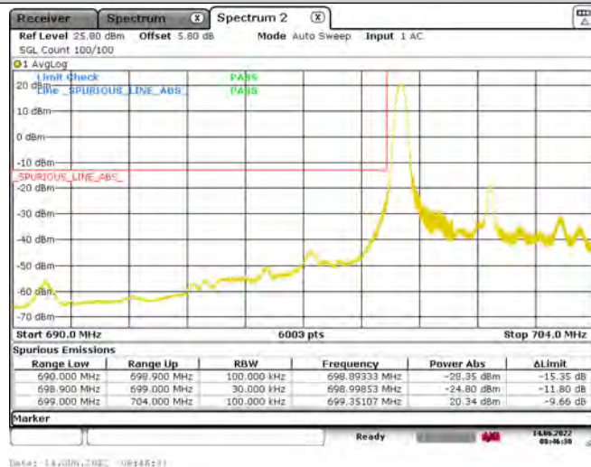
Band12-5MHz-QPSK-23035-25RB#0
