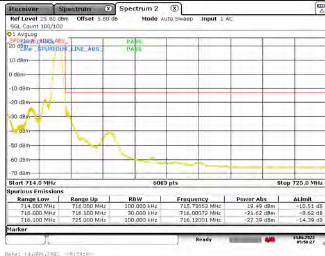
Band12-1.4MHz-QPSK-23173-1RB#5
