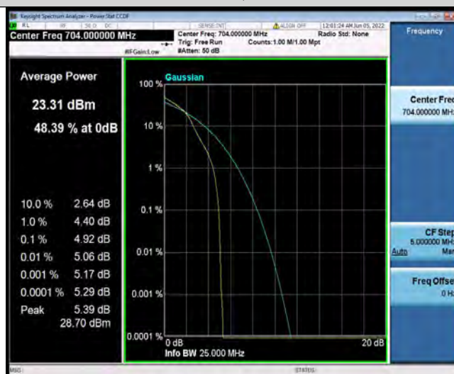
Band12-10MHz-16QAM-23060-27RB#0
