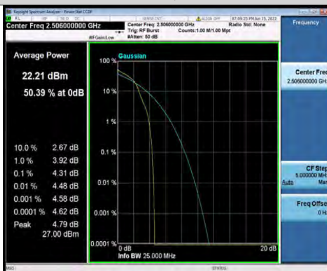
Band41-20MHz-16QAM-39750-27RB#0
