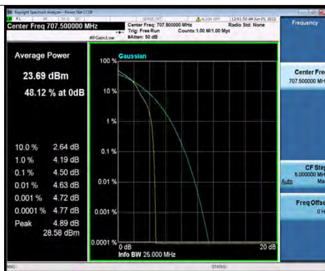
Band12-10MHz-16QAM-23095-27RB#0
