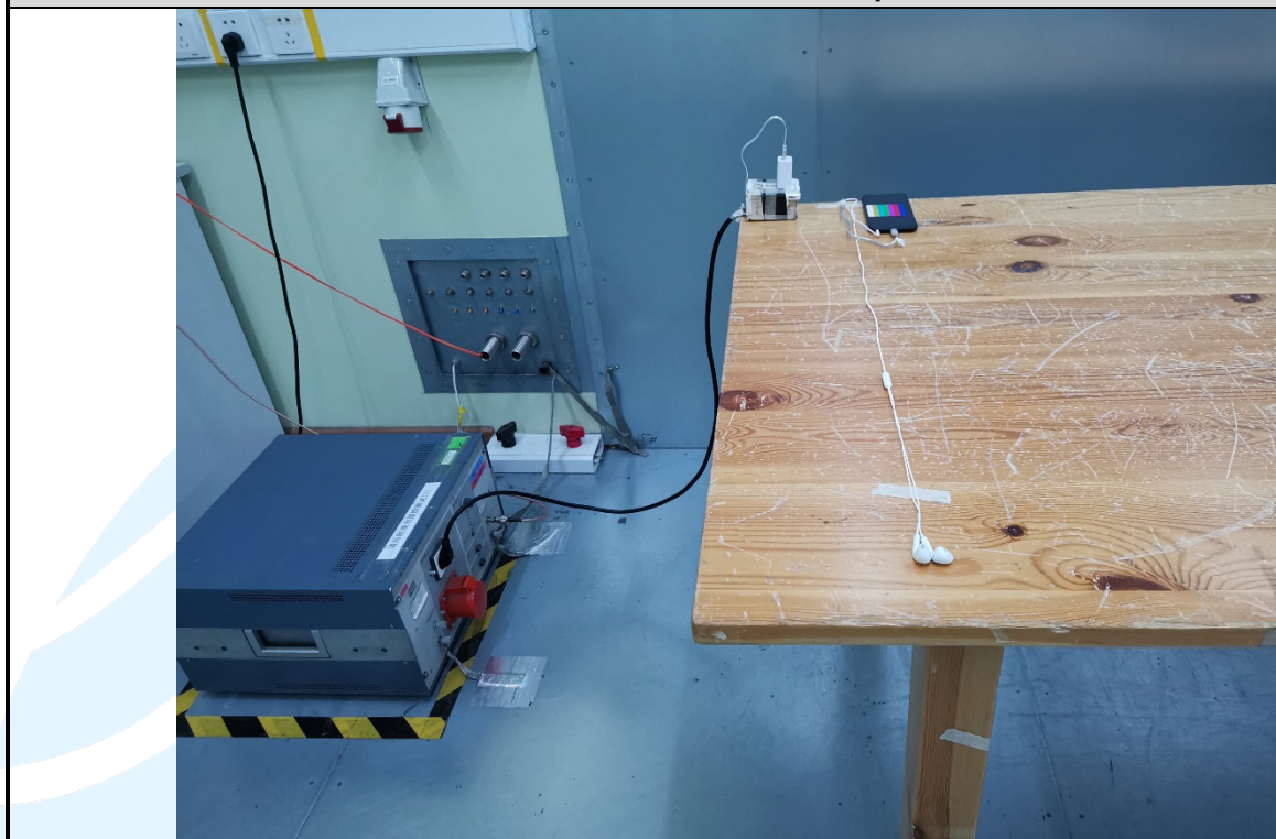
Conducted Emission Test Setup - Mode 1
