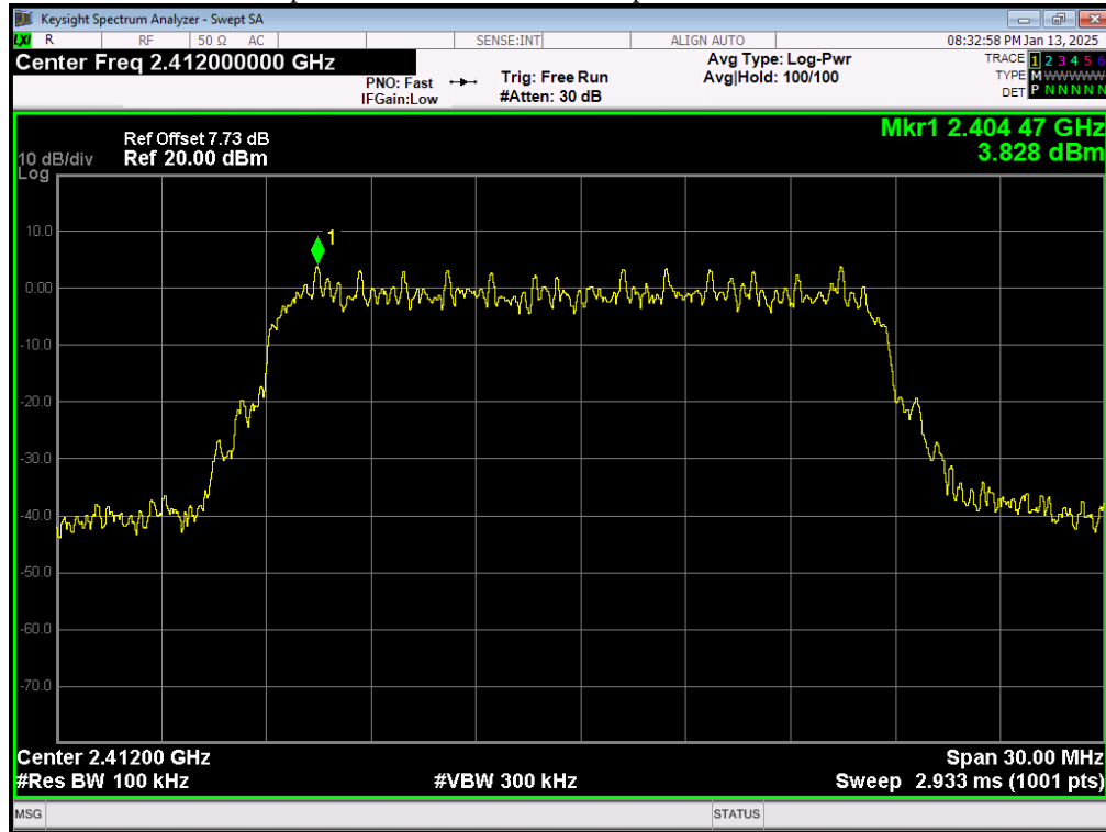
Tx. Spurious NVNT 802.11b 1Mbps 2412MHz Ant1 Ref
