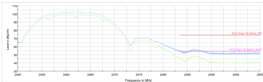
Fig.A.6.2.2 Transmitter Spurious Emission - Radiated (Power): 802.11b, ch11, 2.45 GHz - 2.50GHz
