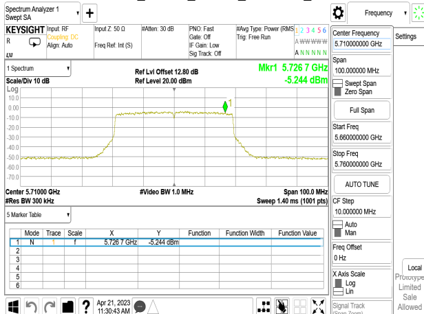
802.11ax_40MHz_Chain0_5710MHz_UNII 3
